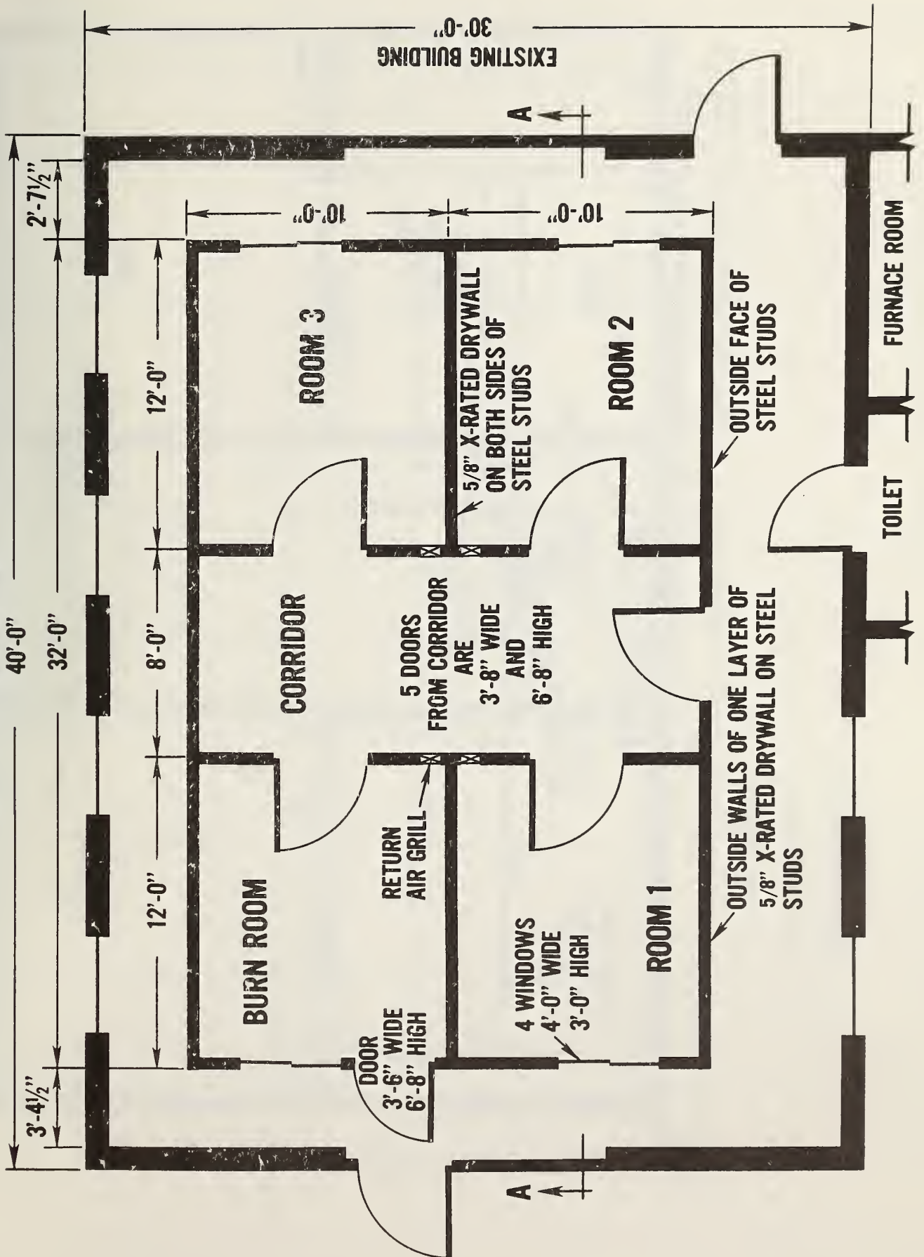
Figure 1. Floor plan of test facility
