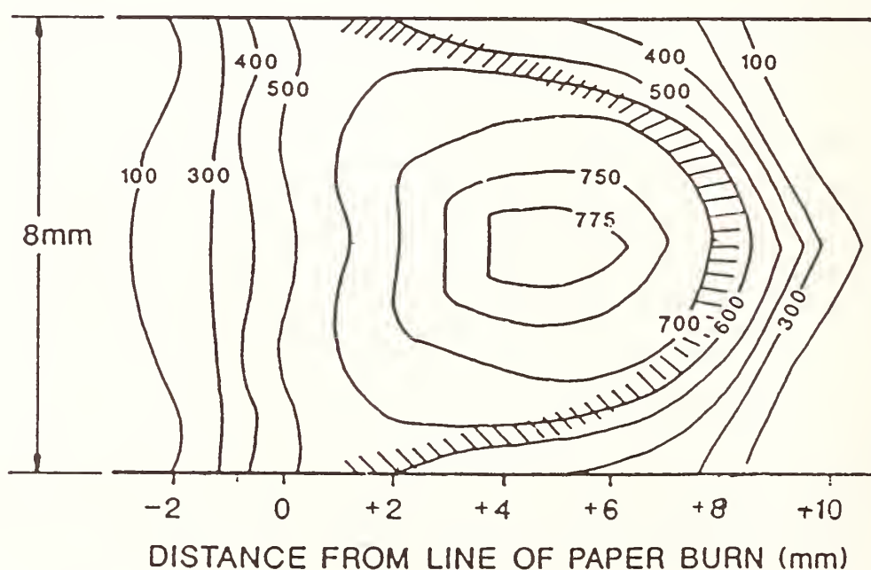
Figure 17. Isotherms in the gaseous part of the cigarette during quiet, steady burning. The shaded region indicates peak reaction rate; i.e., the glowing coal.
