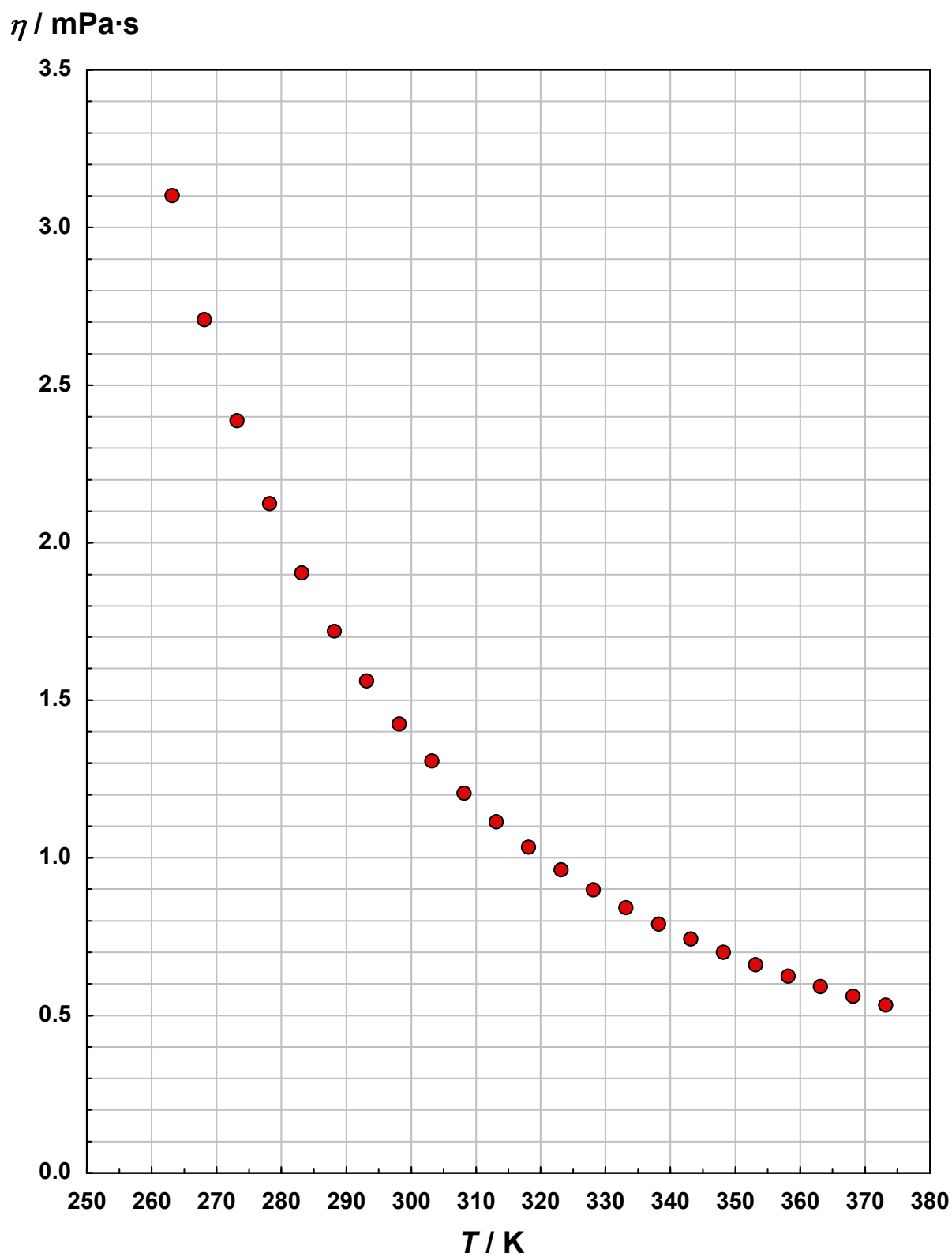
Figure 36: Measurements of the absolute viscosity of Jet-A-4648. The uncertainty is discussed in the text.
