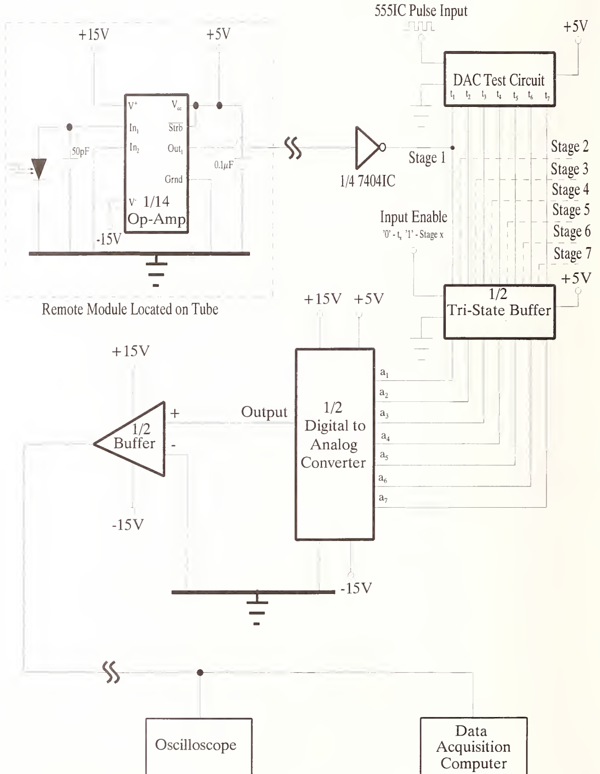
Figure 53. Logic diagram of photodiode sequencing system.
