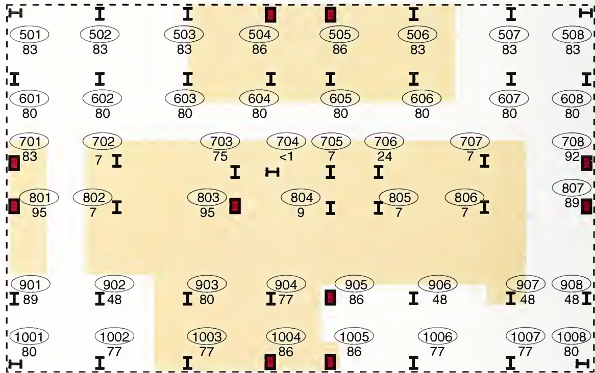
Figure E-7. Core column layout in WTC towers.
