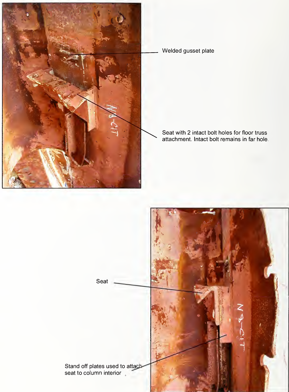
Figure 1-2. Floor truss seats shown from sample N-8.
