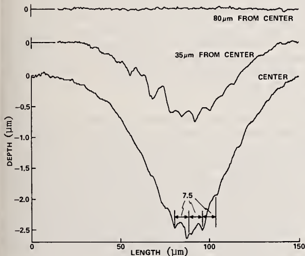
Figure 12. Selected surface profiles made on an exit surface damage crater in the KCl:EuCl specimen. The scans were made parallel to the machining grooves and perpendicular to the ripples in the damage site.
