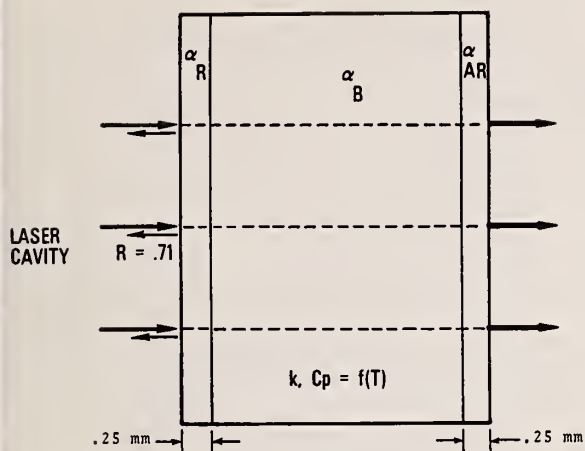
Figure 2. Analytical model of the coated zinc selenide.
