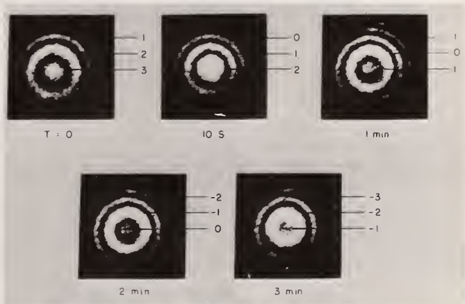
Figure 5. Interferogram of laser-induced optical distortion in polycrystalline CVD zinc selenide. Upper left photo shows reference fringe bias.
