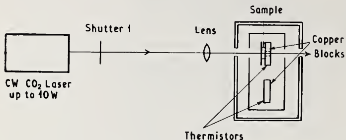
Figure 3. Schematic of absorption apparatus.
