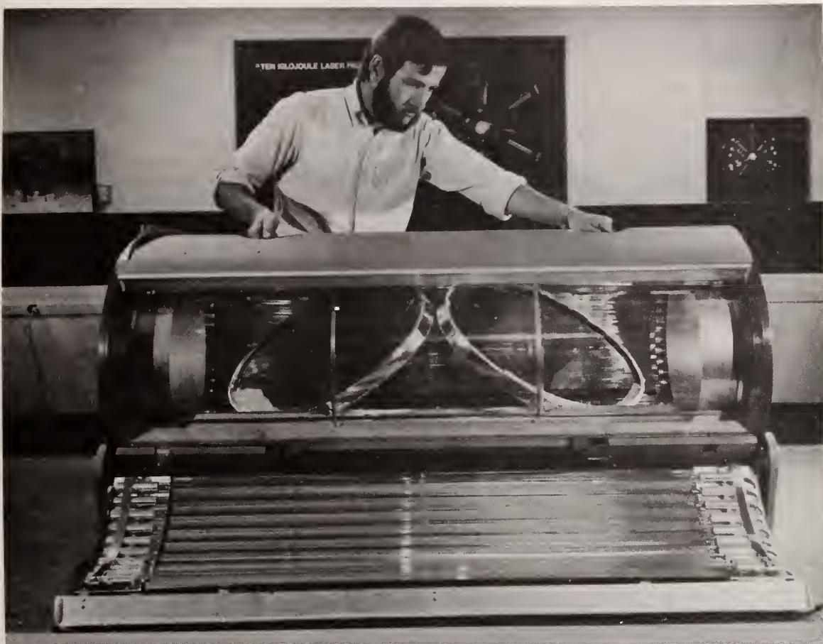
Figure 1. 30-cm aperture disk amplifier.
