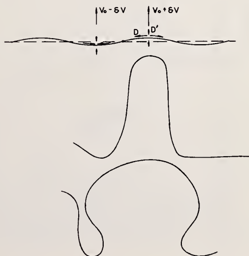
Figure 8. Schematic of breakaway of a grain boundary from its impurity cloud by growth of unstable velocity perturbations.
