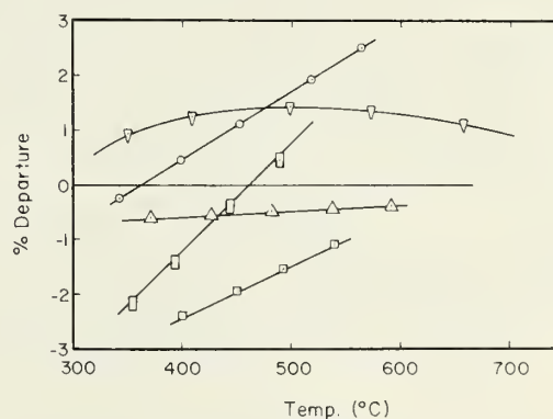
FIGURE 23. Comparison of percent departure of the data for \text{NaNO}_3 .
