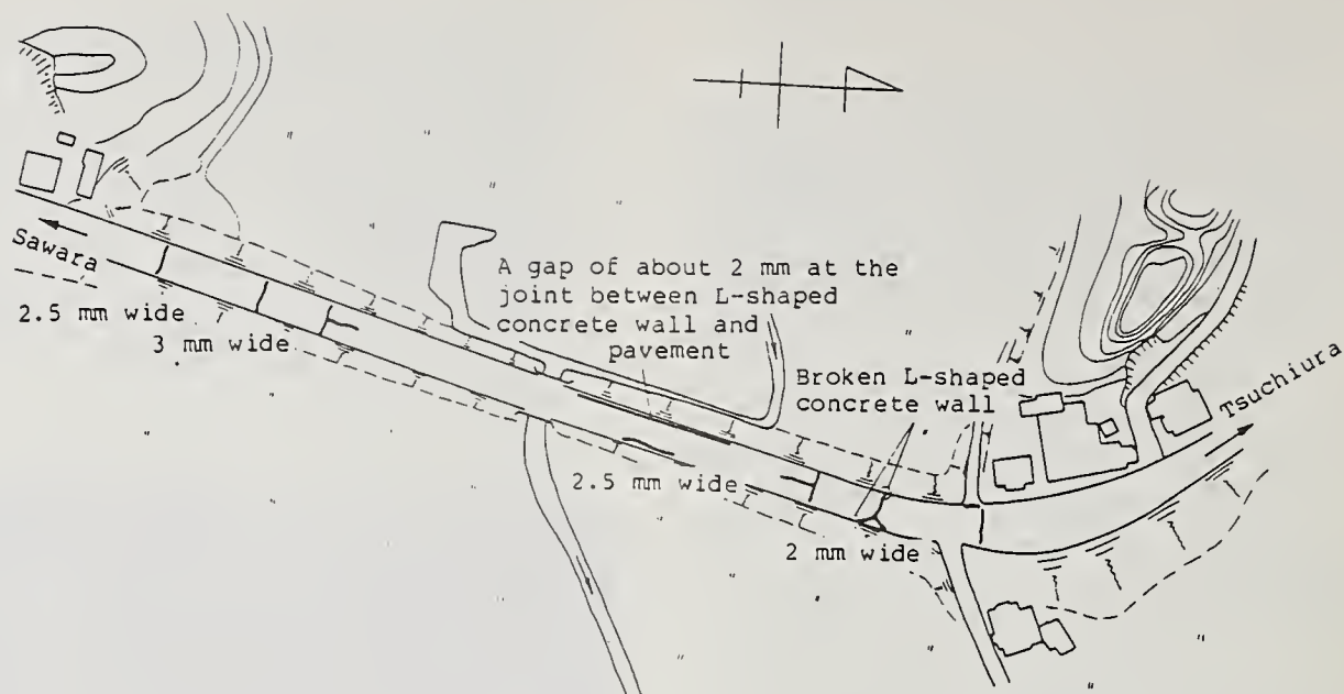
Fig. 11 Damage to National Highway No. 125 (at Sakuragawa)
