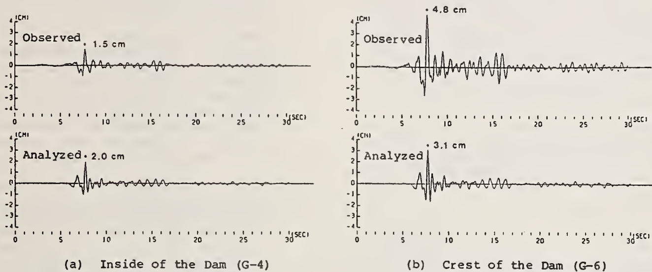
Fig. 21 Comparison of Relative Displacement in Horizontal Direction
