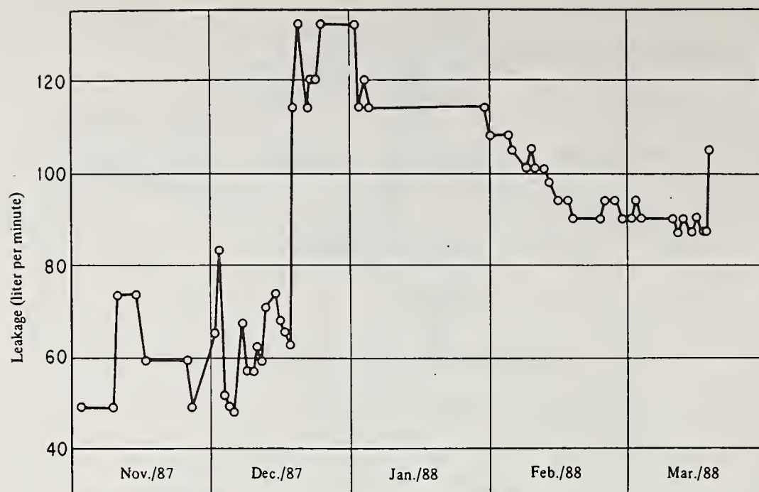
Fig. 11 Leakage in Arakine Dam
