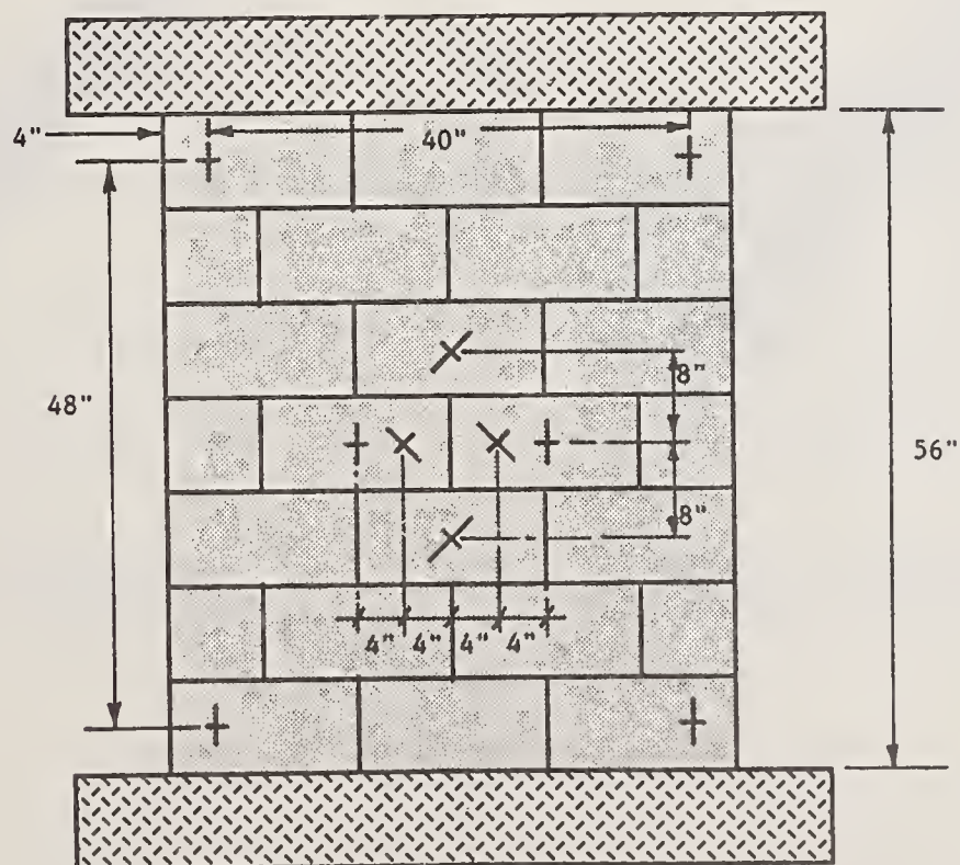
Figure 3 - LST Locations
