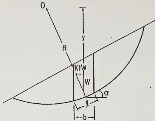
Fig.2 Key sketch for sliding surface method
