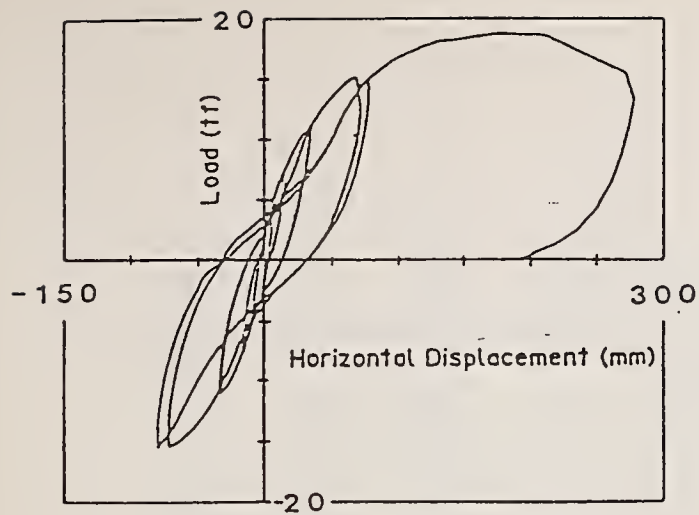
Fig. 10 Load-displacement curves in the Specimen C.
