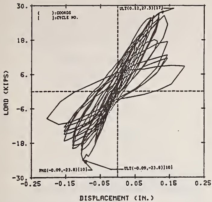
UNREINFORCED WALL (R1)
