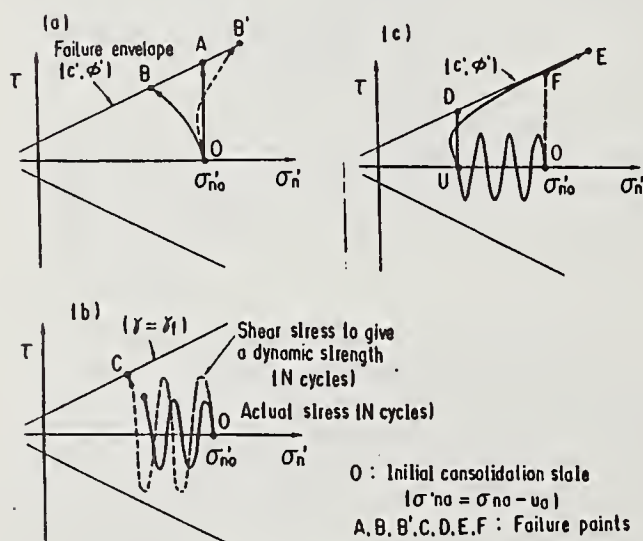
Fig.A2 Stress paths and shear strengths
