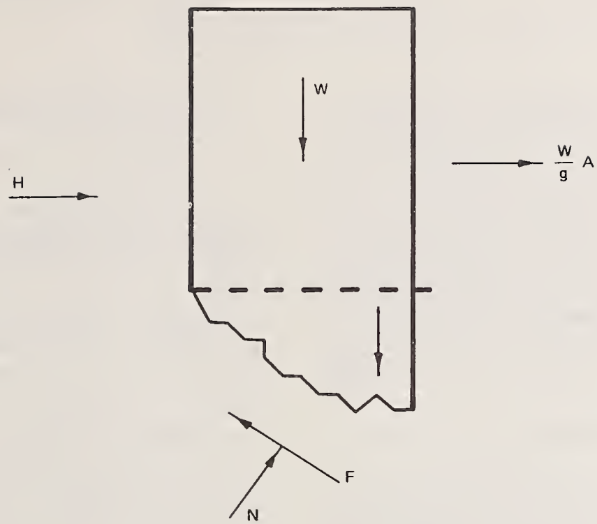
a. IMPENDING SLIDING DOWNSTREAM
