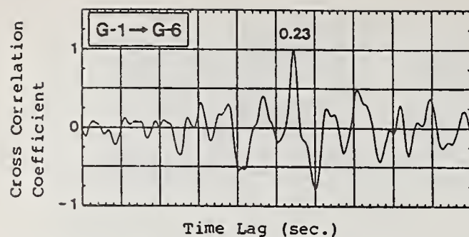
Fig. 10 Cross Correlation Coefficient of Acceleration Records (Upstream-Downstream Direction, Method 1)
