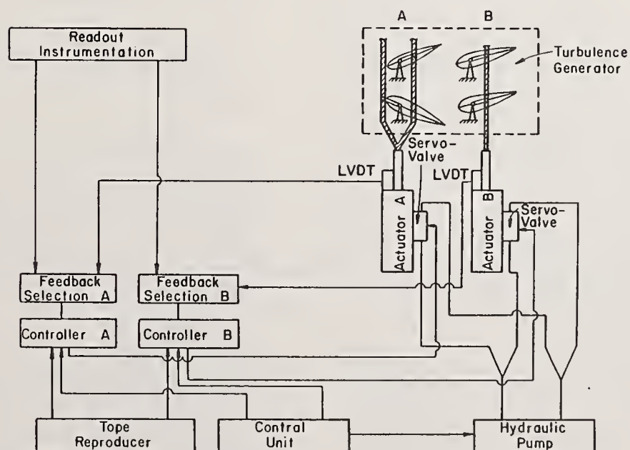
Figure 3. Control-Driving System
