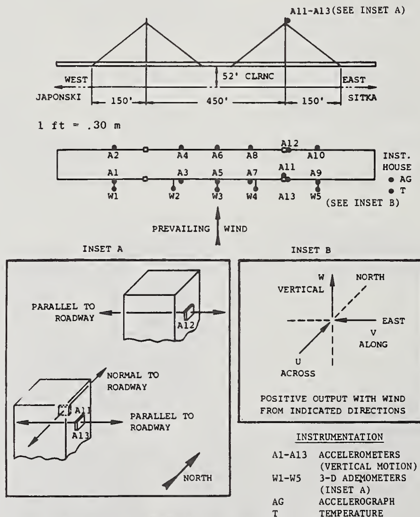
Figure 5. Instrumentation Configuration - Sitka.
