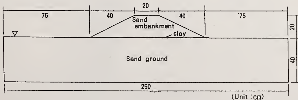
Fig.7 Model configuration
