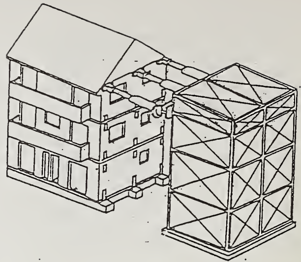
Fig.5 Test set-up.
