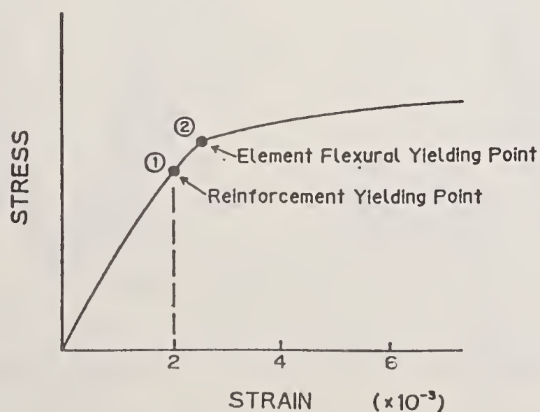
Fig.12 Definition of Yielding
