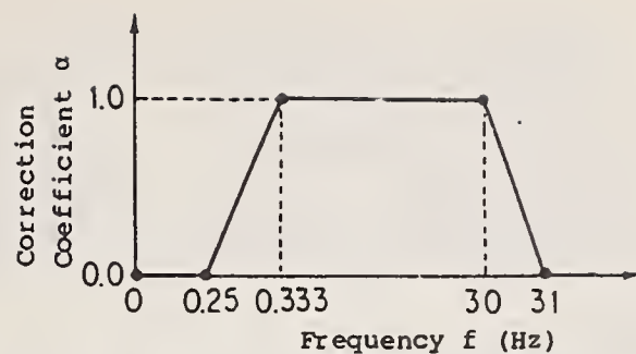
Fig. 3 Correcting Function of Band-Pass Filter
