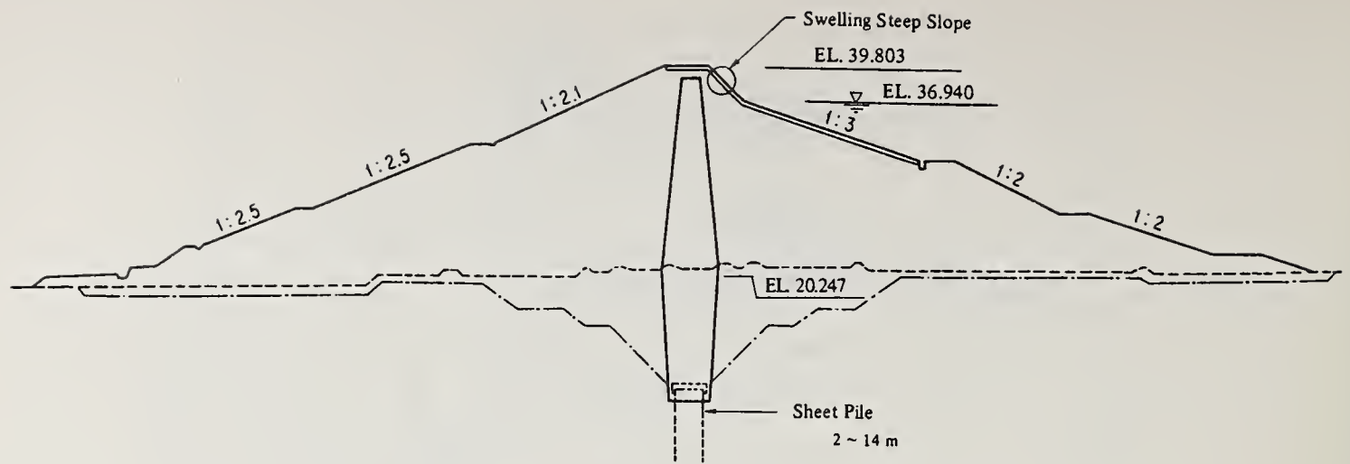
Fig. 16 Section of Konakagawa Dam
