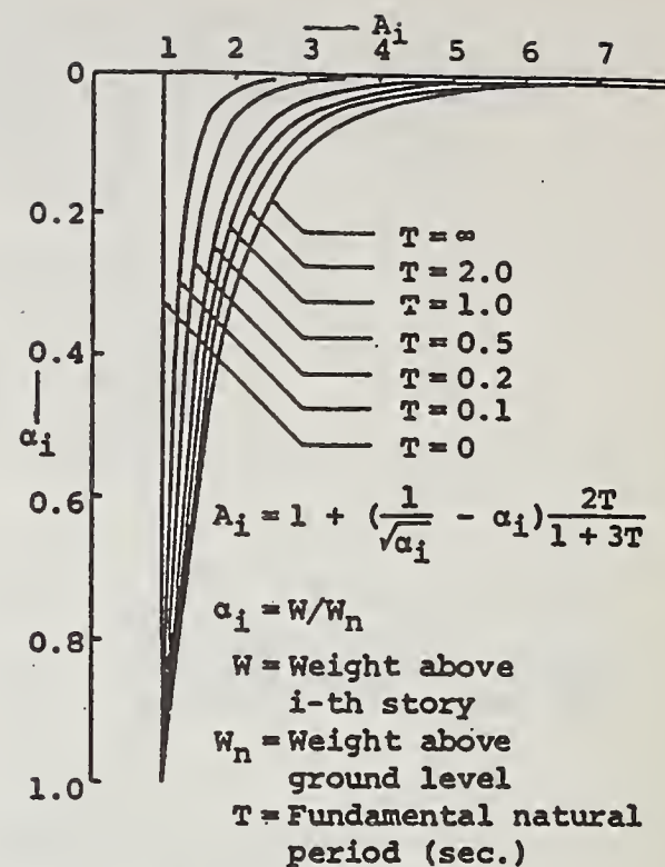
Fig. 3 Lateral Shear Distribution Factor, A_i
