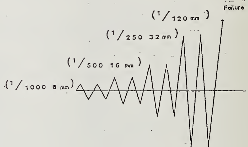
Fig.7 History of loading.
