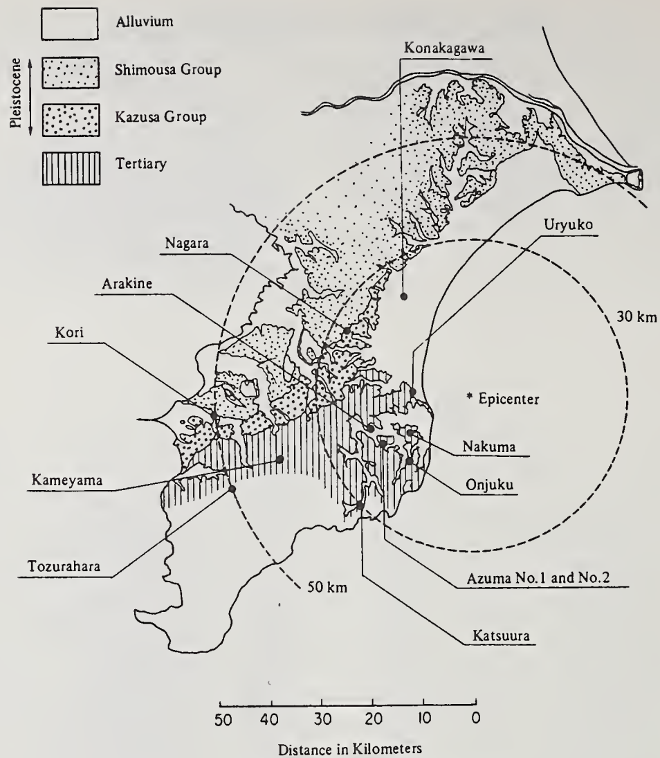
Fig. 1 Location of Dams and Local Geology
