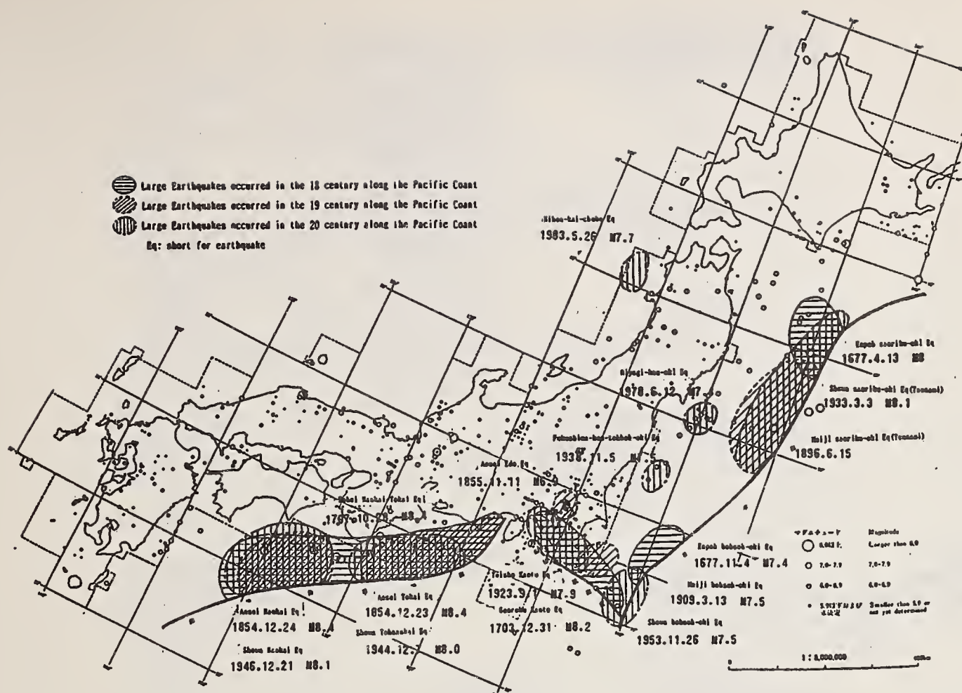
Fig. 1 Hypocenters of Large Scale Earthquakes Distribution Map in Recent Years
