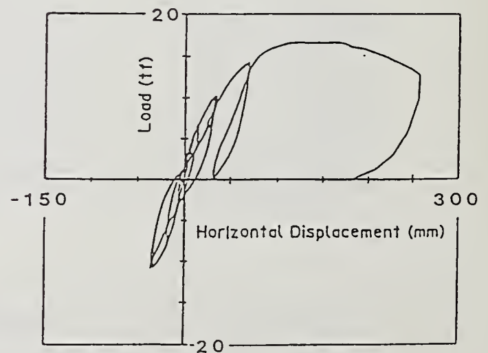
Fig.9 load-displacement curves in the Specimen II.
