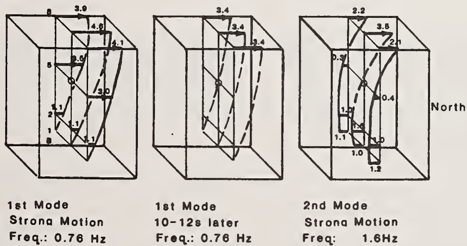
Modal Deflections - cm.
