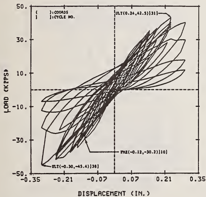
MID-HEIGHT BOND BEAM NO JOINT REINFORCING (R5)
