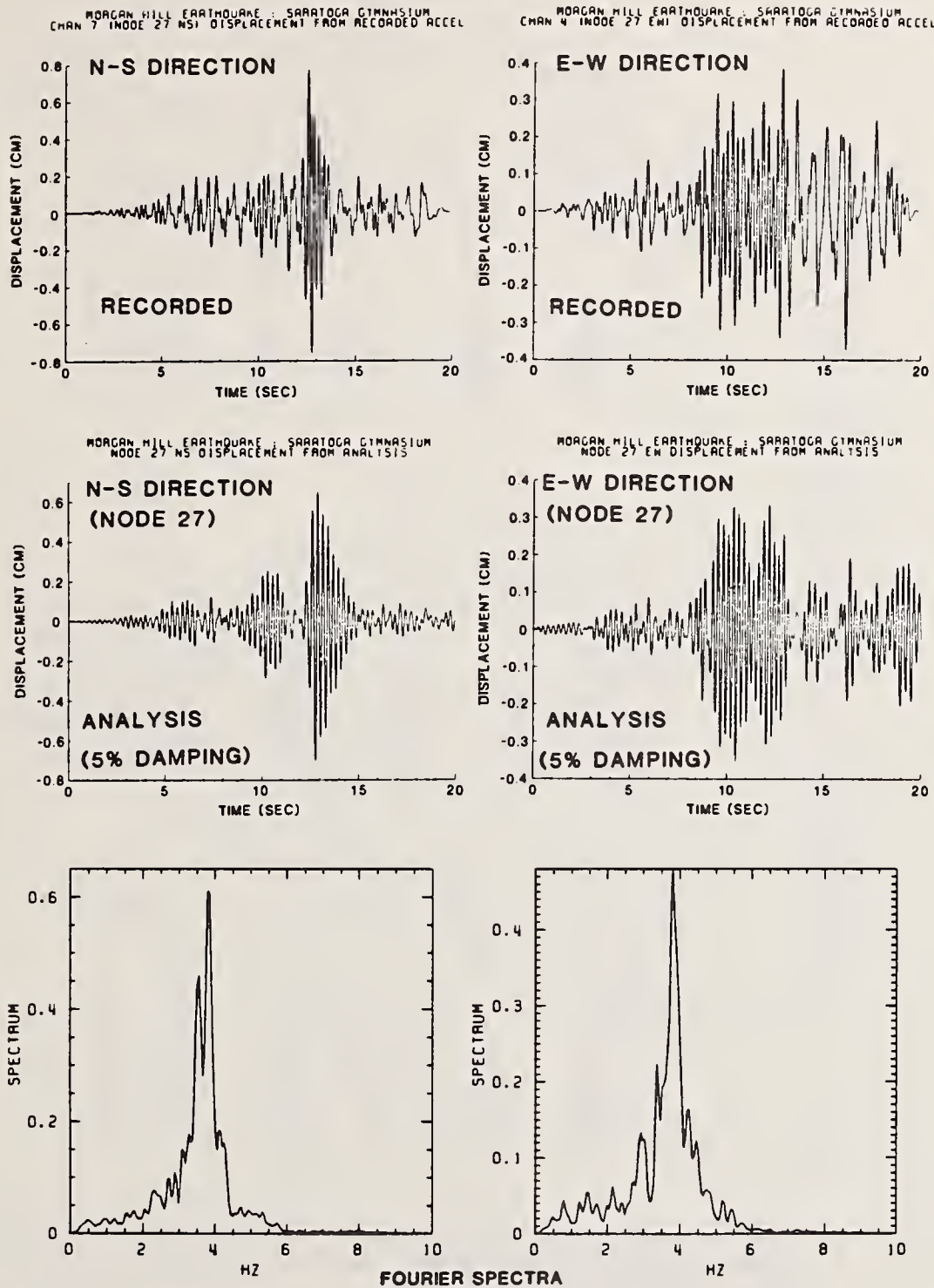
Figure 10. Recorded and calculated displacements at the center of the roof diaphragm in the N-S and E-W directions respectively. The calculated displacements are from dynamic analyses using the finite element model and ground level motions as input. The Fourier spectra corresponds to calculated displacements.
