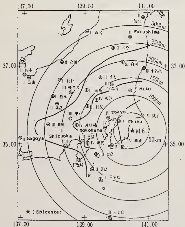
Fig. 1 Seismic intensity (JMA scale) at various places
