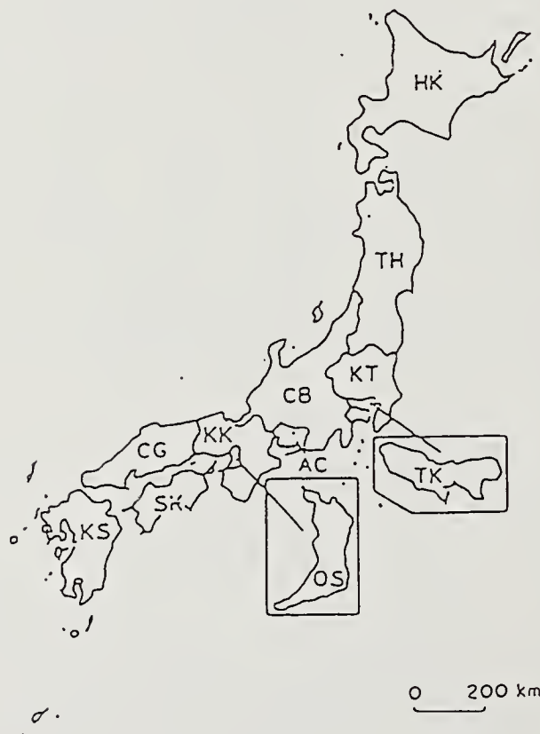
Fig. 1. Distribution of Strong-Motion Accelerographs (as of March 1989)
