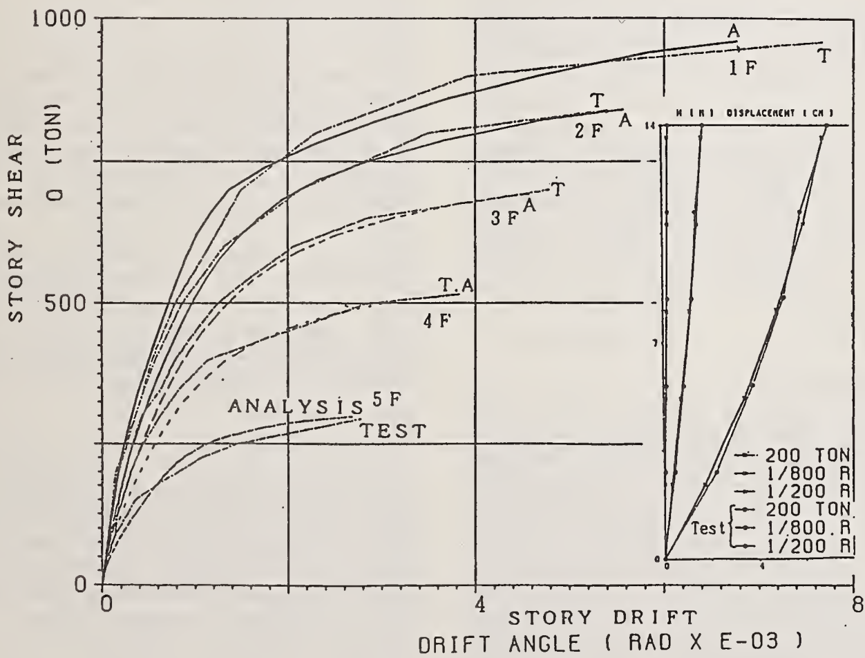
Fig.20 Story Shear vs. Story Drift Relationship
