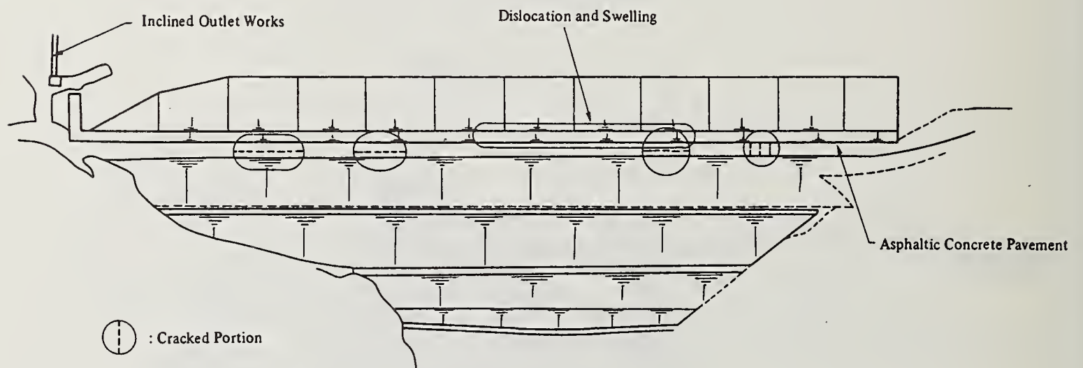
Fig. 17 Location of Cracks in Konakagawa Dam
