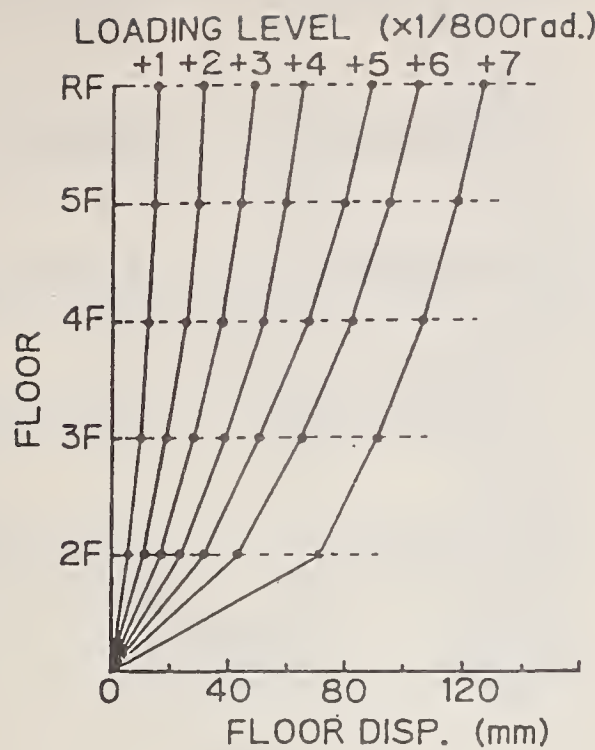
a) Building Deflection Mode
