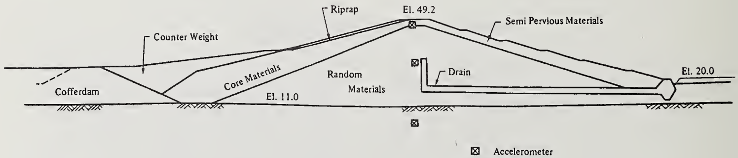
Fig. 2 Section of Kori Dam
