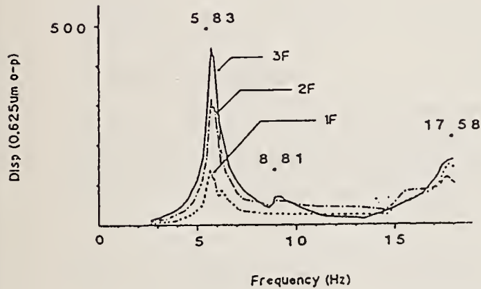
Fig.24 Frequency response curves for EW-direction in the specimen C.
