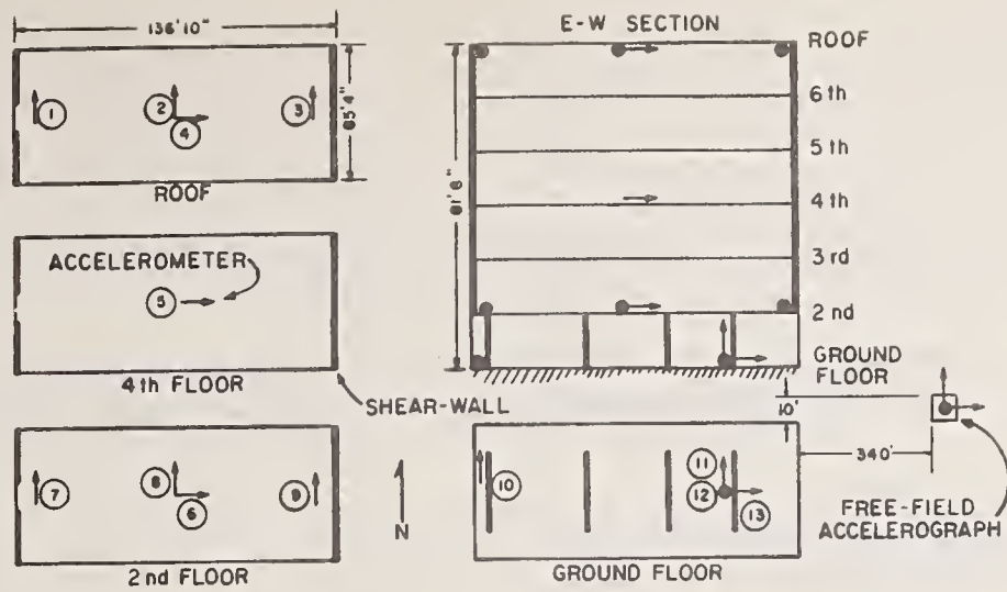
Figure 5. Floor plans and typical vertical section of the Imperial County Services Building. Locations of the sensors are identified.
