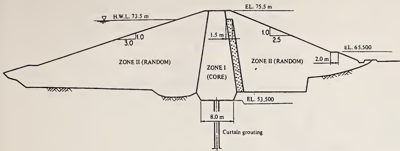
Fig. 8 Section of Azuma No.1 Dam
