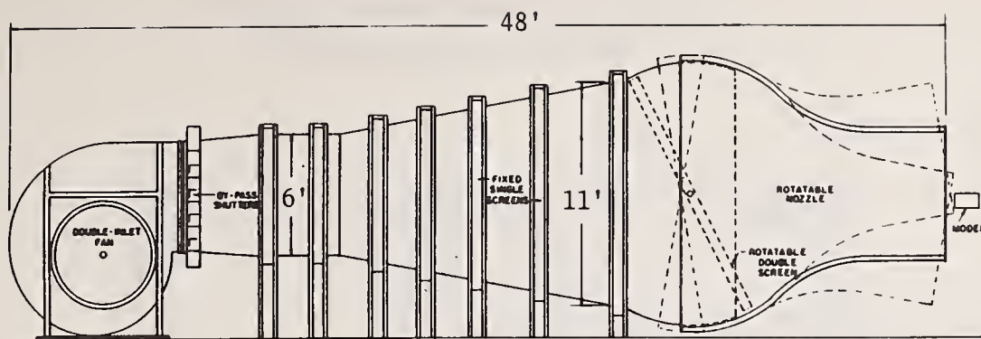
Figure 1. FHWA Wind Tunnel
