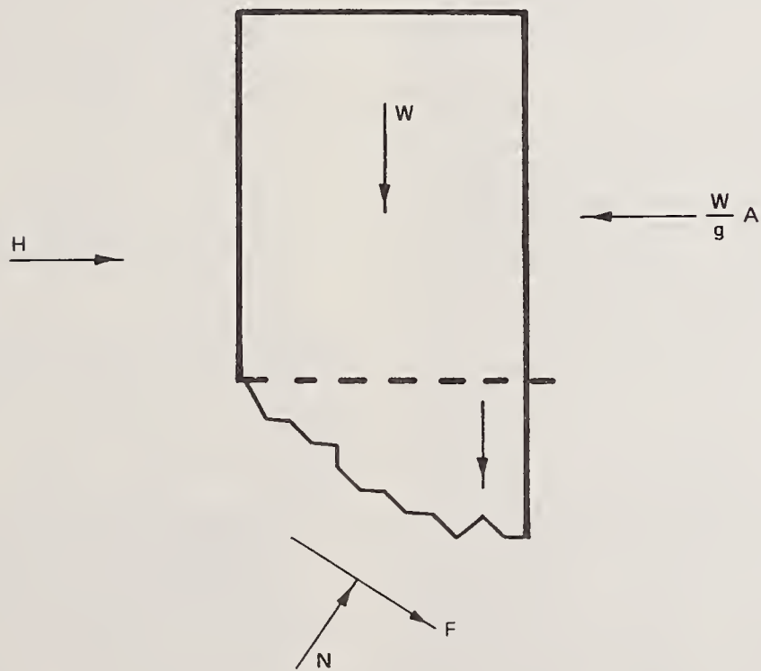
b. IMPENDING SLIDING UPSTREAM
