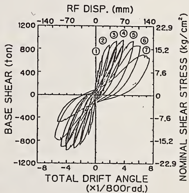
a) Building Drift
