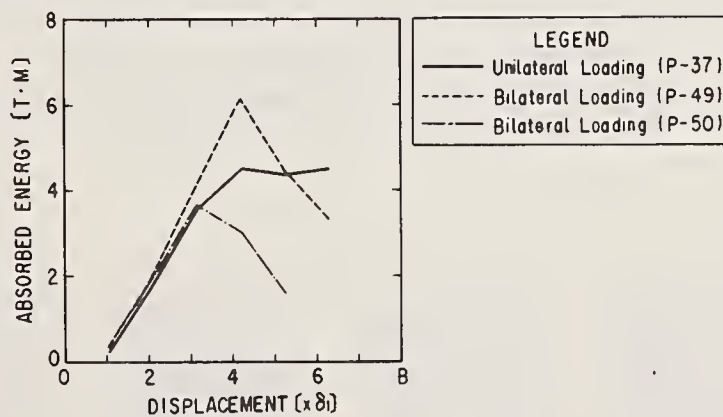
Fig.15 Comparison of Energy Dissipation
