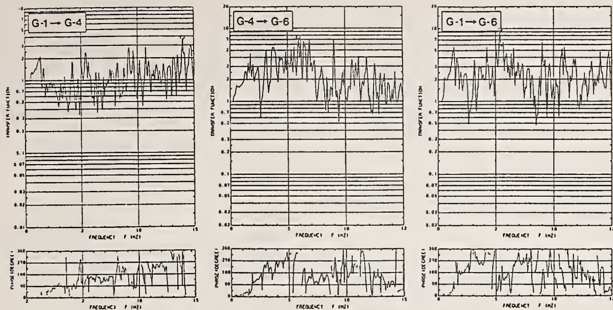
Fig. 7 Transfer Function of Acceleration Records (Upstream-Downstream Direction)
