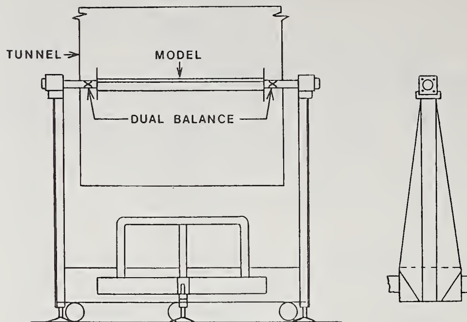
Figure 4. Dual Balance on Mobile Support.
