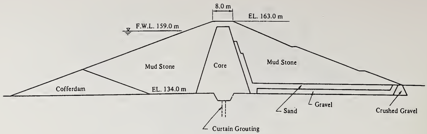
Fig. 5 Section of Katsuura Dam
