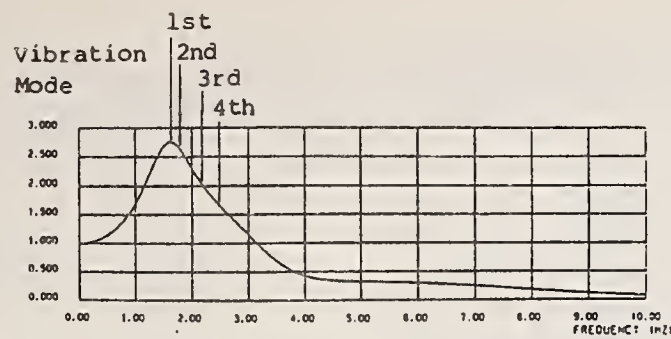
Fig. 20 Transfer Function of the Dam Crest (g-6)
