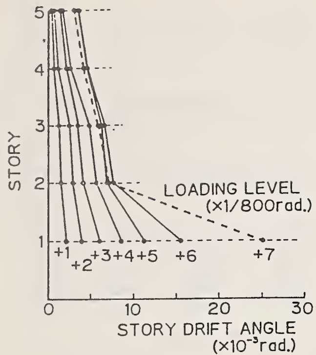
b) Loading Level vs. Story Drift Angle
