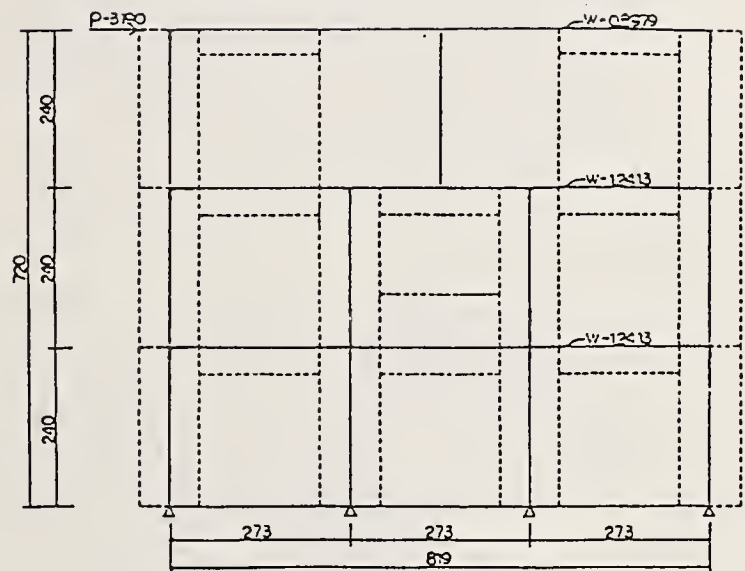
Fig.26 Frame model.
