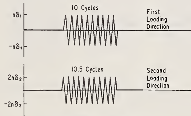
(c) Bilateral Loading in P-50
