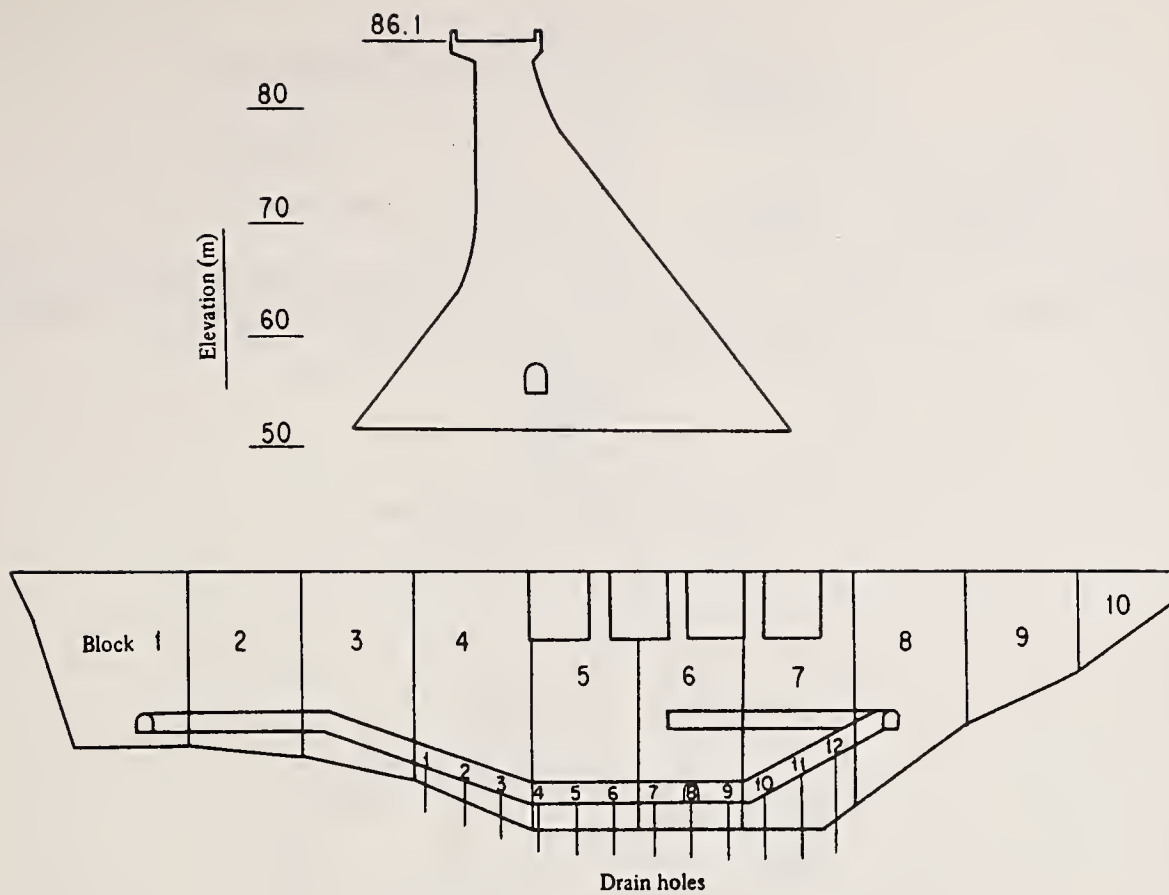
Fig. 3 Section and Elevation of Kameyama Dam
