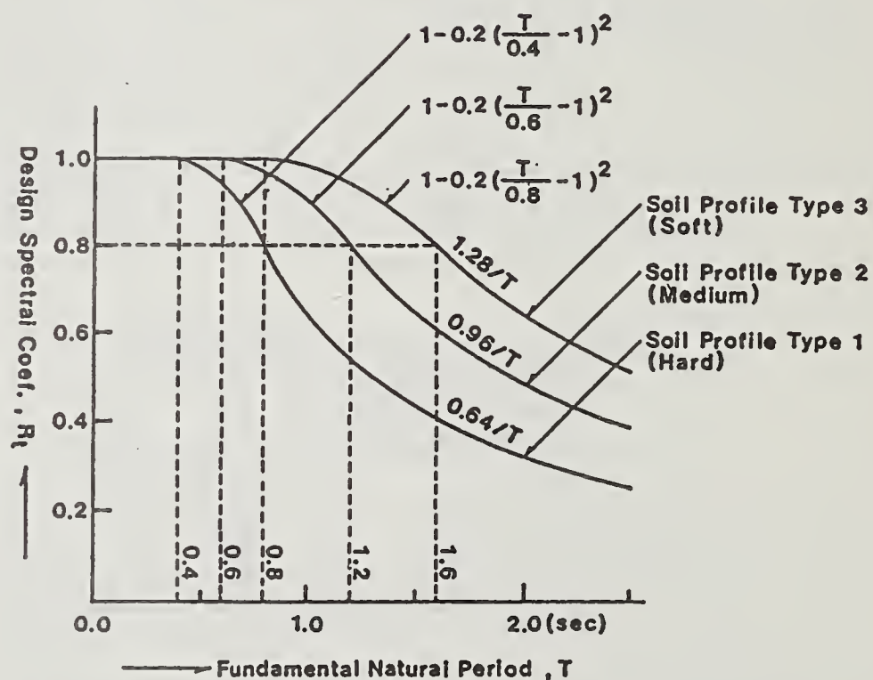
Fig. 2 Design Spectral Coefficient, R_t
