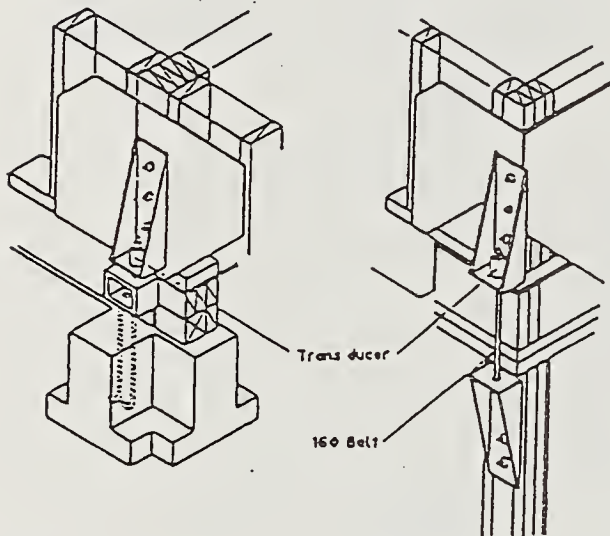
Fig.6 Measurement of a tension force.
