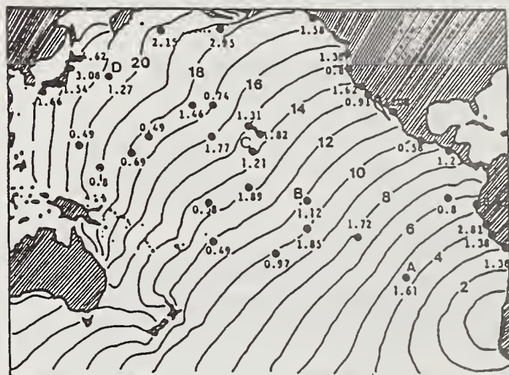
(b) Tsunami travel-time curve
