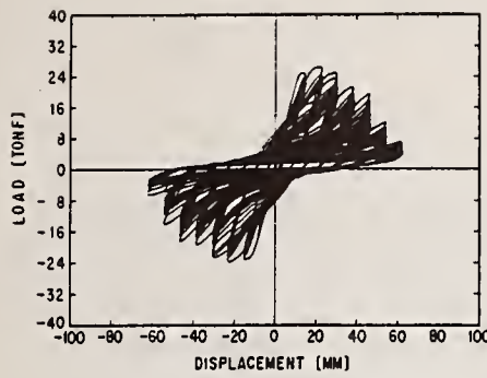
(a) Circular Section (P-29)
