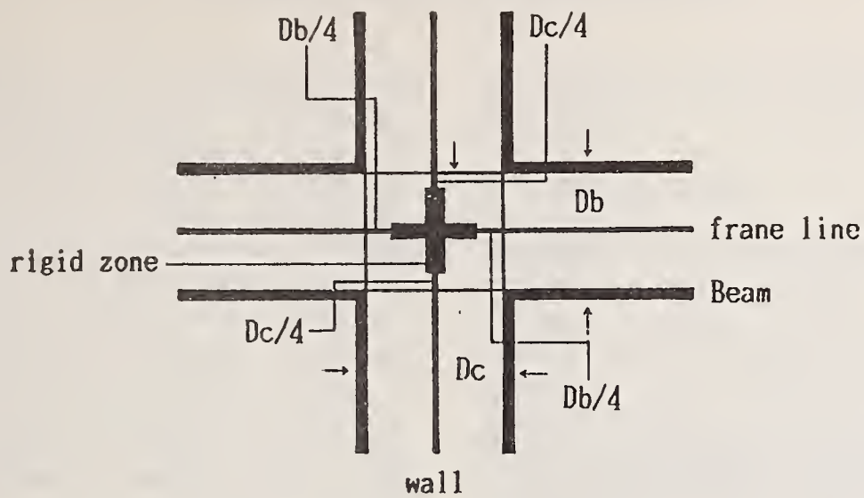
Fig.19 Assumption of rigid zone
