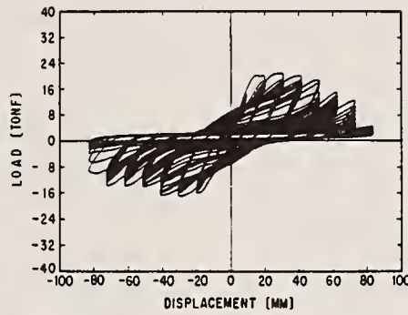
(b) Circular Hollow Section (P-46)
