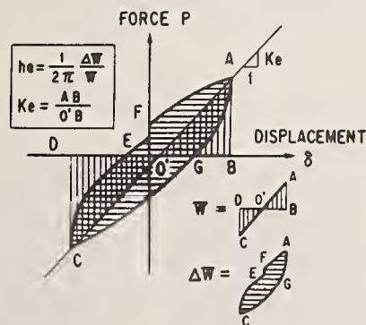
Fig.14 Definition of Equivalent Hysteretic Damping Ratio
