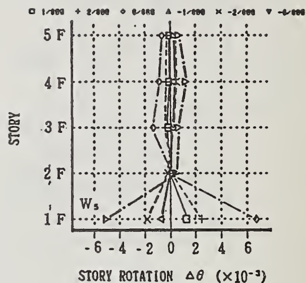
Fig.9 Story Rotation of Wall W5
