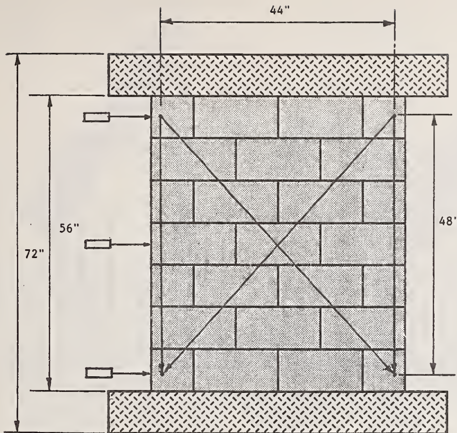
Figure 2 - LVDT Locations
