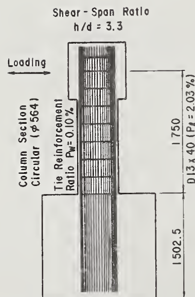
Fig.3 Test Specimens with Circular Section
