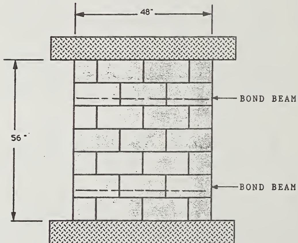
BOND BEAMS AT 2ND AND 6TH COURSES
