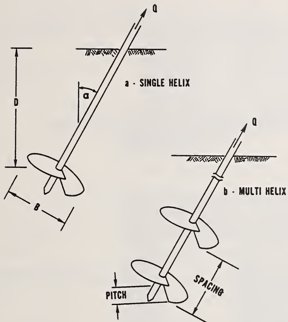
Figure 1 Helix and Multi-helix Anchors
