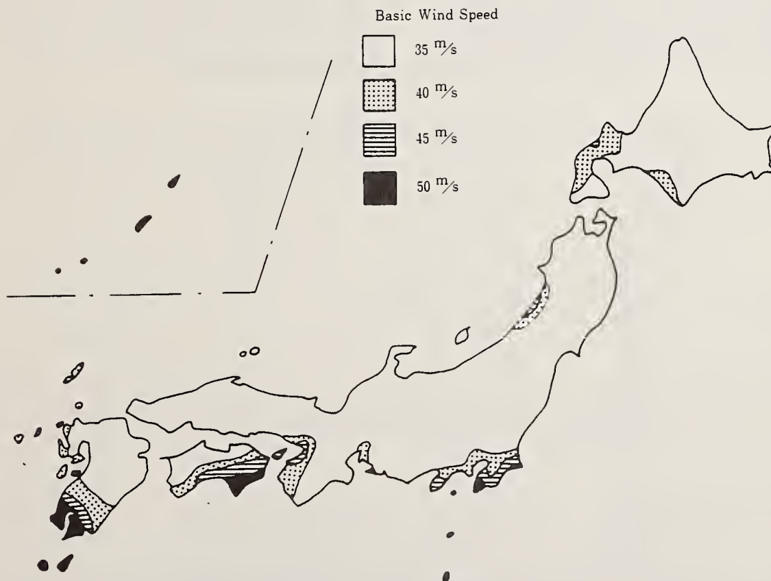
Fig. 2 Basic wind speed
