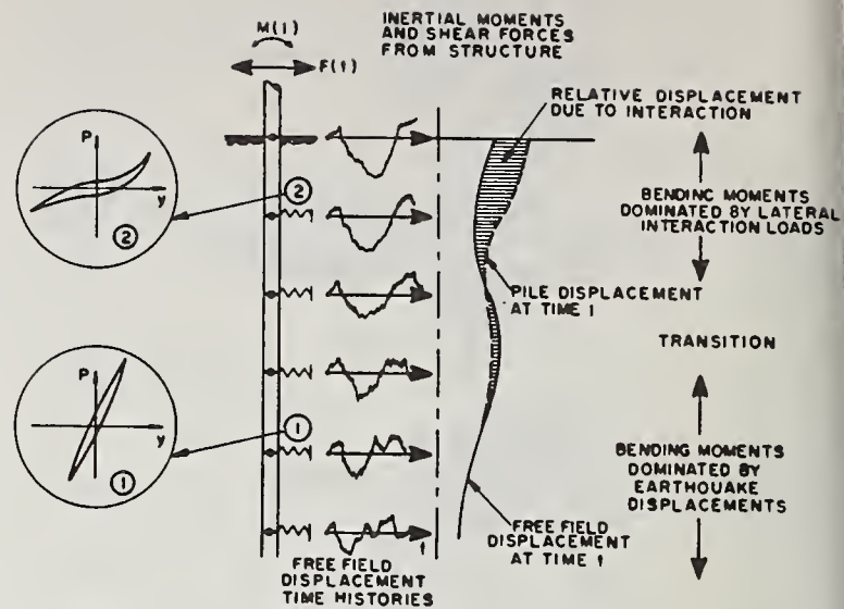
Figure 7. Qualitative description of soil-pile interaction under seismic loads. (Taken from Reference 20)
