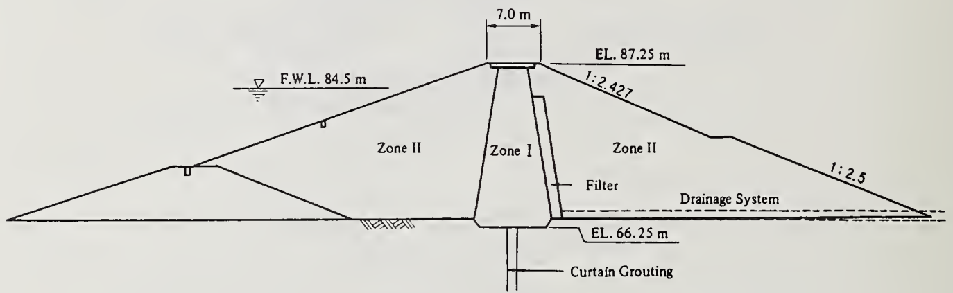
Fig. 6 Section of Onjuku Dam
