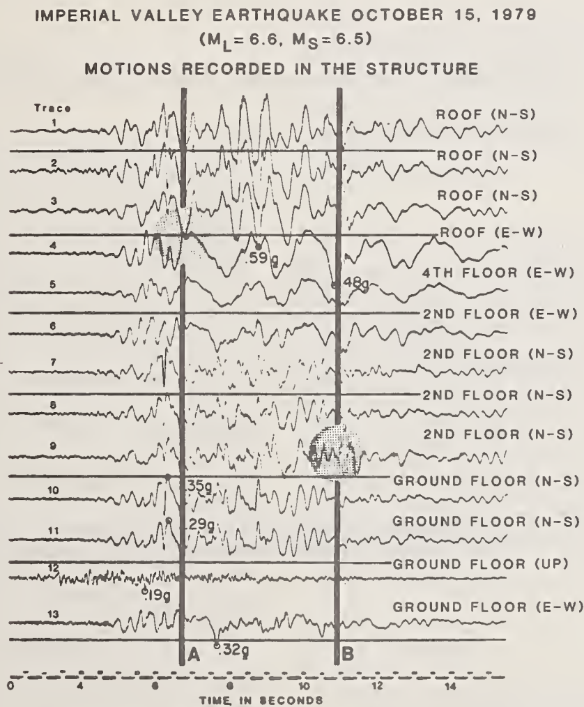
Figure 6. Acceleration records obtained at the Imperial County Services Building during the Imperial Valley earthquake of October 15, 1979.
