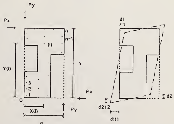
Fig.27 Racking model of a shear element in Tuomi's model.
