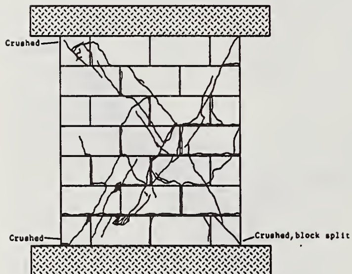
MID-HEIGHT BOND BEAM NO JOINT REINFORCING (R5)
