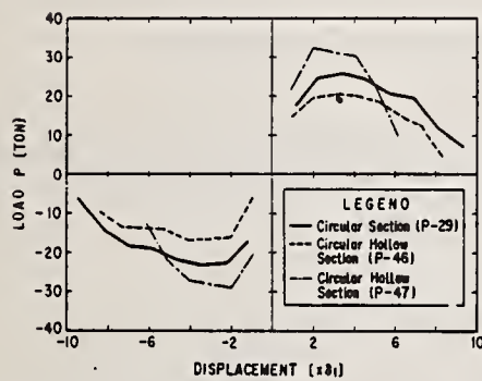
Fig.21 Comparison of Envelope of Hysteresis Loops
