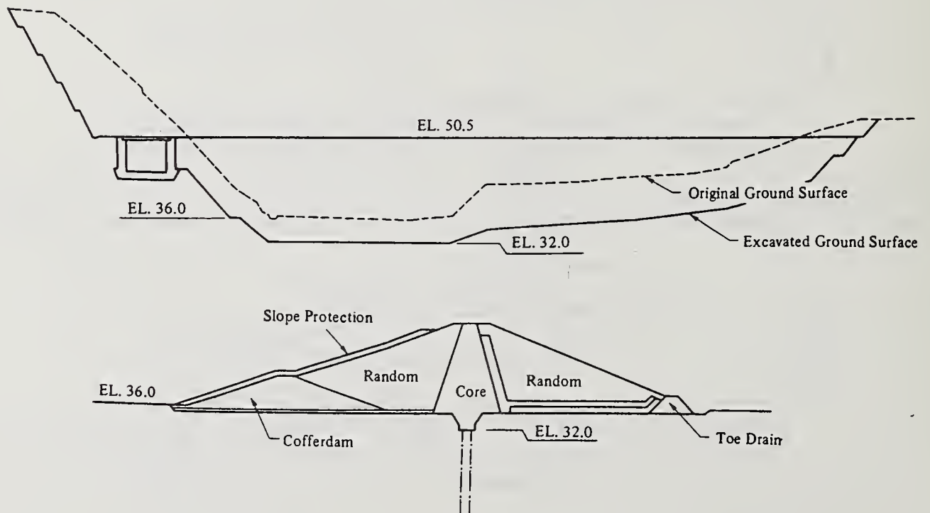
Fig. 7 Profile and Section of Nakuma Dam
