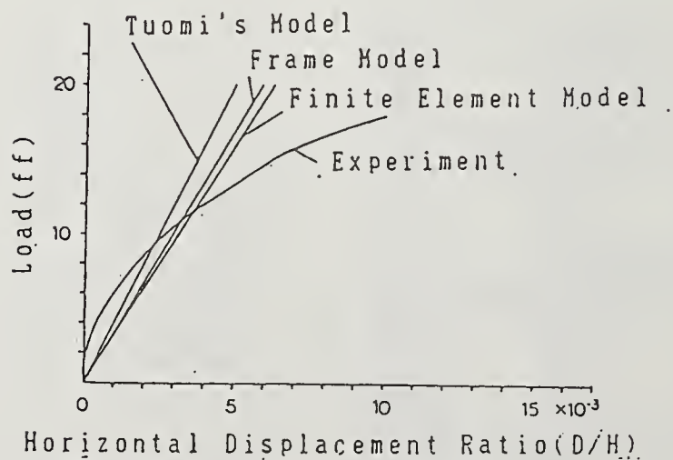
Fig.30 Comparison of the experimental results with the calculated results on the third story of the Specimen C.
