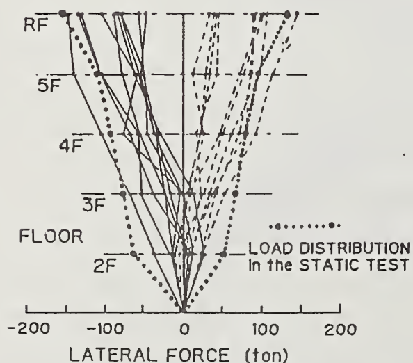
a) Lateral Force Distribution at Peaks of the Response
