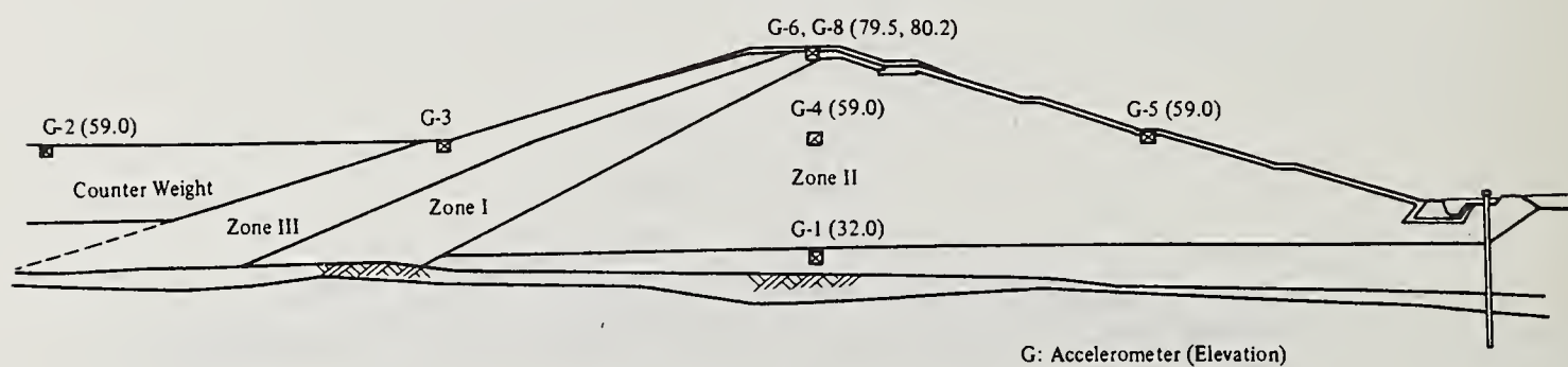
Fig. 13 Section of Nagara Dam
