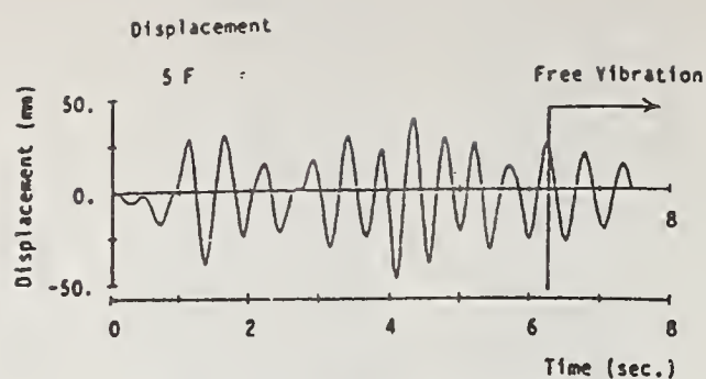
a) Time History of Horizontal Displacement
