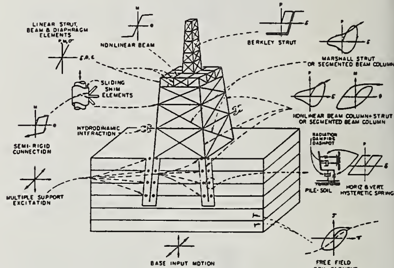
Figure 8. Typical finite element model required to evaluate the soil-pile-structure system. (Taken from Reference 17)
