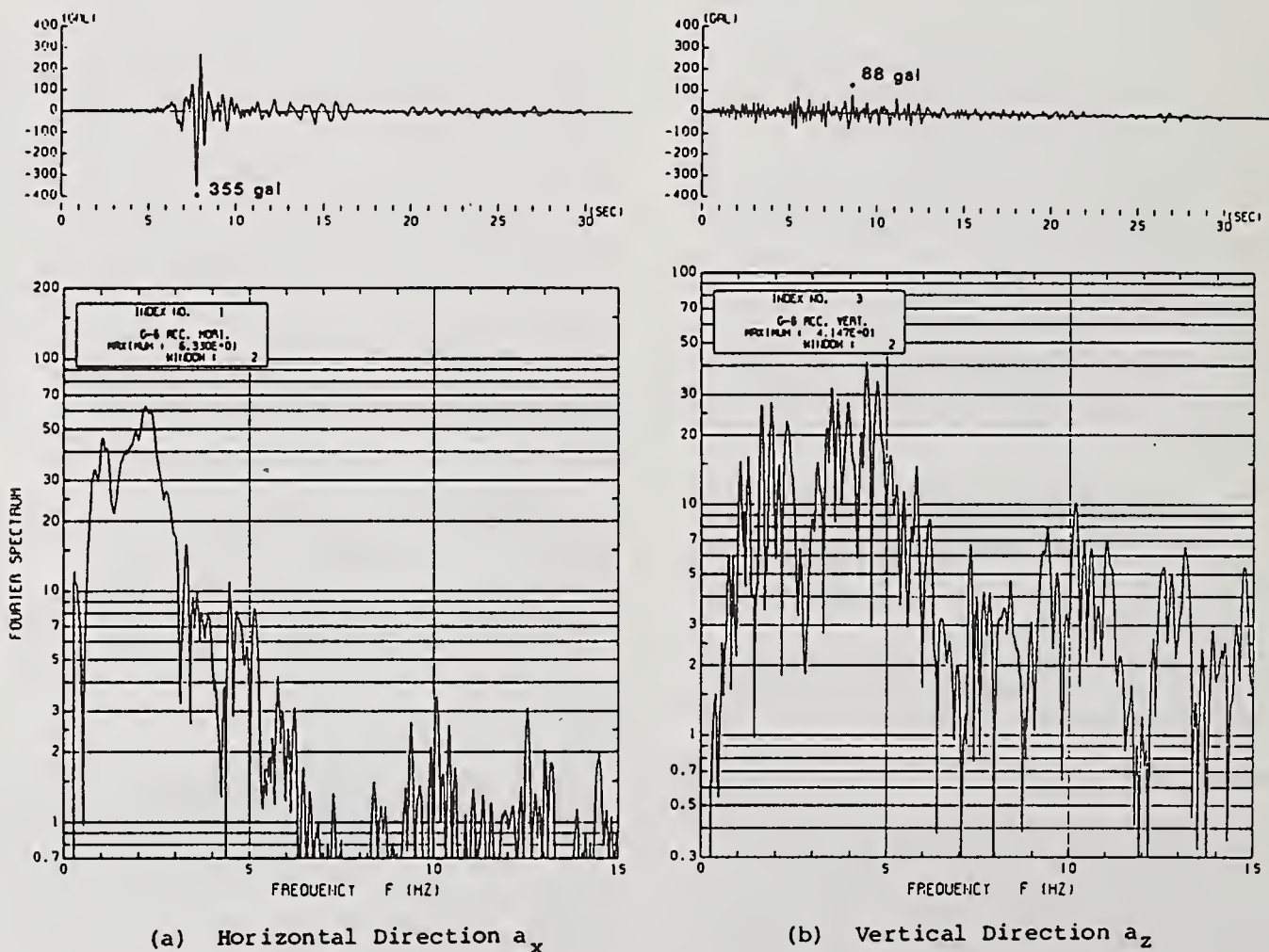
Fig. 19 Analyzed Response Acceleration of the Dam Crest (G-6)
