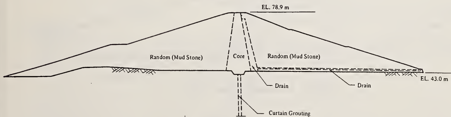
Fig. 10 Section of Arakine Dam
