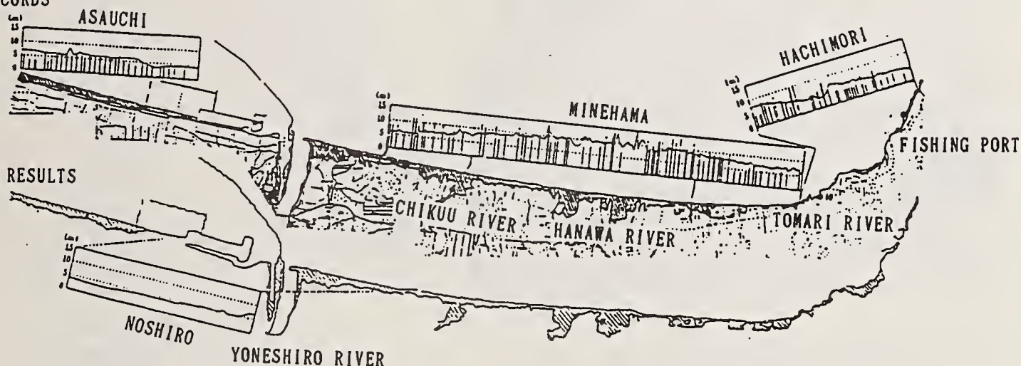
Fig. 4 Computation results for the 1983 Nihonkai-Chubu Tsunami.
