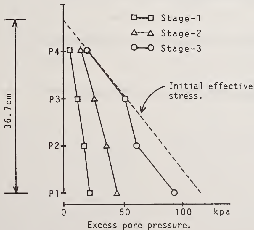
Fig.16 Distribution of the maximum excess pore pressure
