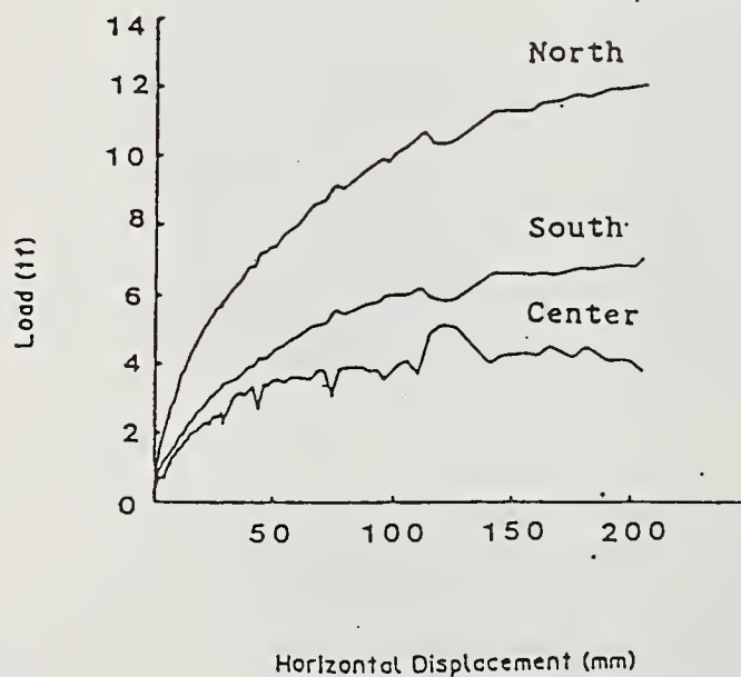
Fig.8 Load-displacement curves in the Specimen A.
