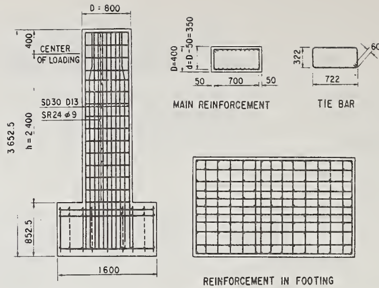
Fig.1 Test Specimens for Bilateral Loading
