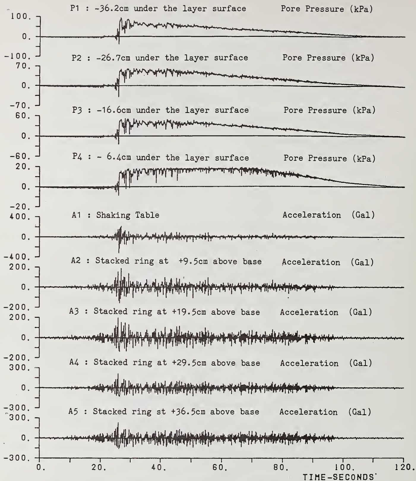
Fig.15 Time histories of stage-3 in prototype scale.
