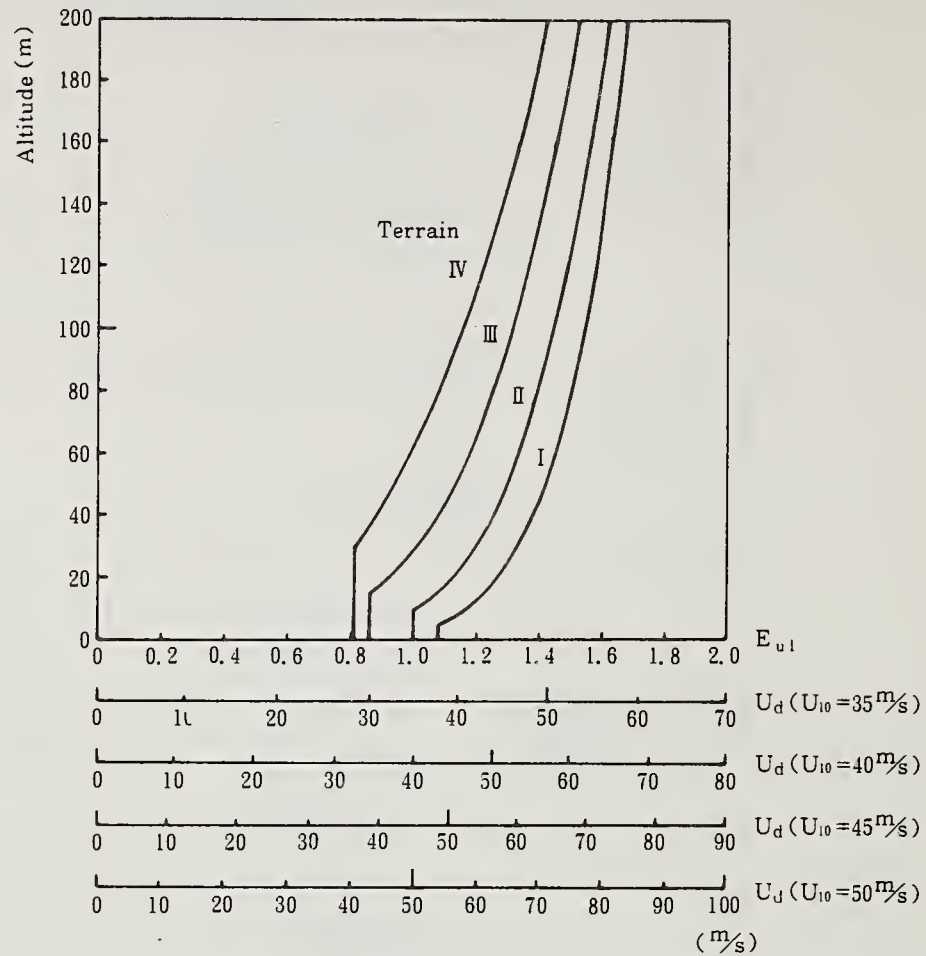
Fig. 3 Correction factor Eul and design wind speed
