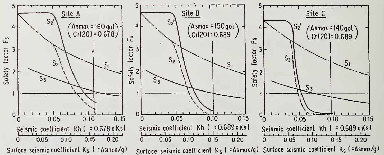
Fig.3 Seismic coefficient vs. safety factor
