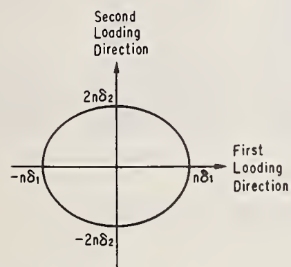
(c) Bilateral Loading in P-50
