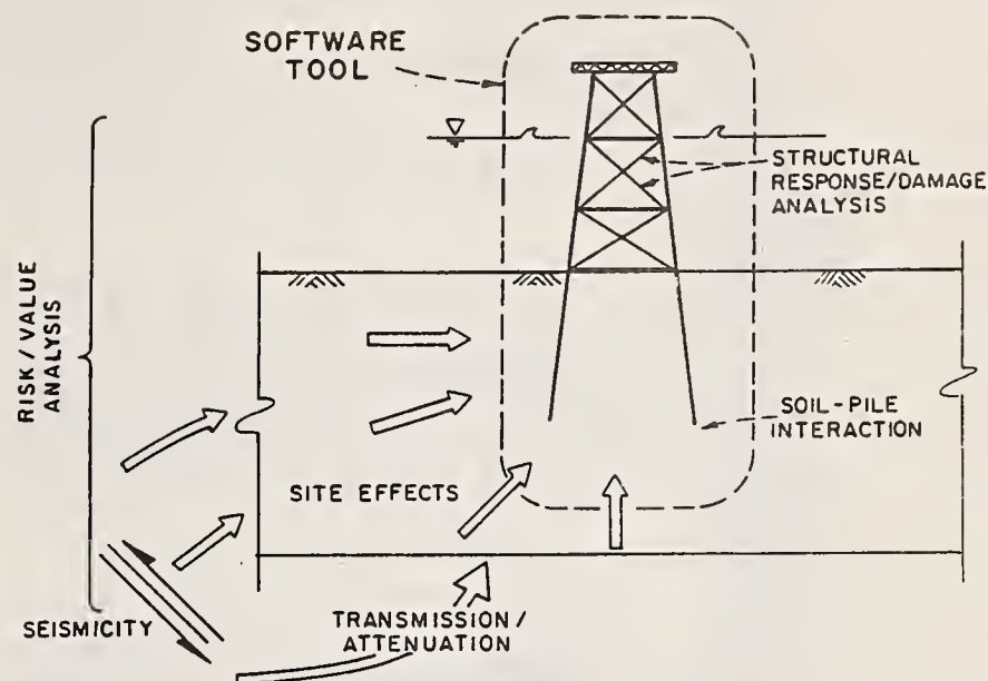
Figure 3. Areas of consideration for offshore earthquake engineering technology. (Taken from Reference 17)
