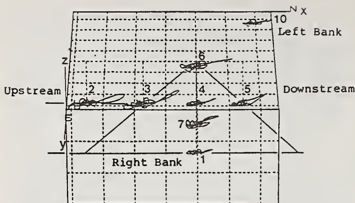
Fig. 6 Displacement Orbits at Observation Points
