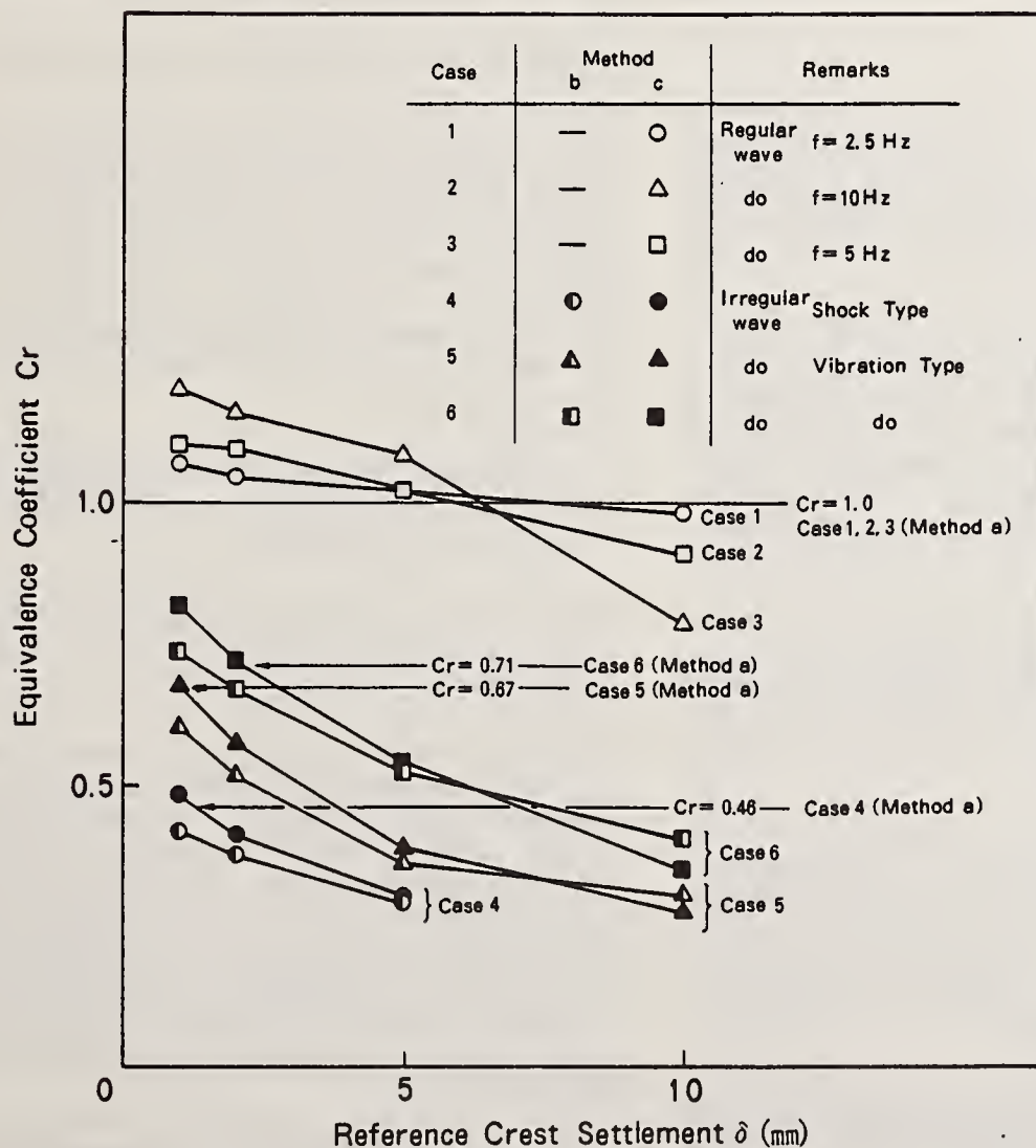
Fig.11 Failure criteria vs. equivalence coefficient
