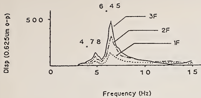
Fig.23 Frequency response curves for EW-direction in the Specimen D.
