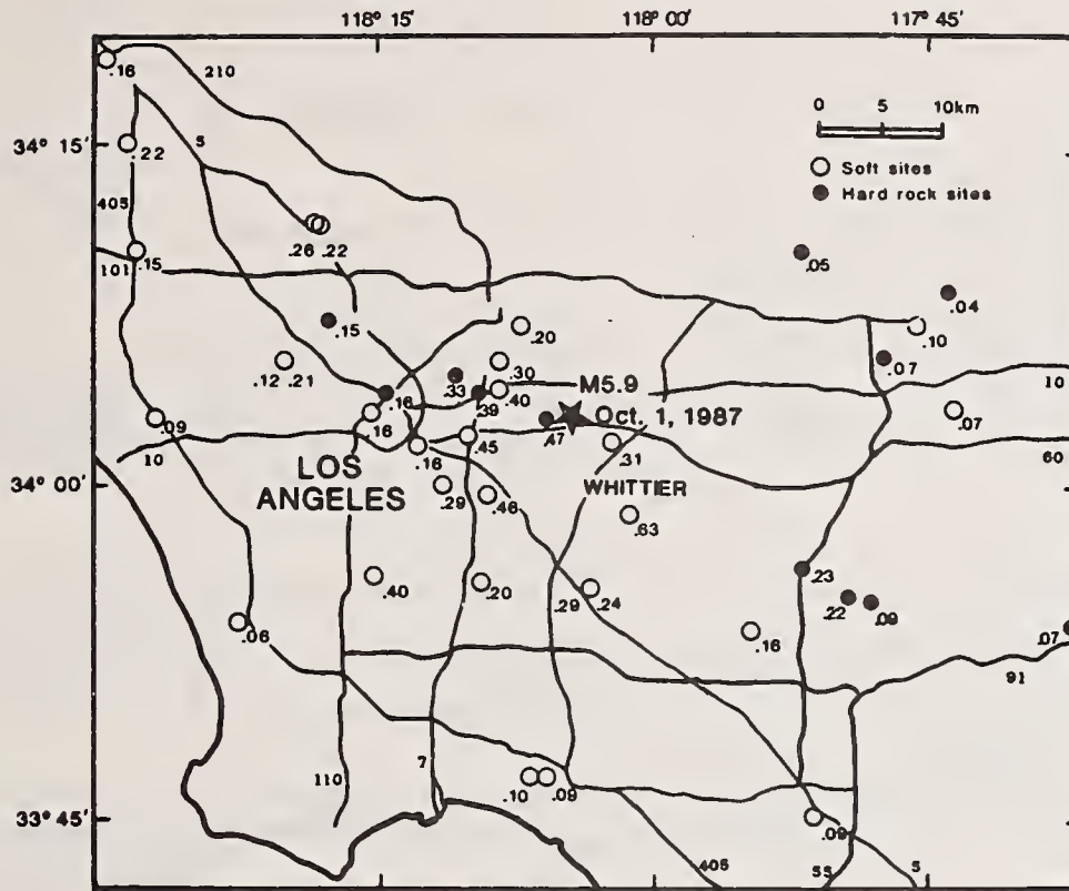
Figure 1. Epicenter of October 1, 1987, M5.9 Whittier Narrows earthquake. Peak ground accelerations at Norwalk, 15 km south of epicenter, are 0.24 and 0.29g.
