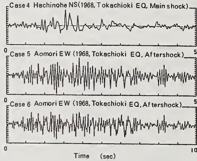
Fig.8 Input acceleration wave form
