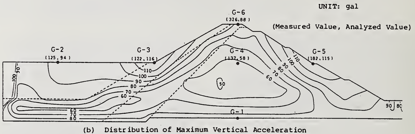
Fig. 18 Distribution of Maximum Response Acceleration
