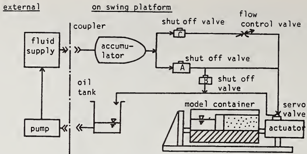
Fig.2 Oil flow circuit
