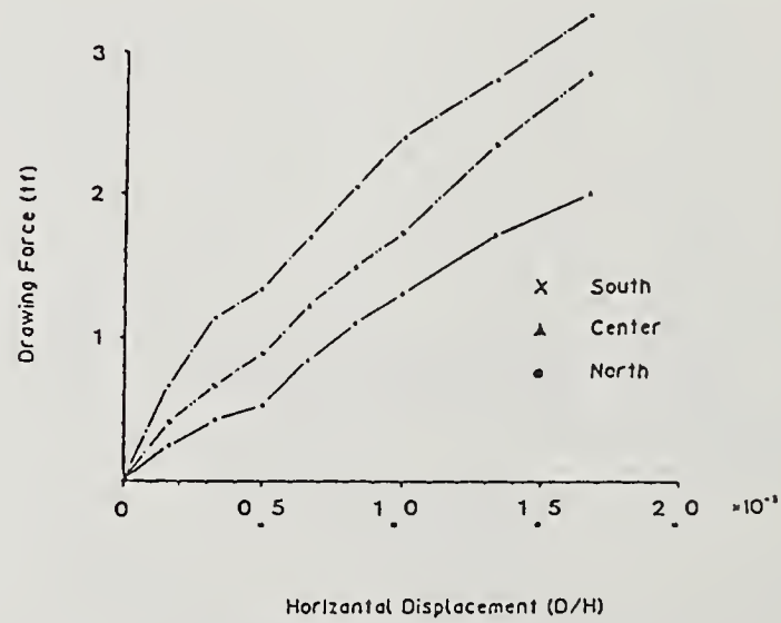
Fig.22 Drawing force of the walls on the first story.
