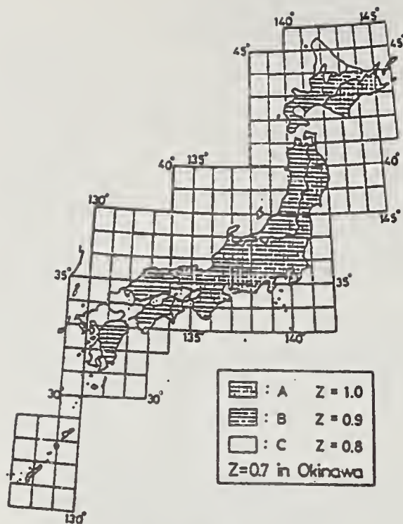
Fig. 1 Seismic Hazard Zoning Coefficient, Z
