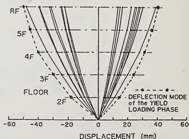
b) Deflection Mode at Peaks of the Response
