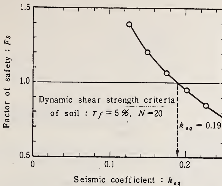
Fig.10 Safety factor vs. equivalent seismic coefficient
