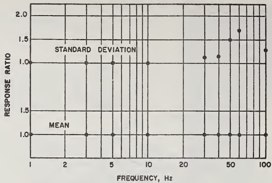
Fig. 4. Frequency response of the pressure transmission system
