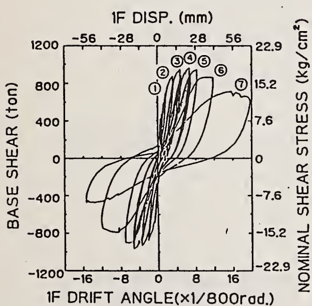
b) 1st Story Drift
