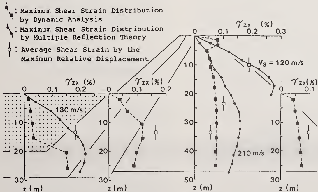
Fig. 15 Distribution of Maximum Shear Strain (Upstream-Downstream Direction)
