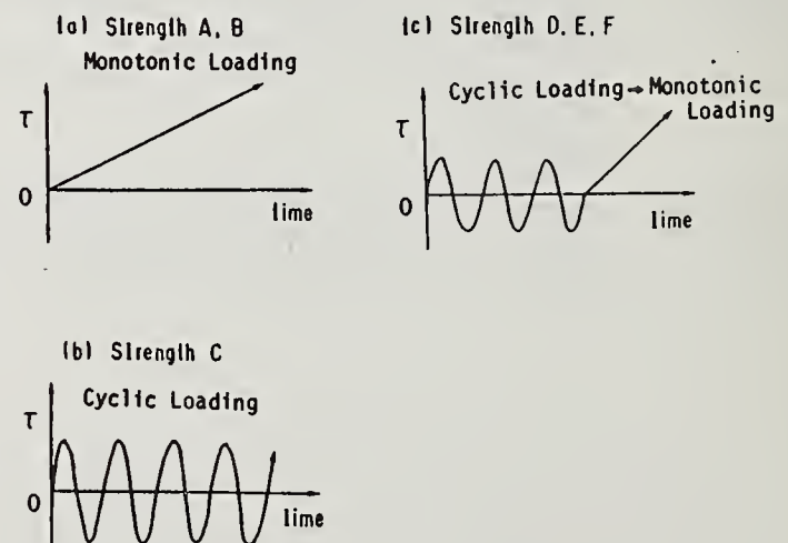
Fig.A1 Loading patterns to obtain shear strength
