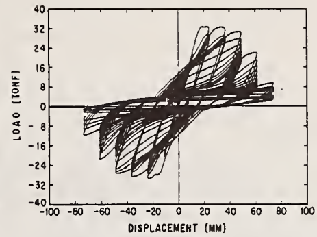
(c) Circular Hollow Section (P-47)
