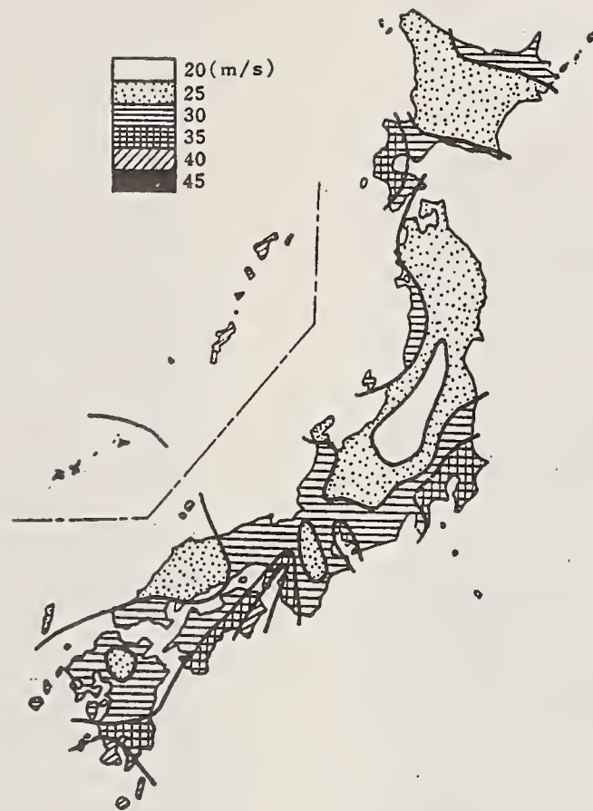
Fig.4 Normal wind velocity V_0
