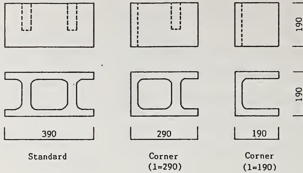
Fig.2 Concrete Block Units [scale in mm]
