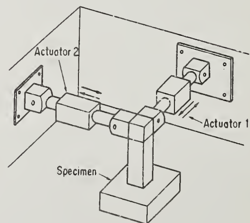
Fig.4 Set-up for Bilateral Loading
