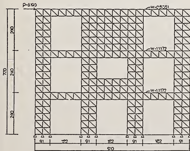
Fig.25 Finite element model.
