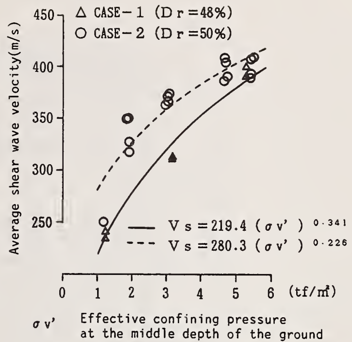
Fig.10 Relation between the average shear wave velocity and effective confining pressure at the middle depth of the ground.
