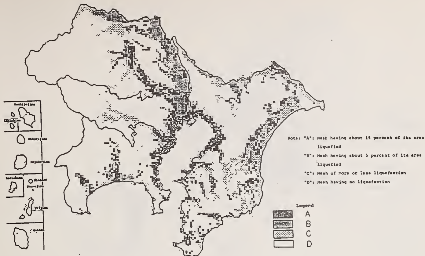
Fig. 8 Liquefaction possibility distribution map
