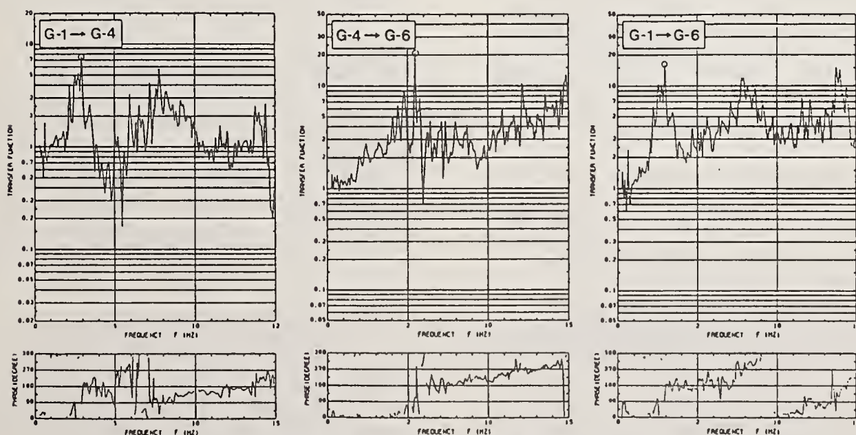
Fig. 9 Transfer Function of Acceleration Records (Vertical Direction)
