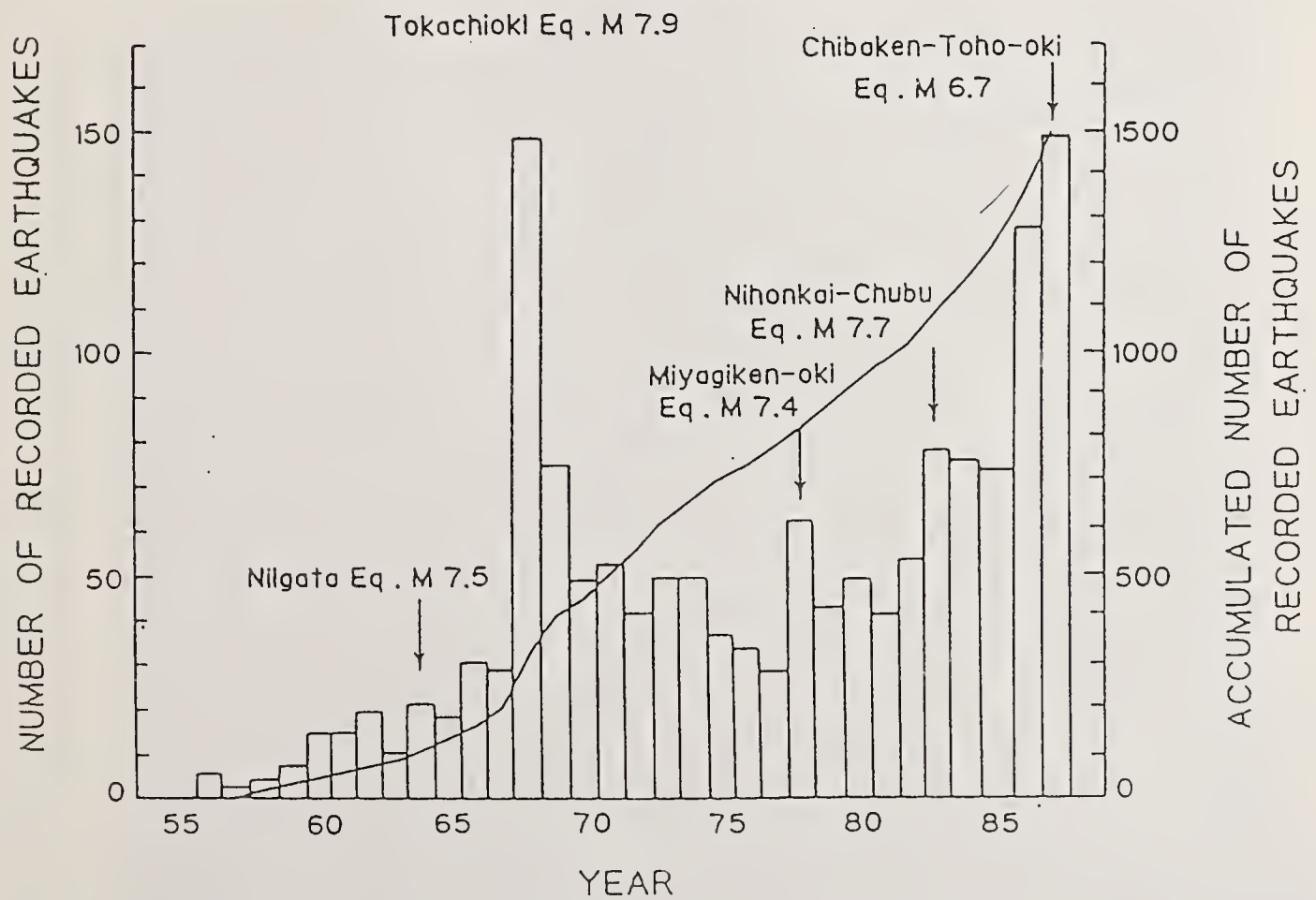
Fig. 3. The Number of Recorded Earthquakes
