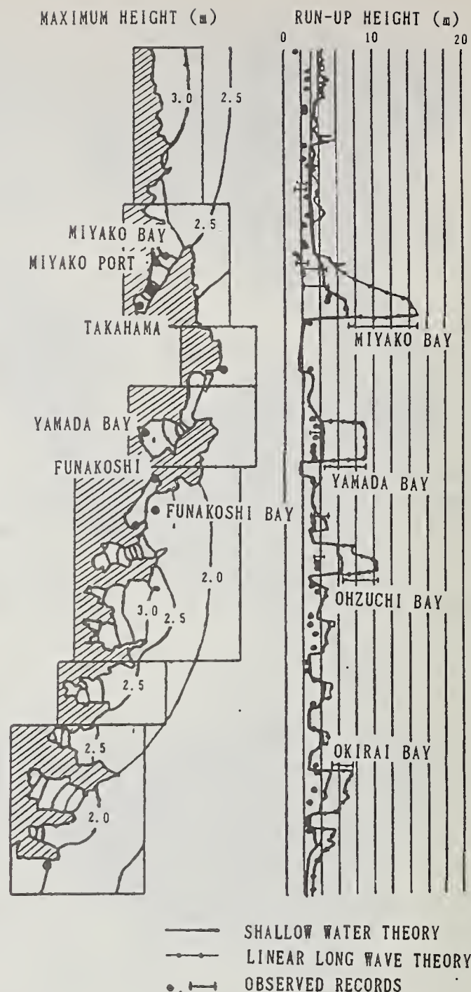
Fig. 6 Computation results of the 1960 Chilean Tsunami ( tsunami height along Sanriku Coast).
