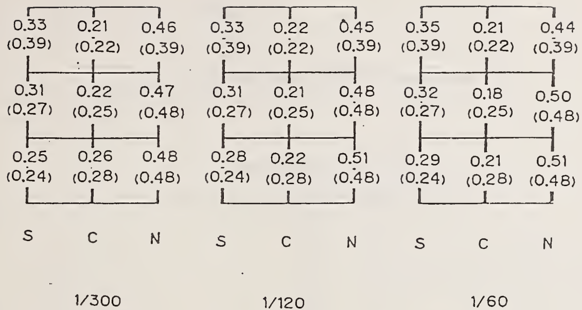
Fig. 18 Distribution of the horizontal load in the Specimen C.
