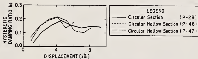
Fig.22 Comparison of Equivalent Hysteretic Damping Ratio
