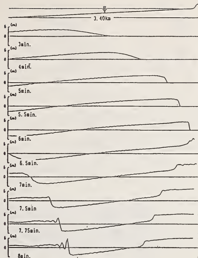
Fig.7 Computation result for tsunamis with soliton fissions.
