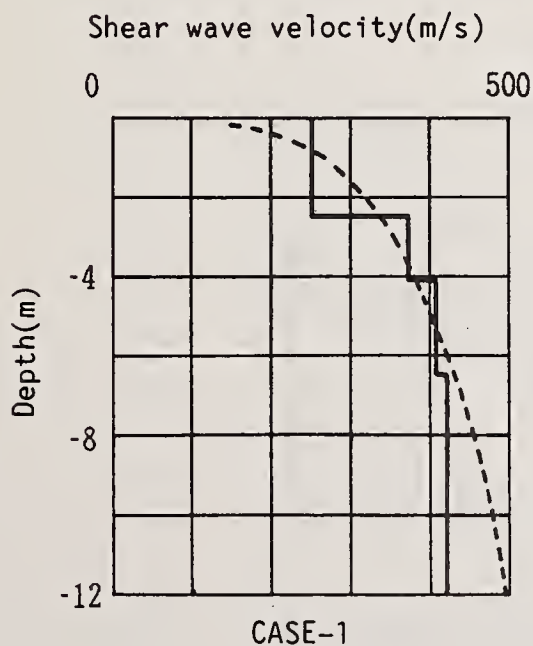
Fig.11 Distribution of the shear wave velocity with depth.
