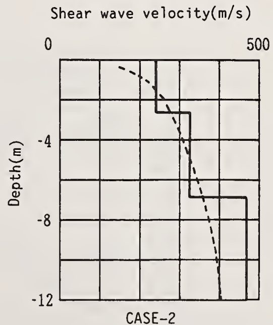
Fig.11 Distribution of the shear wave velocity with depth.
