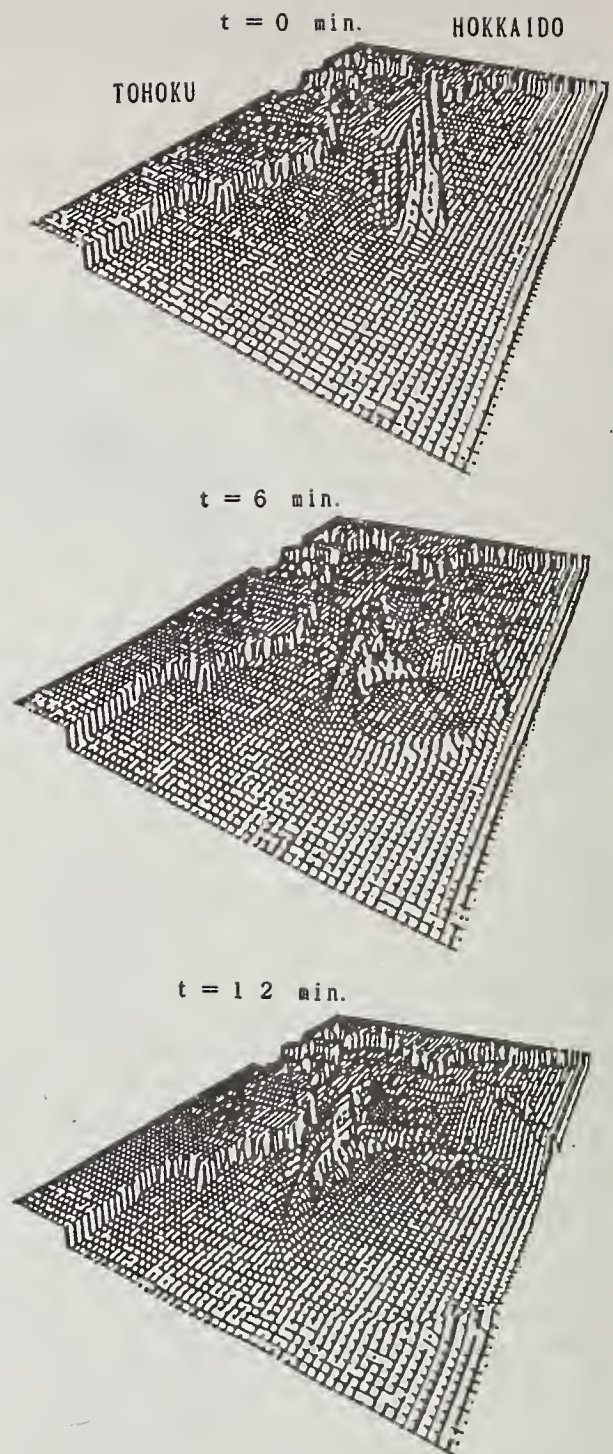
Fig. 2 Computation result for Great Meiji Sanriku Tsunami ( in deep sea).
