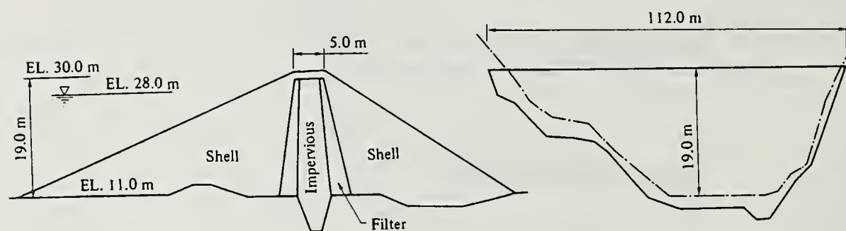
Fig. 12 Section and Profile of Uryuko Dam
