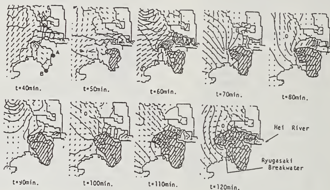
fig. 9 Computation results for oil spreading.
