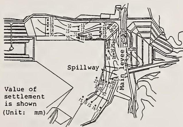
Fig. 14 Plan of the Nagara Dam (including settlement)
