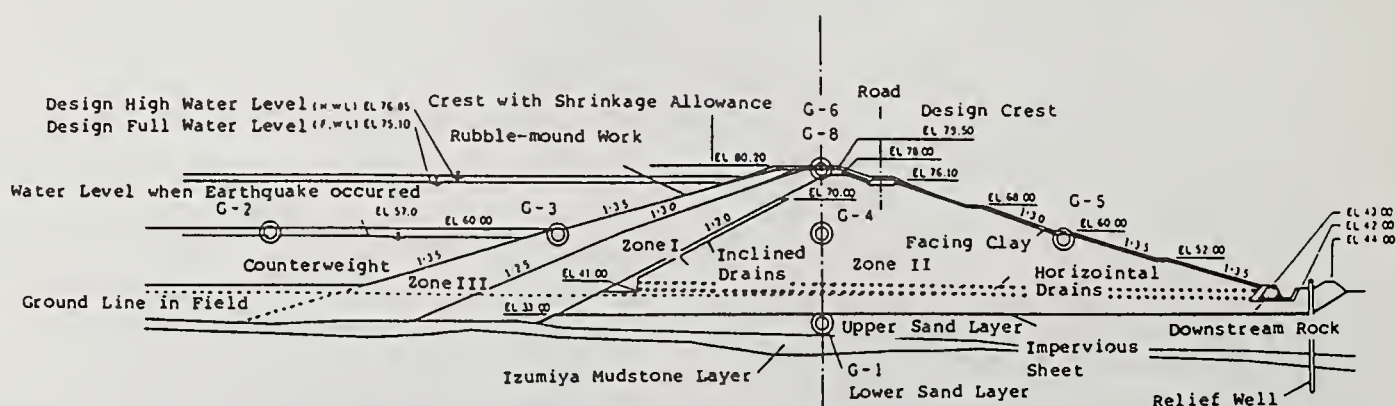
Fig. 2 Cross Section of the Nagara Dam
