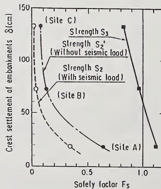
Fig.4 Safety factor vs. crest settlement
