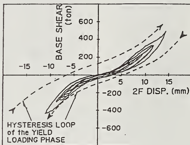
Fig.14 Relationship Between Base Shear and the First Story Displacement During Pseudo Dynamic Test
