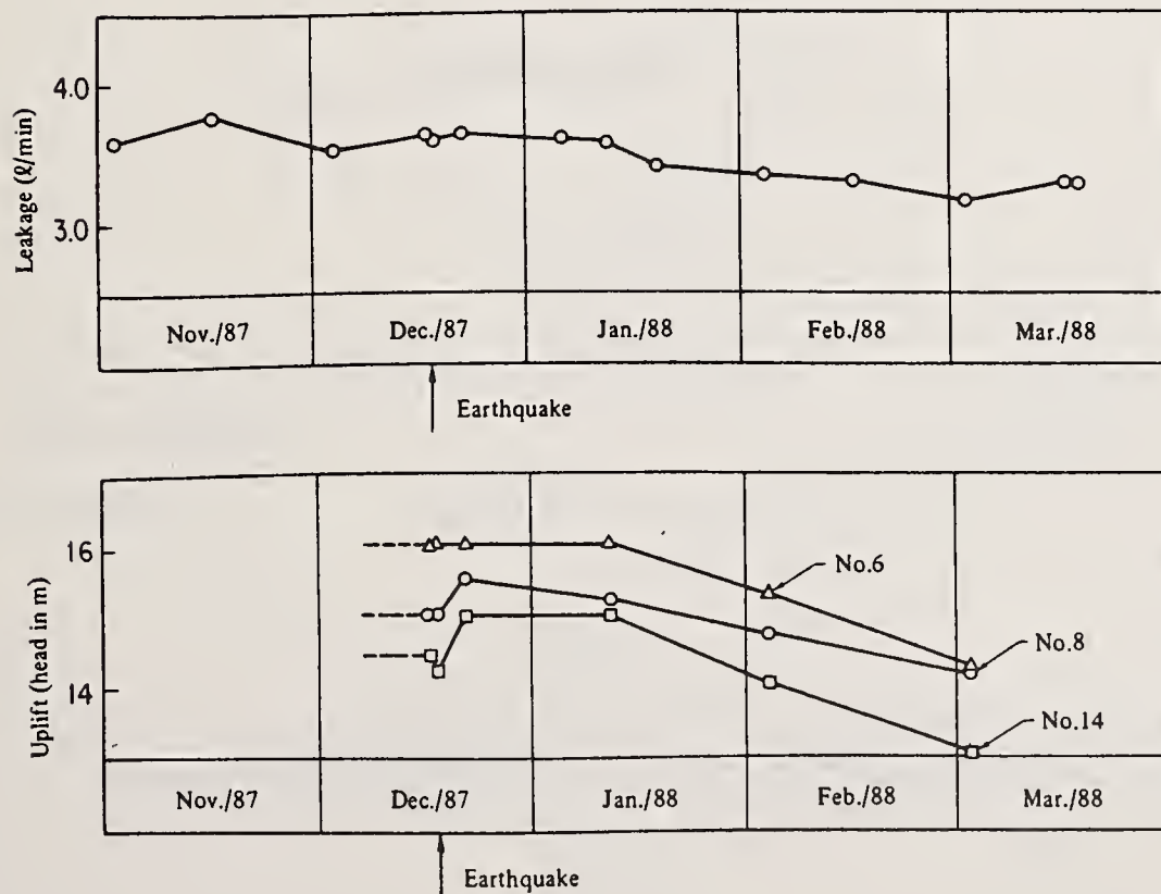
Fig. 4 Leakage and Uplift in Kameyama Dam
