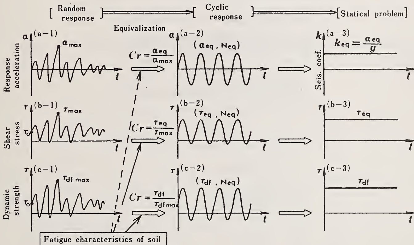
Fig.6 Transformation of irregular response problem to pseudostatic problem
