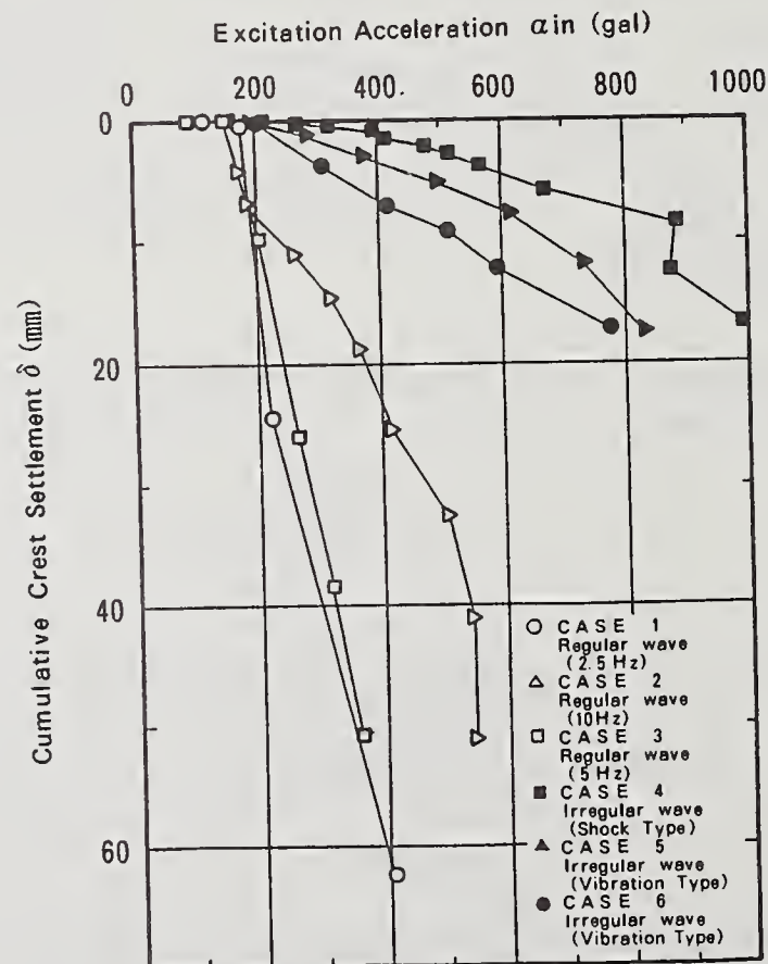
Fig.9 Input acc. vs. cumulative crest settlement
