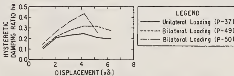
Fig.16 Comparison of Equivalent Hysteretic Damping Ratio
