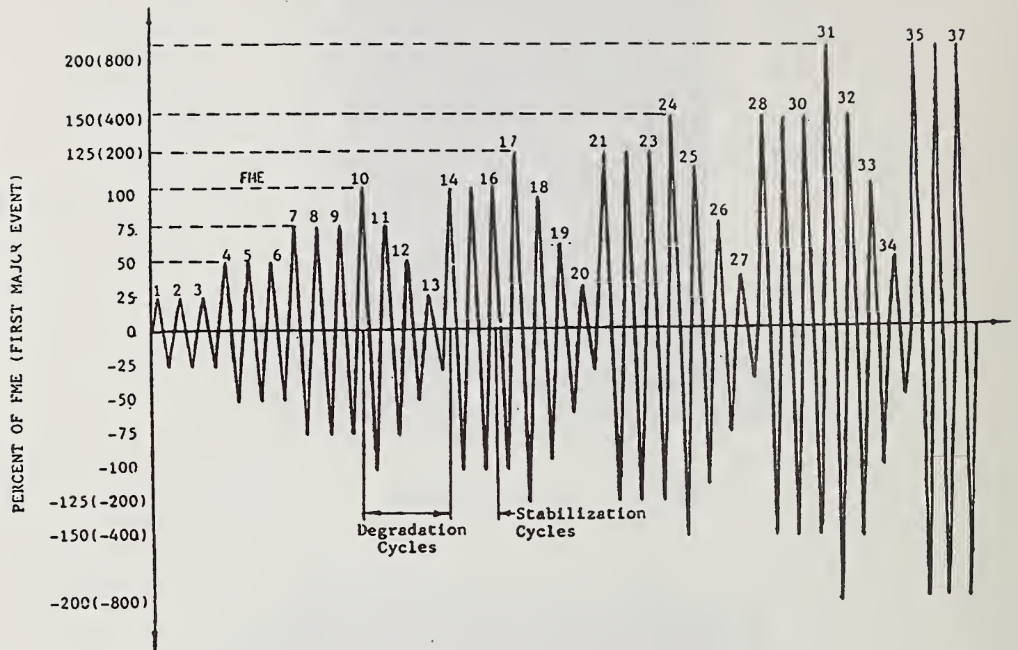
Figure 4 - Cyclic Loading History Used For Masonry Walls
