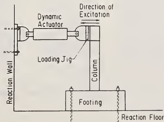
Fig.7 Experimental Set-up in Circular Hollow Section
