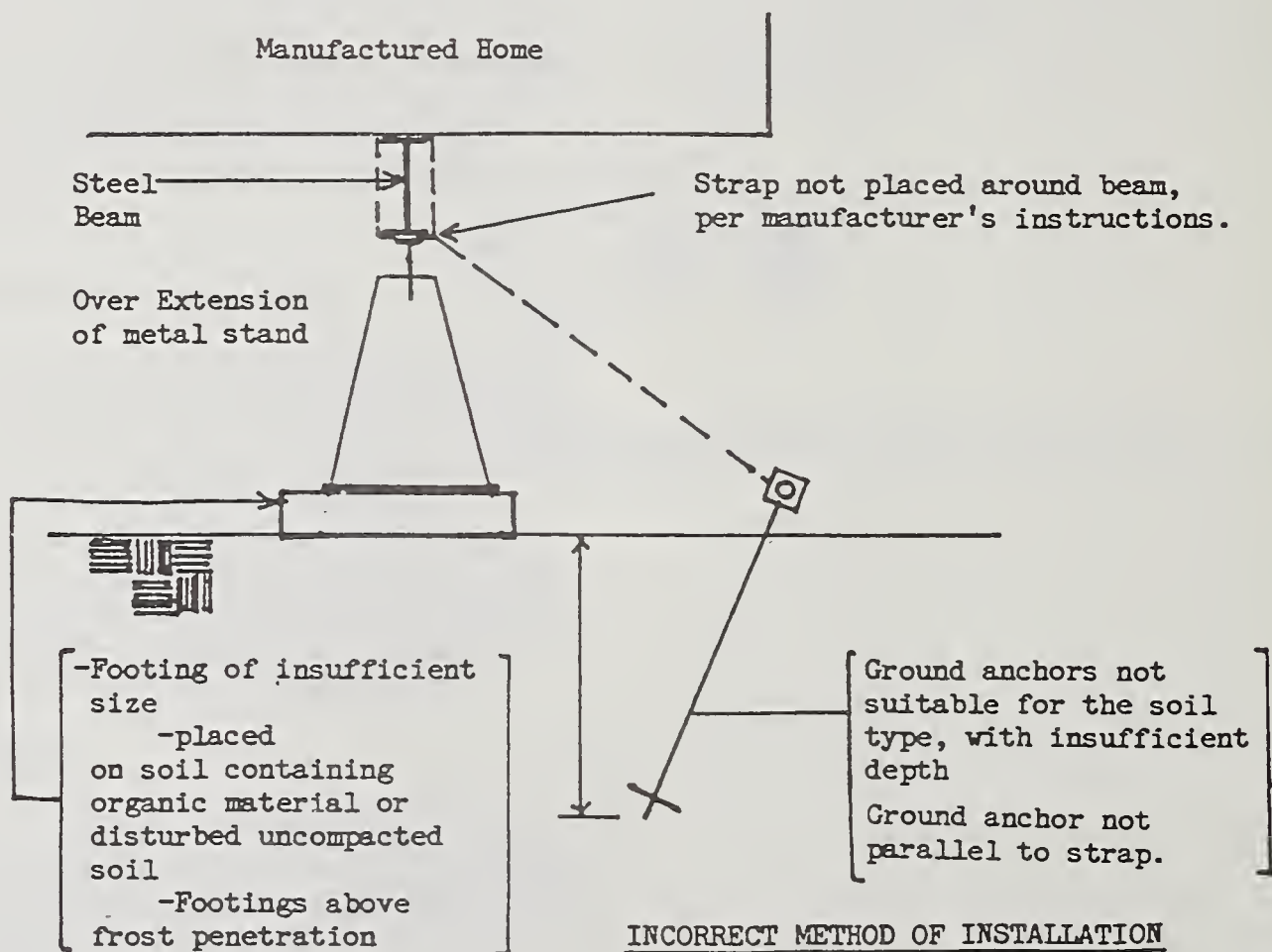
Figure 3 Incorrect Installation and Foundation
