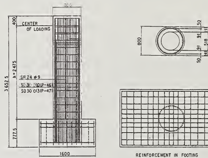
Fig.2 Test Specimens with Circular Hollow Section
