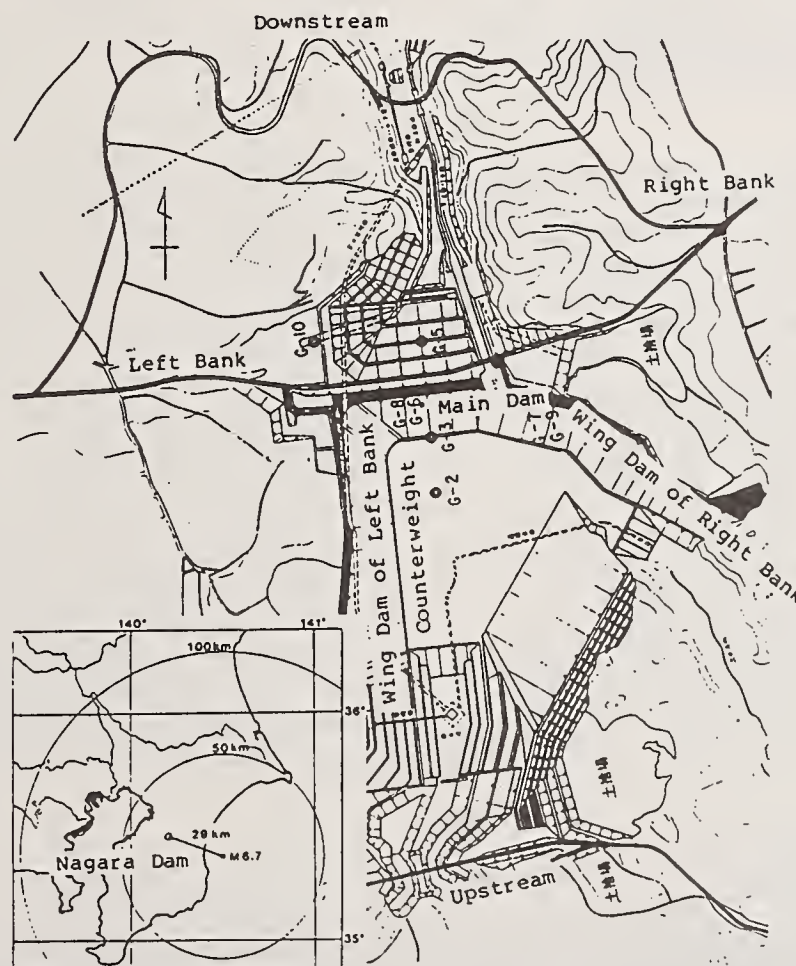
Fig. 1 Plan of the Nagara Dam
