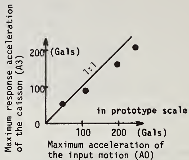
Fig.7 The maximum response acceleration of the caisson.
