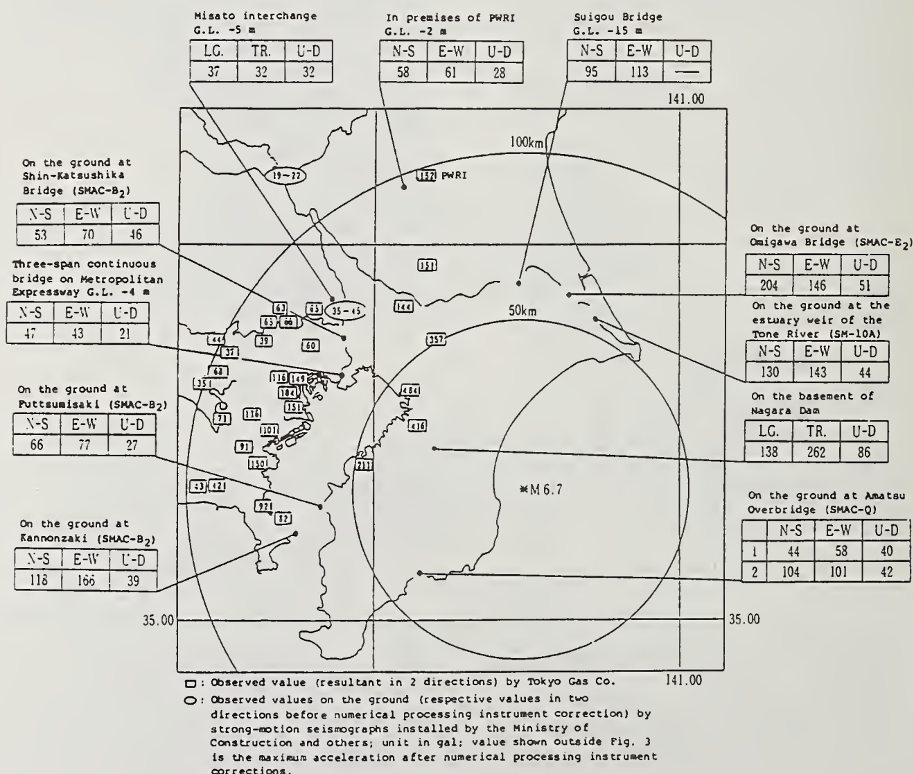
Fig. 3 Maximum acceleration at various places
