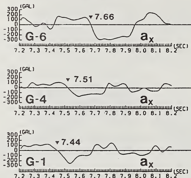
Fig. 11 Wave Propagation (Upstream-Downstream Direction, Method 2)
