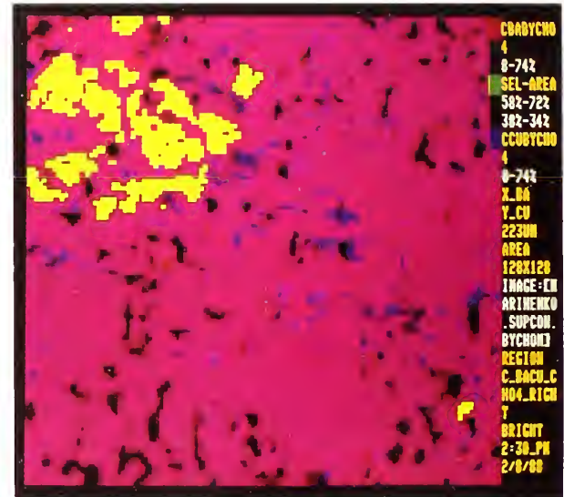
Figure 10(d). Mask of the selected linear feature pixels in figure 10(c) superimposed on the original maps. Image width = 223 micrometers (sample courtesy John Blendell, NIST; images courtesy R. Marinenko and D. Bright, NIST).
