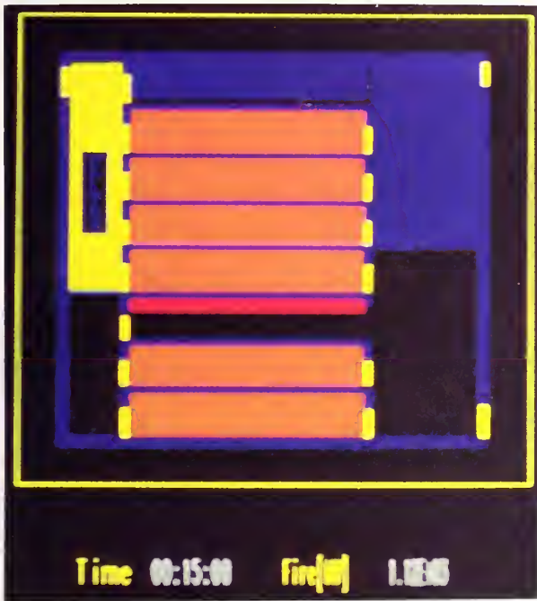
Figure 14. Conditions during the Plaza Hotel fire using a zone fire model. Colors indicate increasing levels of life hazard from blue (none), yellow, orange, and red (on the fire floor).
