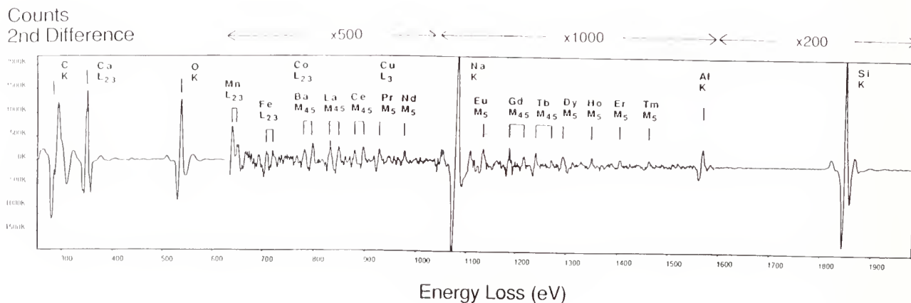
Figure 20. Analytical electron microscopy/parallel detection electron energy loss spectrum of NIST SRM 610. Second difference spectrum.
