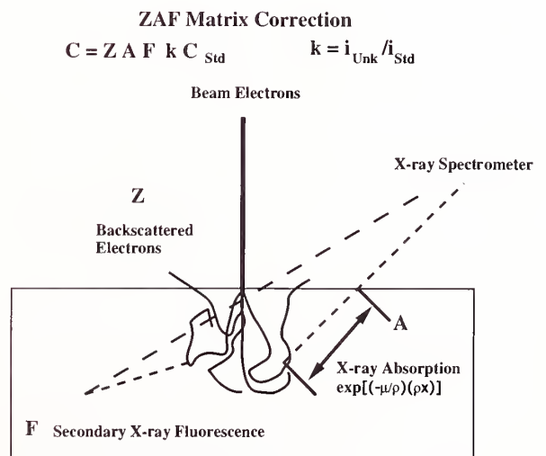
Figure 4(c). Physical origin of corrections to measured radiation for electron backscattering/penetration, x-ray absorption, and x-ray induced secondary fluorescence.
