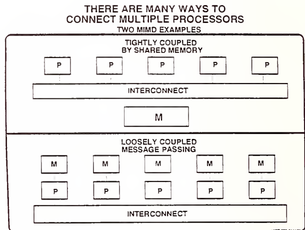
Figure 2. Tightly and loosely coupled MIMD architectures.
