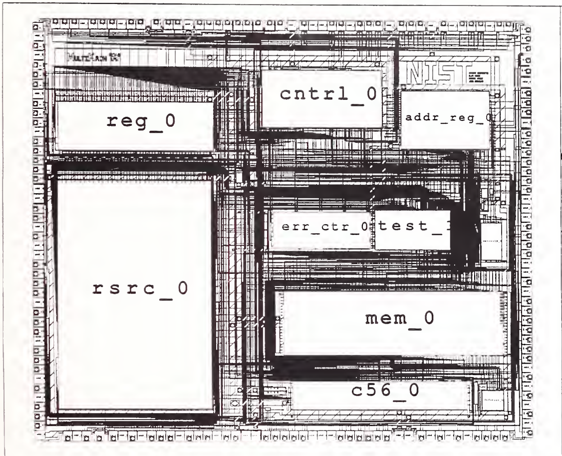
Figure 16. Multikron layout.
