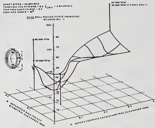
Fig. 15—Optimization of ball separator for minimum ball-pocket FORCE
