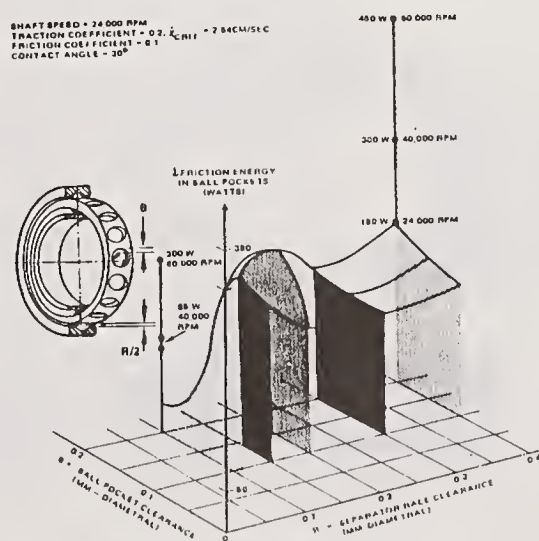
Fig. 14—Optimization of ball separator for minimum ball-pocket WEAR
