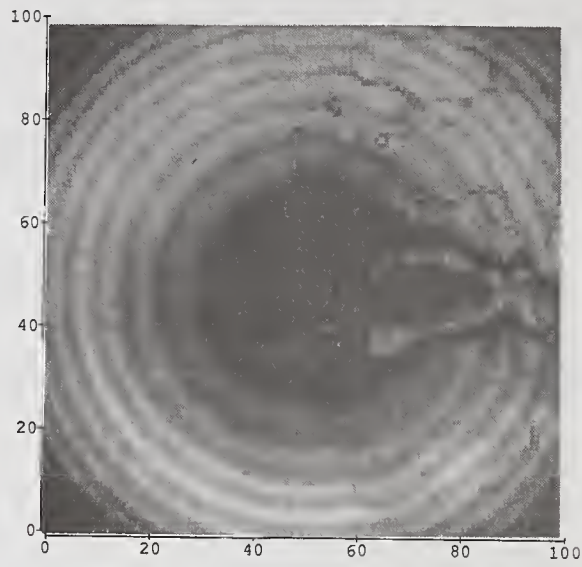
Ceramic Ball, Radius=1/8" Scan Area= 1mm x 1mm, Defocused 0.40 mm
