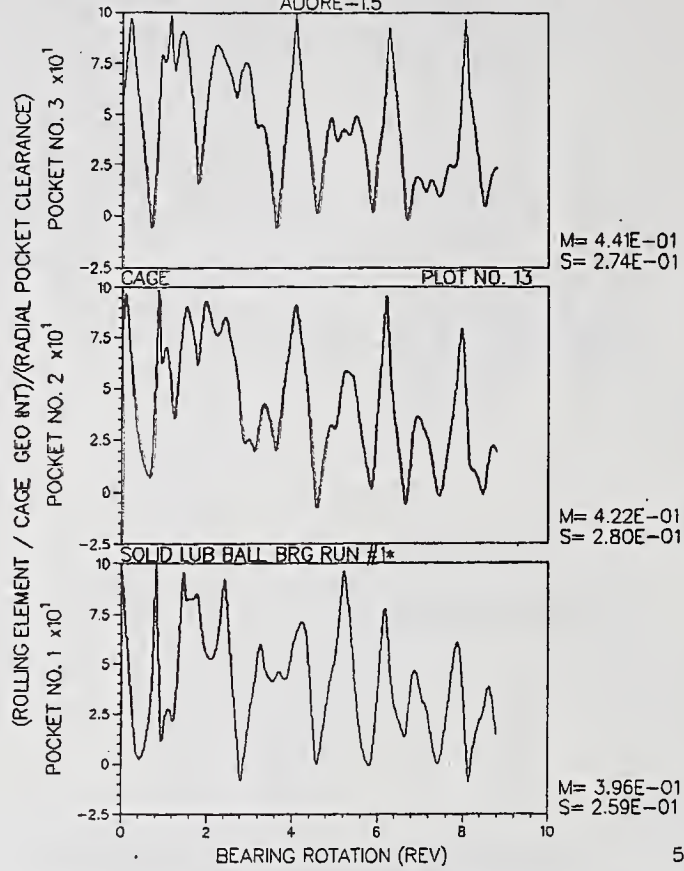
Figure 5. ADORE Computer Simulated Plots of Solid Lubricated Ball/Cage Relative Motions Producing Impacts in Fig. 4
