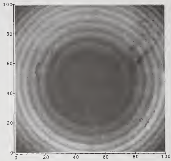
Ceramic Ball, Radius=1/8" Scan Area= 1mm x 1mm, Defocused 0.35 mm
