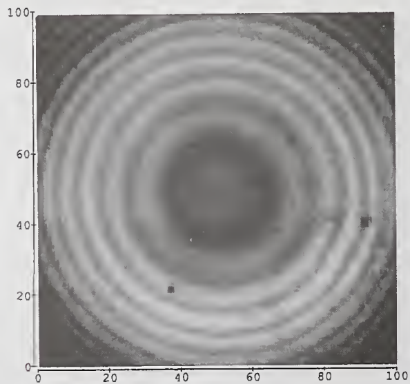
Ceramic Ball, Radius=1/8" Scan Area= 1mm x 1mm, Defocused 0.25 mm
