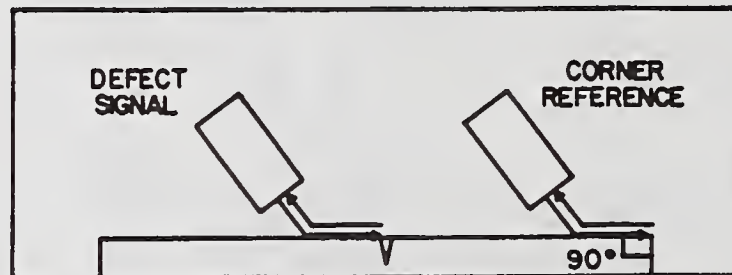
TRANSDUCER-SAMPLE GEOMETRY FOR SINGLE CRACK DATA
