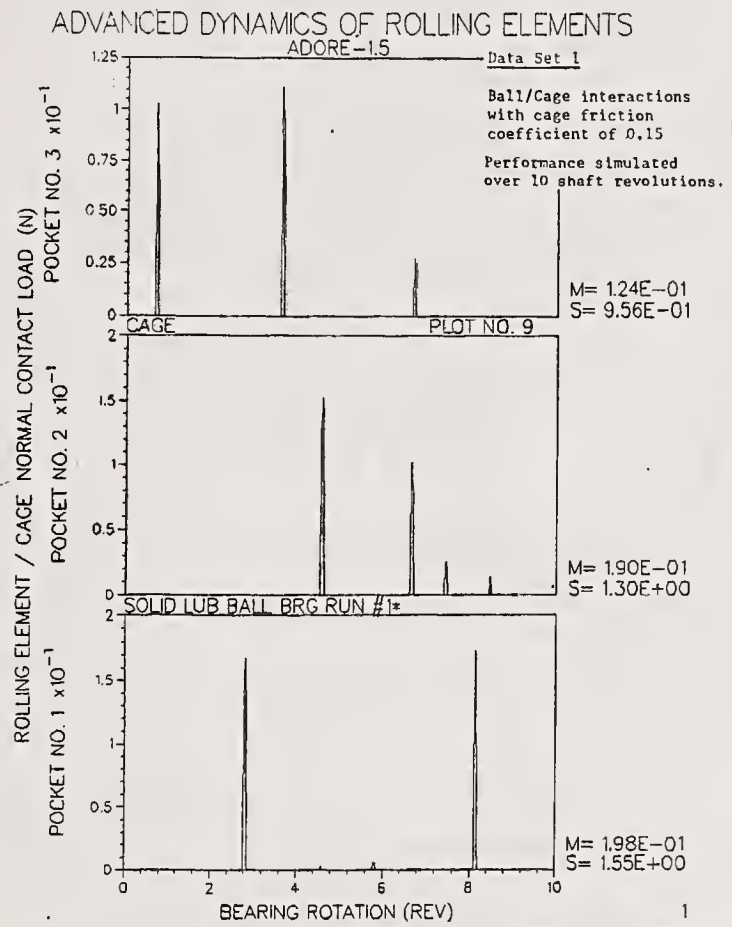
Figure 4. ADORE Computer Simulated Plots of Solid Lubricated Ball/Cage Impact Loads
