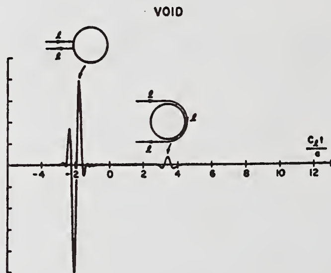
Fig. 4a. Relative scattering cross-section from a void as a function of time.
