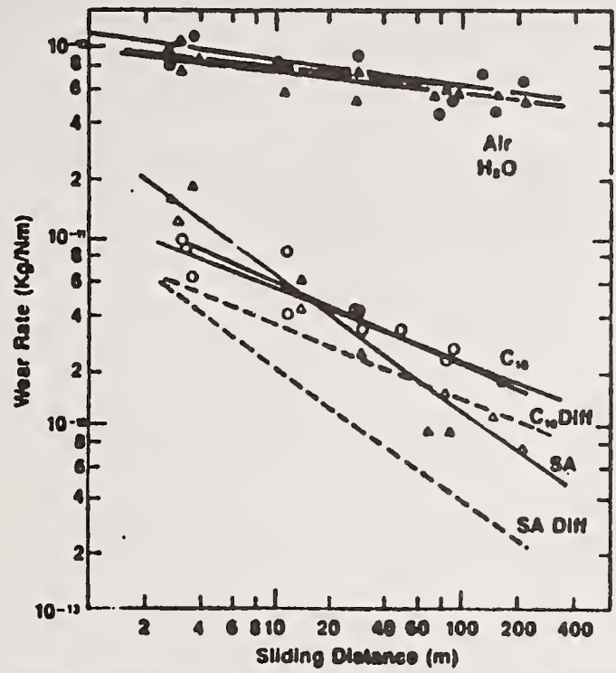
—Logarithmic plot of the wear rate of Si 3 N 4 sliding against itself at low velocity in various environments.
