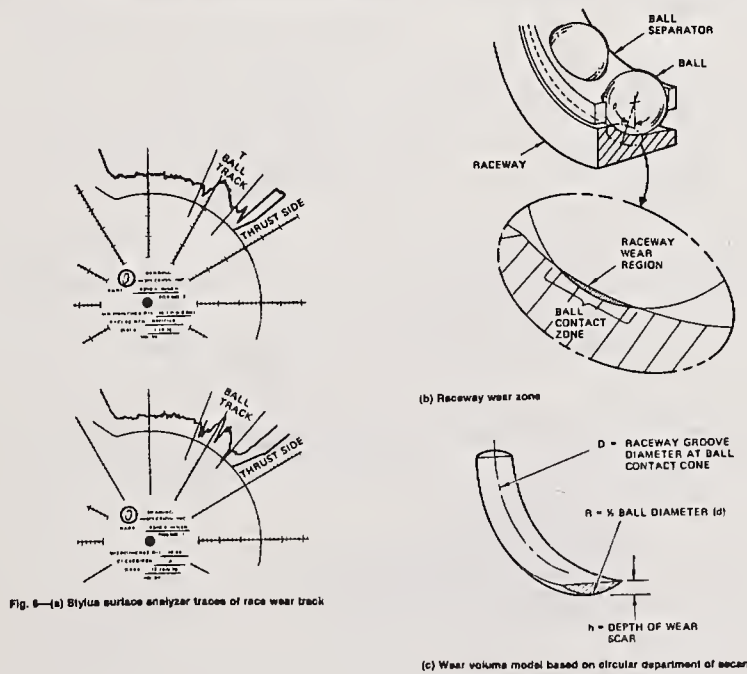
(c) Wear volume model based on circular department of sector
