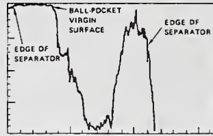
Surface analyzer trace of ball-separator ball-pocket wear
