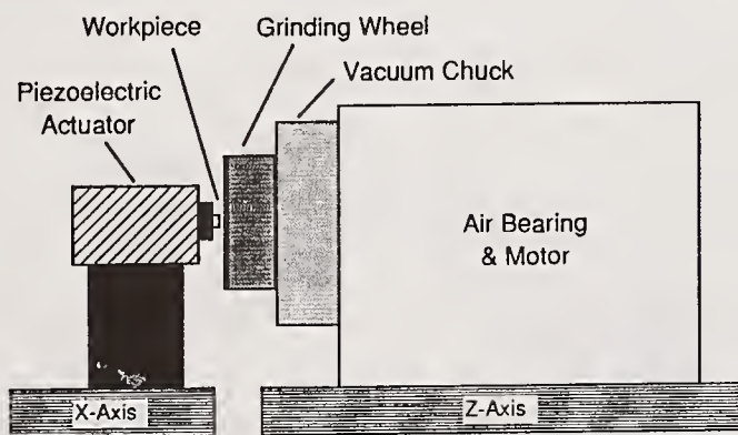
Schematic of the plunge grinding apparatus.
