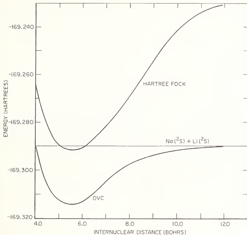
Fig. 11. Extended Hartree-Fock potential curves for LiNa.
