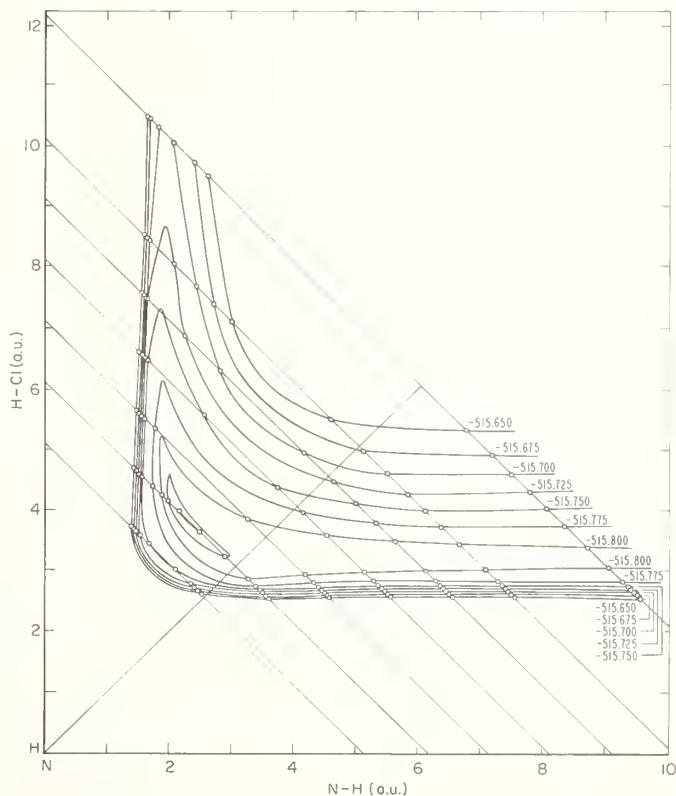
Fig. 17. Reaction surface for \text{NH}_3 + \text{HCl} \rightarrow \text{NH}_4\text{Cl} (horizontal valley) or \text{NH}_3 + \text{Cl} \rightarrow \text{NH}_4\text{Cl} (vertical valley). The abscissa gives the N-H(4) distances; the ordinate gives the H(4)-Cl distances. Each energy contour represents steps of 0.025 a.u. ( \approx 0.68 e.v.).
