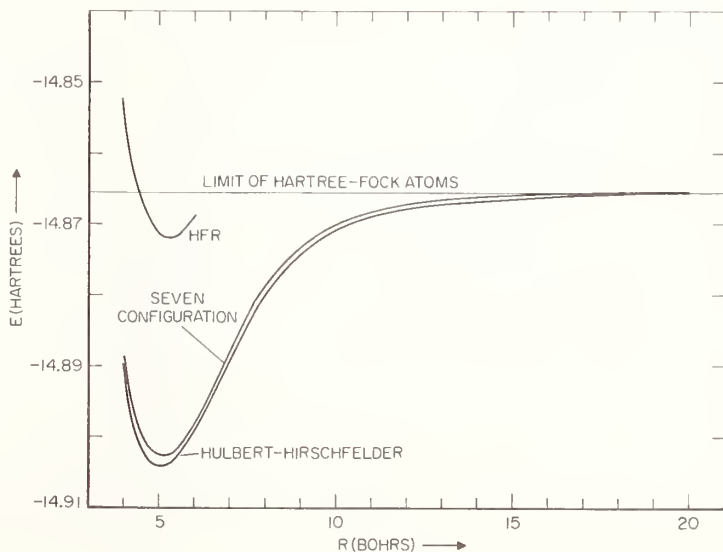
Fig. 5. \text{Li}_2 potential curve. Comparison of extended Hartree-Fock theory with experiment.
