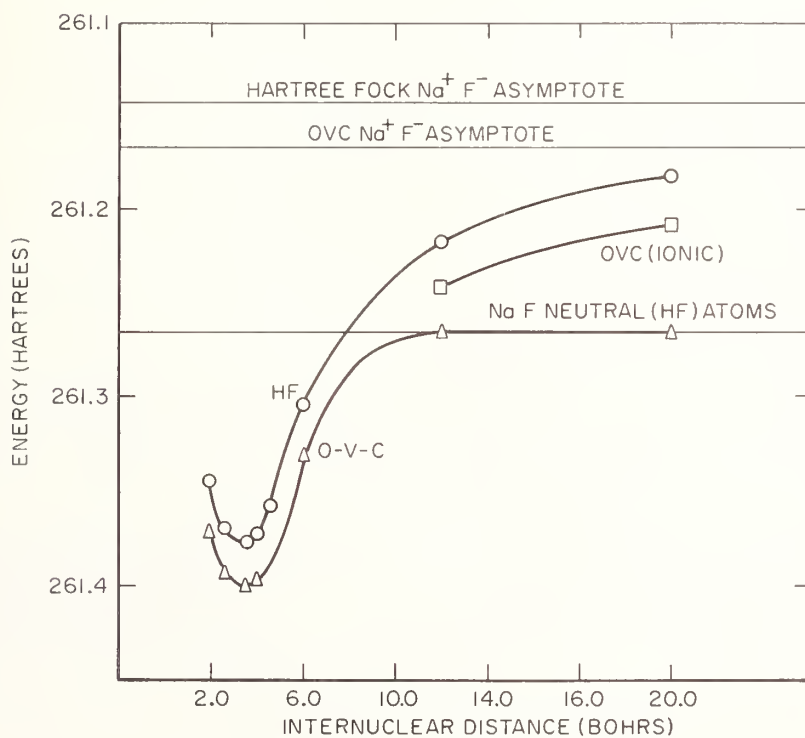
Fig. 12. Extended Hartree-Fock potential curves for NaF.
