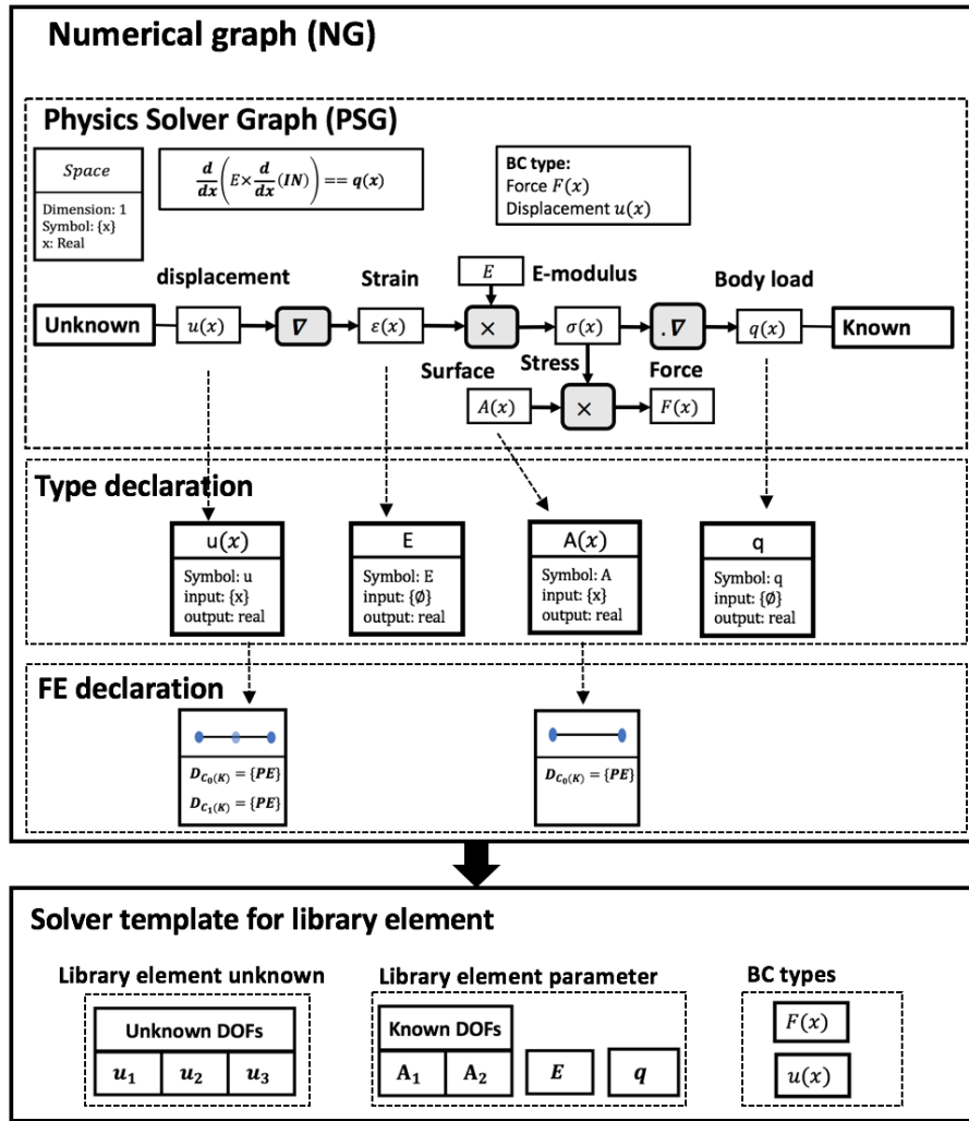
Figure 2: Example numerical graph for a bar element
