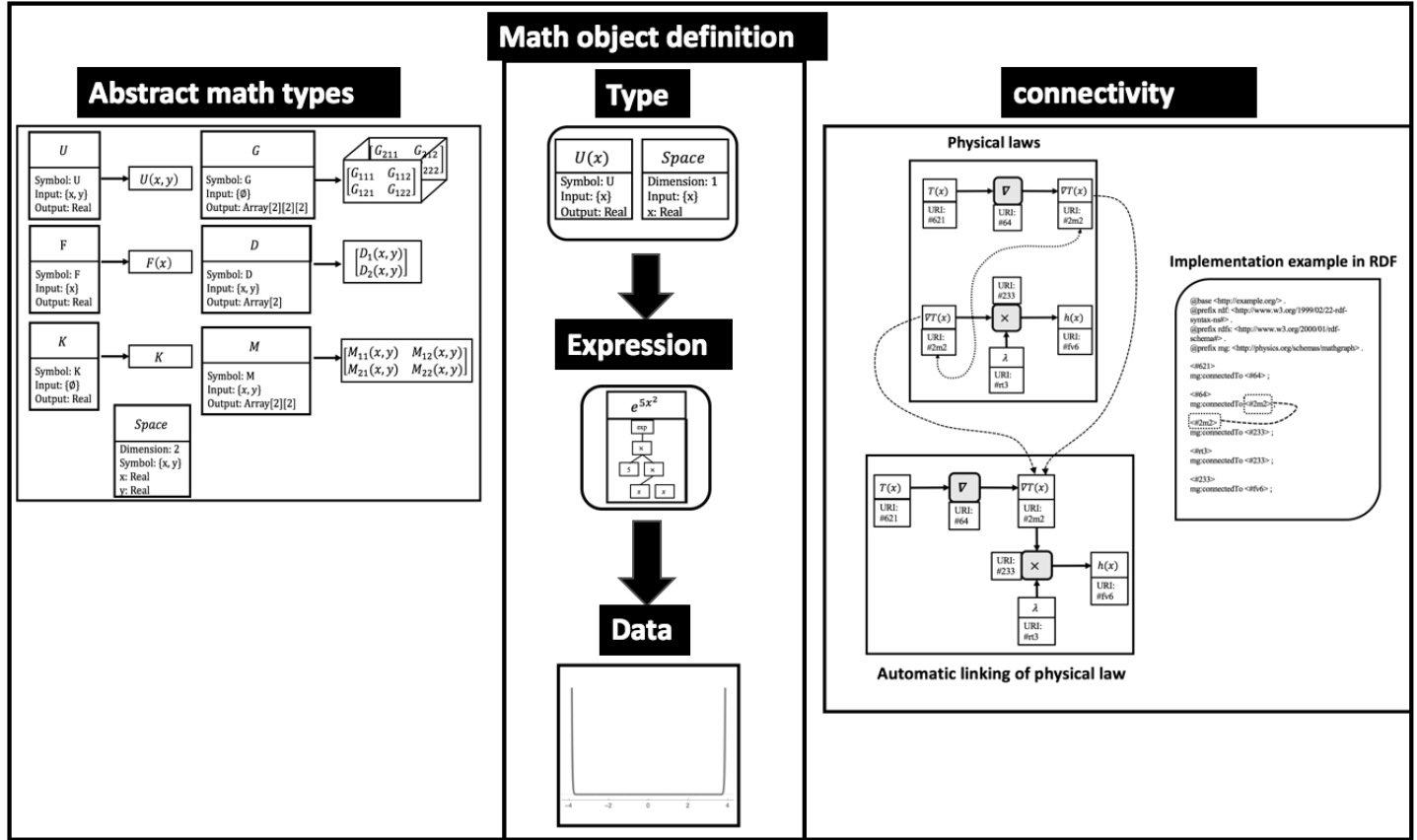
Figure 1: Layers of math objects
