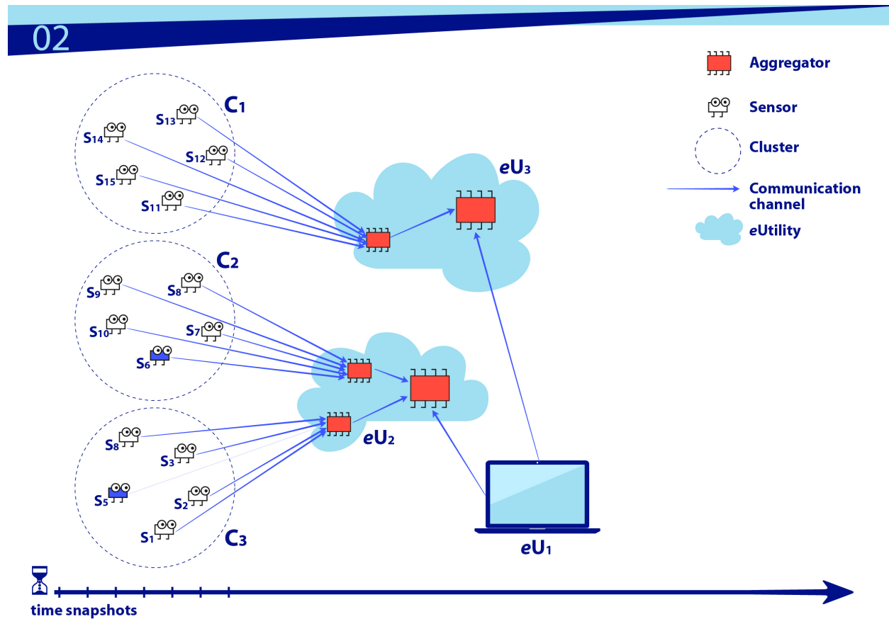
Figure 2: eUtility
