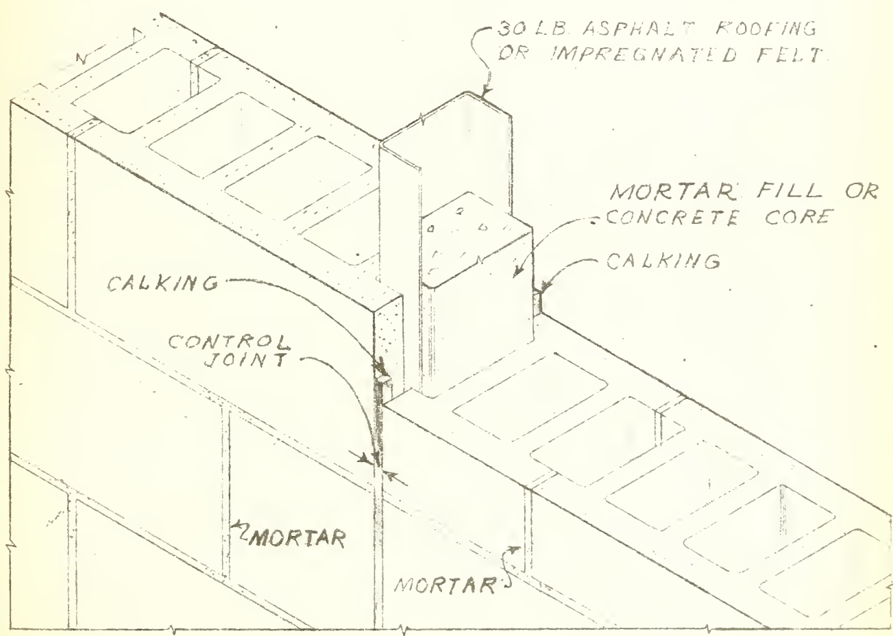
FIG. 4 TYPICAL CONTROL JOINT USING STANDARD STOCK STRETCHER BLOCK AND CONCRETE CORE.
