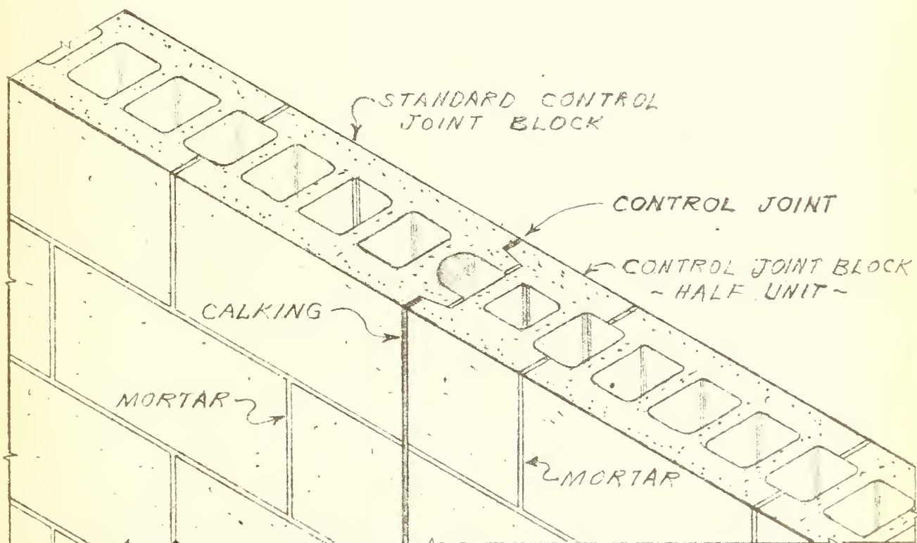
FIG. 6 TYPICAL CONTROL JOINT USING STANDARD CONTROL JOINT BLOCK
