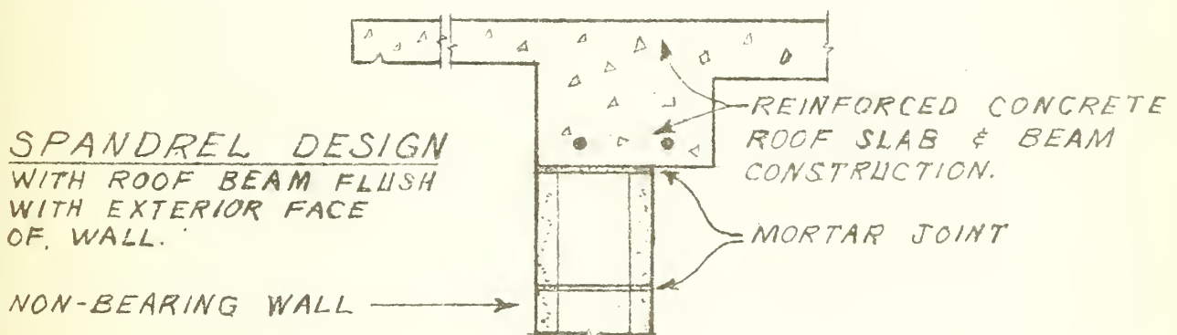
DETAIL OF INTERSECTION OF ROOF & WALL WITH NON-BEARING WALL STRUCTURE.
