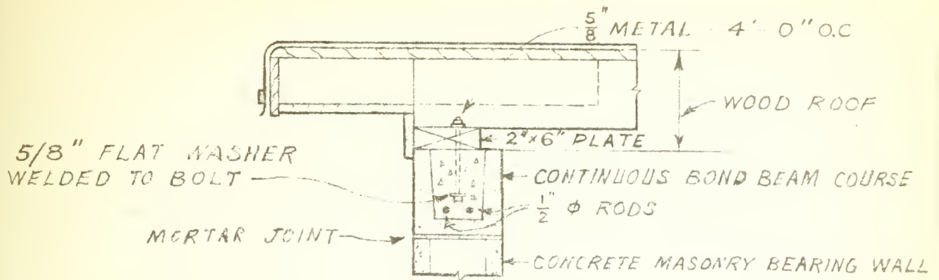
DETAIL OF INTERSECTION OF ROOF & WALL OF ONE STORY STRUCTURE WITH BEARING WALL & WOOD ROOF.
