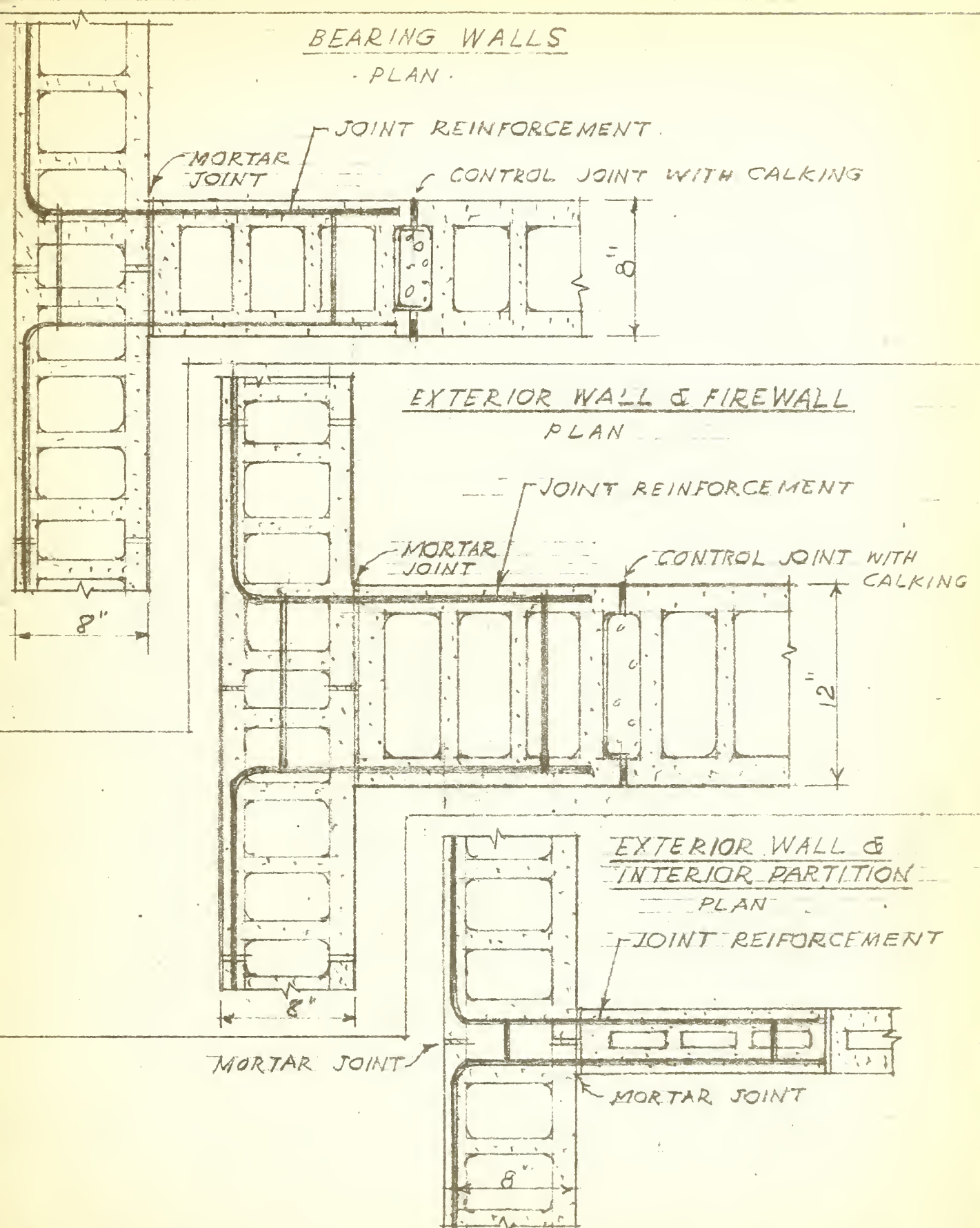
FIG. 9 WALL INTERSECTION SHOWING WIRE WALL TIES
