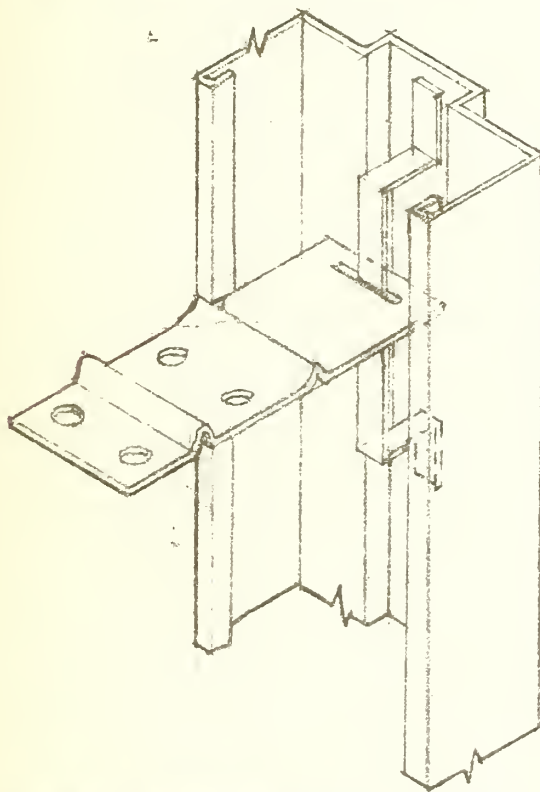
UNDERWRITER'S TYPE ANCHOR
