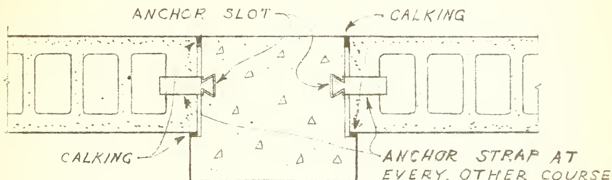
PLAN OF REINFORCED CONCRETE COLUMN SHOWING DOVETAIL TIE.
