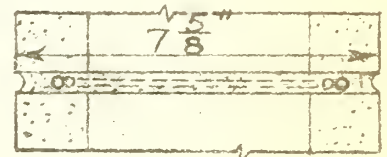
DETAIL THRU WALL WHERE SPLICE OCCURS
