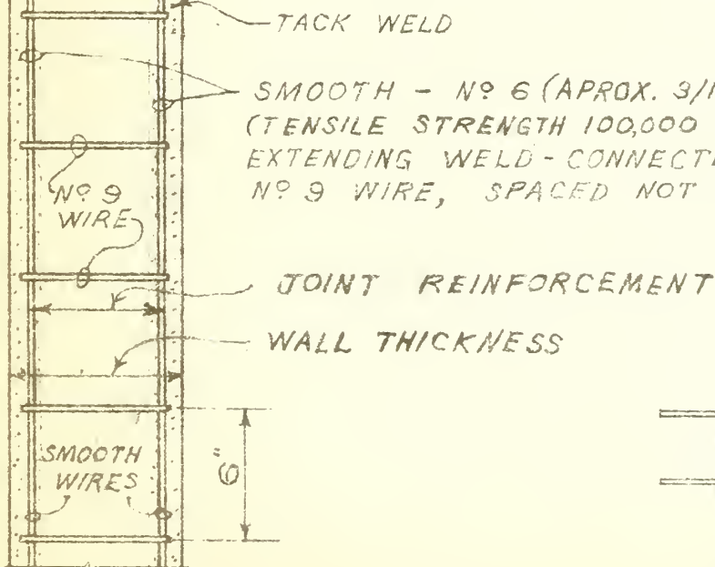
OPTIONAL TYPES OF JOINT REINFORCEMENT
