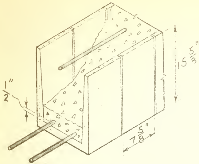
BEAM LINTEL BLOCK
