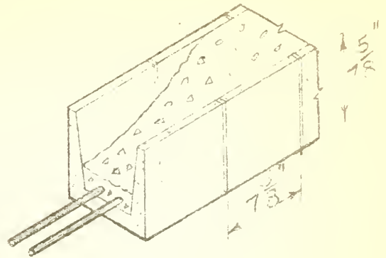
BEAM LINTEL BLOCK
