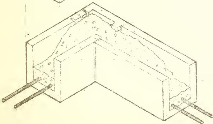
BOND BEAM BLOCKS AT CORNER
