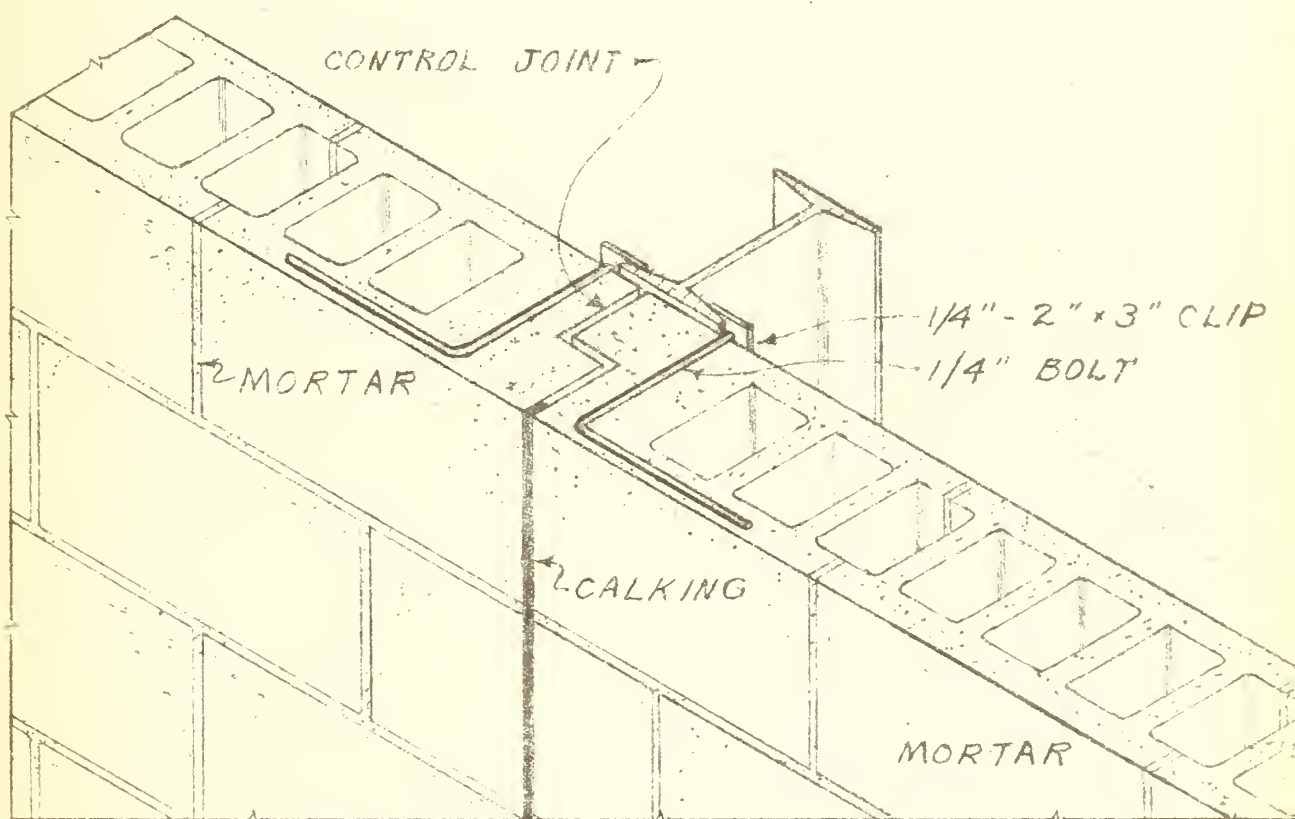
FIG. 7 TYPICAL CONTROL JOINT USING STANDARD STOCK JAMB BLOCK AND METAL CLIPS & BOLTS
