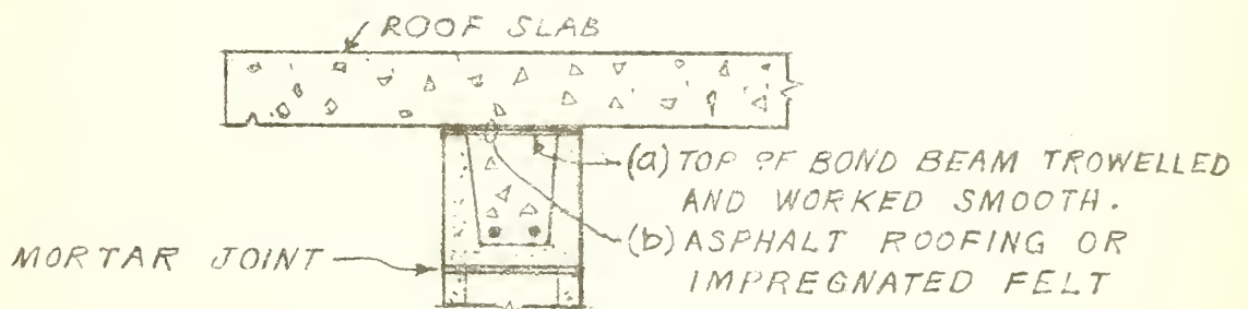
DETAIL OF INTERSECTION OF ROOF & WALL OF ONE STORY BEARING WALL STRUCTURE HAVING CONCRETE ROOF SLAB.
