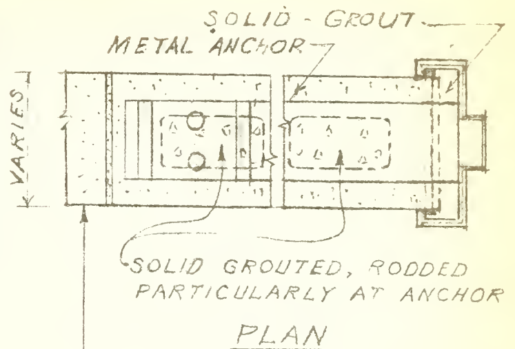
ADJUSTABLE T-ANCHOR
