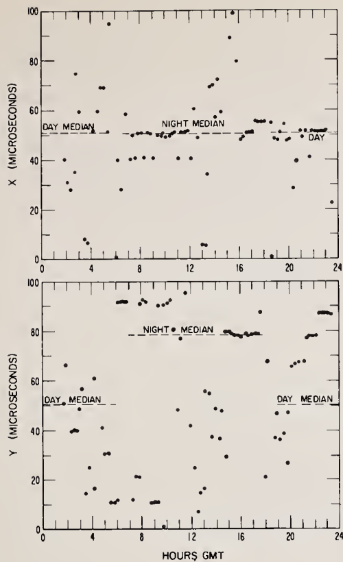
Figure 8.8. Wake Island, Nov. 1, 1963.
