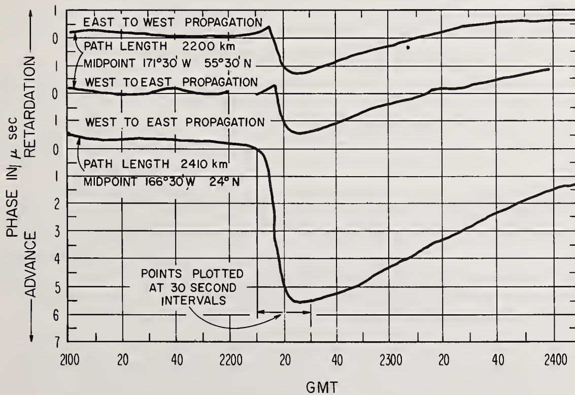
Figure 8.7. Solar event of September 28, 1961.
