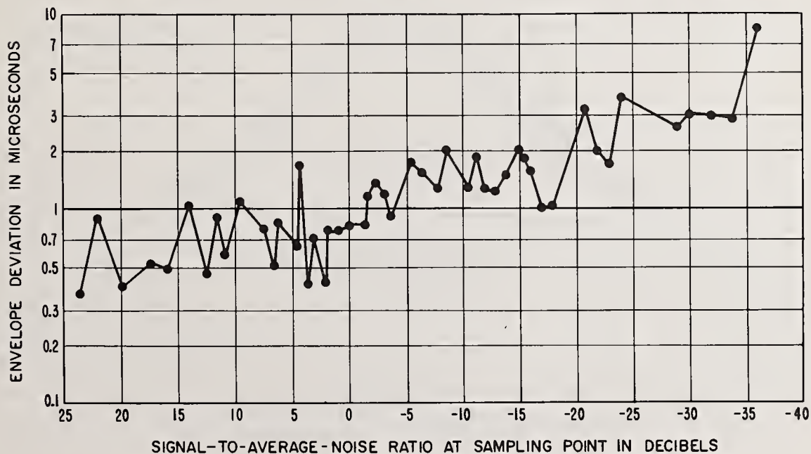
Figure 4.6. Cytac envelope deviations ordinate value not exceeded 90 percent of time.
