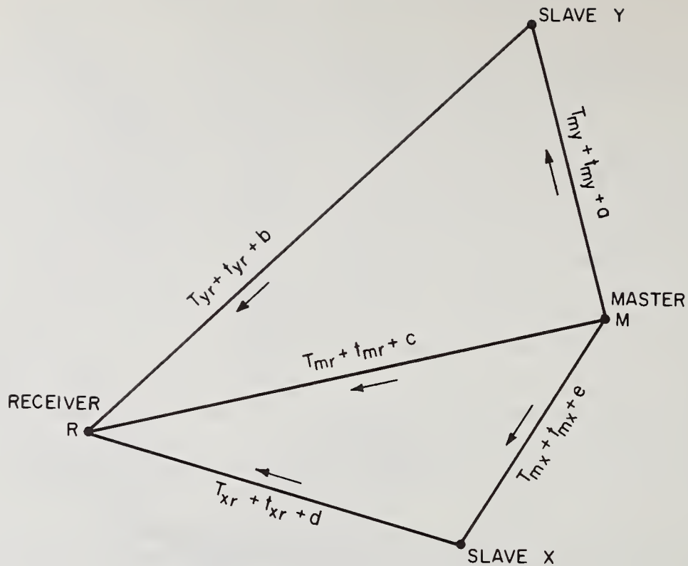
Figure 3.2 Loran triad geometry.
