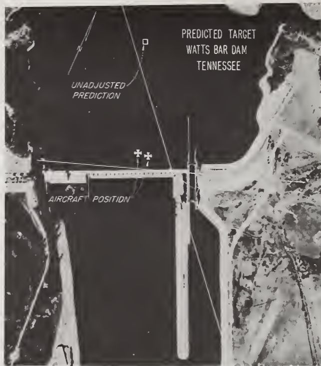
Figure 5.21. Simulated bombing runs. The unadjusted prediction shows the error that would have been made without using the correction contours.
