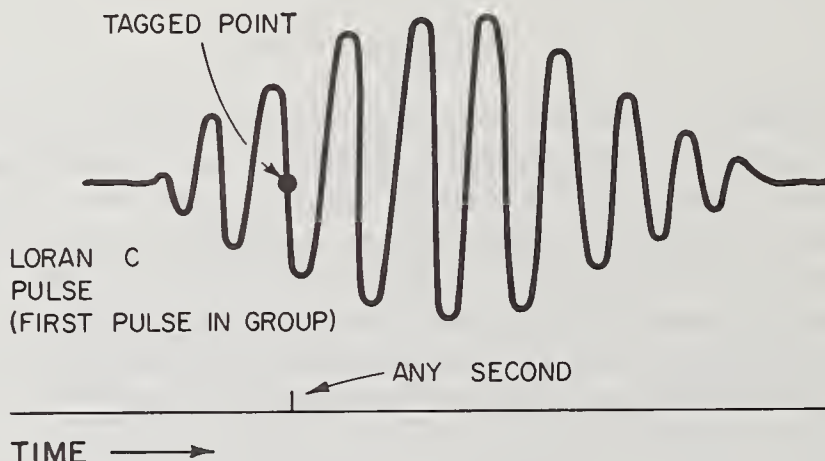
Figure 7.1. Time-scale distribution by Loran-C transmitter.
