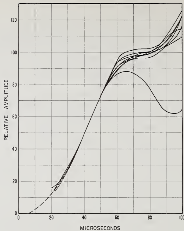
Figure 4.5. Pulse envelope tracings.
