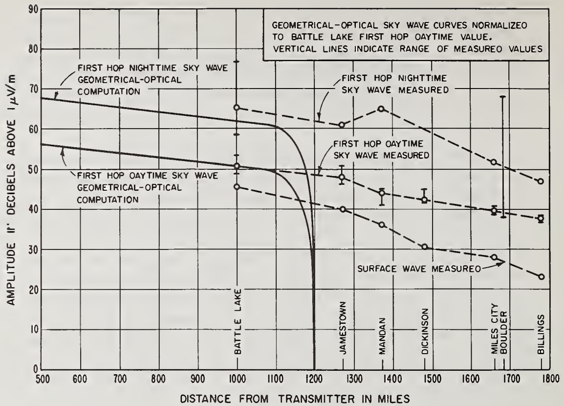
Figure 4.7. Cytac ground- and skywave measurements.
