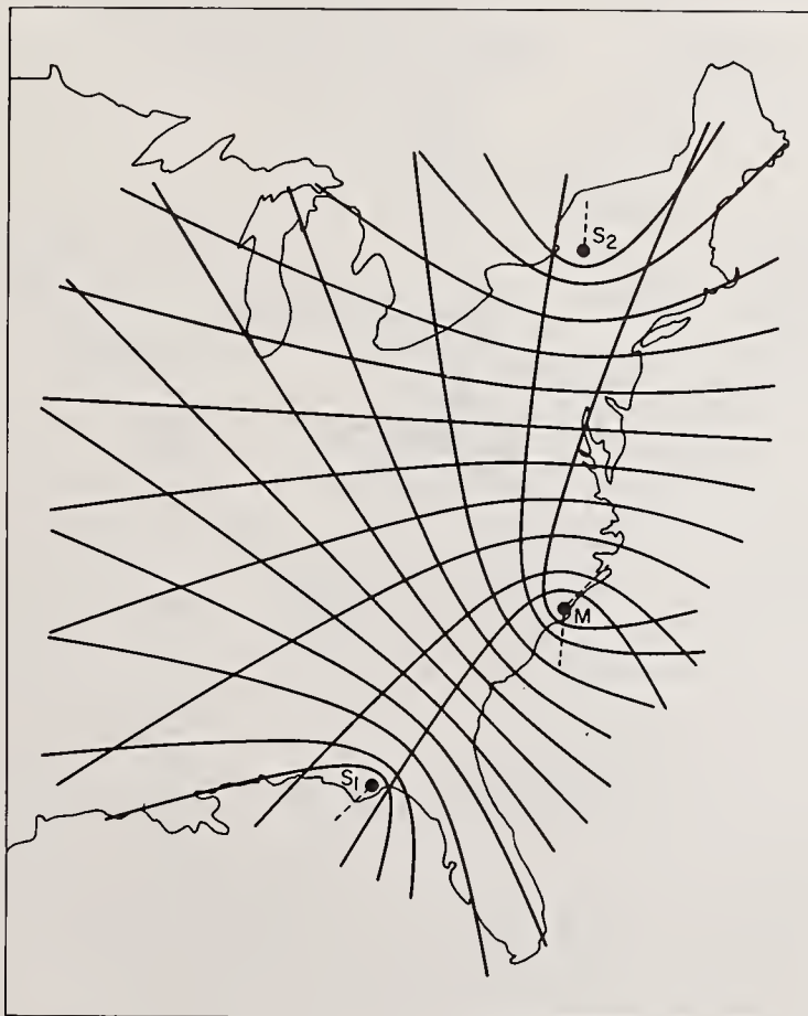
Figure 5.1. Cytac transmitters and grid.
