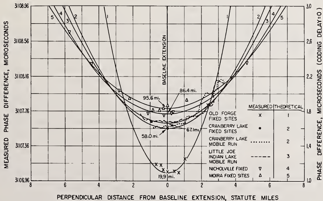
Figure 5.4. Forestport measurements. Smooth curves are for \sigma = 0.001 .
