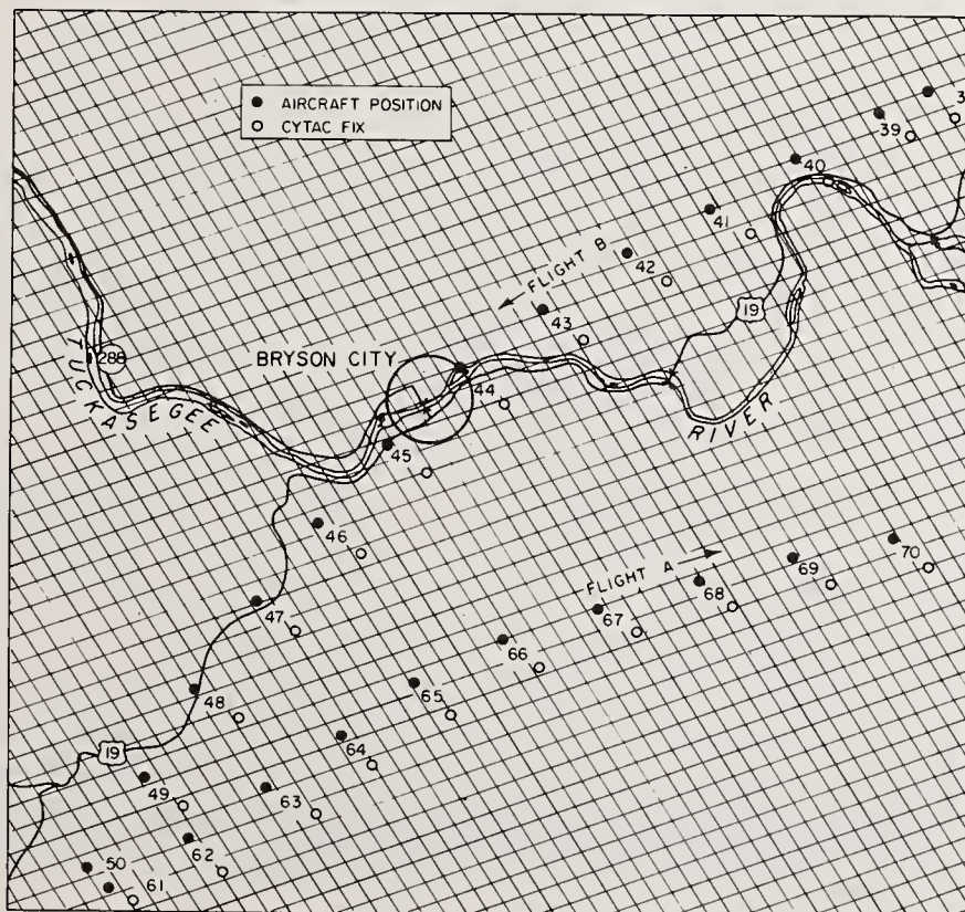
Figure 5.26. Airborne measurements of systematic errors.
