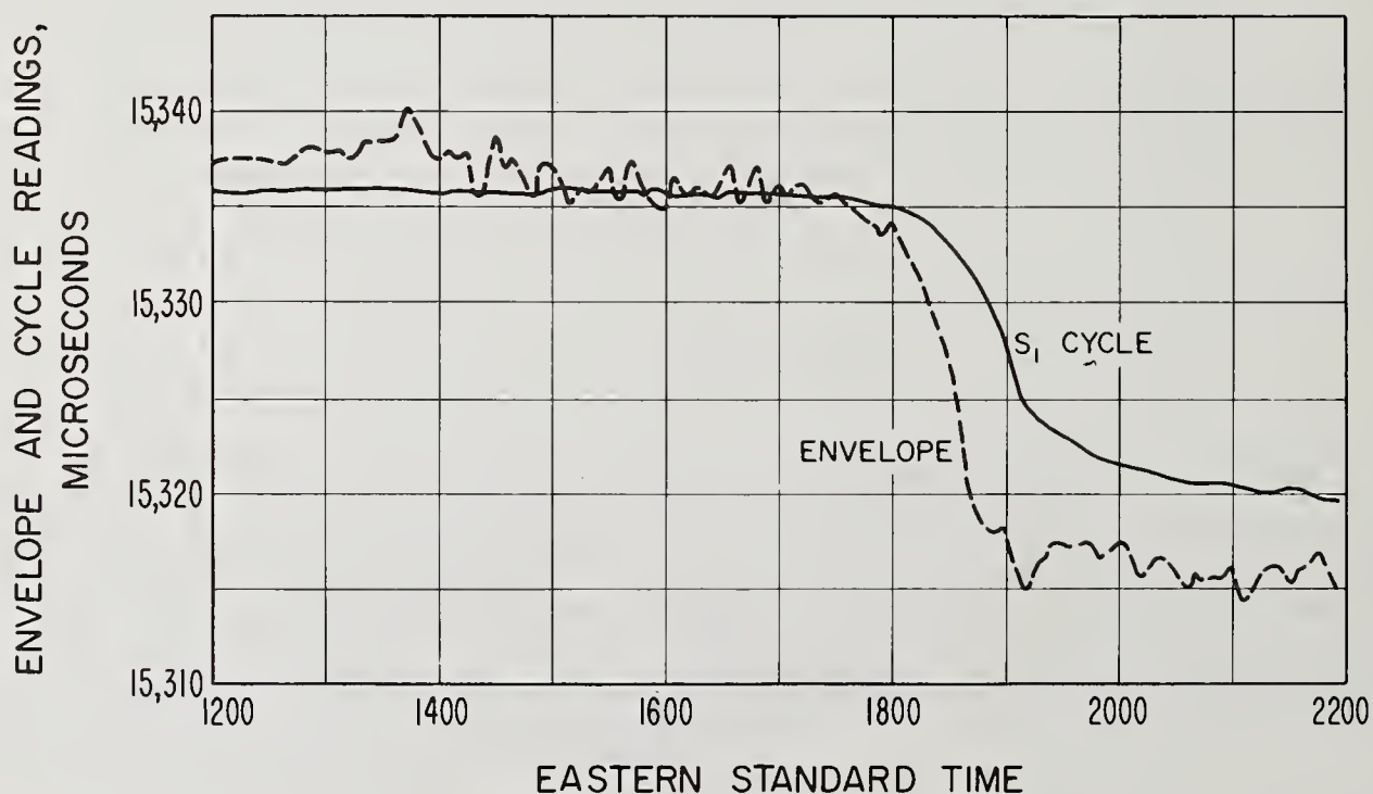
Figure 5.37. First-hop skywave measurements, Carolina Beach to Boulder.
