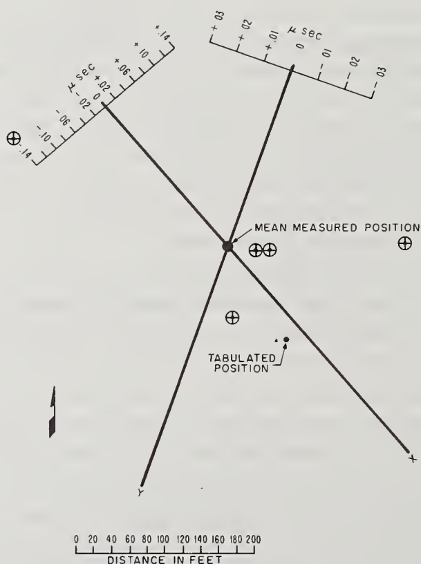
Figure 6.8. Airborne fixes, Walker Cay (Jansky & Bailey).
