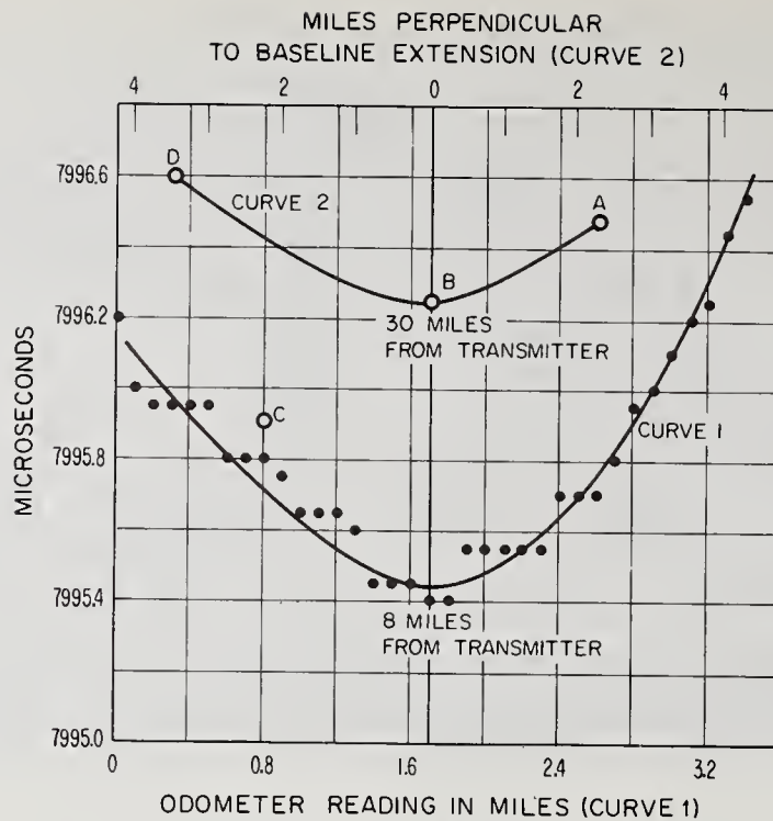
Figure 3.10. Cyclan baseline extension data.
