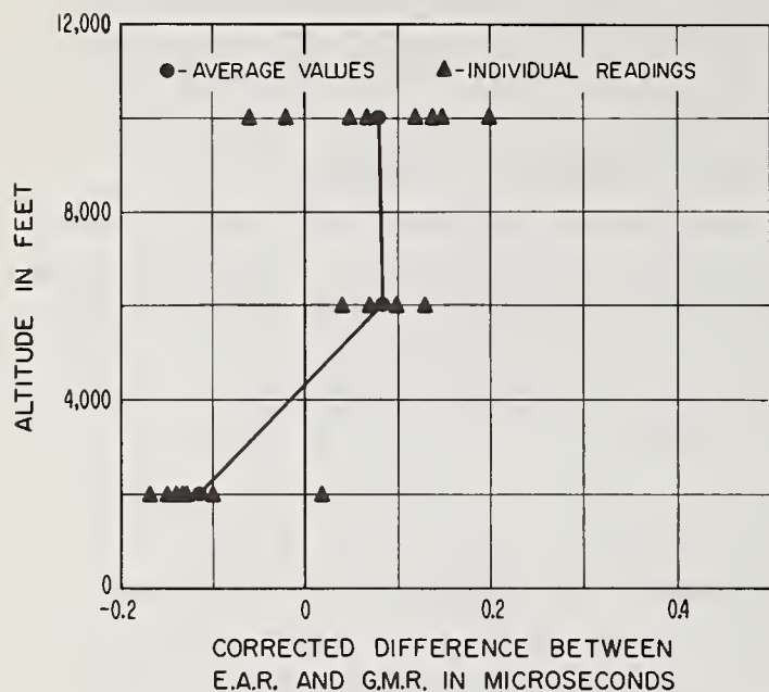
Figure 5.18. S_1 readings, Dayton, Tennessee.
