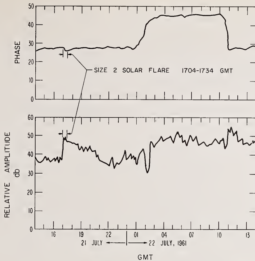
Figure 8.6. First-hop skywave from Carolina Beach, North Carolina, to Boulder, Colorado.
