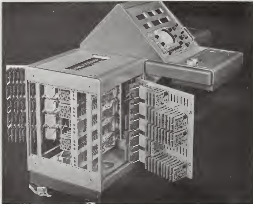
Figure 7.3. Loran-C Clock.
