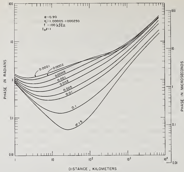
Figure 9.1. Secondary-phase corrections as a function of distance parametric in conductivity.
