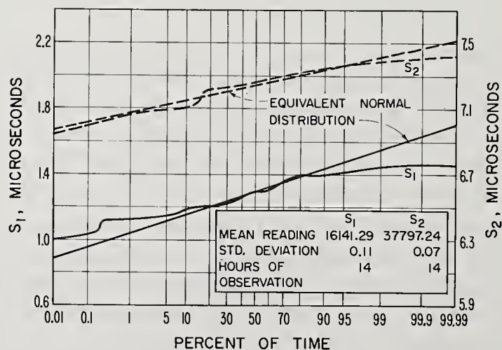
Figure 5.10. Readings at Twin City, Georgia.
