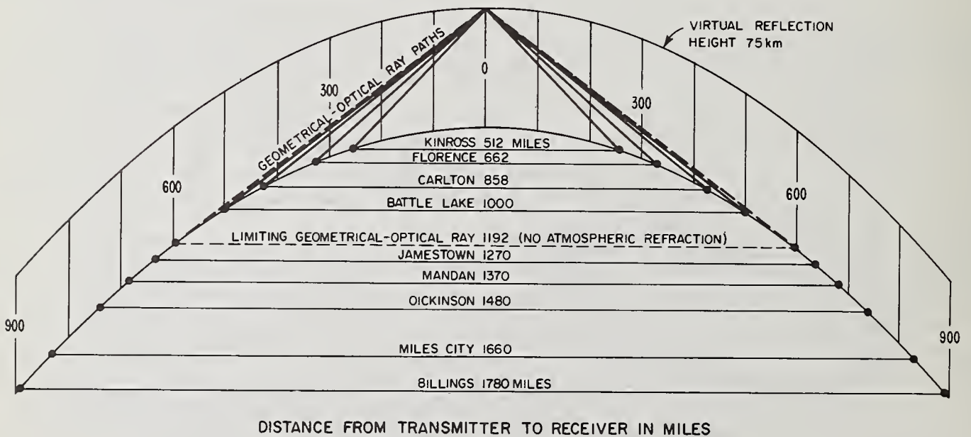
Figure 4.8. Geometric representation of skywave paths.
