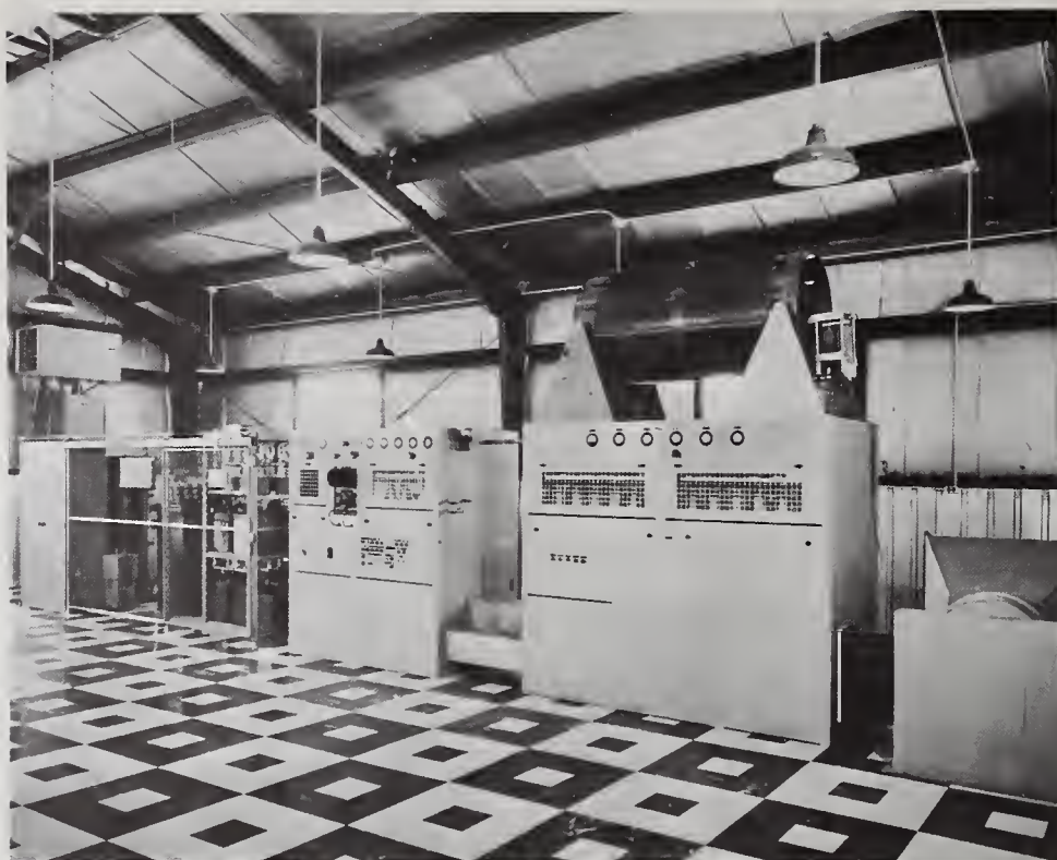
Figure 6.3. Jupiter transmitter (AN/FPN 15).
