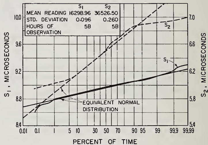
Figure 5.9. Readings at Dayton, Tennessee.
