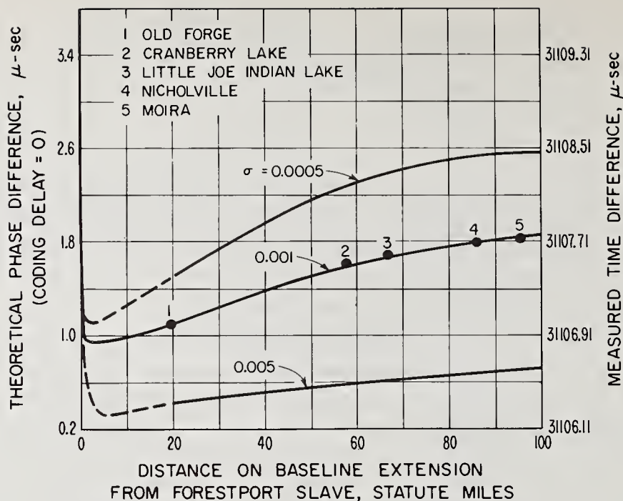
Figure 5.5. Forestport measurements.
