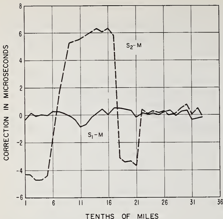
Figure 5.31. Time-difference errors from fig. 5.30.
