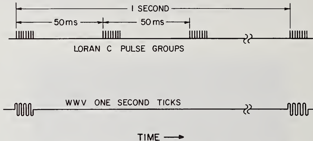
Figure 7.4 Pulse group to time relationship.
