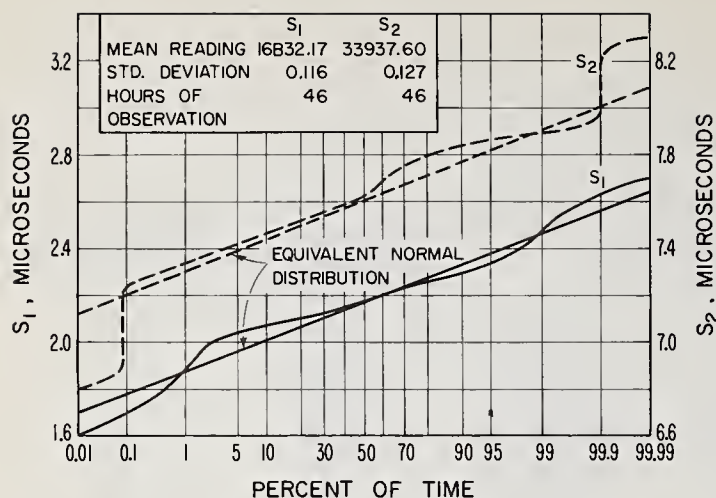
Figure 5.6. Readings at Williams Bay, Wisconsin.
