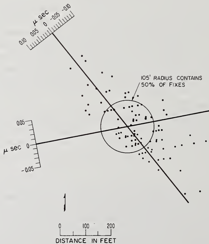
Figure 6.5. Bermuda fixes - September 4-6, 1957, 15-min averages (Jansky & Bailey).
