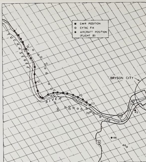
Figure 5.27. Measured systematic errors.
