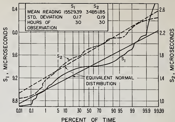
Figure 5.7. Reading at Smith Center, Kansas.
