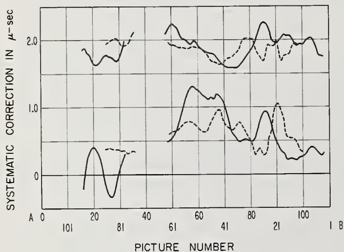
Figure 5.28. Airborne measurements of systematic corrections.
