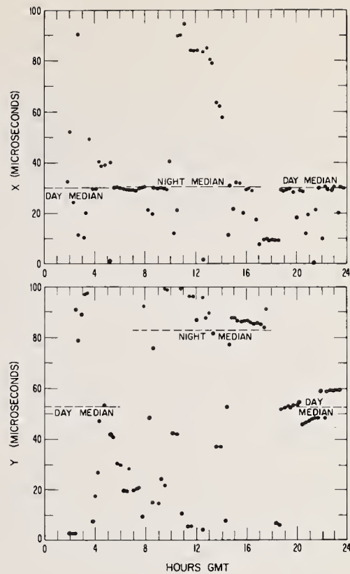
Figure 8.9. Wake Island, Nov. 8, 1963.
