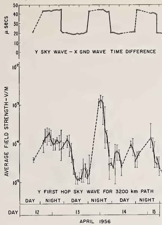
Figure 8.2. Phase and amplitude of the Loran-C skywave recorded on a north-south path.
