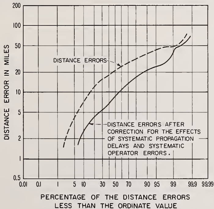
Figure 3.5. Wright Field data (Signal Corps).
