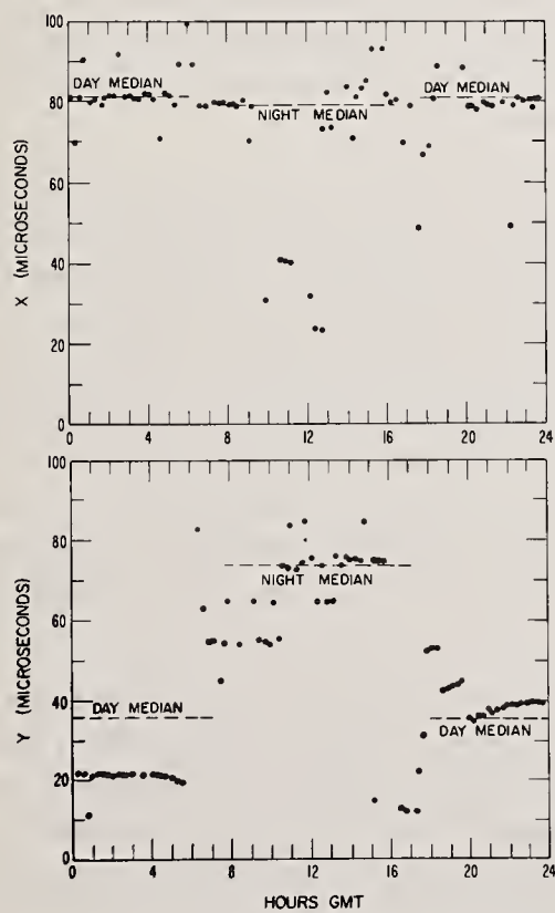
Figure 8.10. Wake Island, May 1, 1964.
