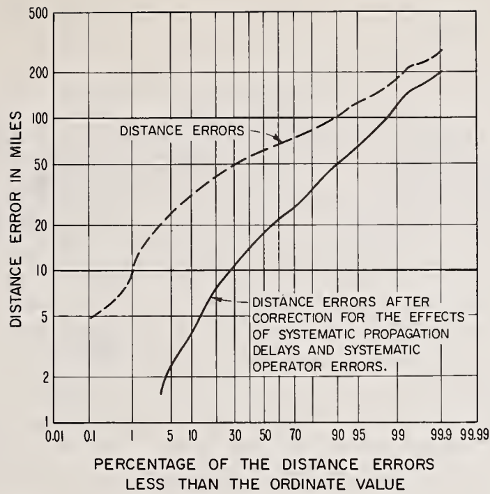
Figure 3.4. Camp Ripley data (Signal Corps).
