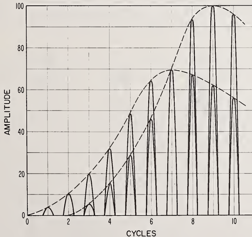
Figure 4.2. NBS pulse scheme.
