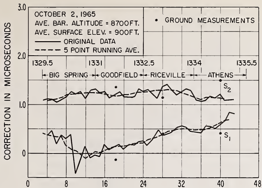
Figure 5.25. Airborne and ground measurements of systematic corrections.
