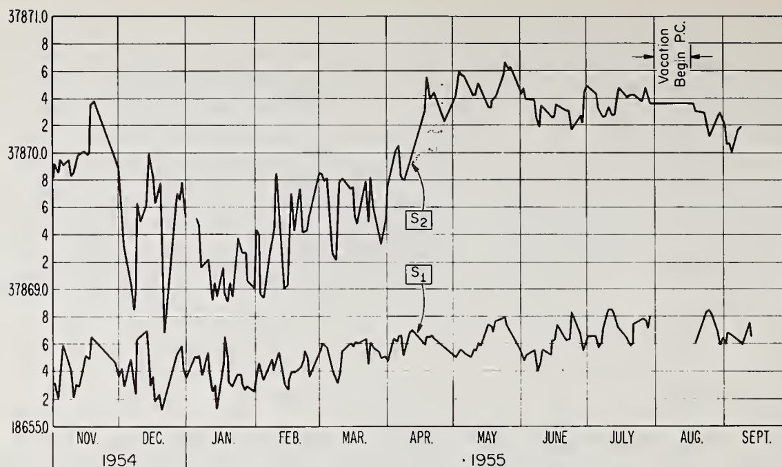
Figure 5.36. S_1 and S_2 daily average cycle readings at Clarkton, North Carolina (Rodgers).
