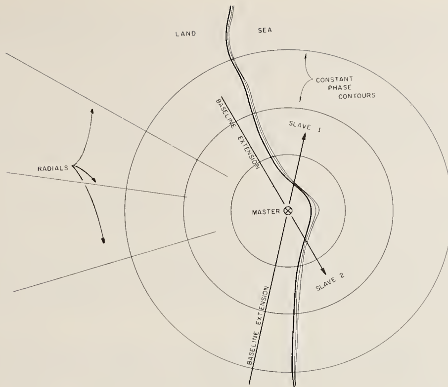
Figure 9.5. Typical master station location.
