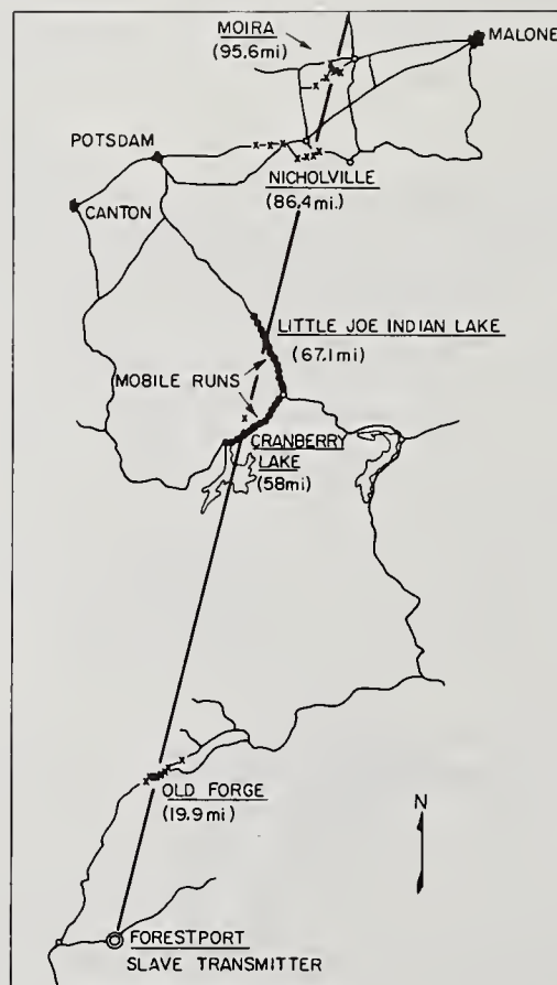
Figure 5.3. Forestport ( S_2 ) baseline extension.
