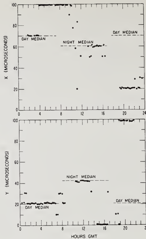
Figure 8.12. Wake Island, July 10, 1964
