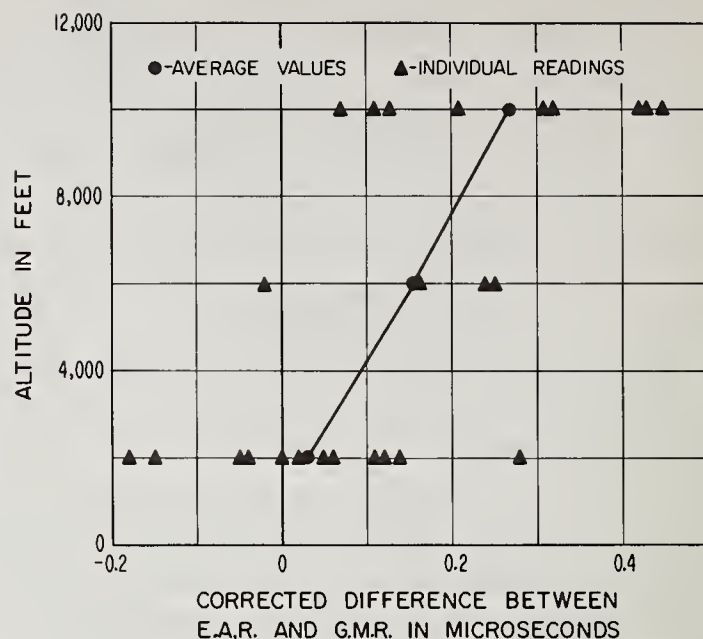
Figure 5.19. S_2 readings, Dayton, Tennessee.
