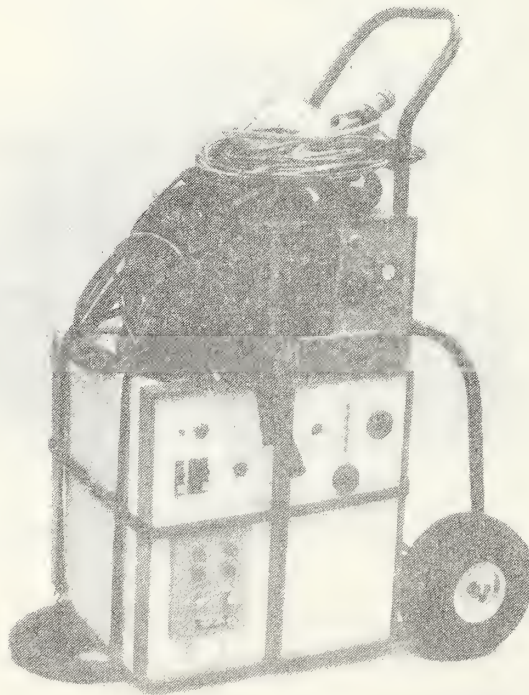
FIGURE 13. Field Circuit Breaker Tester Prepared for Travel
