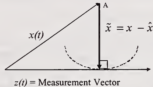
Figure 1 - Orthogonality Relationship between z(t) and \tilde{x}
