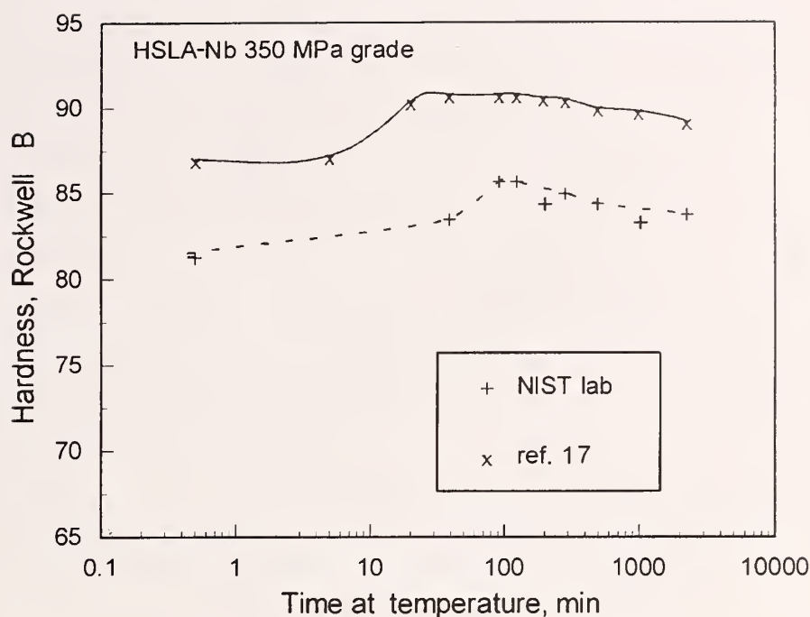
Figure 21. Aging curves for HSLA-Nb steel processing at NIST as a function of time and data from literature [17].
