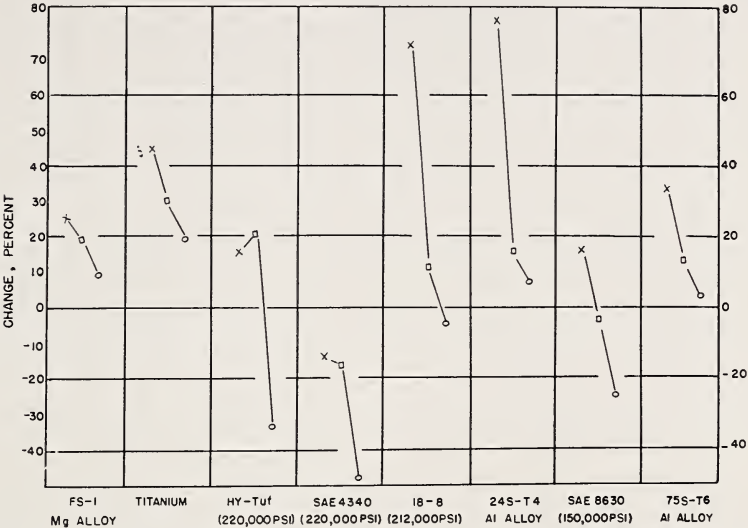
FIGURE 5.8. Effect of change in temperature from room to -320^{\circ}\text{F} on the fatigue strengths at 10^4 , 10^5 , and 10^7 cycles of notched specimens of various metals.
