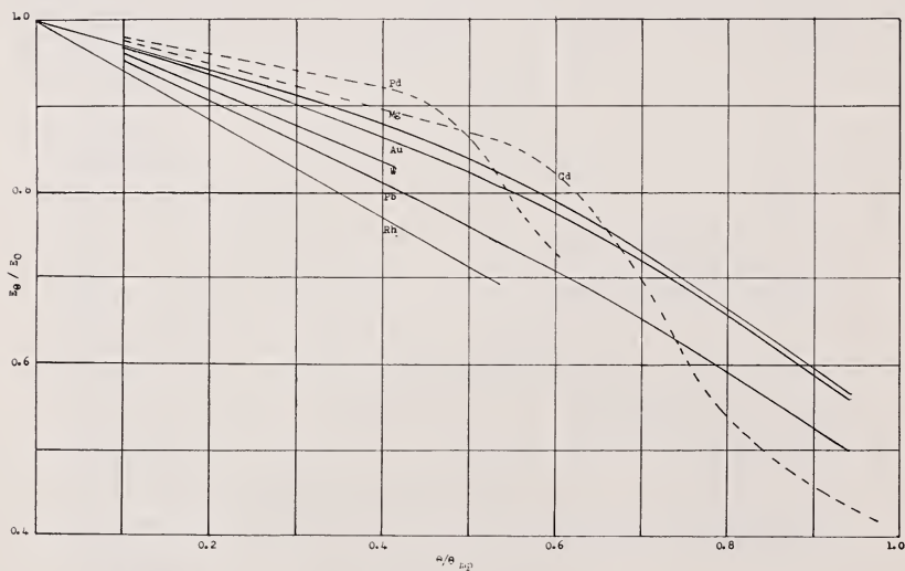
FIGURE 1.4. Fall of Young's modulus with rise of temperature. E_{\theta} is Young's modulus at \theta^{\circ}\text{K} ; E_0 is Young's modulus at 0^{\circ}\text{K} ; \theta_{mp} is melting point of metal. (Köster)
