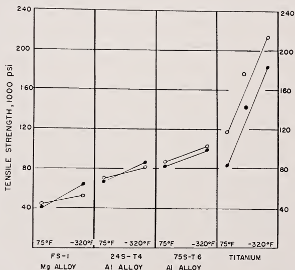
FIGURE 5.4. Tensile strength of notched and unnotched specimens of nonferrous metals at room temperature to -320^{\circ}\text{F} .
