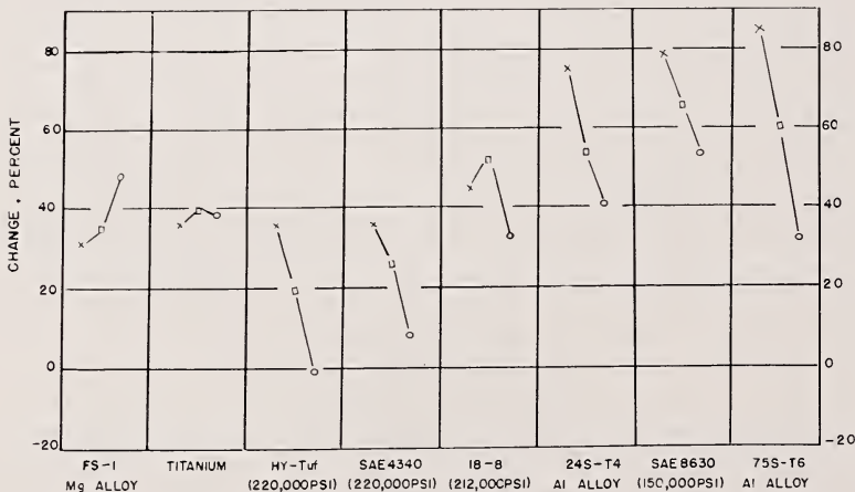
FIGURE 5.7. Effect of change in temperature from room temperature to -320^\circ\text{F} on the fatigue strengths at 10^4 , 10^6 , and 10^7 cycles of unnotched specimens of various metals.
