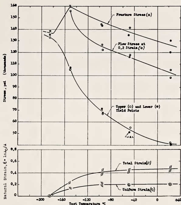
FIGURE 8.10. Effect of temperature on the tensile properties of iron-carbon alloy containing 0.49 percent of carbon.
