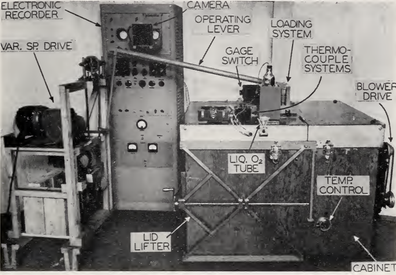
FIGURE 7.4 Load-deflection apparatus
