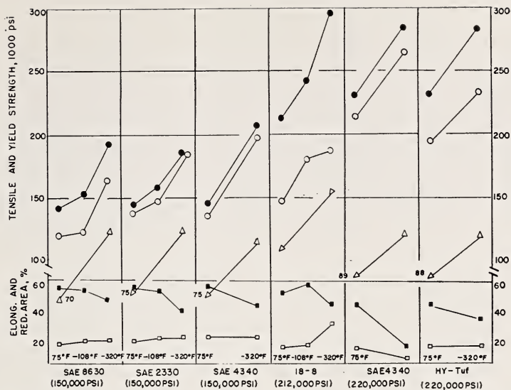
FIGURE 5.2. Tensile and fatigue properties of ferrous metals at room temperature to -320^{\circ}\text{F} .
