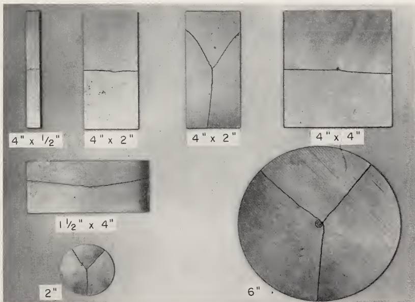
FIGURE 7.7. Typical fractures.
