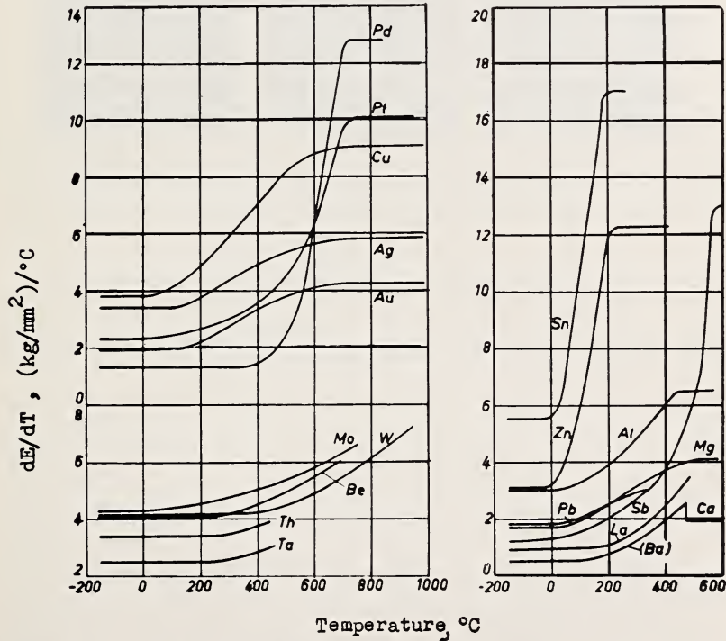
FIGURE 1.5. Temperature coefficient of elasticity plotted against temperature for various metals. (Köster)
