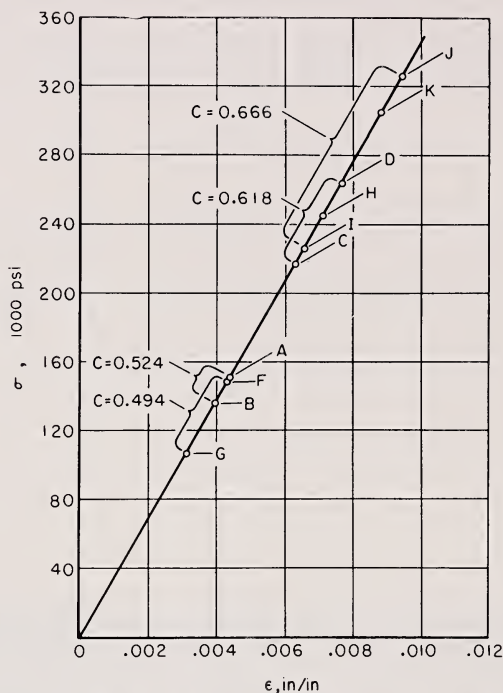
FIGURE 7.8. Effect of combined stresses on effective fracture stresses and strains.
