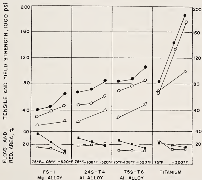
FIGURE 5.3. Tensile and fatigue properties of nonferrous metals at room temperature to -320^{\circ}\text{F} .
