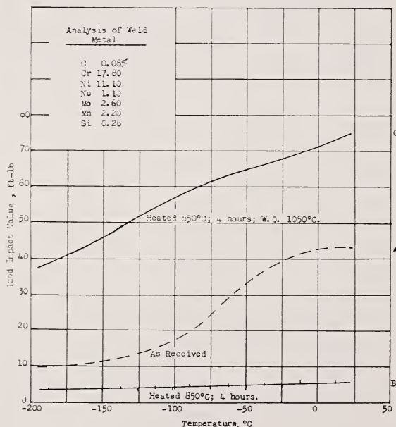
FIGURE 1.27. Izod impact tests at low temperatures on austenitic steel weld metal in various conditions.
