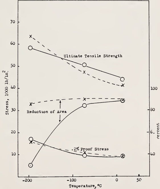
FIGURE 1.30. Tensile properties at room temperature, -73^{\circ}\text{C} , and -196^{\circ}\text{C} , of copper-zinc and copper-arsenic alloys of similar electron: atom ratio (1.165 and 1.173).
