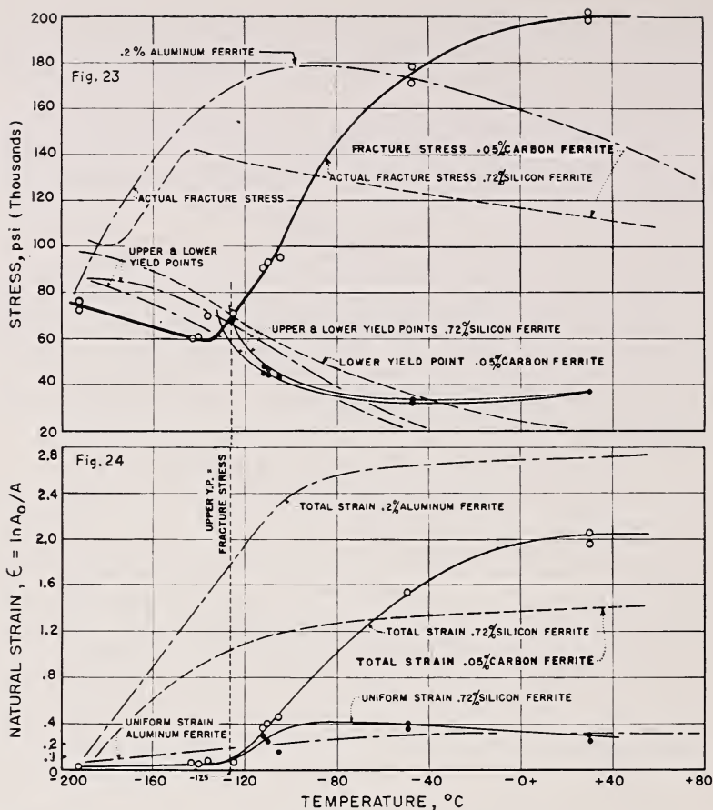
FIGURE 8.23. (Top) Effect of temperature on the actual fracture stress and yield stress of some iron alloys.
