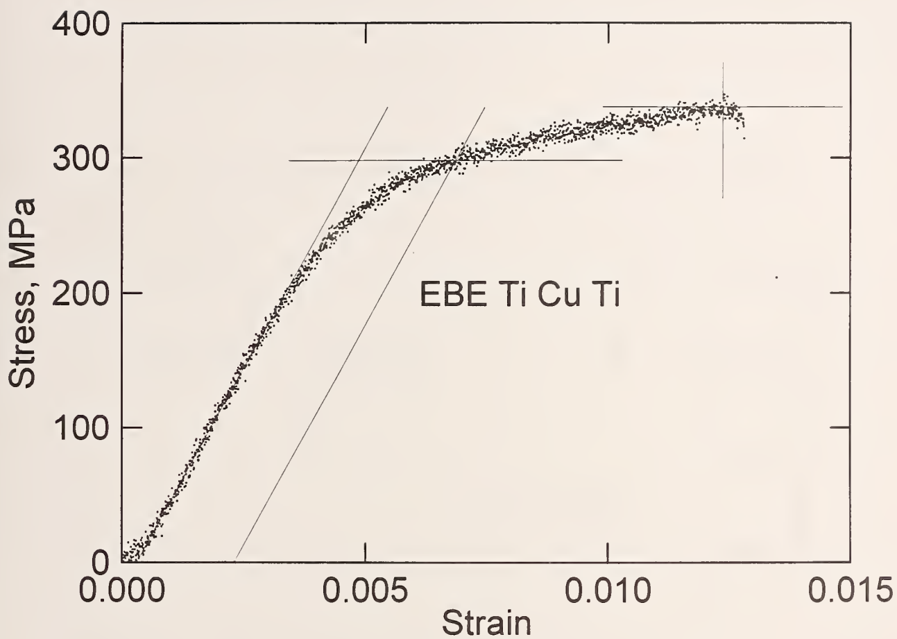
Figure 8. Stress-(engineering) strain record for a tensile test of an electron-beam-evaporated (EBE) thin film trilayer of Ti, Cu, and Ti. The total thickness is 1.2\text{ }\mu\text{m} ; the Ti layers are 0.05\text{ }\mu\text{m} thick.
