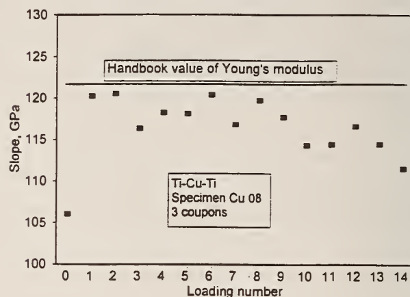
FIGURE 8. SLOPES OF STRAIGHT-LINE PORTIONS OF THE STRESS-STRAIN RECORD SHOWN IN FIGURE 7. THE X-AXIS IS LOADING NUMBER, INCLUDING INITIAL LOADING, UNLOADINGS, AND RELOADINGS.
