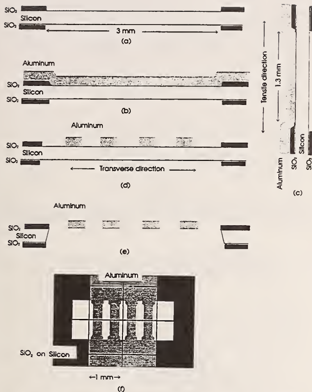
Fig. 1 Schematic diagrams showing specimen preparation sequence. Thicknesses of \text{SiO}_2 and aluminum films are exaggerated relative to the thickness of the silicon wafer. (a) Window patterned in the \text{SiO}_2 on the silicon wafer. (b) Aluminum thin film deposited over the whole wafer. (c) Cross section along the tensile direction showing the aluminum film covering the whole wafer. (d) Tensile coupons within the windows on the silicon wafer. (e) Tensile coupons suspended on the frame, after removal of the silicon within the window. (f) Plan view of specimen assembly, at a smaller scale.
