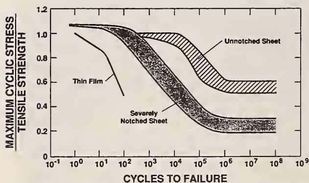
Fig. 10 Comparison of the present results for TiAlTi thin-films to results for fatigue of thin sheets of aluminum and stainless steel with stress concentrations [4]
