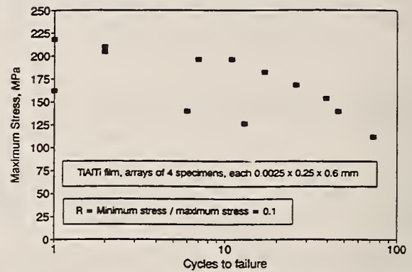
Fig. 5 S-N_f curve for TiAlTi thin-film specimen array, showing the maximum cyclic stress as a function of number of cycles to failure
