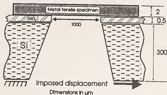
FIGURE 1. SCHEMATIC CROSS-SECTION OF THE SPECIMEN ASSEMBLY AFTER FABRICATION IS COMPLETE.
