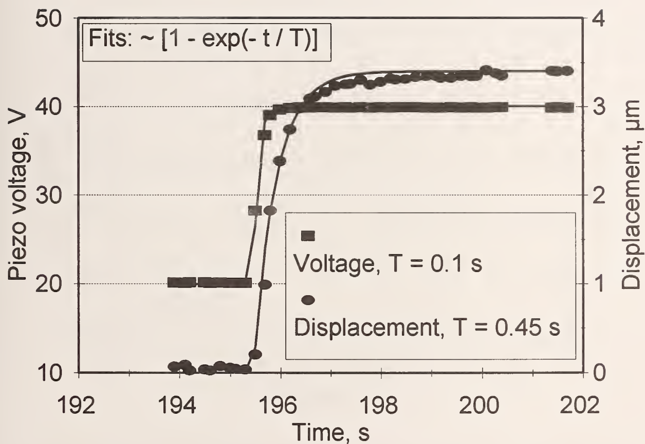
Figure 4. Plot of piezo-stack voltage and moving grip displacement against time, showing the response to a voltage step.
