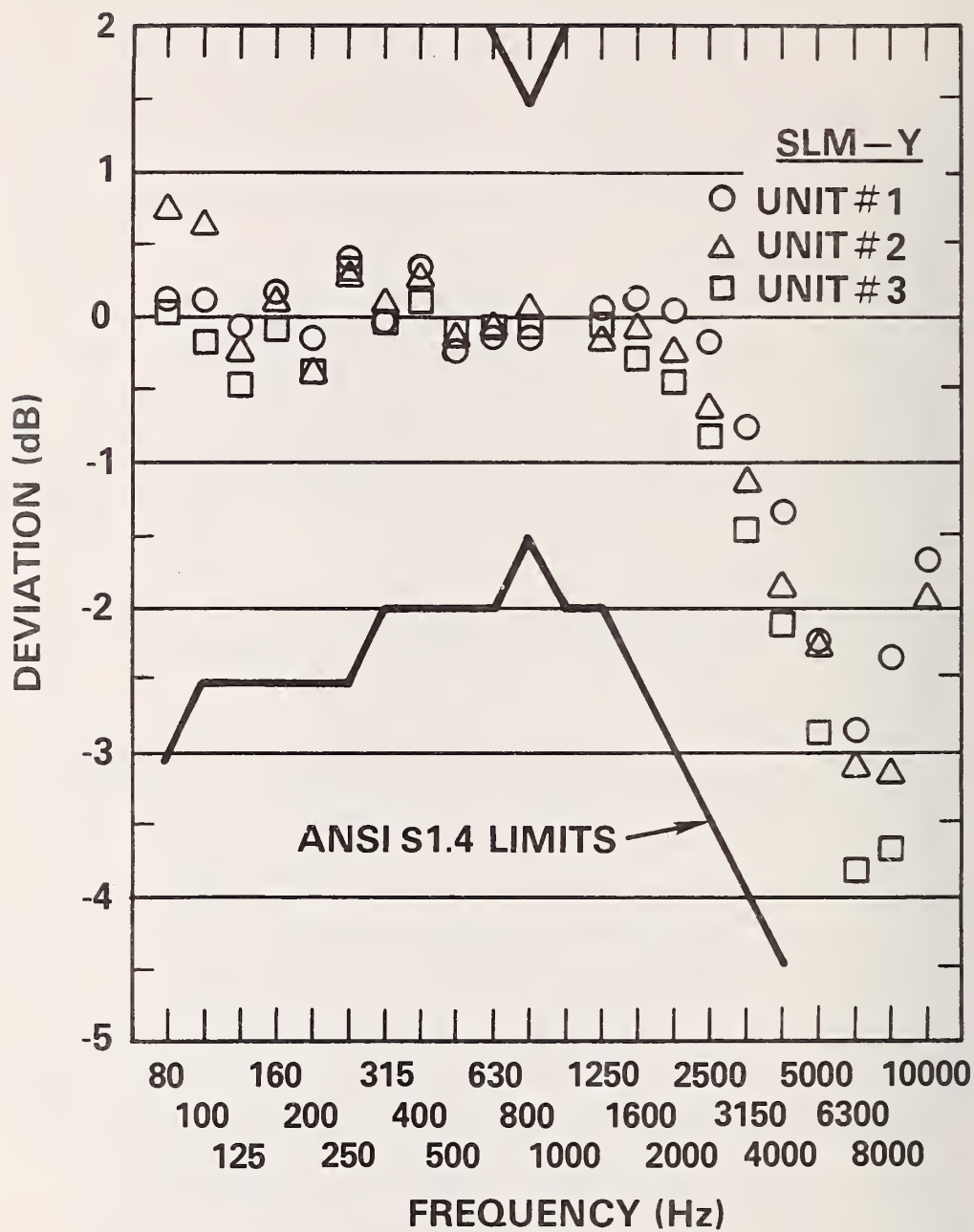
FIGURE 28. DEVIATION OF SLM-Y FROM THE IDEAL RANDOM INCIDENCE A-WEIGHTING.
