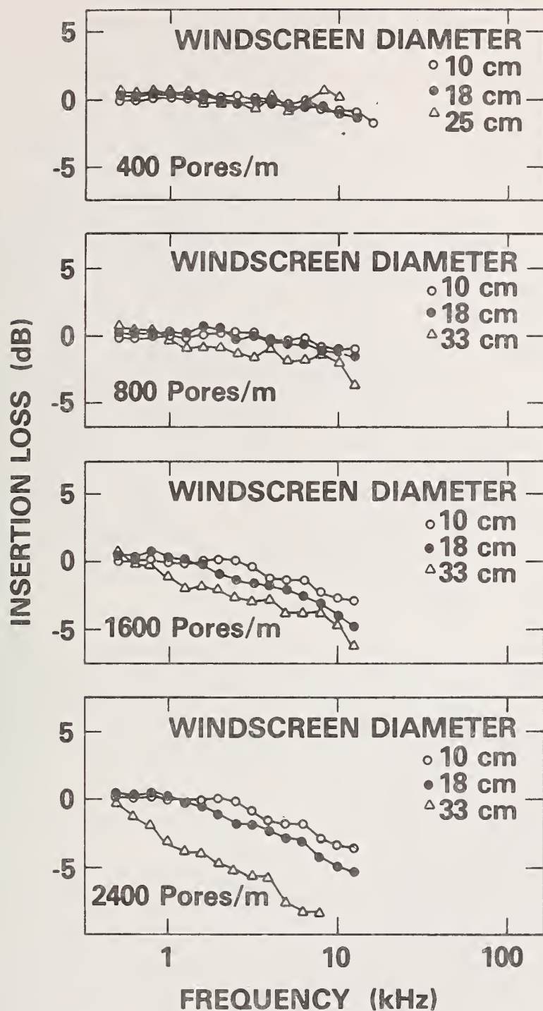
FIGURE 19. RANDOM INCIDENCE INSERTION LOSS AS A FUNCTION OF FREQUENCY FOR WINDSCREENS OF VARIOUS DIAMETERS AND LINEAR PORE DENSITY.
