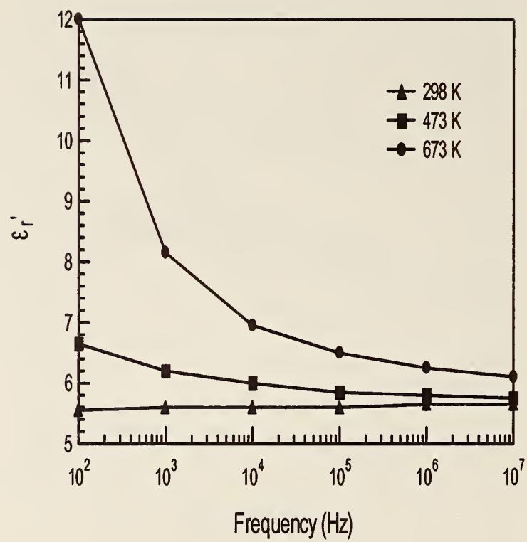
Figure 66. Measurements on \epsilon'_r for silicon nitride as a function of temperature [154] (no uncertainties assigned).
