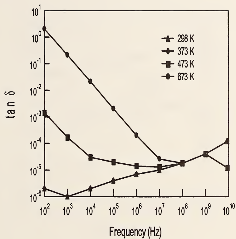
Figure 63. Measurements of the loss tangent part of \text{SiO}_2 as a function of temperature [154] (no uncertainties assigned).
