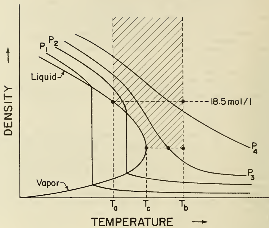
Figure 1. Density-temperature phase diagram.
