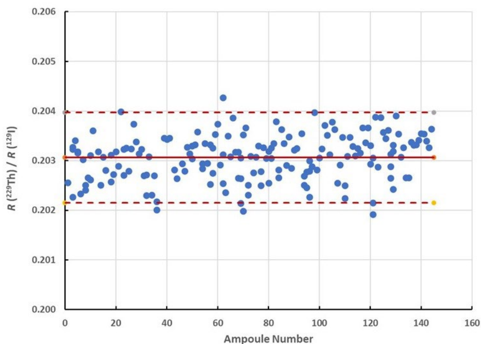
Fig. 4 The background-corrected mean counting ratio R(^{229}\text{Th}) / R(^{129}\text{I}) for the integral counting rates from 171 measurements on 137 ampoules of SRM 4328d plotted versus ampoule number (filling order) as measured in a NaI(Tl) well counter. The dashed lines show the mean \pm 2s interval, where s is the standard deviation of the distribution for the n = 171 measurements. Twenty-eight ampoules were measured in duplicate, with a 0.20 % average relative difference.
