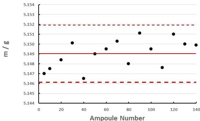
Fig.3. Dispensed masses of the SRM 4328d dispensing solution m (in units of grams) in 5 mL aliquants as a function of filling order. The solid horizontal line corresponds to the mean mass (5.1490 g) and the dashed lines represent the upper and lower limits for the \pm 2s about the mean, where s = 0.0015 g is the standard deviation for the n = 15 distribution.
