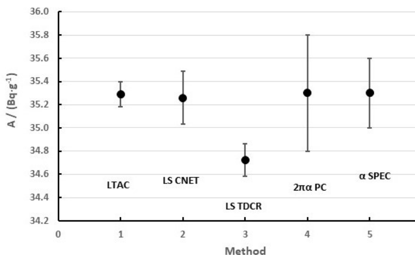
Fig. 2. Measurement results for the ^{229}\text{Th} massic activity A in units of \text{Bq}\cdot\text{g}^{-1} in SRM 4328c as reported by Fitzgerald [2010]. The uncertainty intervals for each value corresponds to a combined standard uncertainty on the measurement. The NIST certified value for SRM 4328c is based on only the anticoincidence (LTAC) value.
