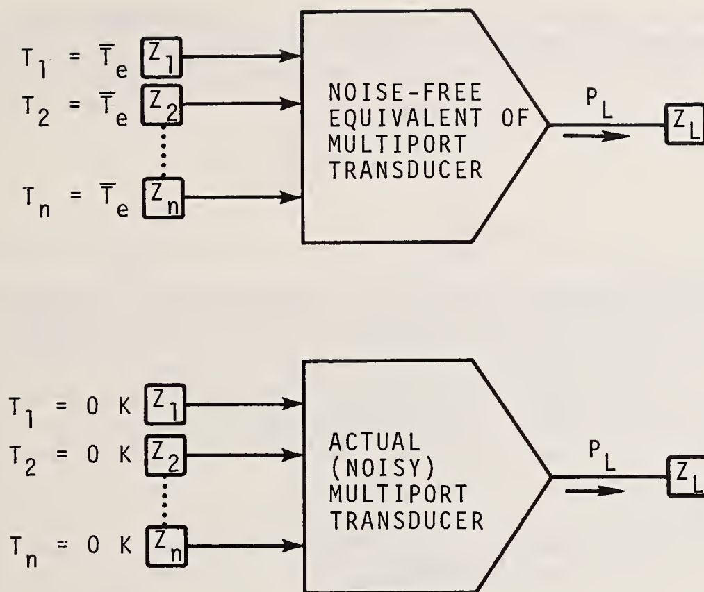
Figure 6. IEEE's Concept of \bar{T}_e .
