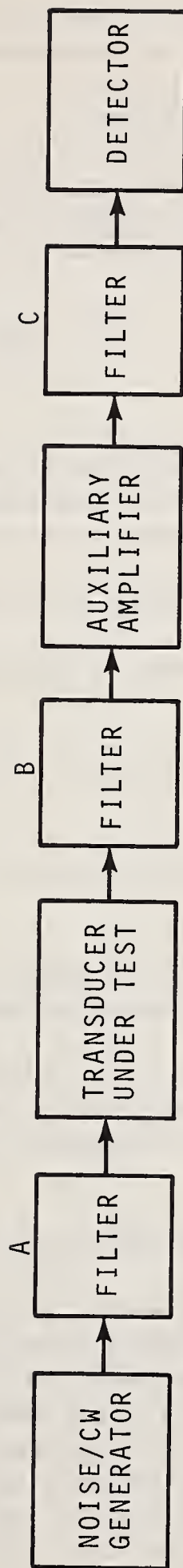
Figure 19. Possible Locations For Pre-Detection Filters.
