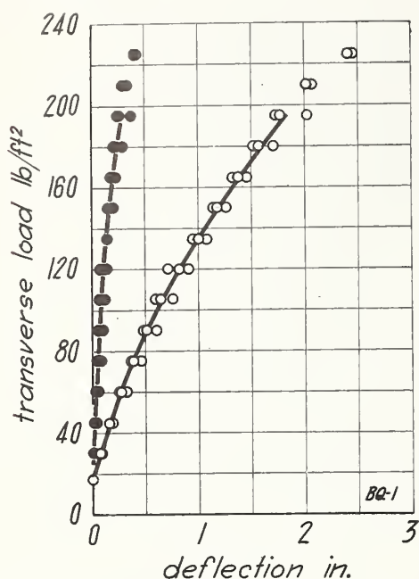
FIGURE 9.—Transverse load on wall BQ, load applied to inside face.
