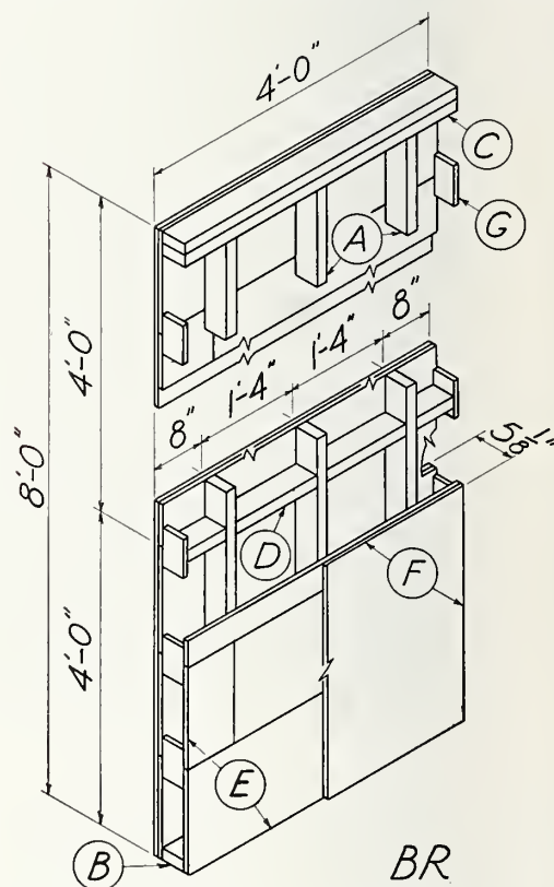
FIGURE 17.—Partition specimen BR.
