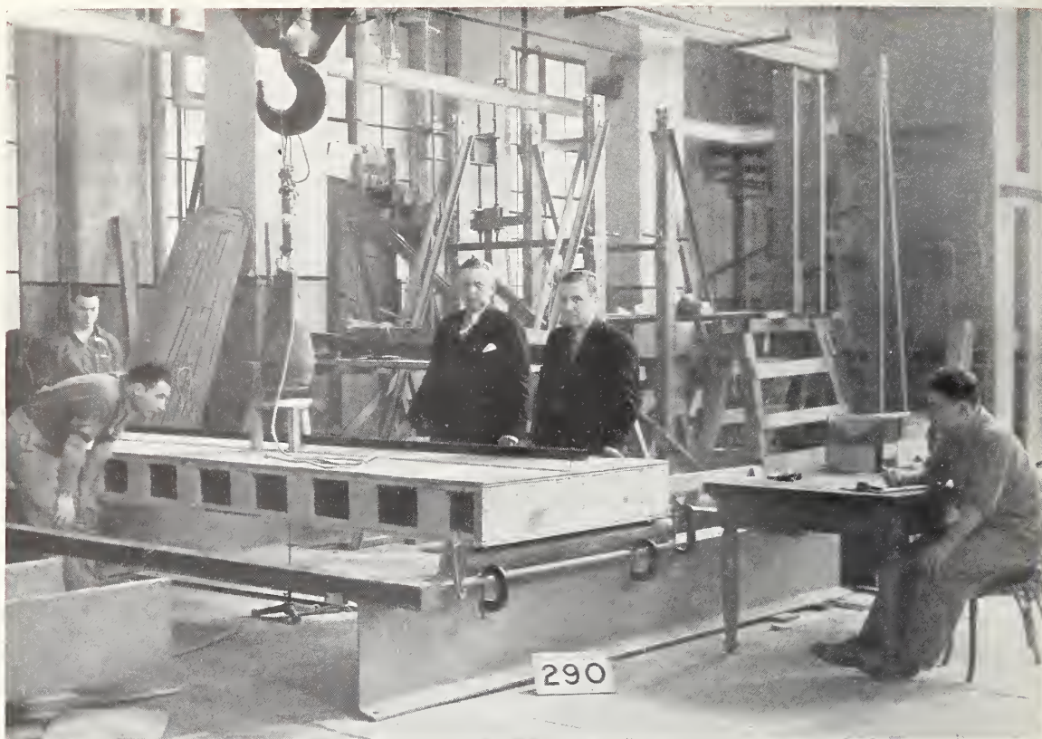
FIGURE 24.—Floor specimen BS-11 during the impact test.
