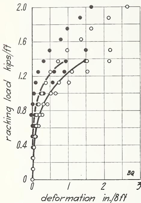
FIGURE 16.—Racking load on wall BQ.
