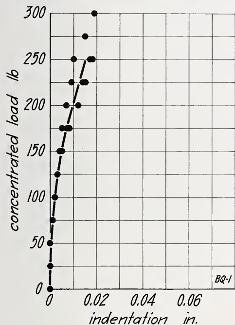
FIGURE 11.—Concentrated load on wall BQ, load applied to inside face. Load-indentation results for specimens BQ-P1, P2, and P3.
