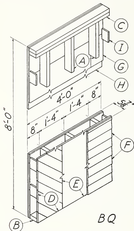
FIGURE 6.—Four-foot wall specimen BQ.
