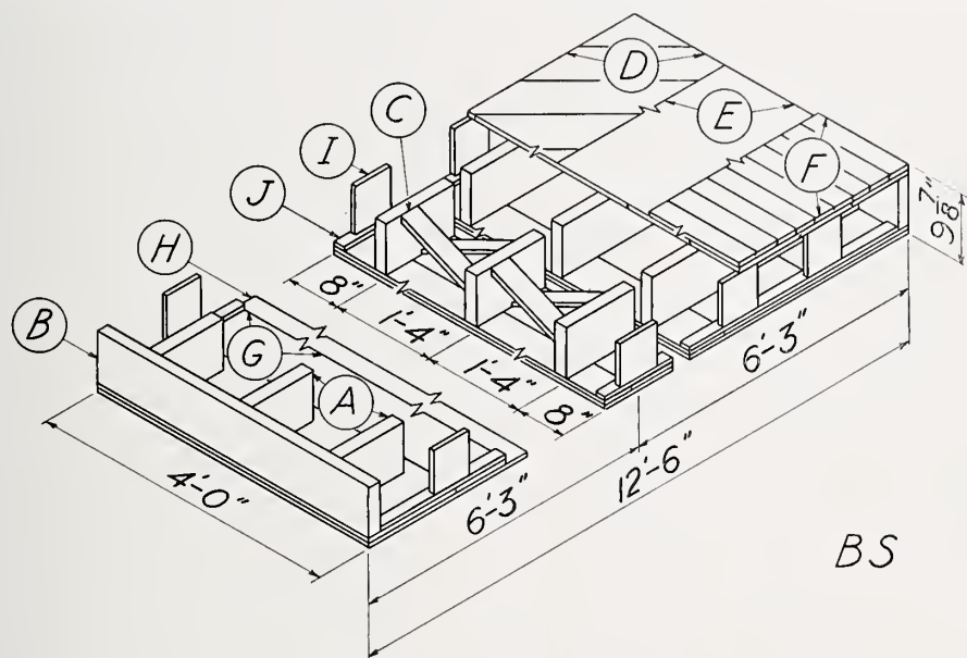
FIGURE 21.—Floor specimen BS .
