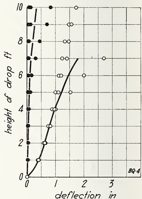
FIGURE 14.—Impact load on wall BQ, load applied to outside face.
