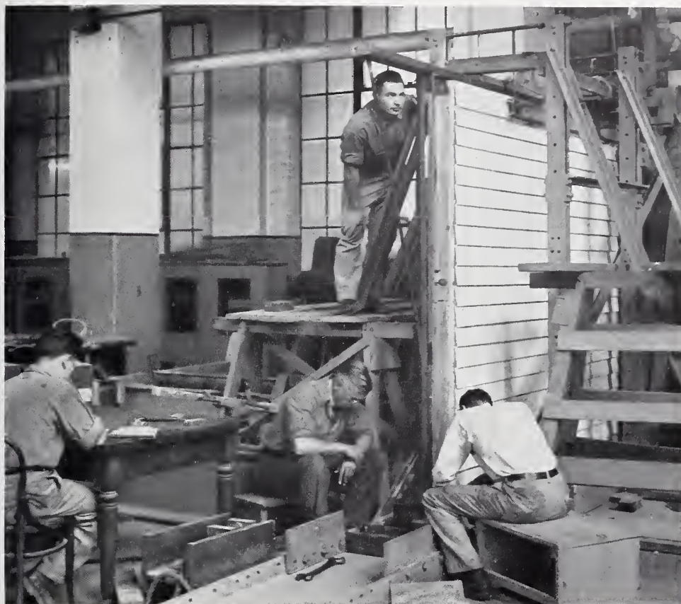
FIGURE 15.—Wall specimen BQ-R1 under racking load.
