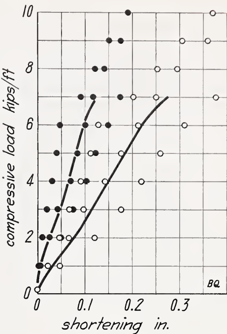
FIGURE 7.—Compressive load on wall BQ .
