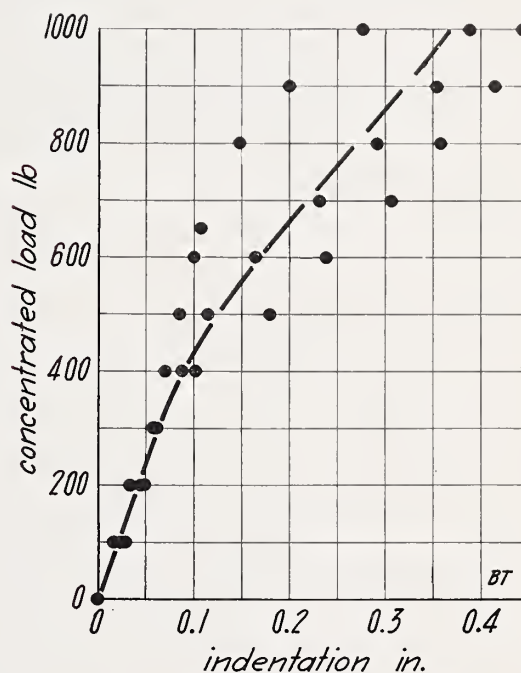
FIGURE 29.—Concentrated load on roof BT .
