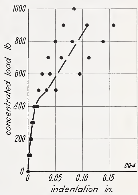
FIGURE 12.—Concentrated load on wall BQ, load applied to outside face. Load-indentation results for specimens BQ-P4, P5, and P6.
