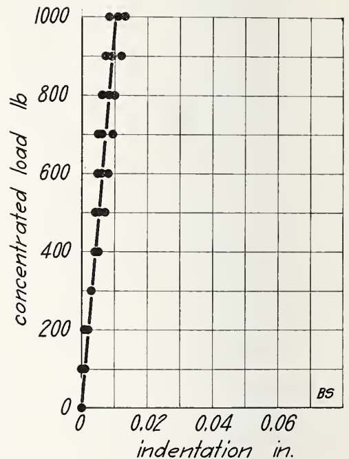
FIGURE 23.—Concentrated load on floor BS.
