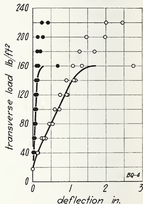
FIGURE 10.—Transverse load on wall BQ, load applied to outside face.
