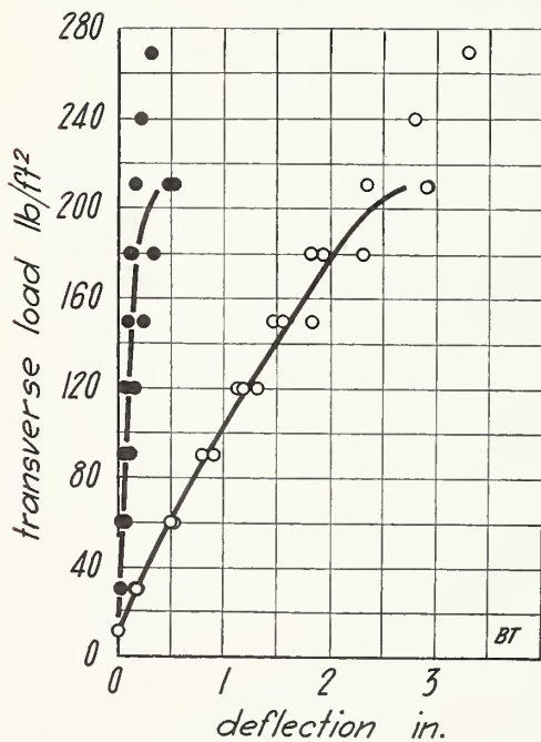
FIGURE 28.—Transverse load on roof BT .
