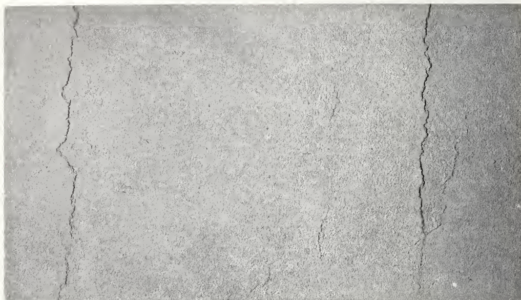
FIGURE 5.—Typical cracks in the base coat of the plaster.
