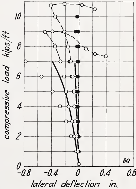
FIGURE 8.—Compressive load on wall BQ .
