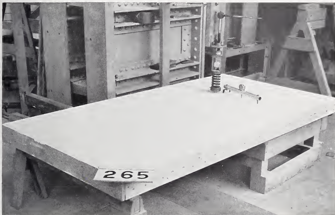
FIGURE 18.—Partition specimen BR-P2 under concentrated load.
