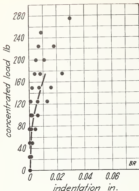
FIGURE 19.—Concentrated load on partition BR. Load-indentation result for specimens BR-P1, P2, and P3.
