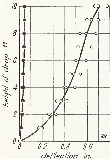
FIGURE 25.—Impact load on floor BS.
