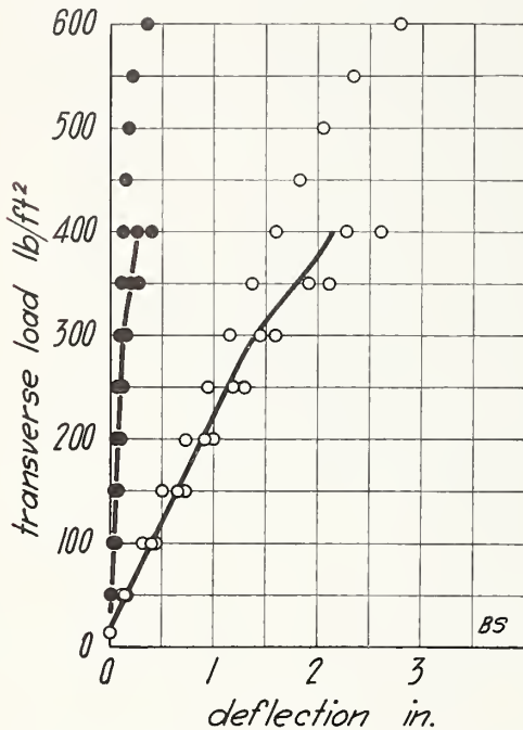
FIGURE 22.—Transverse load on floor BS.
