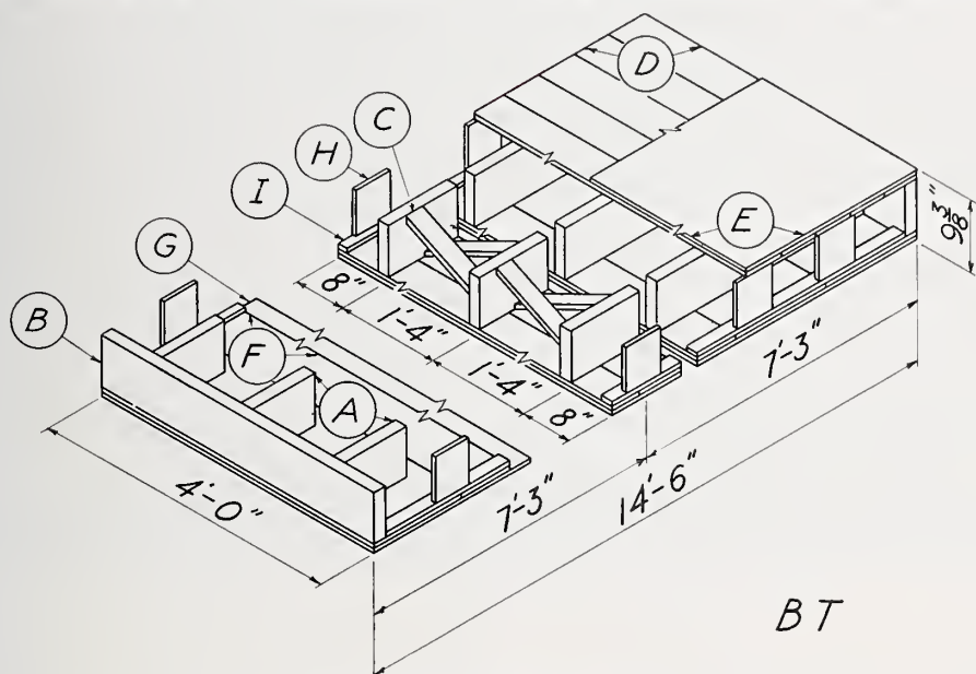
A , rafter; B , end member; C , bridging; D , sheathing; E , asphalt roofing; F , lath; G , plaster; H , spacer block; I , ground strip.
