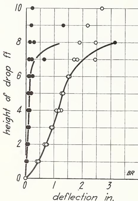
FIGURE 20.—Impact load on partition BR. Height of drop-deflection (open circles) and height of drop-set (solid circles) results for specimens BR-I1, I2, and I3 on the span 7 ft 6 in.
