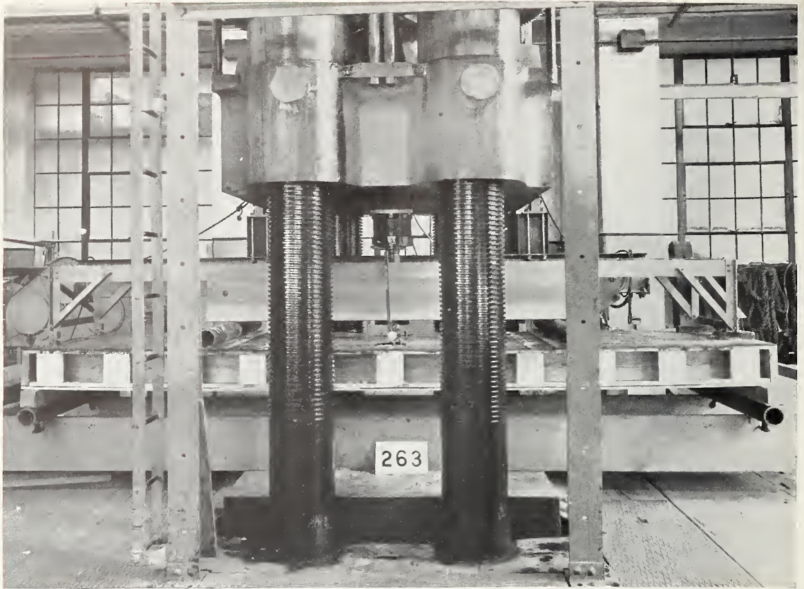
FIGURE 27.—Roof specimen BT-T2 under transverse load.
