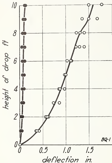
FIGURE 13.—Impact load on wall BQ, load applied to inside face.
