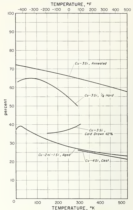
ELONGATION OF Cu-Si (Silicon Bronze) AND Cu-Ni-Si
