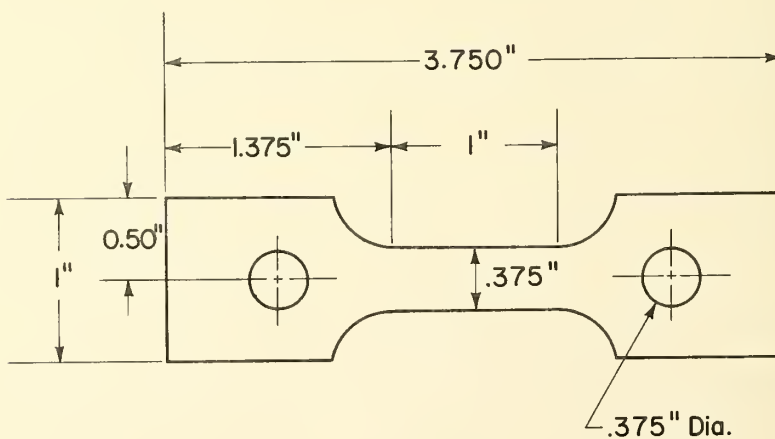
Figure 2. Electron microscopy specimen, thickness = 0.1 in.
