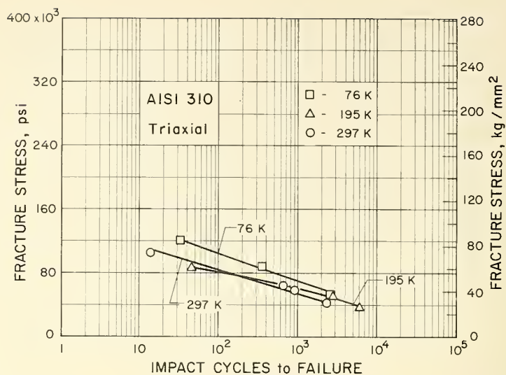
Figure 20. Fracture stress for AISI 310, triaxial.
