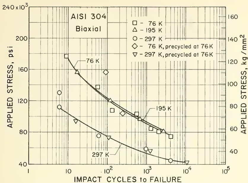
Figure 8. S-N curve for AISI 304, biaxial.
