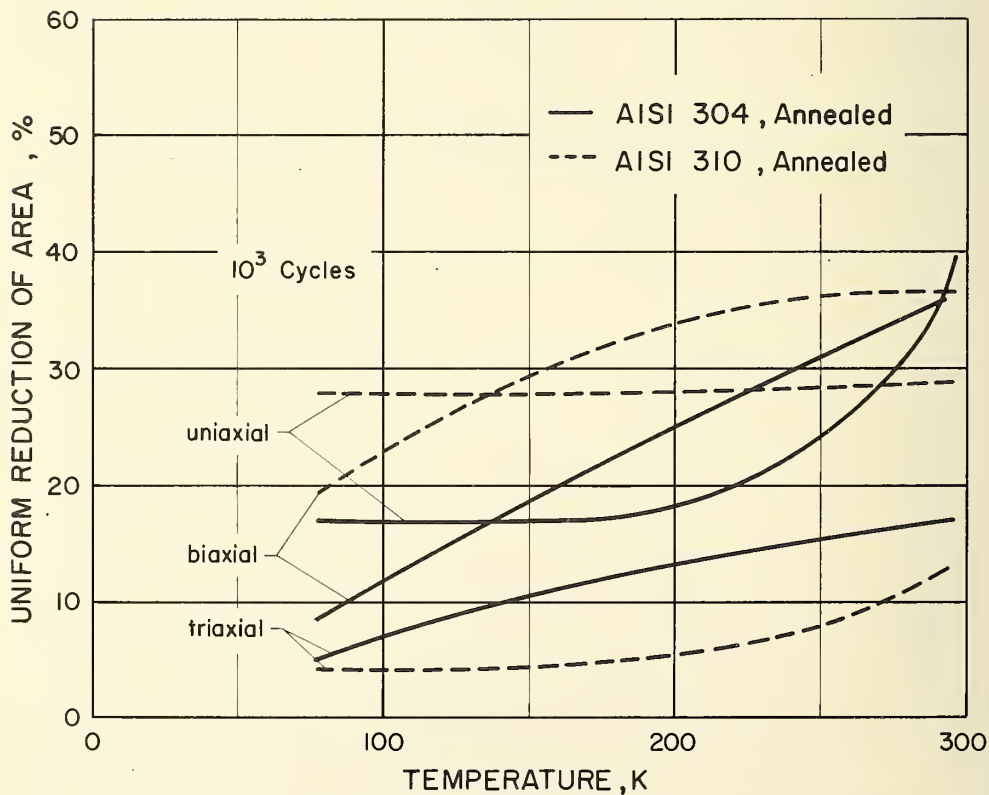
Figure 35. Uniform reduction of area for fracture at 10^3 cycles.
