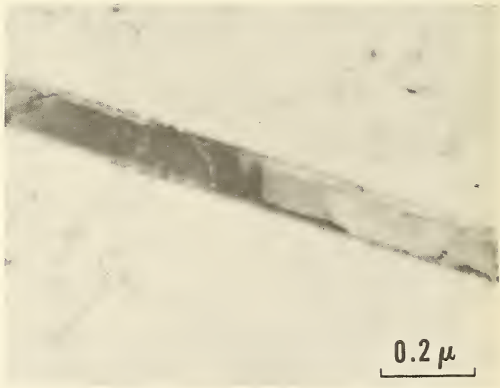
Figure 46. Deformation twin in 304 stainless steel after \sim 9\% strain. 100,000X
