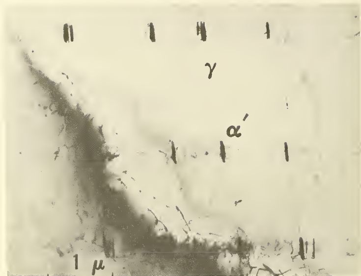
Figure 48. 304 stainless steel strained \sim 3\% at 76 K; \alpha' and \gamma present but no \epsilon . 16,000X
