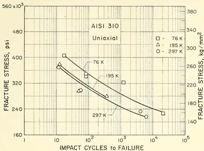
Figure 18. Fracture stress for AISI 310, uniaxial.
