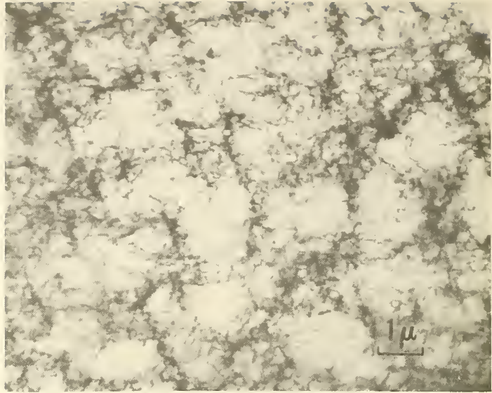
Figure 45. Cell dislocation structure of 310 stainless steel after strain of \sim 9\% . 40,000X
