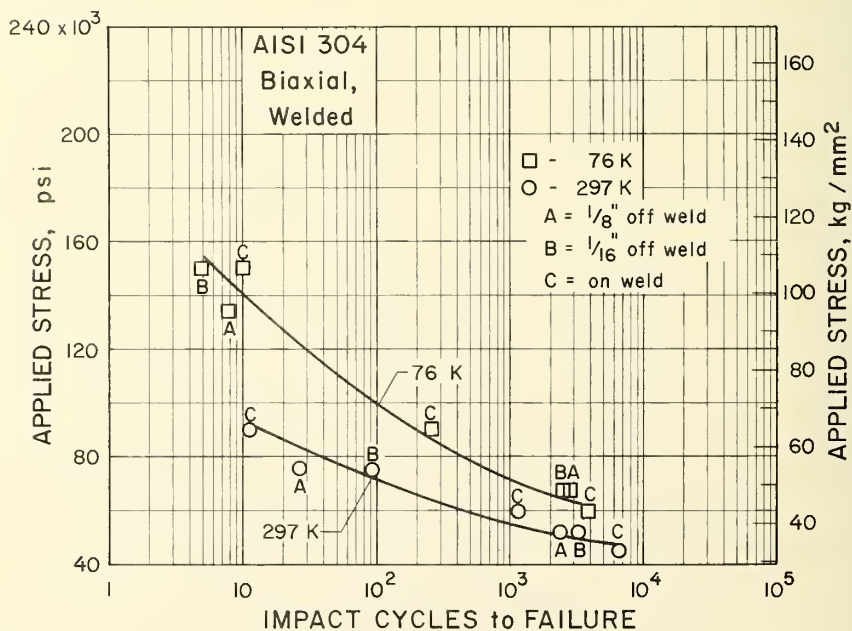
Figure 11. S-N curve for AISI 304, biaxial, welded.
