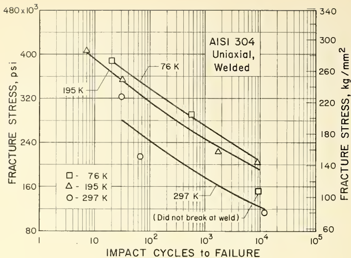
Figure 24. Fracture stress for AISI 304, uniaxial, welded.
