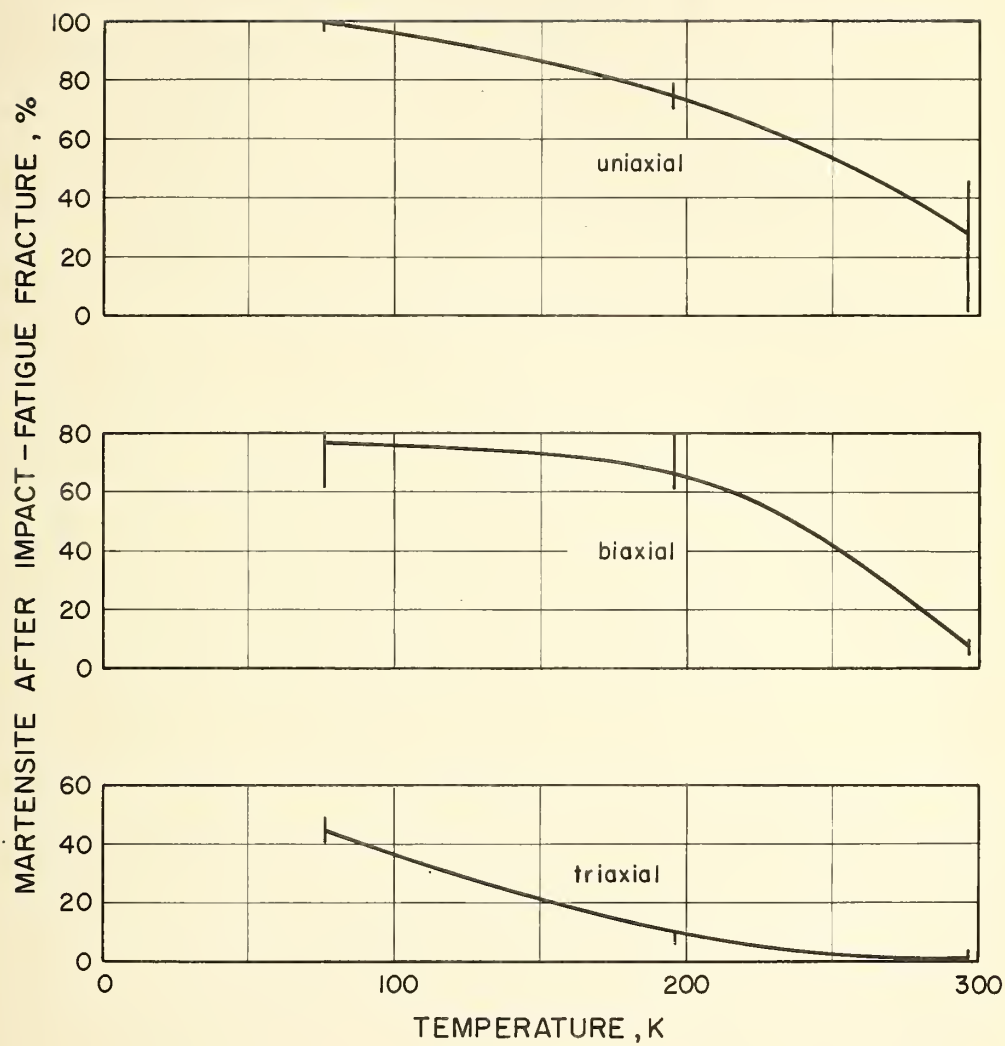
Figure 42. Temperature dependence of martensite formed after impact-fatigue fracture in AISI 304.
