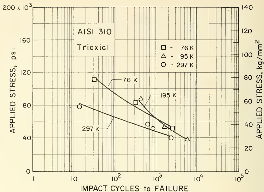
Figure 6. S-N curve for AISI 310, triaxial.
