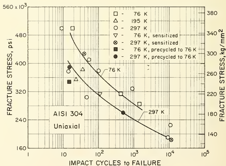
Figure 21. Fracture stress for AISI 304, uniaxial.
