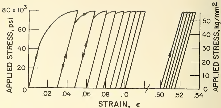
Figure 6. Typical stress-strain curve for AISI 310 stainless steel showing repeated impact cycles at 297 K ( 1 \text{ kg/mm}^2 = 9.8 \times 10^3 \text{ N/m}^2 ). Compressive stresses due to recoil of specimen upon itself are very small and not shown.
