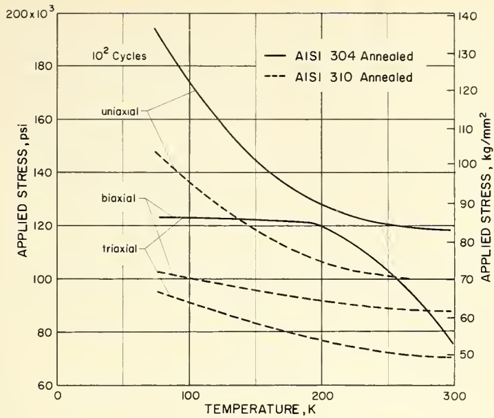
Figure 12. Fatigue life at 10^2 cycles.
