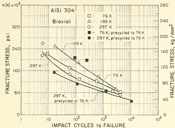
Figure 22. Fracture stress for AISI 304, biaxial.
