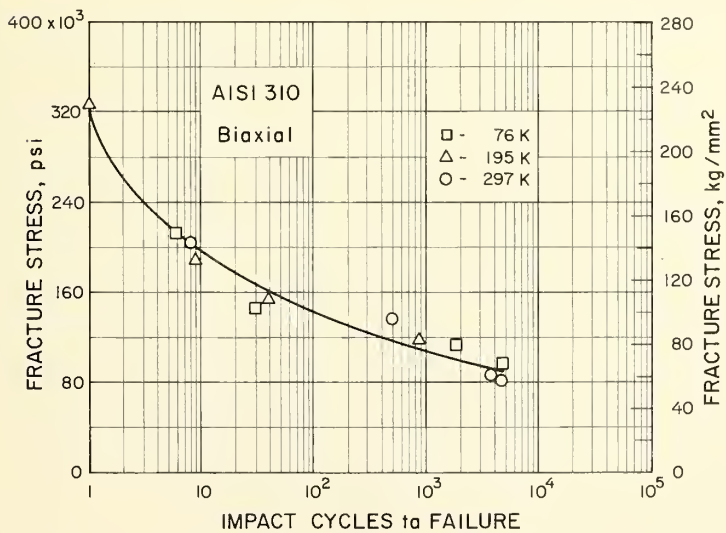
Figure 19. Fracture stress for AISI 310, biaxial.
