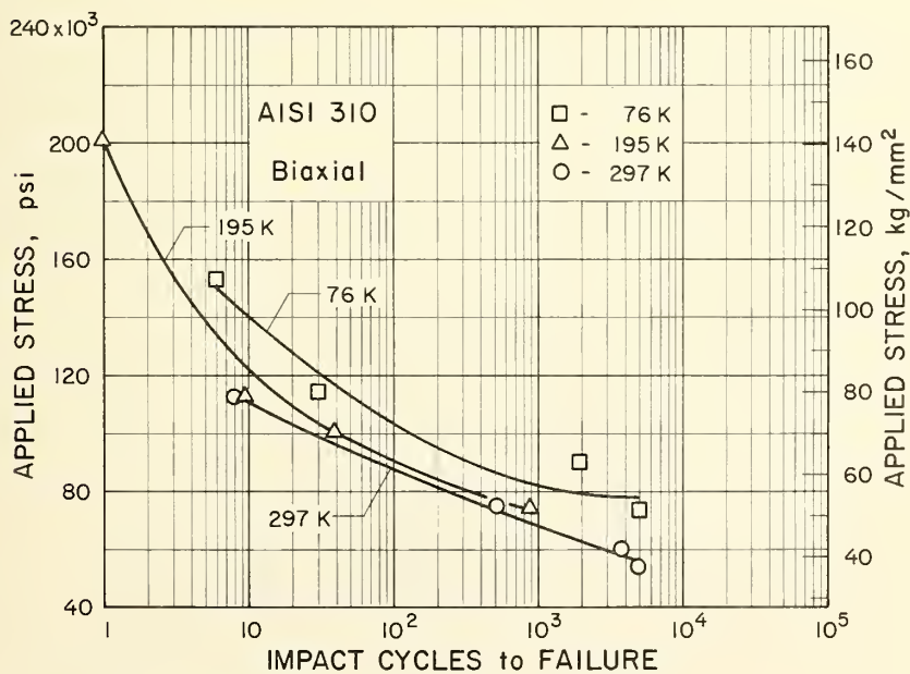
Figure 5. S-N curve for AISI 310, biaxial.
