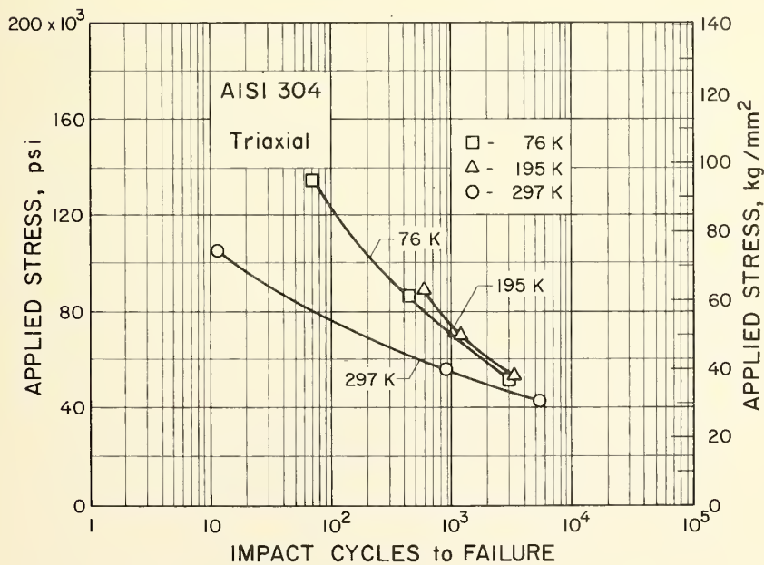
Figure 9. S-N curve for AISI 304, triaxial.
