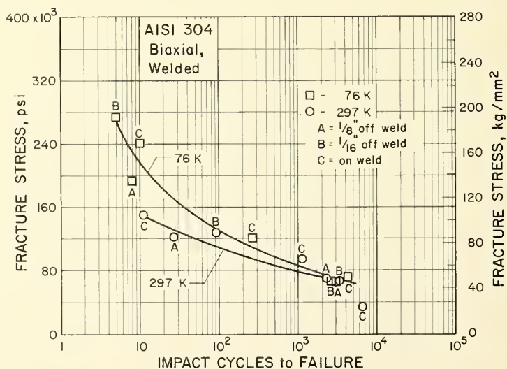
Figure 25. Fracture stress for AISI 304, biaxial, welded.
