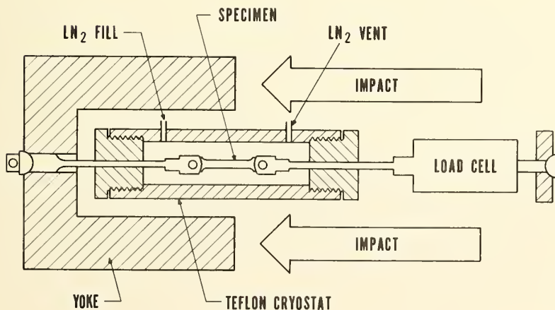
Figure 3. Specimen impact system.
