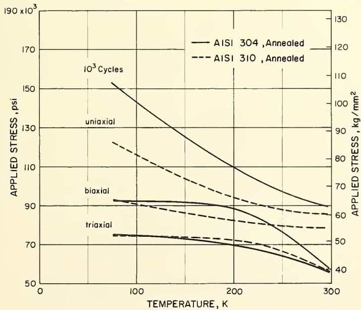
Figure 13. Fatigue life 10^3 cycles.
