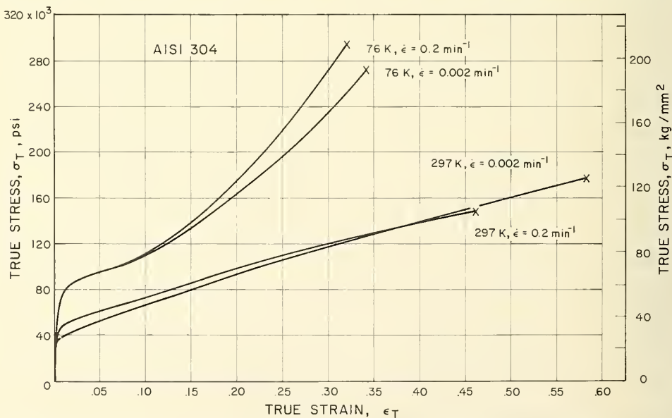
Figure 38. True stress-true strain curves for tensile tested AISI 304.
