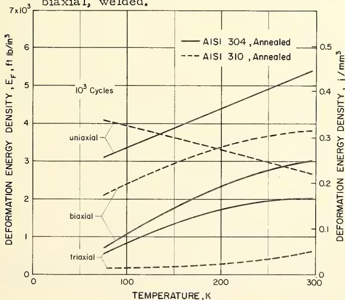
Figure 33. Summary of deformation energy density for fracture at 10^3 cycles.
