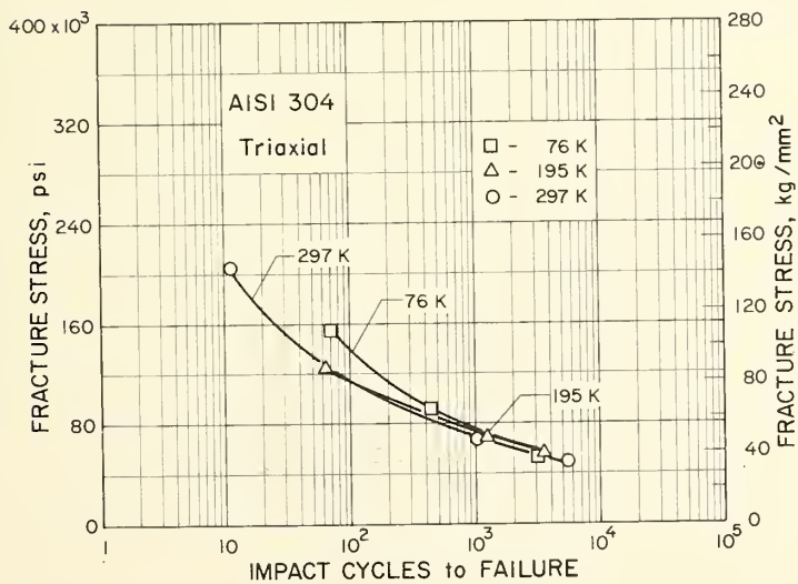
Figure 23. Fracture stress for AISI 304, triaxial.
