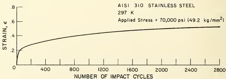
Figure 5. Specimen strain during impact-fatigue life.
