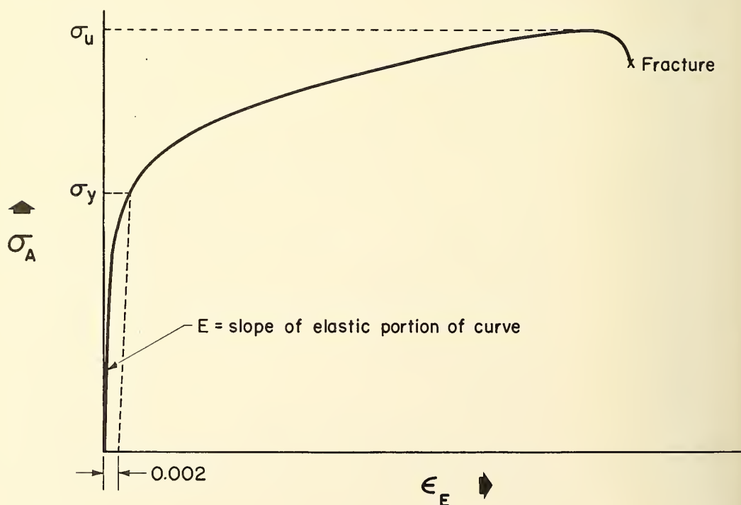
Figure 3. Determination of E , \sigma_u , and \sigma_y from a stress-strain curve.
