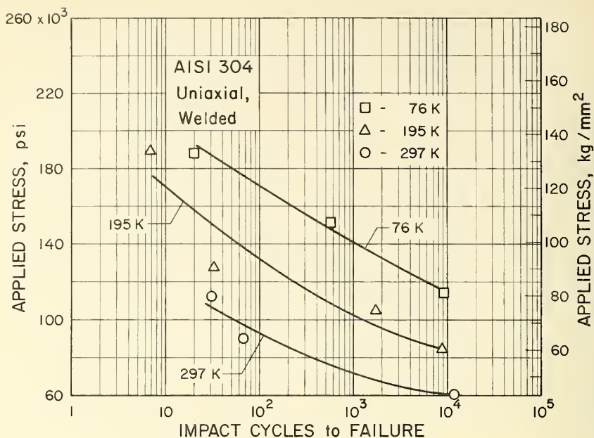
Figure 10. S-N curve for AISI 304, uniaxial, welded.
