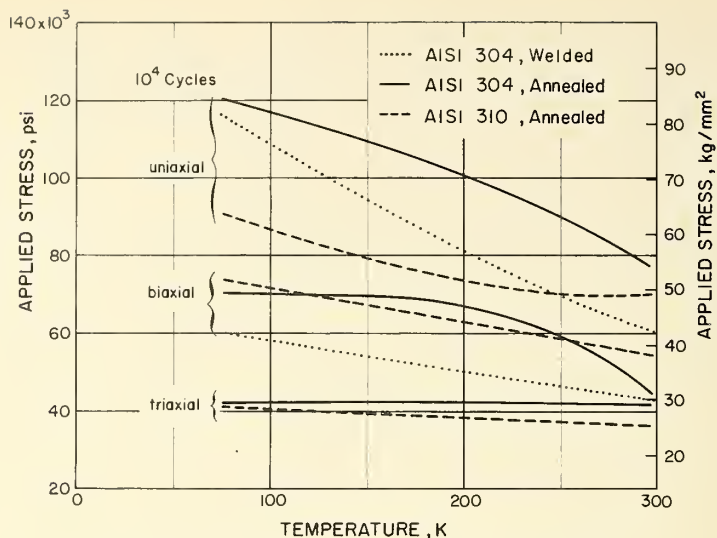
Figure 14. Fatigue life at 10^4 cycles.
