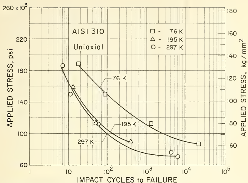
Figure 4. S-N curve for AISI 310, uniaxial.
