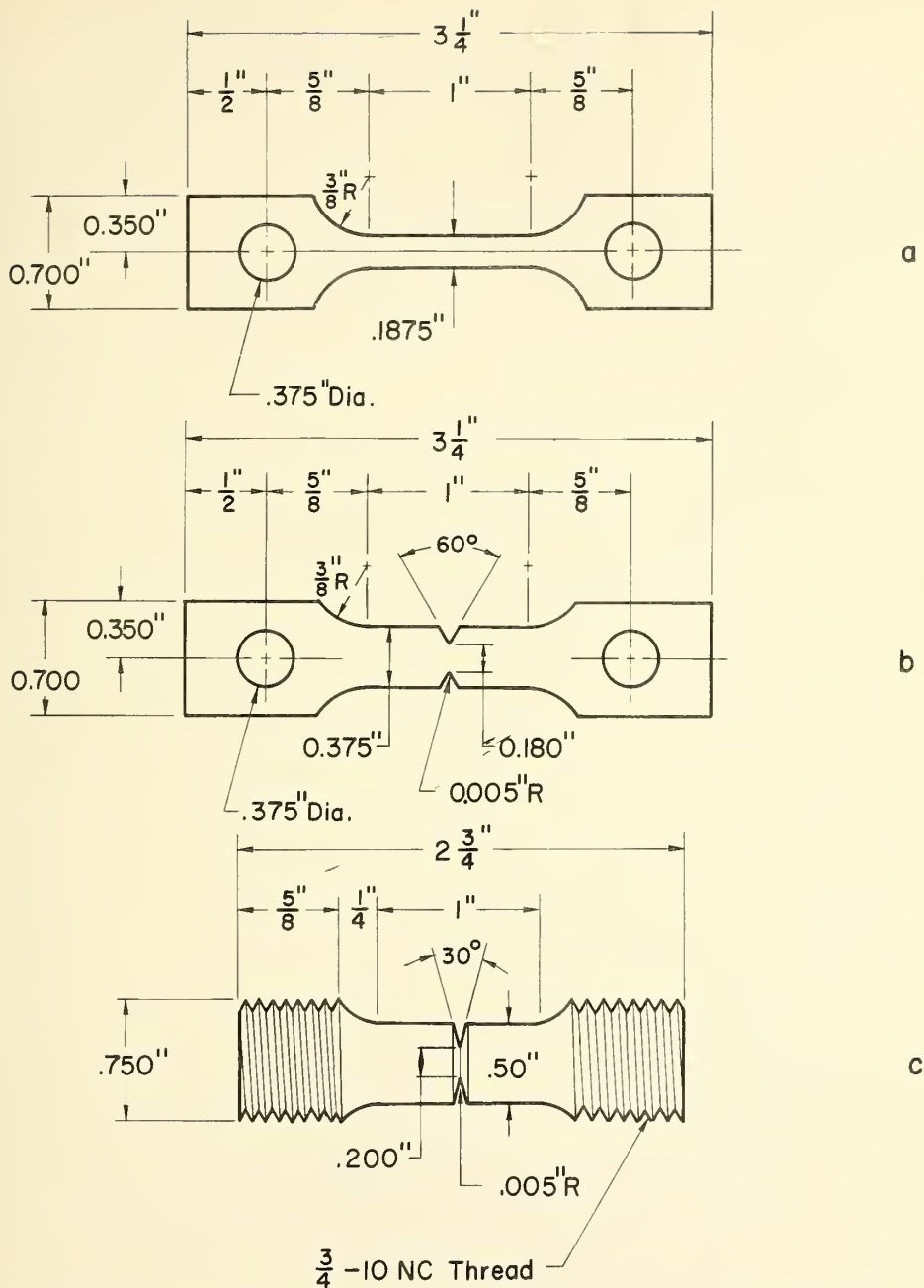
Figure 1. Sample geometries for tensile and impact tests: a. Uniaxial, thickness = 0.1 in; b. Biaxial, thickness = 0.1 in; c. Triaxial.
