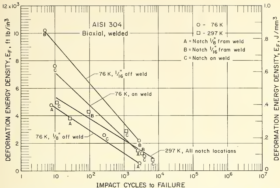
Figure 32. Deformation energy density for fracture of AISI 304, biaxial, welded.
