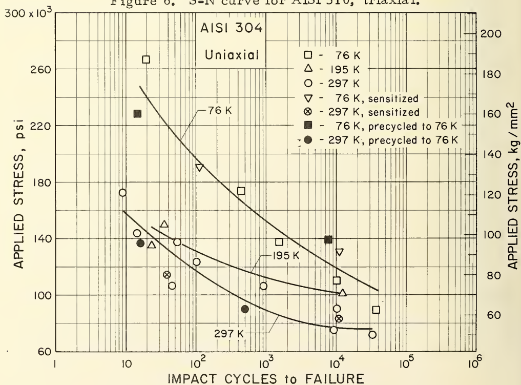
Figure 7. S-N curve for AISI 304, uniaxial.
