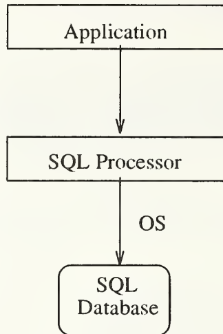
Figure 1: Standalone model.
