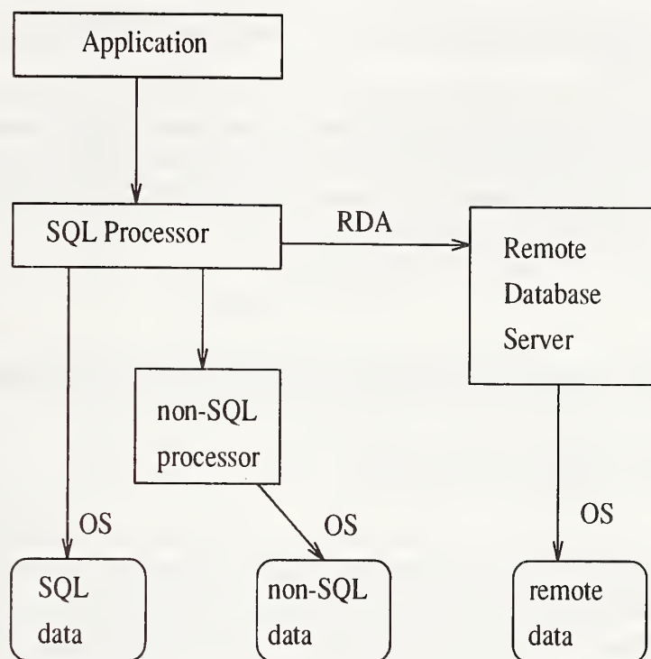
Figure 2: Client/server model.
