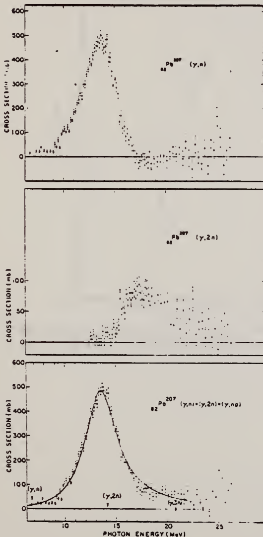
FIG. 2. Top figure shows data points for \sigma[(\gamma,n) + (\gamma,np)] for Pb 207 , obtained from single-neutron counting data. Center figure shows data for \sigma(\gamma,2n) obtained from double-neutron counting data. Data points for the compound nucleus formation cross section of Pb 207 , i.e., \sigma[(\gamma,n) + (\gamma,np)] + \sigma(\gamma,2n) are shown in bottom figure. Solid curve is a plot of a Lorentz line having the parameters given in Table II. The data are uncertain below 8 MeV owing to low beam intensities encountered.
