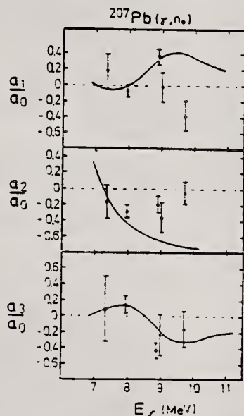
Fig. 8. Angular distribution coefficients a_0, a_1 for the (\gamma, n) transitions to the ^{206}\text{Pb} ground state. The solid curves are calculated using the DSD model.
