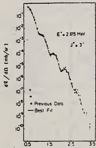
FIG. 1. Experimental cross sections recalculated to an incident energy of 502 MeV. The solid line represents the best fit obtained with the Fourier-Bessel analysis. Solid circles, new data taken at Saclay; crosses, new data taken at M.I.T.; open circles, previous data (Refs. 3-5).
