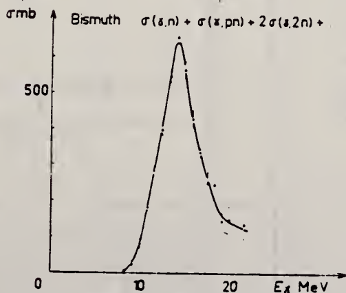
Fig. 12. Section efficace \sigma = \sigma(\gamma, n) + \sigma(\gamma, np) + 2\sigma(\gamma, 2n) + \dots pour le bismuth.
