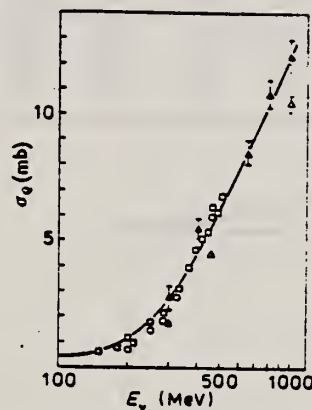
Fig. 3. - The Bi photofission cross-section per equivalent quantum, plotted against E_\gamma . The data from BERNARDINI et al. (*) (circles), from JUNGERMAN et al. (□) (squares) and from DE CARVALHO et al. (△) (open triangles) are shown, together with those obtained in the present work (full triangles).
