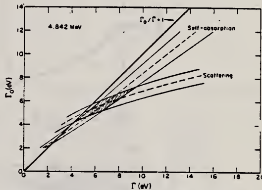
FIG. 7. Combined results of the self-absorption and scattering measurements for the 4.842 MeV level in 208 Pb. The dashed curves indicate combinations of \Gamma_0 and \Gamma which reproduce the experimental results; the solid curves represent the error band for each case. The shaded region contains the values of \Gamma_0 and \Gamma consistent with both experiments, and with the condition \Gamma_0/\Gamma \leq 1 .
