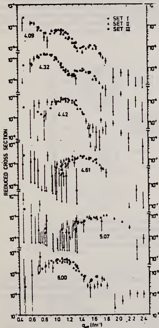
Fig. 3. Reduced cross section (= measured cross section divided by the Mott cross section, often called form factor) for the levels at the indicated energies. Sets I and III are explained in the text.
