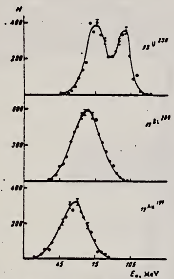
FIG. 2. Single-ended energy spectra of fragments from photofission of {}_{92}\text{U}^{238} , {}_{83}\text{Bi}^{209} , and {}_{79}\text{Au}^{197} .
