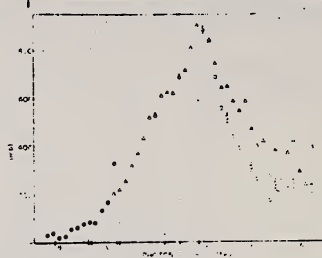
Fig. 7. The neutron production cross section for Pb-206. The points represent the \sigma_0 values in the curve for neutron multiplicity. Points were obtained from a 1 MeV \beta - \gamma source. (The neutron yield curve except near threshold limits, and below 1.0 MeV, is the same as used.) The points represented by the open circles have been corrected for the neutron multiplicity. The arrows beneath the axis of abscissas indicate the energies of the important dipole transitions calculated by Balashov, et al. (1). The heights of the vertical lines are proportional to the calculated strengths of the transitions.
