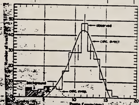
FIG. 2. The histogram gives the energy distribution of the photoprotons from lead 208 exposed to 21-Mev bremsstrahlung. The smooth curve is the distribution calculated for the direct process and normalized to the observed protons. The dashed curve is the calculated distribution for the evaporation process fitted to indicate the maximum possible evaporation yield. The shaded groups are background.
