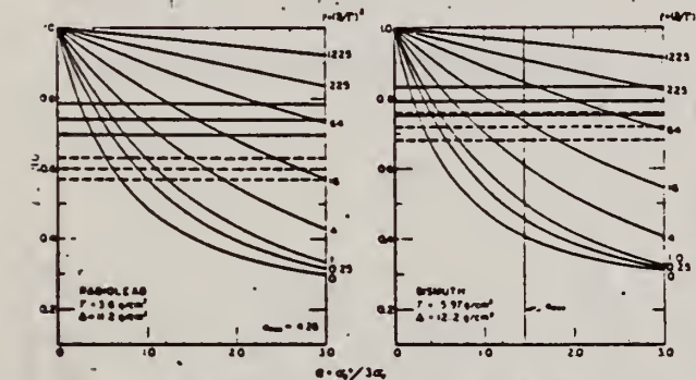
Fig. 2. Self-absorption attenuation curves for radium and bismuth. The rate R(N)/I_0 as defined in the text (eq. (4)) has been evaluated as a function of the peak absorption cross section \sigma_p for the target and absorber (thicknesses used in the experiments). The horizontal lines represent the measured attenuations and their uncertainties for the experiments performed at room temperature (solid lines) and liquid nitrogen temperature (dashed lines). The quantity \sigma_{max} is the maximum possible value of the average peak absorption cross section at 6 MeV in units of \sigma_p (using the electronic absorption cross sections). The maximum value assumes elastic dipole scattering and represents an average over all possible angles for the incident neutrons.
