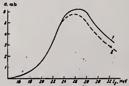
FIG. 2. Cross section of photoneuclear reactions in lead: 1 - cross section calculated from the total yield curve, 2 - cross section for the (γ, p) reaction.
