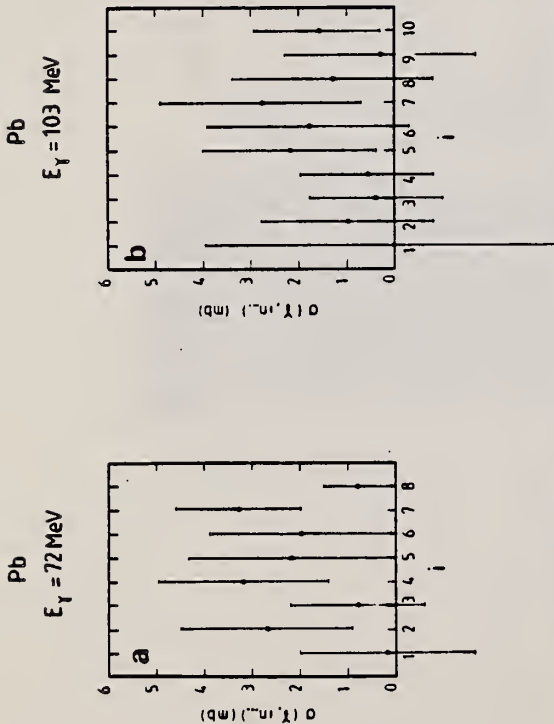
Fig. 1. (a) Partial photoneutron cross sections \sigma(\gamma, in \dots) for Pb at a fixed "monochromatic" photon energy of E_\gamma = 72 MeV, plotted against the measured photoneutron multiplicity i . Data points were obtained from ref. 1). (b) Partial photoneutron cross sections \sigma(\gamma, in \dots) for Pb at a fixed "monochromatic" photon energy of E_\gamma = 103 MeV, plotted against the measured photoneutron multiplicity i . Data points were obtained from ref. 1).
