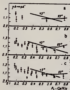
FIG. 2. Dependence of the exponent n in the A^0 dependence of the cross section for the reaction \gamma A \rightarrow pA' as a function of proton transverse momentum: a — E_0 = 2.0 GeV, b — E_0 = 3.0 GeV, c — E_0 = 4.5 GeV. The points for a and b : \Delta — \phi_p = 60^\circ , \circ — 90^\circ , \square — 150^\circ ; for c : \Delta — \phi_p = 46^\circ , \circ — 86^\circ , \square — 136^\circ . The curves show the dependence of n on p_\perp for the reaction A(p, p')A' taken from Ref. 9.
