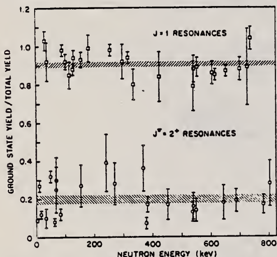
FIG. 3. Yield ratios showing clear separation into two groups leading to J^\pi assignments for the resonances. Ratios with error bars greater than 25% and 50% for J = 1 and J^\pi = 2^+ resonances, respectively, have been omitted for clarity. The shaded regions (eye-guides) denote unweighted averages.
