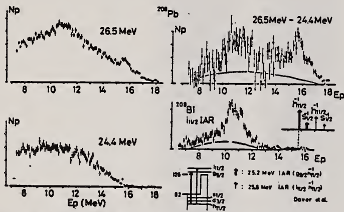
Fig. 9 Energy distribution of protons from ^{208}\text{Pb}(e,e'p) reaction. Top of the right hand side is a difference spectrum. Proton hole states and the core analogue state are indicated by arrows and ^{209}\text{Bi} result respectively.
