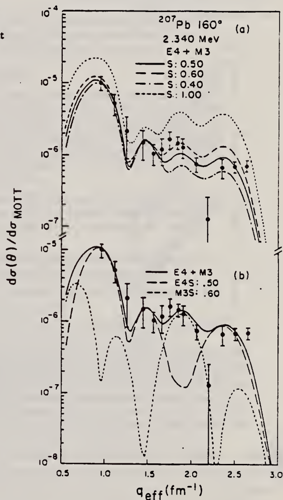
FIG. 1. (a) d\sigma/d\sigma_{MOTT} for the 2.340 MeV state in 207 Pb measured at 160°. The curves shown correspond to single-particle predictions with Hartree-Fock wave functions whereby the resulting amplitude has been scaled by the factor indicated. Core-polarization contribution has been fixed by our 90° measurements (Ref. 4). (b) A different scaling of the magnetic and the transverse electric contributions is possible in this case and results in a better fit.
