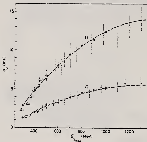
Fig. 3 - Our experimental data of the photofission cross-section per equivalent quantum for Bi and Pb compared with previous results. Experimental points: ● our data calculated as mean values of the results obtained with thin and thick targets; ▲ ref. (2); ○, □ ref. (3). The dashed lines are the best curves calculated by the least-squares method taking into account our results only. 1) Bi, 2) Pb.
