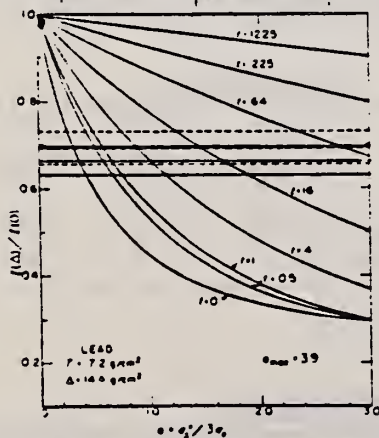
Fig. 6. Self-absorption attenuation curves for lead. See description for fig. 5.
