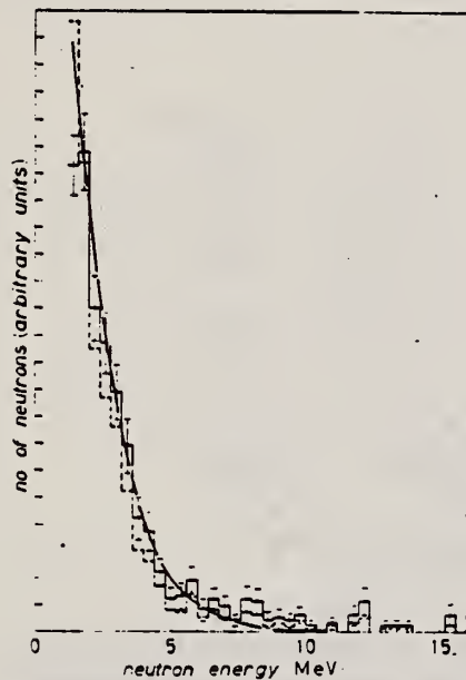
Fig. 2. - Energy distribution of photoneutrons from Bi. The dashed and the full-line histogram represent respectively the uncorrected and the corrected spectrum. The full-line curve corresponds to the expression given by LE COUTER and LANG (15) to represent the neutron energy distribution (see the text for the normalization chosen).
