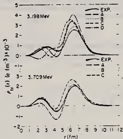
Fig. 2. Comparison of the extracted transition charge densities to a number of theoretical calculations for the lowest J^\pi = 5^- states of ^{208}\text{Pb} : curve A is that of Knüpfner and Huber [9]; B is that of Khodel and Saperstein [12]; C is that of Gogny and Dechargé [10] and D is that of Bertsch and Tsai.
