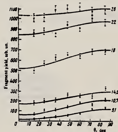
FIG. 3. Angular distributions of the emission of \text{Ra}^{226} photofission fragments relative to the direction of the bremsstrahlung beam. The curves were plotted by least squares.
