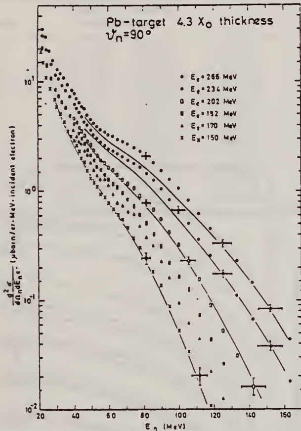
Fig. 7. Photoneutron spectra produced by electrons on a thick lead target (4.3 X 0 thickness) with primary energies of 150, 170, 182, 202, 234 and 266 MeV. These results are compared with the predictions of a quasi-deuteron model calculation (solid lines) with the parameters (defined in the text): α = 140 MeV/c, E well = 30 MeV, E b = -10 MeV and C'L = 19.0
