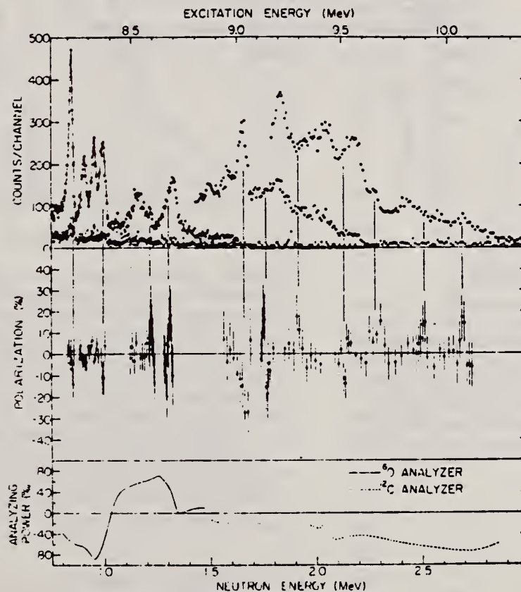
FIG. 1. The 90^\circ photoneutron polarization time-of-flight spectra for endpoint energies of 9.0, 9.6, and 10.2 MeV are shown at the top. The measured background is indicated with \times 's. Below this is the measured polarization. The error bars are statistical. The analyzing powers of ^{16}\text{O} and ^{12}\text{C} are given at the bottom.
