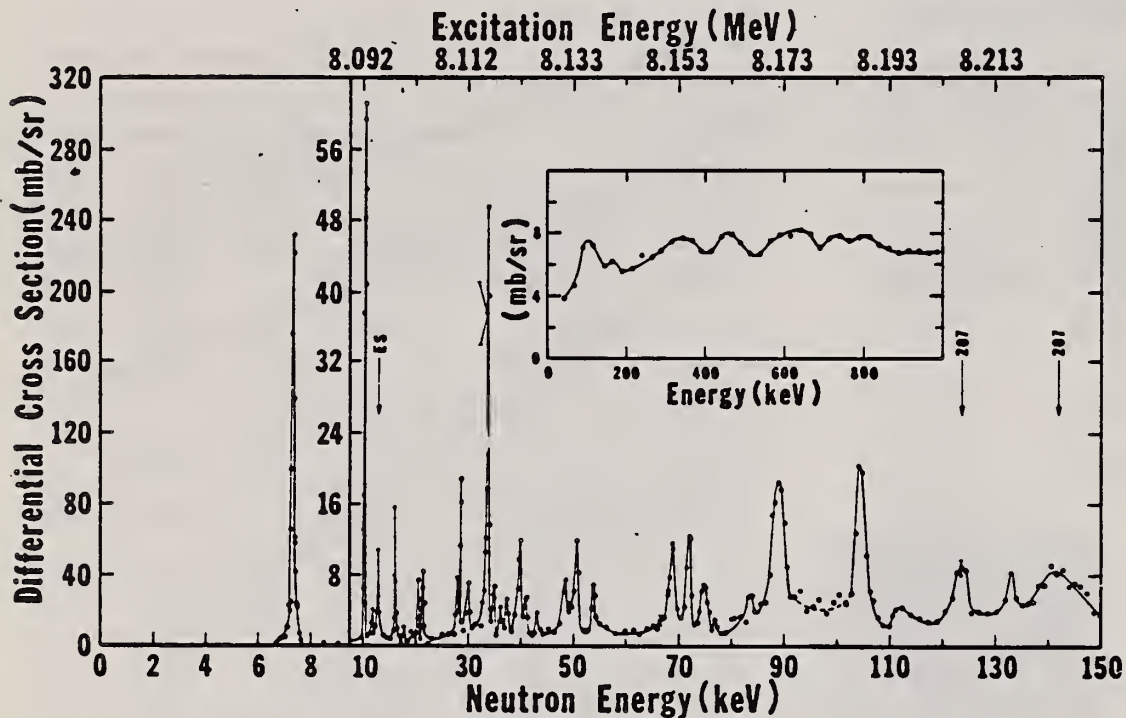
FIG. 8. The 135° differential threshold photoneutron cross section for 206 Pb (see caption to Fig. 4).
