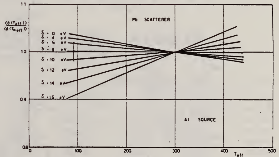
Fig. 9. Al-Pb resonance.
