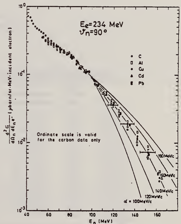
Fig. 8. Comparison of the shape of the high-energy part of the photoneutron spectra from C, Al, Cu, Cd and Pb. These measurements were performed with the same γ-shower spectrum, produced in a 0.3 cm thick lead sheet (see Fig. 2b). All spectra were fitted to the value for carbon at E n = 100 MeV. The values predicted by a quasi-deuteron model (solid lines), which are also fitted at E n = 100 MeV, were calculated with the parameters (defined in the text): E b = -10 MeV, E well = 30 MeV and C'L = 19.0 for different impulse parameters α = 100, 120, 140, 160 and 180 MeV/c
