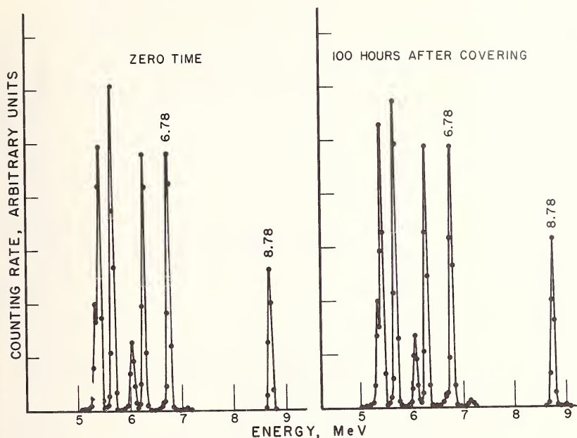
Figure 2. \alpha -particle spectra of a thorium-228 source immediately after covering the source with thin plastic and 100 hours after (see text). The highest energy peak, 8.78 MeV, has increased significantly over the initial value indicating accumulation of progeny of radon-220 behind the mylar covering layer.
