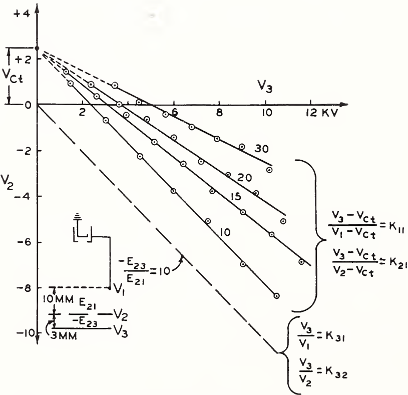
FIGURE 38.5. Focusing limit characteristics (dots tangent) for electron lens raster system. 40 holes per linear centimeter. V_{ct} =contact potential.
