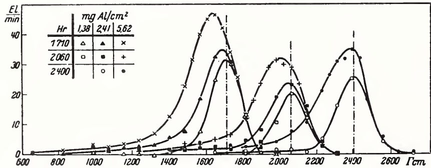
FIGURE 7.2. Momentum distribution of electrons scattered from thin Al-foils.
