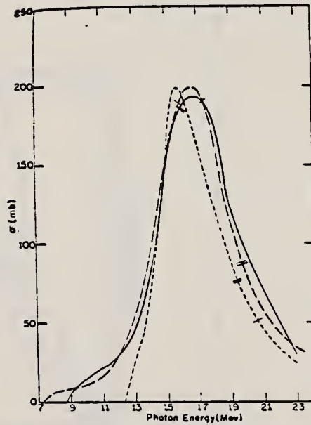
FIG. 5. Cross sections for the (\gamma, n) reactions in zirconium isotopes. Short dashes Zr^{20} , long dashes Zr^{21} , full curve Zr^{22} . The previously published Zr^{20} and Zr^{21} results have been recomputed, taking into account the present Zr^{22} measurements. The single and double slash marks on each curve represent the locations of the (\gamma, pn) and (\gamma, 2n) thresholds respectively. The units of the ordinate are 10^{-27} \text{ cm}^2 .
