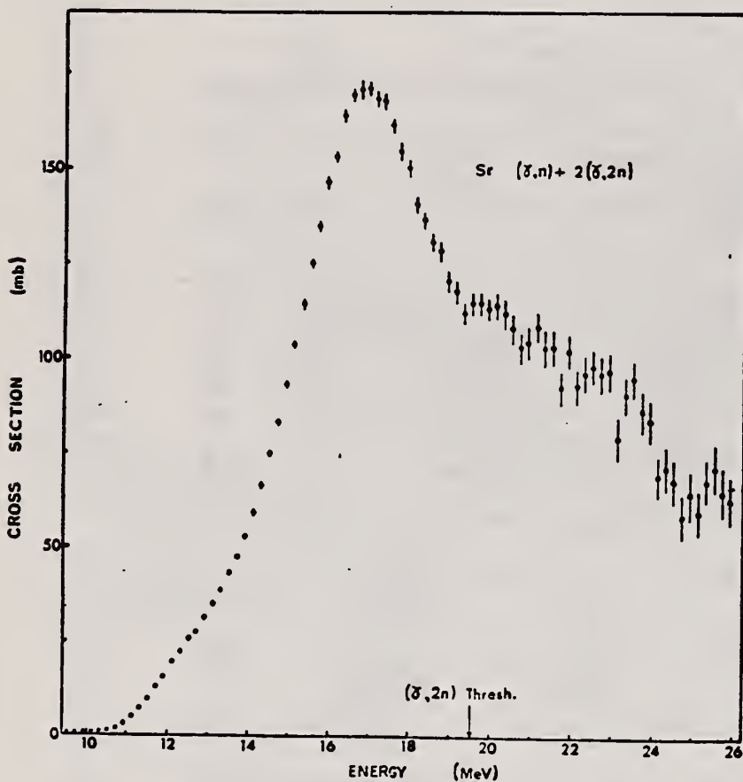
Fig. 1. The [\text{Sr}(\gamma, n) + 2\text{Sr}(\gamma, 2n)] cross section obtained by analysis of the yield curve using three interlocking second difference calculations. The resolution applied is 1.08 MeV.
