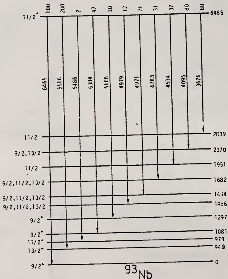
Fig. 3. Decay scheme of the 6465 keV level of 93 Nb showing level energies and relative intensities normalized so that the intensity of the ground-state transition is taken to be 100. The level spins are those obtained by combining the results of the present work (table 1) and those reported in refs. 3, 7 .
