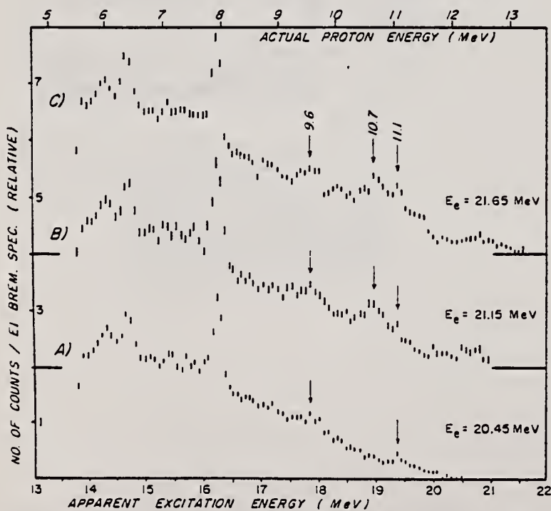
Fig. 3. The ^{90}\text{Zr}(e, e'p)^{90}\text{Y} spectra: (a) E_e(\text{max}) = 20.45 MeV; (b) E_e(\text{max}) = 21.15 MeV; (c) E_e(\text{max}) = 21.65 MeV. 378
