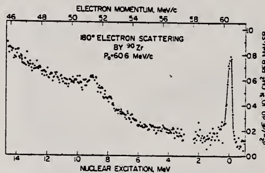
FIG. 2. Inelastic cross section spectrum of 60.6 MeV electrons scattered at 180° from 90 Zr.
