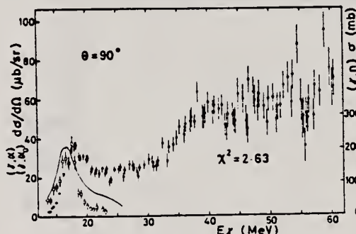
FIG. 6. Photoalpha differential cross section of 90 Zr (closed points) analyzed from the (e,α) cross section in Fig. 5 and 90 Zr(γ,α 0 ) differential cross section (open circles), at θ = 90°. E1 interaction only was considered in these analyses. The value of χ 2 for the total (γ,α) cross section was calculated for the cross section smoothed by eye. Solid line shows 90 Zr(γ,α) cross section.
