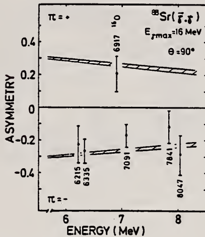
Fig. 1. Observed asymmetries for five ground state dipole transitions in 88 Sr and for the 2 + transition at 6917 keV in 16 O. The energies for the 88 Sr states were taken from /2/. The hatched band represents the expected asymmetry for states with positive parity (upper part) and negative parity (lower part)
