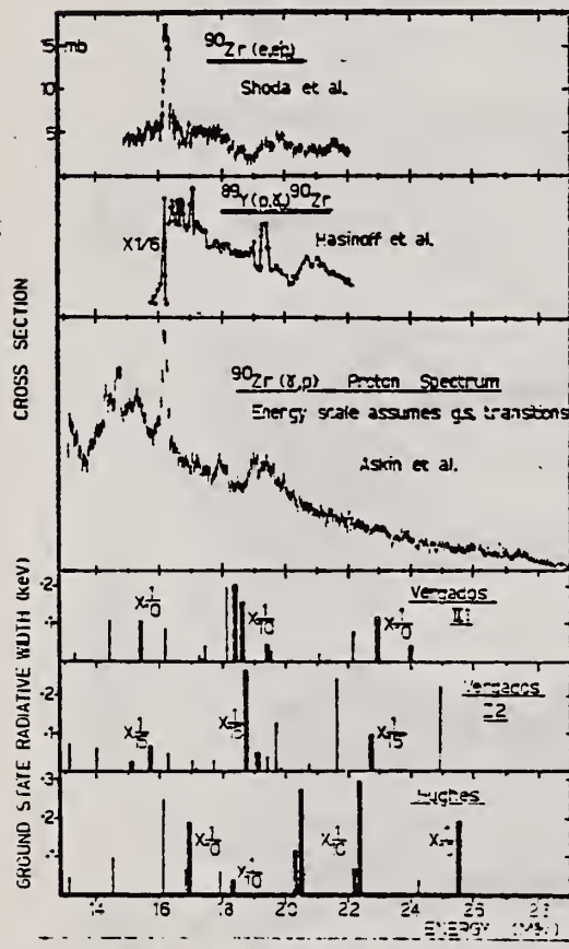
Fig. 3. Comparison of the presented ^{90}\text{Zr}(\gamma, p) proton spectrum with the (e, e'p_0) data of Shoda (6) and the (p, \gamma_0) measurement by Hasinoff et al. (5) . Also shown are the results of calculations by Hughes and Fallieros (3) and Vergados and Kuo (4) of the excitations and ground state radiative widths of T_{1-} states in ^{90}\text{Zr} .
