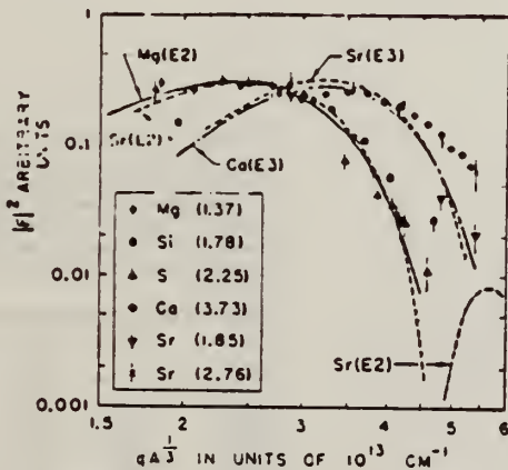
FIG. 7. Inelastic "universal curves." A composite plot of inelastic data from Mg, Si, S, Ca, and Sr against qR . The various form factors are arbitrarily normalized to minimize the spread of points. The point from sulfur and the point from silicon which seem to deviate from the "universal curve" are assumed to contain undetected experimental errors. The curves labeled Mg(E2), Sr(E2), Ca(E3), and Sr(E3) are calculated for electric-quadrupole and-octupole transitions using the "smeared \delta -function" transition charge densities of Sec. V, and are arbitrarily normalized.
