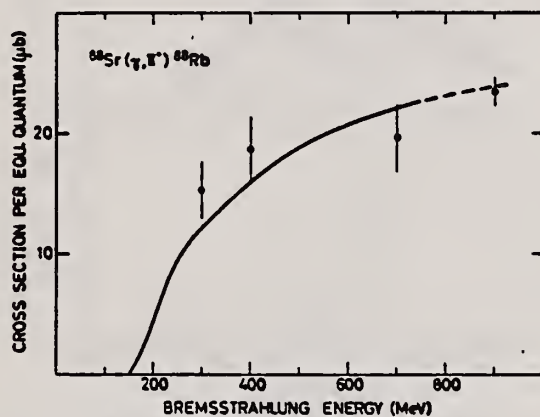
Fig. 4. Absolute yield for ^{88}\text{Sr}(\gamma, \pi^+)^{88}\text{Rb} .
