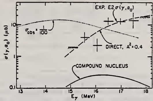
FIG. 6. Solid lines are the E2 ( \gamma, \alpha_0 ) cross section, obtained from the observed E2 capture by detailed balance. The cross hatching indicates an upper limit. Solid curve is the compound nucleus E2 ( \gamma, \alpha_0 ) expected from a 4-MeV wide resonance centered at 14.5 MeV. The broken curve is that calculated for a direct reaction proceeding through a giant quadrupole state that has a 40% ^{86}\text{Sr} + \alpha component. Dotted curve is the gamma-ray absorption cross section, divided by 100, expected for a 4-MeV wide resonance centered at 14.5 MeV.
