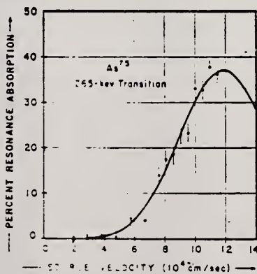
Fig. 3. Calculated absorption points with experimental points with F = 4.07 \times 10^{-10} .
