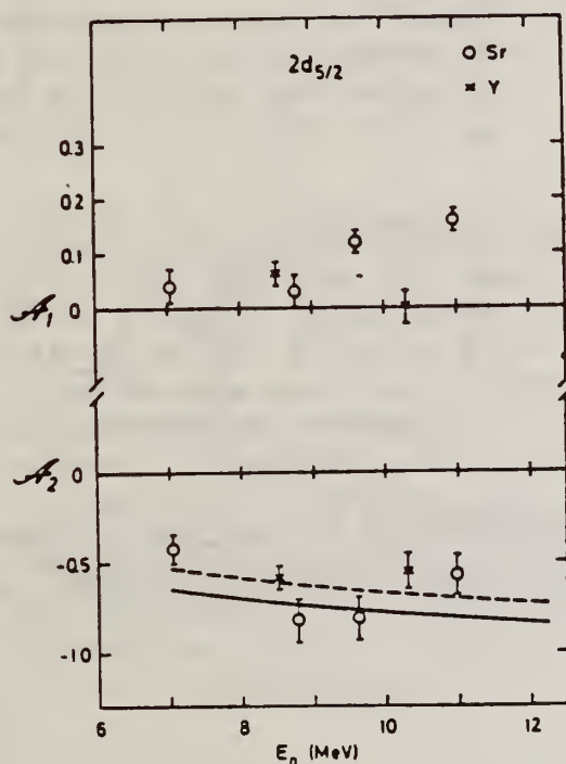
Fig. 2. Angular distribution coefficients A_1 and A_2 versus neutron energy for the reactions ^{88}\text{Sr}(n, \gamma)^{89}\text{Sr} (open circles) and ^{89}\text{Y}(n, \gamma)^{90}\text{Y} (crosses). The curves for the A_2 coefficient represent the results of theoretical calculations for E1 transitions to the 2d_{5/2} state in ^{89}\text{Sr} from the direct (solid line) and DSD (dashed line) capture models.
