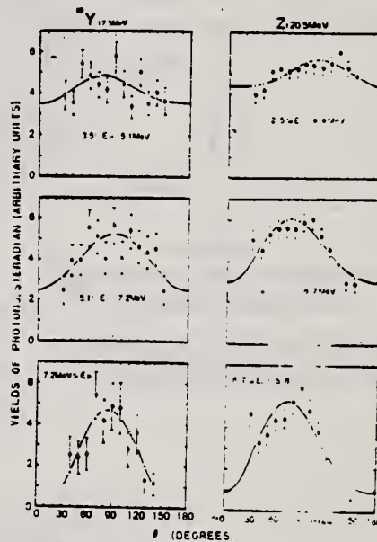
Fig. 3. Examples of angular distributions of photoprotons from 88 Y and Zr.
