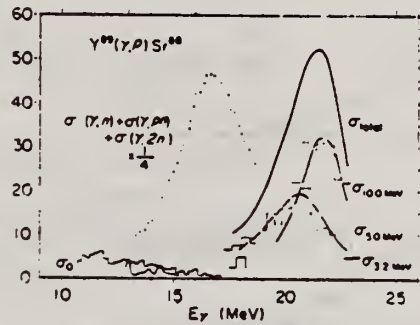
Fig. 10. Cross sections for strong photoproton transitions on ^{89}\text{Y} . The neutron emission cross section (9) and the result of the ^{88}\text{Sr}(p, \gamma)^{89}\text{Y} reaction (10) are also shown.
