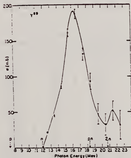
FIG. 1. Cross section for the (\gamma, xn) reaction in Y^{89} , calculated from the yield data, at an intermediate stage of the smoothing process (see text). The vertical lines through the calculated points show the rms-uncertainty in the cross-section values, produced by the statistical uncertainty of the recorded counts of the raw yield data. Other sources of errors, and the partial smoothing already done have been ignored in calculating these uncertainties. The arrows along the abscissa indicate the thresholds for emission of the particles indicated by the labels therewith. The units of the ordinate are 10^{-27} \text{ cm}^2 .
