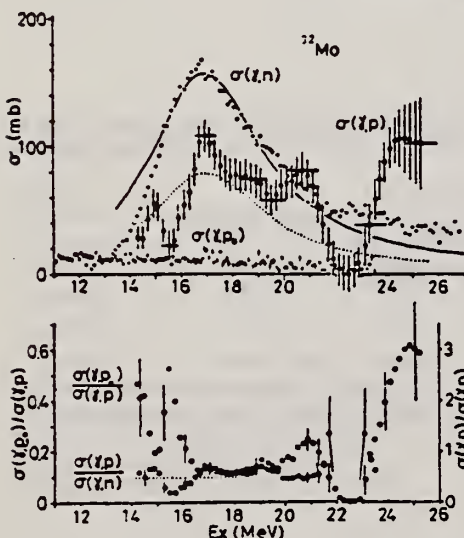
Fig. 5. The caption is the same as in fig. 5, but \sigma(\gamma, p_0) is the present result while the plots and Lorentz line for the (\gamma, n) reaction are from ref. 15 .
