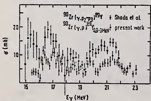
FIG. 8. A comparison of present results for the 90 Zr(γ, p) 89 Y 0-3 cross section with the data of Shoda et al. (Ref. 4).
