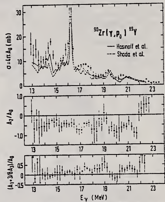
FIG. 4. Legendre polynomial coefficients for the angular distributions of protons in the reaction 90 Zr(γ, p 0 ) 89 Y obtained from differential cross sections for the angles 30°, 90°, and 150° assuming an angular dependence of the form W(\theta) = \sum_{l=0}^3 A_l P_l(\cos\theta) . Cross sections for particular angles were determined from measured spectra by means of a least-squares-fit analysis (Ref. 13). On the top diagram present results for \sigma = 4\pi A_0 (data points) are compared to the data of Refs. 11 and 8.
