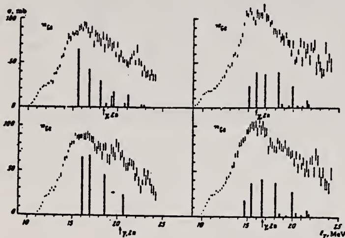
Fig. 2. The same as in Fig. 1, but for ^{70,72,74,76}\text{Ge} .
