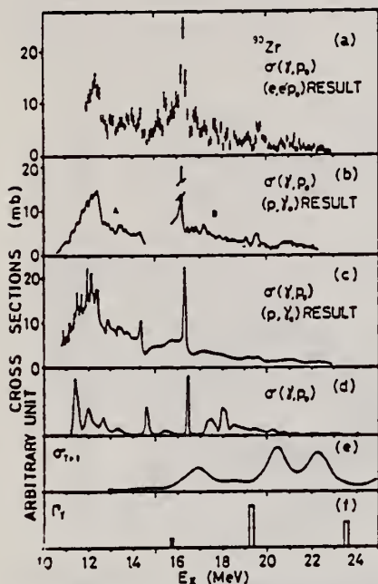
Fig. 11. Comparison of p, \nu proton cross sections of ^{90}\text{Zr} . (a) Present result. (b) Curve A, ref. 31 ); curve B, ref. 3 ); open circles, ref. 32 ). (c) Ref. 4 ). (d), (e), (f) Theoretical estimates, refs. 12, 14, 13 respectively.
