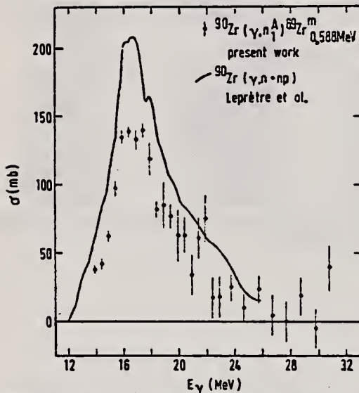
FIG. 12. The (\gamma, n_1^+) cross section represented by data points contains, in addition to the ^{90}\text{Zr}(\gamma, n_1^+)^{89}\text{Zr}_{0.588} contribution, also contributions of all photoneutron cross sections involving those residual ^{89}\text{Zr} states which subsequently decay to the first-excited state. For comparison the (\gamma, n + np) data of Leprêtre et al. (Ref. 6) (continuous curve) are also shown.
