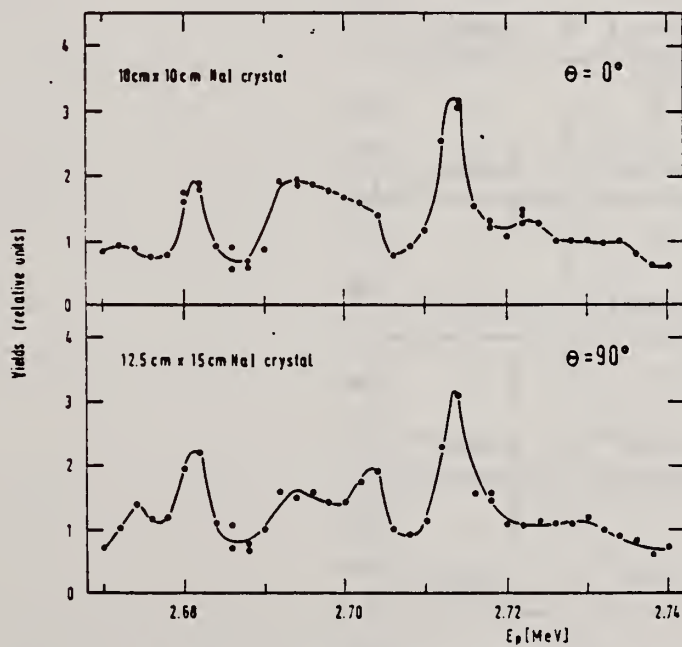
The excitation functions for the reaction ^{89}\text{Y}(p, \gamma)^{89}\text{Zr} measured at \theta = 0^\circ and \theta = 90^\circ with an energy resolution of 2 keV.
