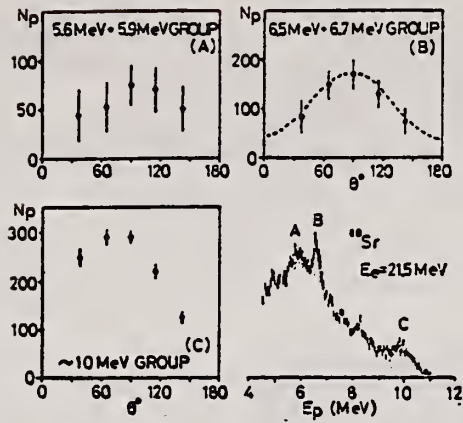
Fig. 16. Angular distributions of proton groups indicated by hatching in the proton spectrum which is summed over various angles. The result for group B is compared with that of the E_p = 7.9 \text{ MeV} group of ^{90}\text{Zr} (dashed line).
