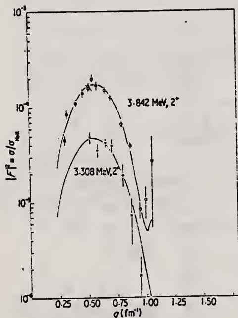
Figure 4. Inelastic form factors for the 3.842 MeV, 2 + (□ and ○) and for the 3.308 MeV, 2 + (×) levels. The data points □ are those of Bellicard et al. (1970). The solid lines are the best fits to these levels with the model independent measurements of Metzger (1974) used as constraints (see text).
