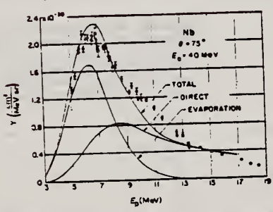
Fig. 8. Energy distribution of protons from Nb. The curves are calculated distributions arbitrarily normalized.
