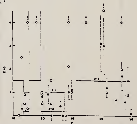
FIG. 4. The values of the fast photoproton anisotropy coefficient b/a found by the present authors (●) and other workers (○) in the region of the periodic table 10 < Z < 50 . Arrows indicate inaccessible points. The references to the results of other workers are given in Table II. The demarcations are explained in the text.
