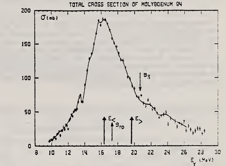
Fig. 8. Same as fig. 7, for ^{94}\text{Mo} .
