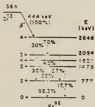
FIG. 1. Decay scheme of Br^{82} , showing only the major transitions and their percentages based on the summary (Ref. 2) of the data of recent measurements. The relative gamma-ray intensities are given in parentheses. The percentages of the gamma rays shown are adjusted to agree with the data of the decay of the 2648 level.
