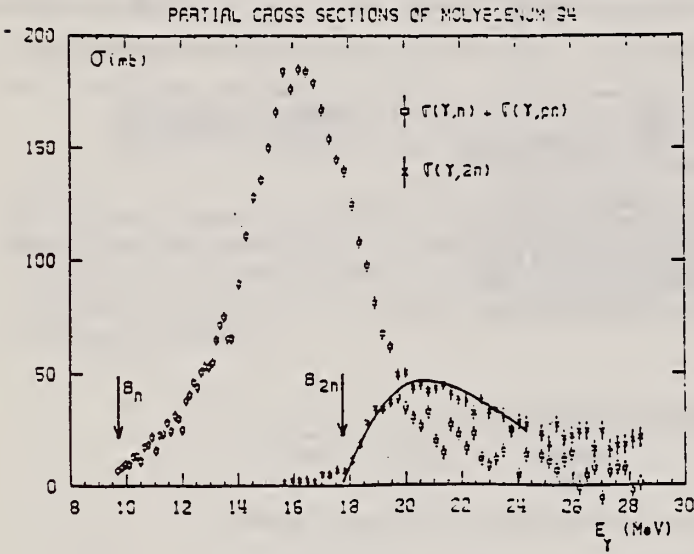
Fig. 2. Same as fig. 1, for ^{94}\text{Mo} .
