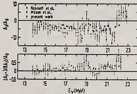
FIG. 5. A comparison of present results for the Legendre polynomial coefficients of the reaction ^{90}\text{Zr}(\gamma, p)^{89}\text{Y}_{x} with the data of Refs. 3 and 8.
