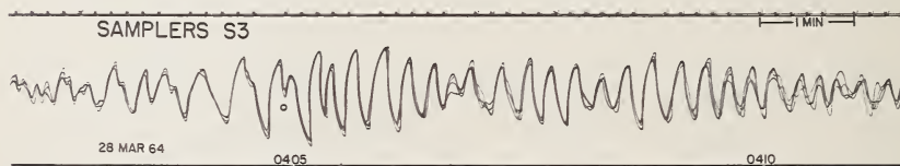
Superimposed recordings from four spaced infrasonic microphones show atmospheric sound waves caused by Rayleigh waves from the great Alaskan earthquake passing through the Washington, D.C., area. These recordings indicate a total earth motion of almost 2 inches, too large a movement to be measured accurately by conventional seismometers. (See page 62)
