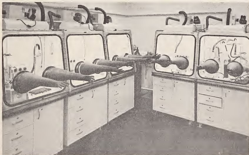
Inside view of clean room used in sample preparation for high sensitivity activation analysis. All chemical procedures are conducted inside the glove boxes. (See page 126)
