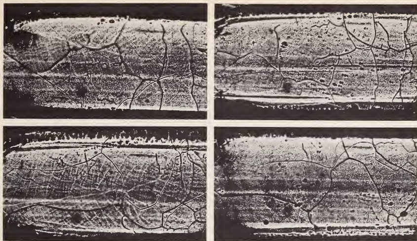
Four sides of a methane crystal at 87 °K seen through liquid argon. The heavy lines are grain boundaries on the back faces of the crystal and the lighter ones are grain boundaries on the front faces. These crystals provide excellent sources for spectroscopic, solid state, and surface physics studies at low temperatures. (See page 154)
