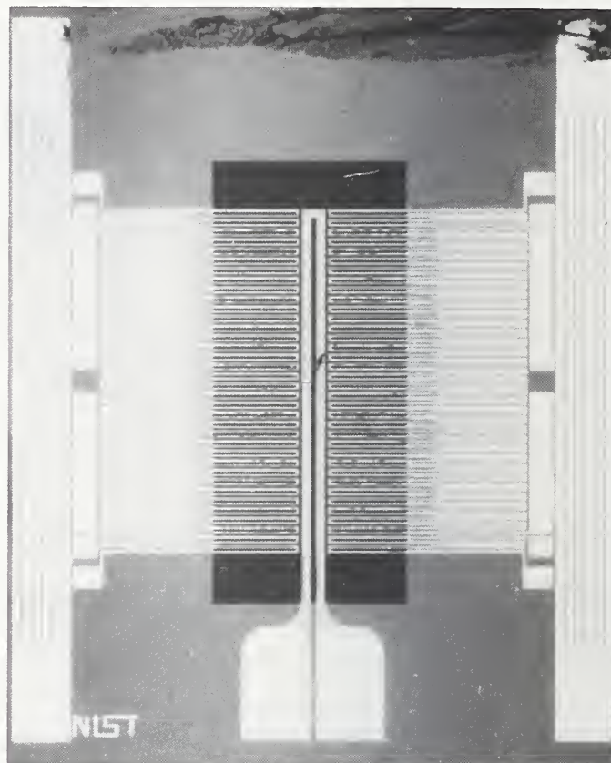
Thermal voltage and converters are used to make accurate ac to dc transfer measurements. To improve the Nation's capability to make these measurements, NIST is investigating multijunction thermal converters made using thin-film technology developed for the semiconductor industry. An experimental NIST device is shown.
