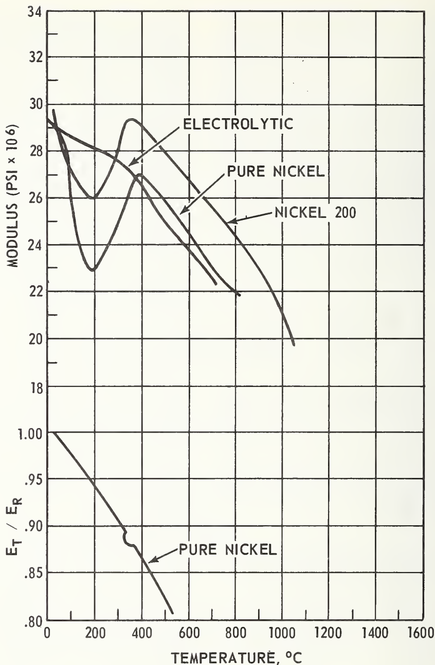
FIGURE 40. Effect of temperature on the elastic modulus of nickel [329,330,331,332].
