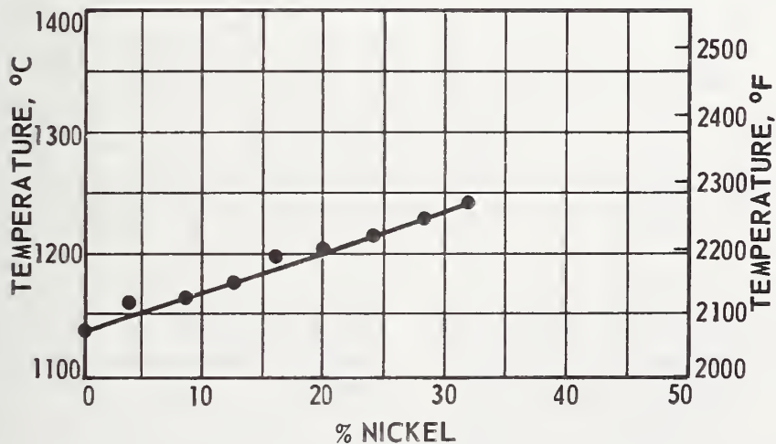
FIGURE 92. Effect of nickel on the carbon content and temperature of the eutectic in iron-nickel alloys [809].
