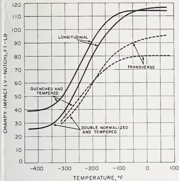
FIGURE 90. Impact properties of 9 percent nickel steel [765].
