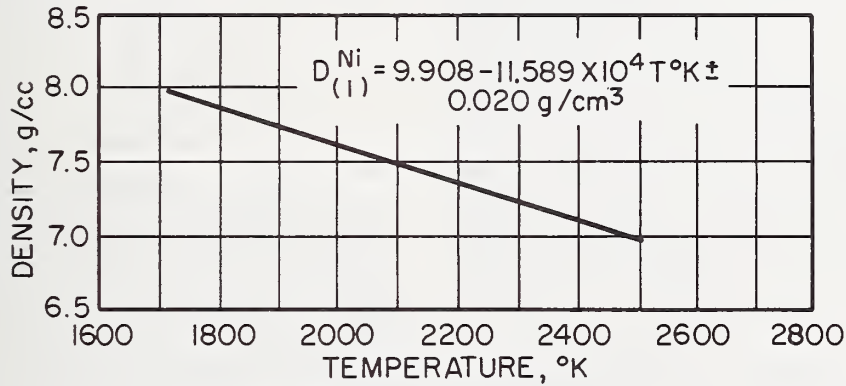
FIGURE 5. The density of liquid nickel [86].
