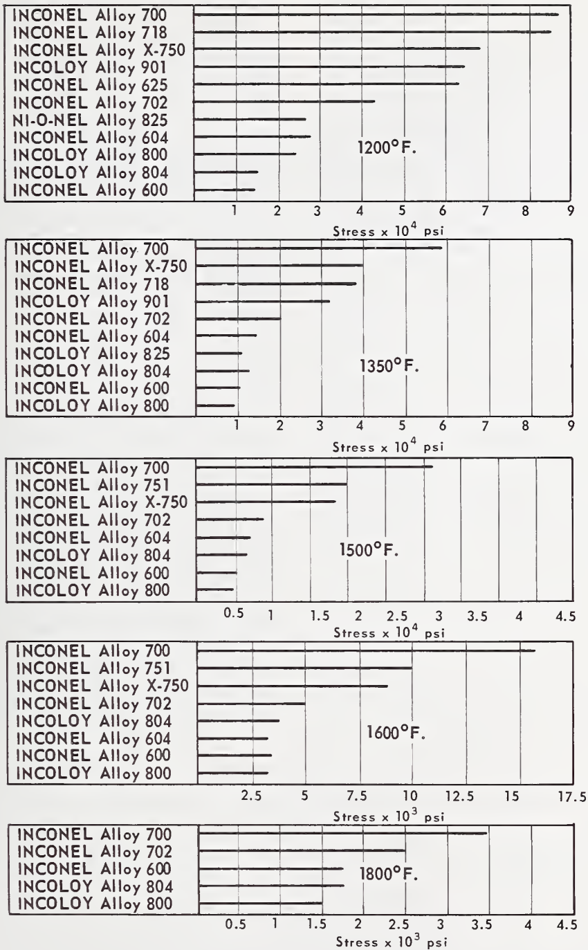
Typical Stress for 1000 Hour Rupture Life At Various Temperatures
