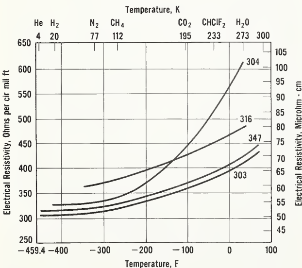
FIGURE 99. Effect of temperature on the electrical resistivity of some stainless steels [844].
