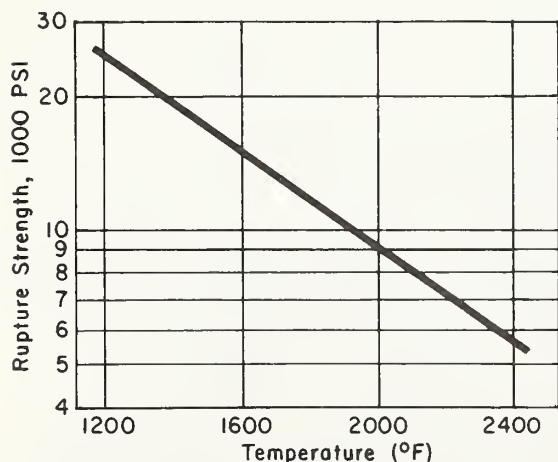
FIGURE 63. 100-hr stress-rupture strength of TD nickel [626].
