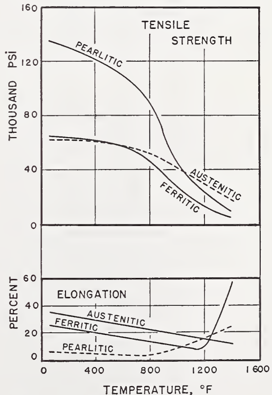
FIGURE 94. Effect of temperature on the tensile strength and elongation of ductile cast irons [821].
