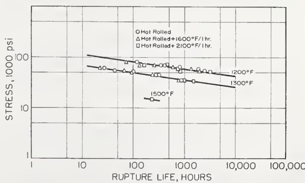
FIGURE 56. Stress-rupture strength of Inconel alloy 625 [609]. (Hot rolled 9/16 in rod, annealed 1 hr at 1600 °F.)
