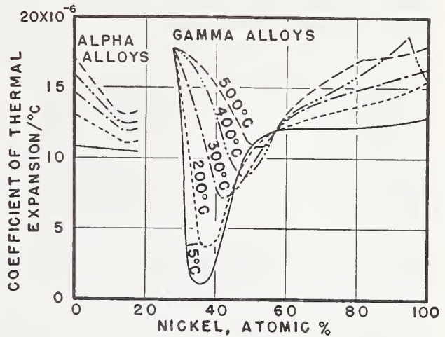
FIGURE 105. Coefficient of thermal expansion of iron-nickel alloys at temperatures up to 500 °C [120].
