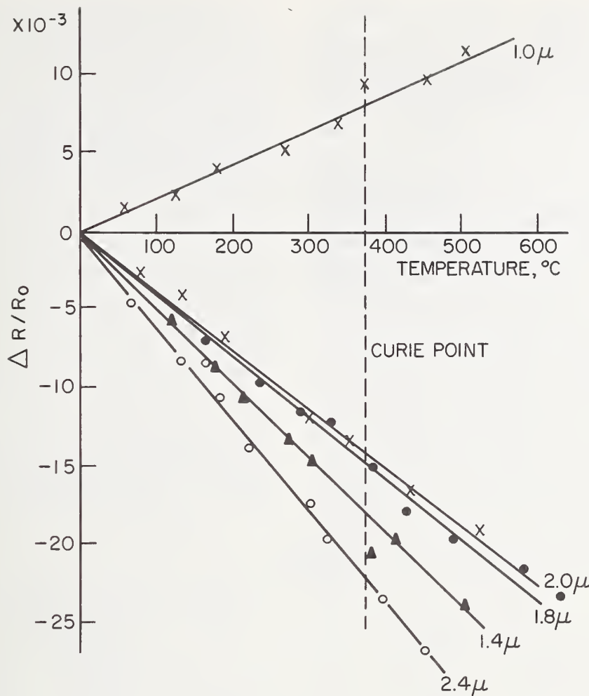
FIGURE 7. Change in reflectivity of nickel as a function of temperature for several wave lengths of light [96].
