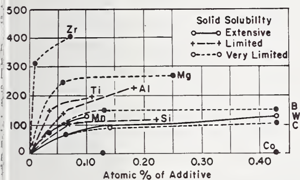
FIGURE 15. Increase in recrystallization temperature of high-purity nickel resulting from additions of indicated elements [144].
