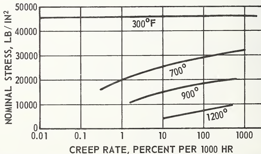
FIGURE 46. Influence of stress on the average creep rate of nickel during the second stage of creep [344].
