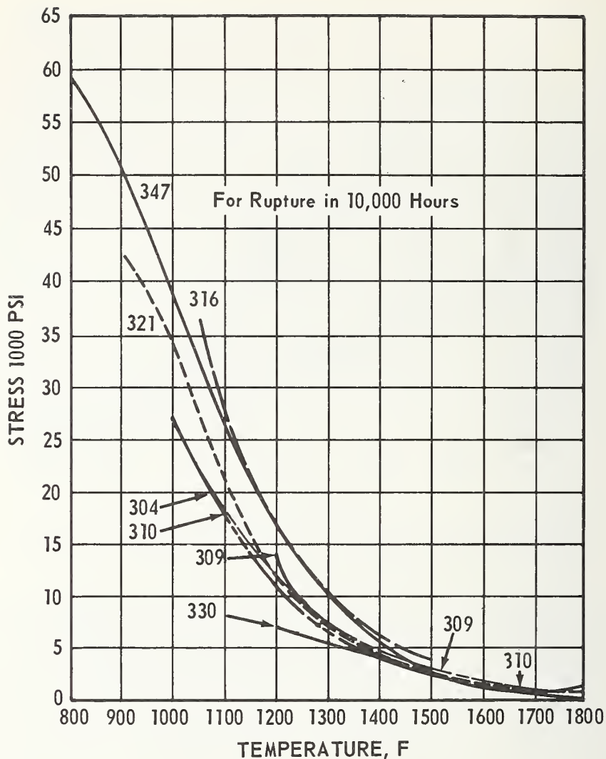
FIGURE 103. Stress-rupture curves for several annealed austenitic stainless steels [845].
