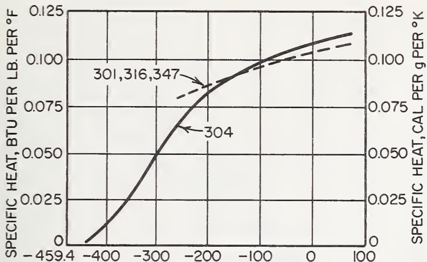
FIGURE 96. Effect of temperature on the specific heat of some stainless steels [844].
