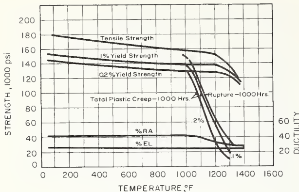
FIGURE 57. Tensile, creep, and rupture properties of Inconel alloy 718 [610]. (Bar stock annealed 1 hr at 1700 °F and aged 16 hr at 1325 °F.)
