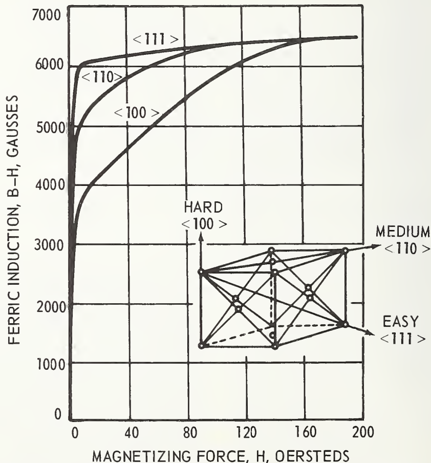
FIGURE 24. Crystal structure of nickel and types of magnetization curves obtained in crystallographic directions [173].
