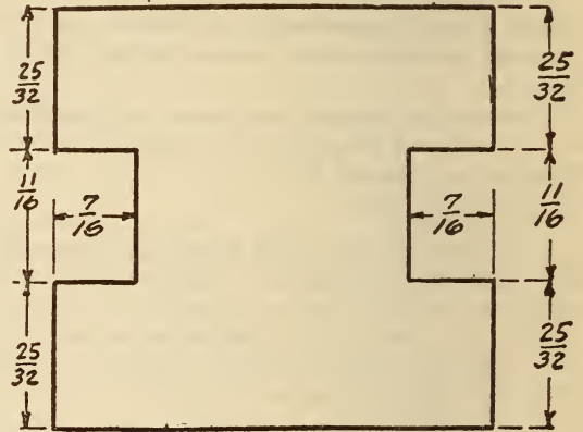
FIG. 52.—2½-inch factory flooring grooved for splines
