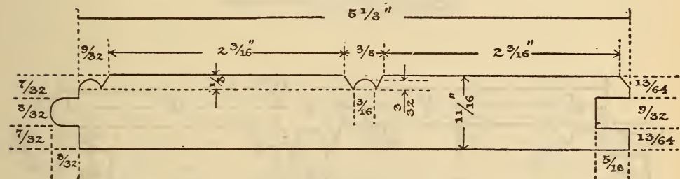
FIG. 88.—1 by 6 inch kiln-dried double beaded ceiling, green 5\frac{3}{8} -inch face
