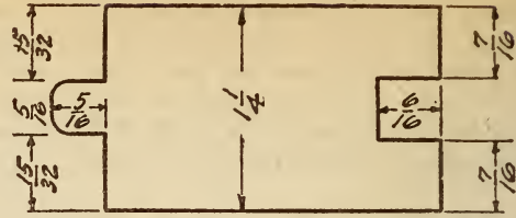
FIG. 49.—1½-inch T. and G. factory flooring
