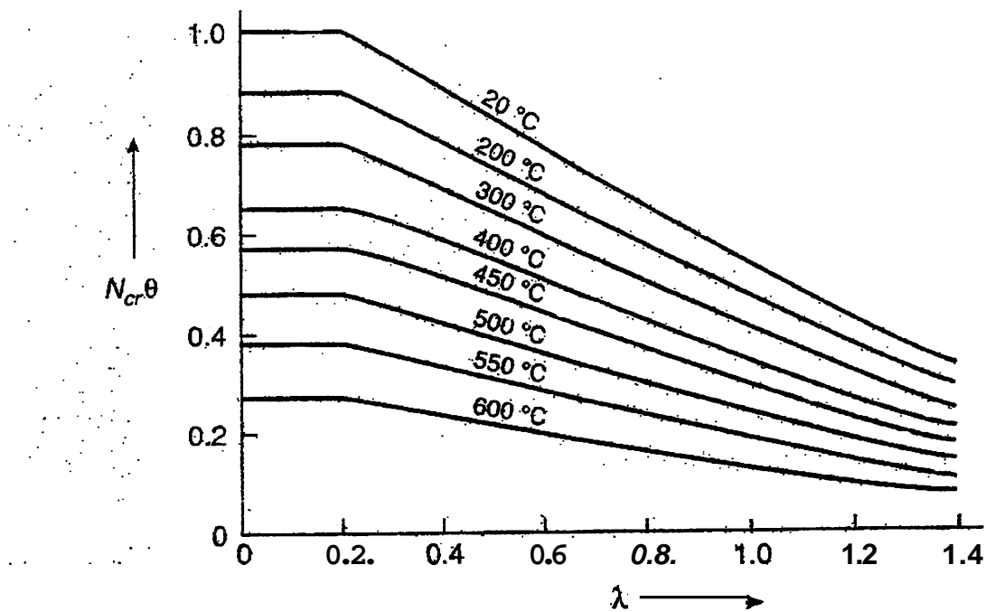
Figure 3.1 Buckling Curves for Steel Columns [Milke, 2002, p. 4-232] (from ECCS, 1985)
