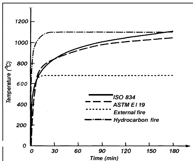
Figure 2. Standard time temperature curves
