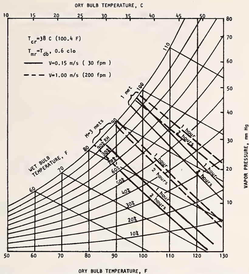
Fig. (4) Lines of Constant Core Temperature ( 38^\circ\text{C} ) at One and Three Mets, after One and Two House Exposure.
