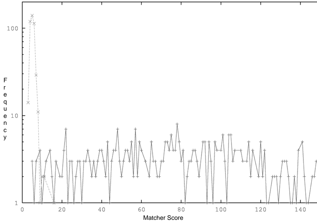
Figure 3: Match and non-match score distributions
