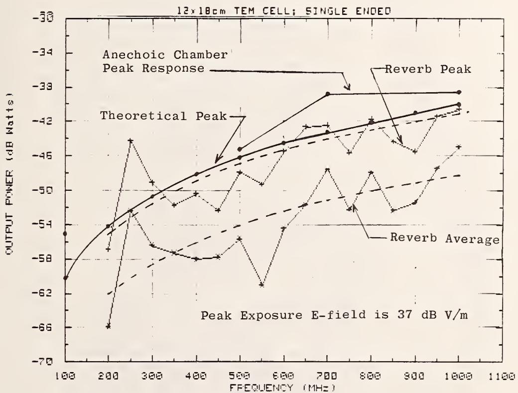
Figure 5.5 Comparison of power coupled to one port of 12 cm x 18 cm x 36 cm TEM cell with 5.1 cm x 5.1 cm aperture placed inside NBS reverberation and anechoic chambers.
