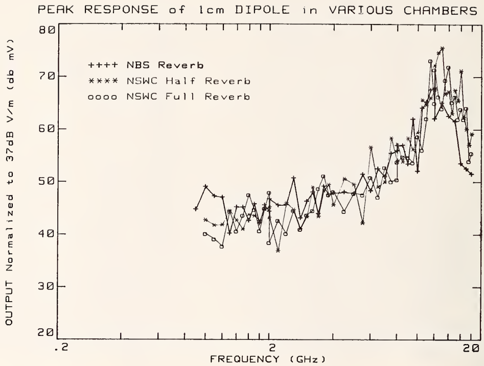
Figure 5.15 Comparison of 1 cm dipole probe's peak response to normalized E-field of 37 dB V/m using NBS and NSWC reverberation chambers.
