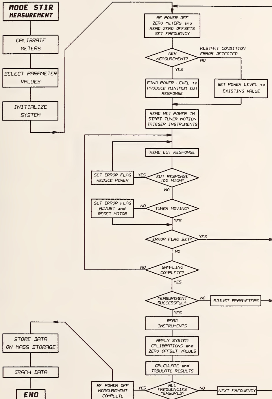
Figure 4.4 Flow diagram for mode-stirred measurements.
