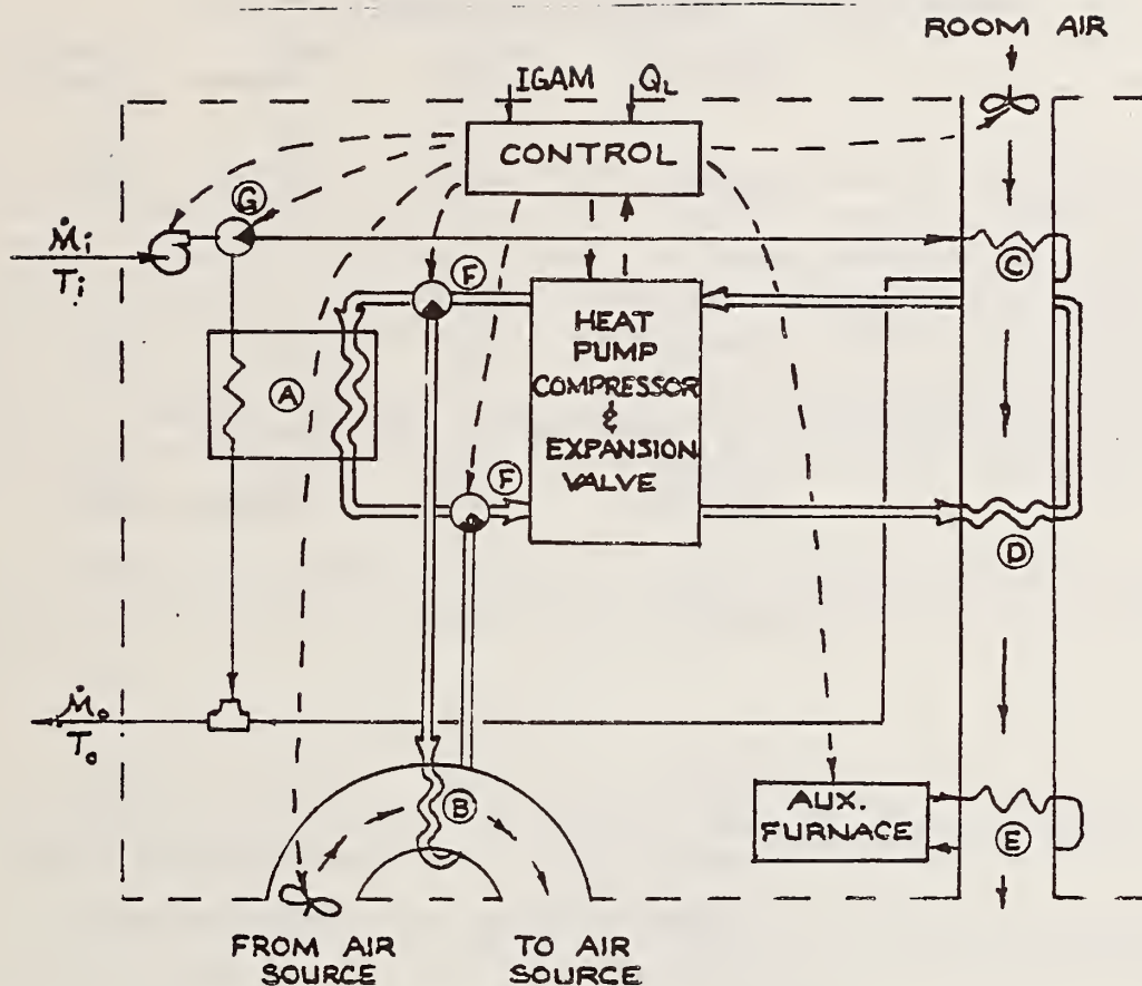
Figure D-1 Heat Pump Model Schematic.
