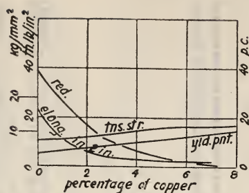
FIG. 3.—Tensile properties of aluminum-copper sand-cast alloys.
