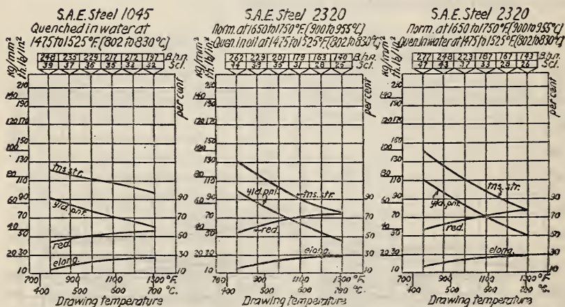
FIG. 19.—Effect of drawing temperature on the tensile properties of steel.
