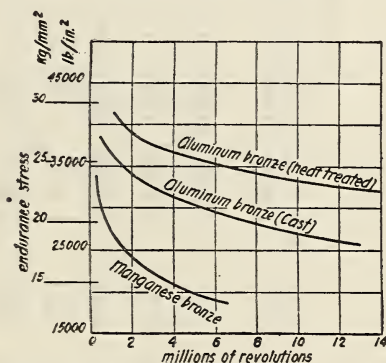
FIG. 14.—Fatigue properties of aluminum and manganese bronzes.
