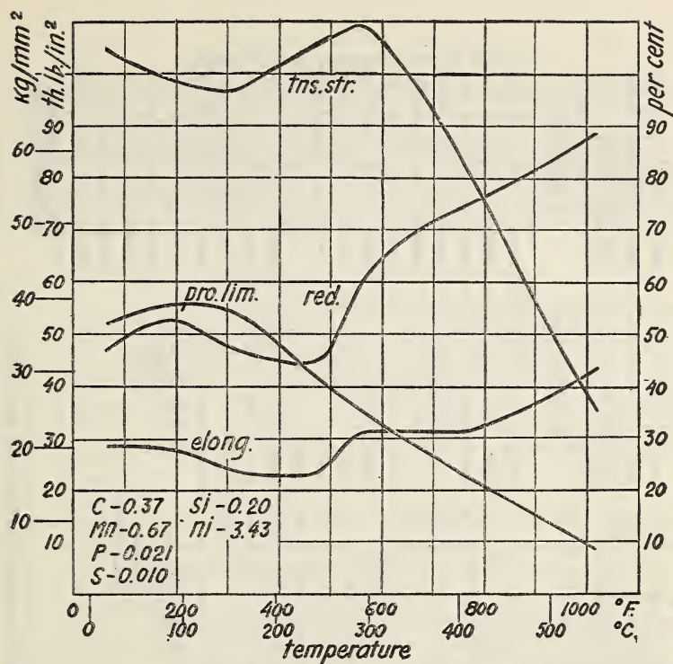
FIG. 44.—Tensile properties at elevated temperatures of 3\frac{1}{2} per cent nickel steel containing 0.37 per cent carbon.
