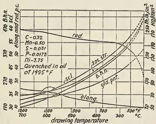
FIG. 31.—Effect of drawing temperature on the tensile properties of nickel steel.
