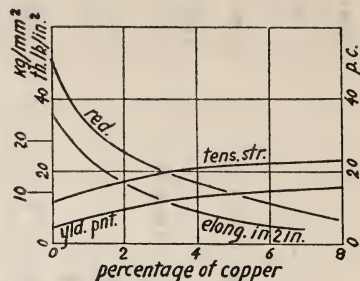
FIG. 4.—The tensile properties of aluminum-copper chill-cast alloys.
