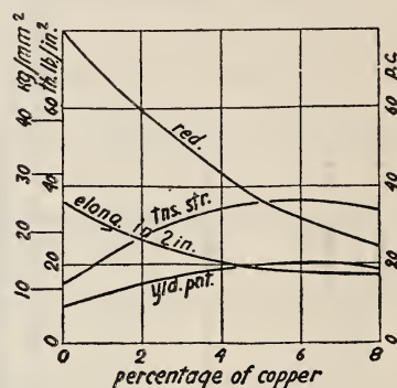
FIG. 6.—The tensile properties of aluminum-copper alloys 1\frac{1}{4} in. (31.7 mm) diameter bars hot rolled from 3 in. (76.2 mm) ingots.
