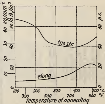
FIG. 8.—Effect of annealing on the tensile properties of duralumin.
