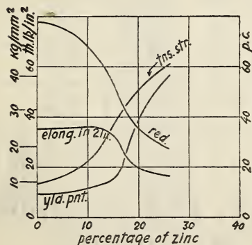
FIG. 12.—The tensile properties of aluminum-zinc alloys; 1 1/4 in. (31.7 mm), diameter bars hot rolled from 3 in. (76.2 mm) ingots.
