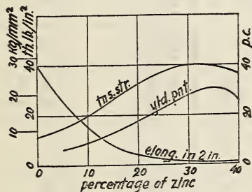
FIG. 11.—The tensile properties of aluminum-zinc chill-cast alloys.
