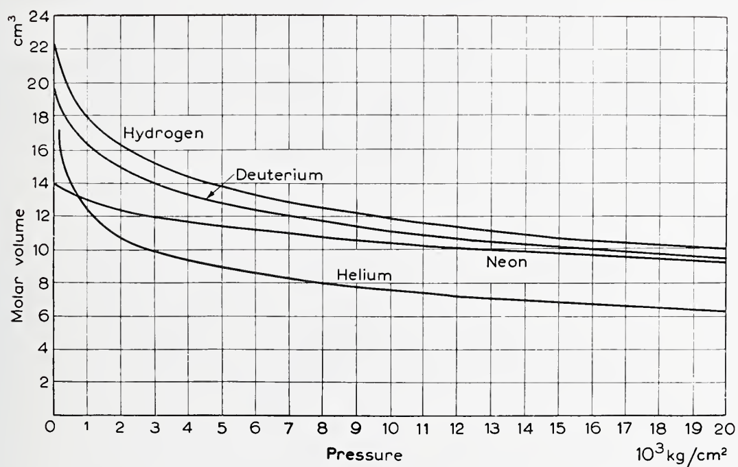
FIGURE 41. PVT diagram for compressed solid hydrogen at high pressures and 4K.
