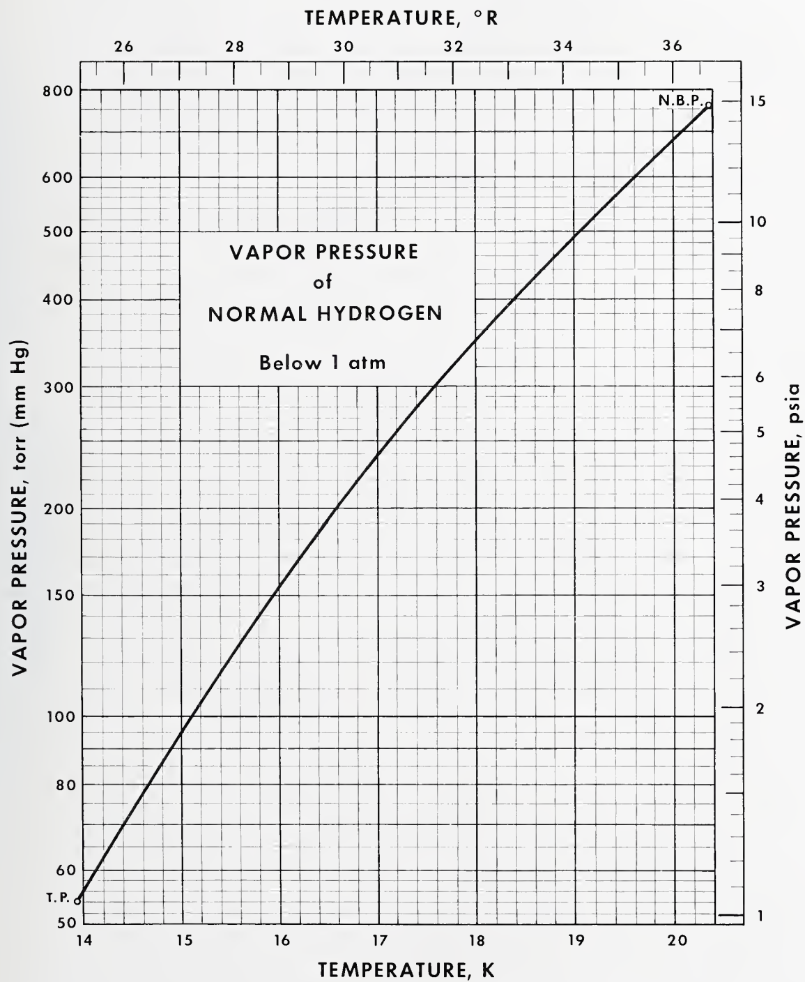
FIGURE 30. Vapor pressure of normal hydrogen below 0.101325 MPa (1 atm).
