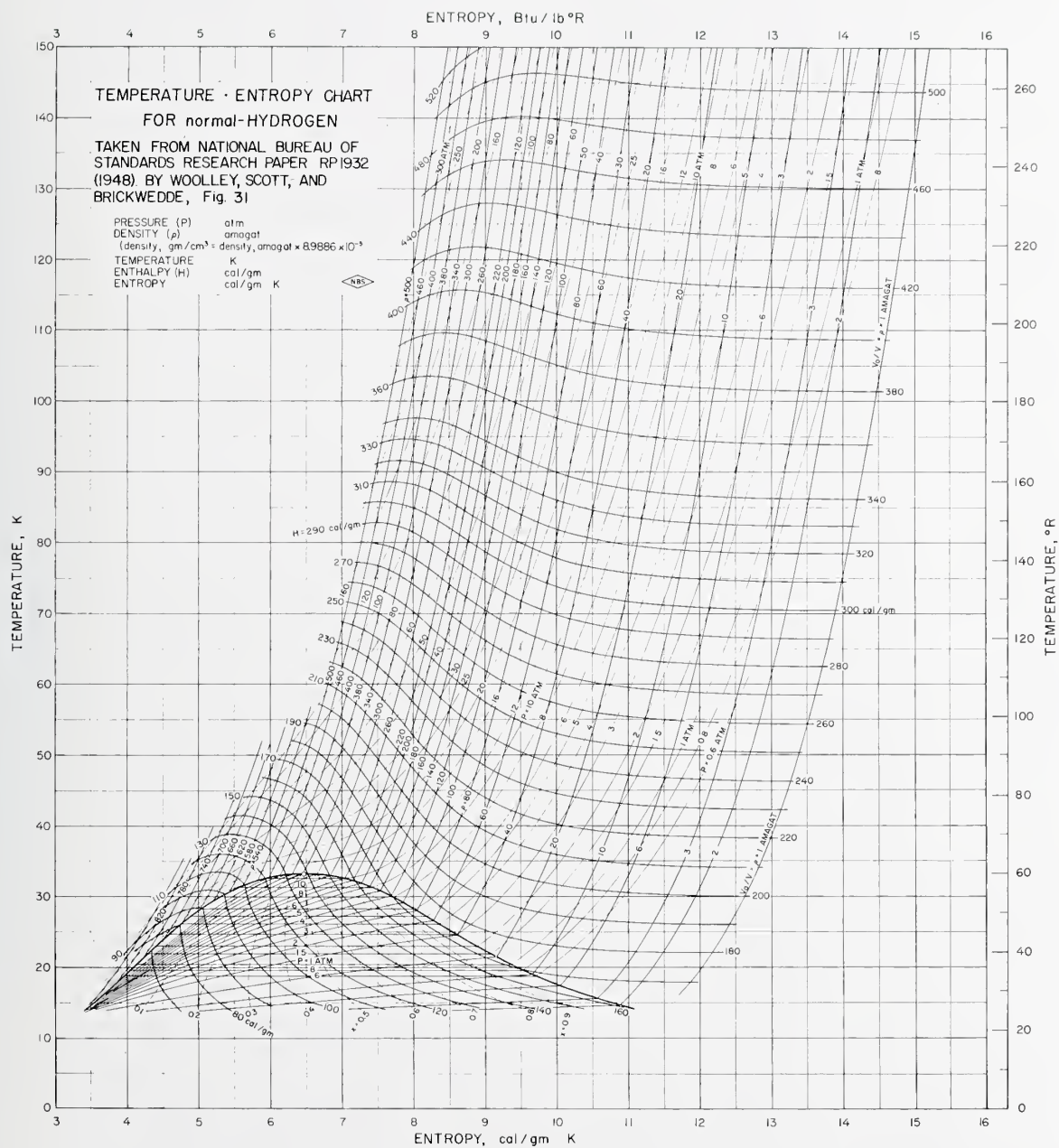
FIGURE 6. Normal hydrogen temperature-entropy chart (15 to 150 K).
