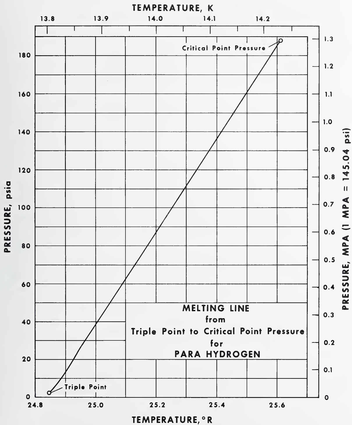
FIGURE 18. Melting line from triple point to critical point pressure for parahydrogen.
