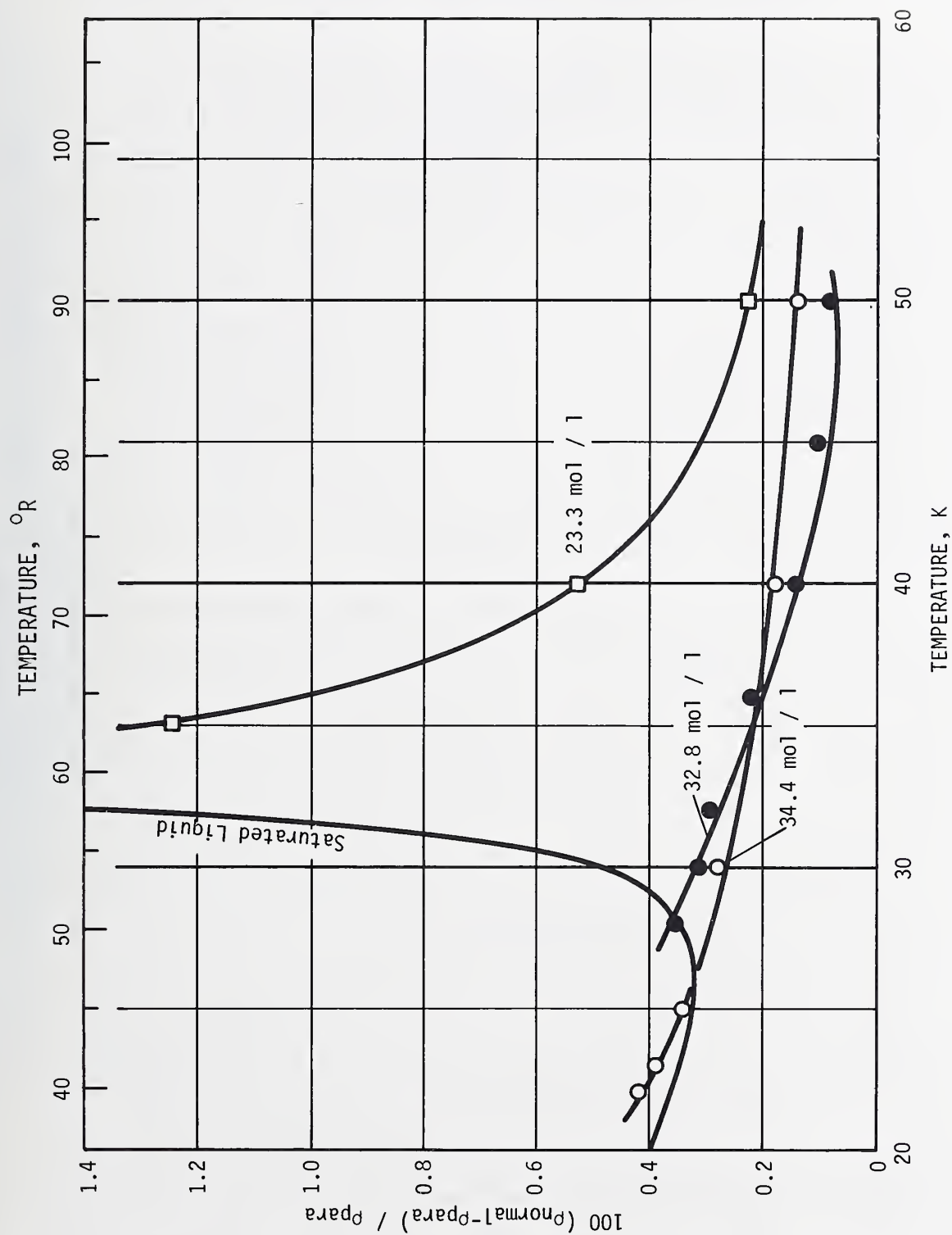
FIGURE 57. Density differences between normal and parahydrogen.
