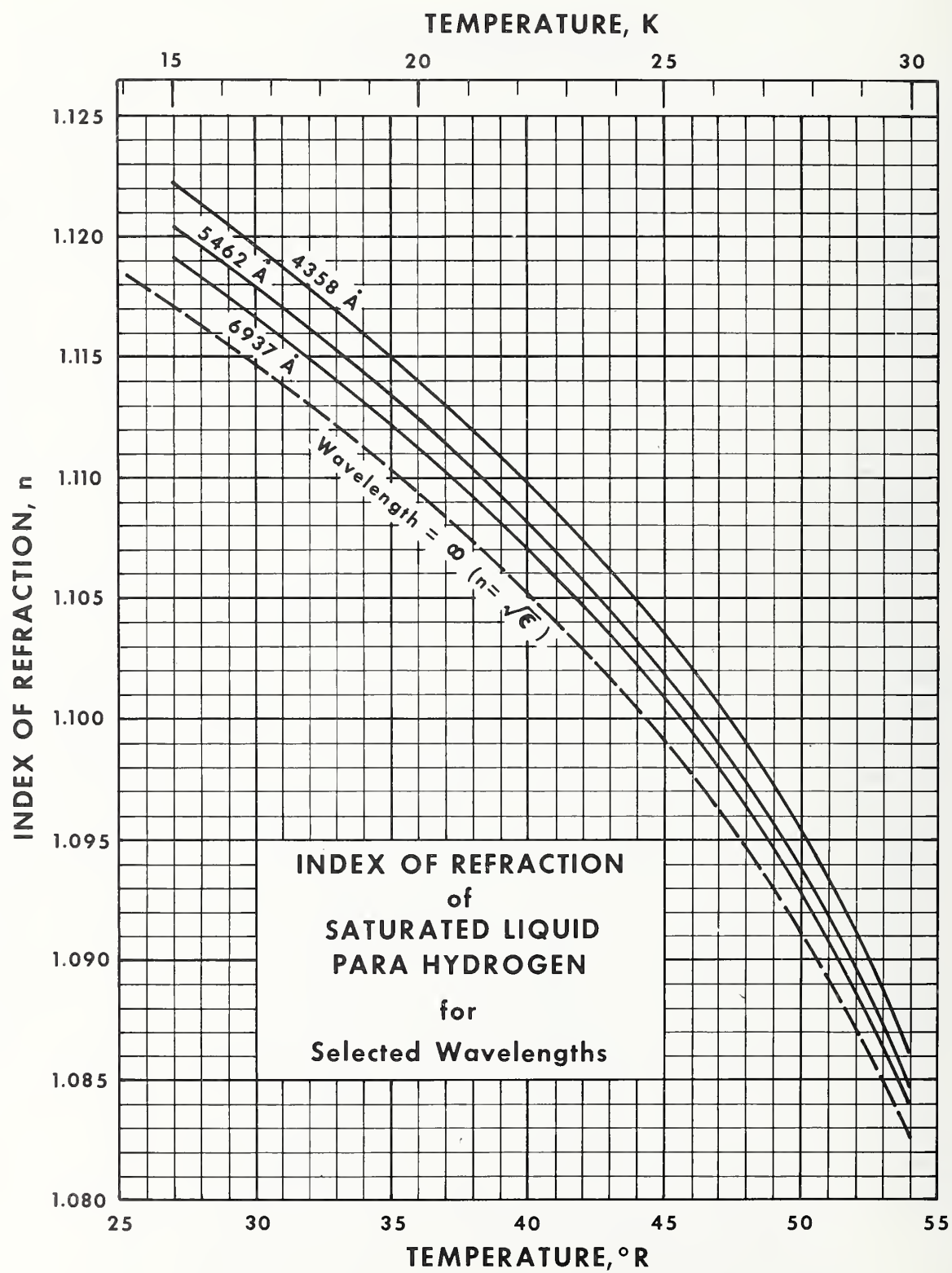
FIGURE 13. Index of refraction of saturated liquid parahydrogen.
