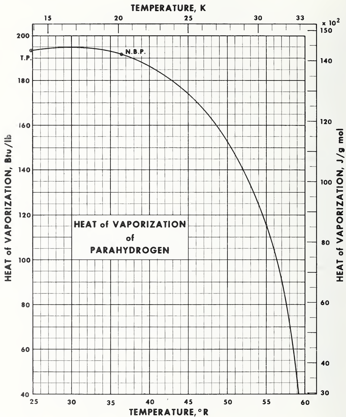
FIGURE 15. Latent heat of vaporization of parahydrogen.
