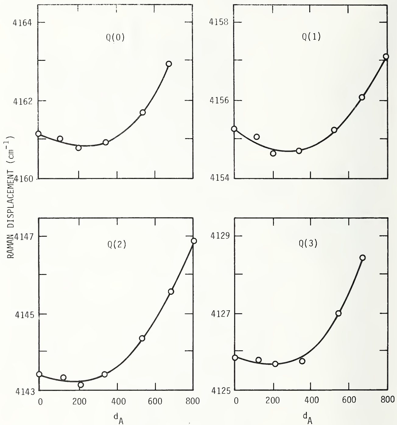
FIGURE 48. Raman displacement. Note: d_A = density in Amagats and Amagats \times 0.089881 = \text{kg/m}^3 . See Chapter 7 for density conversions.
