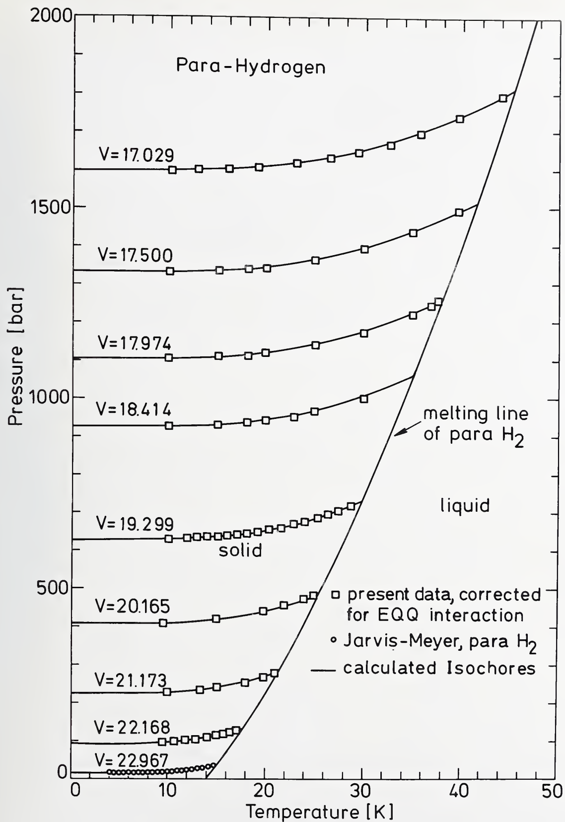
FIGURE 34c. Isochores of solid parahydrogen in the P-T plane.
