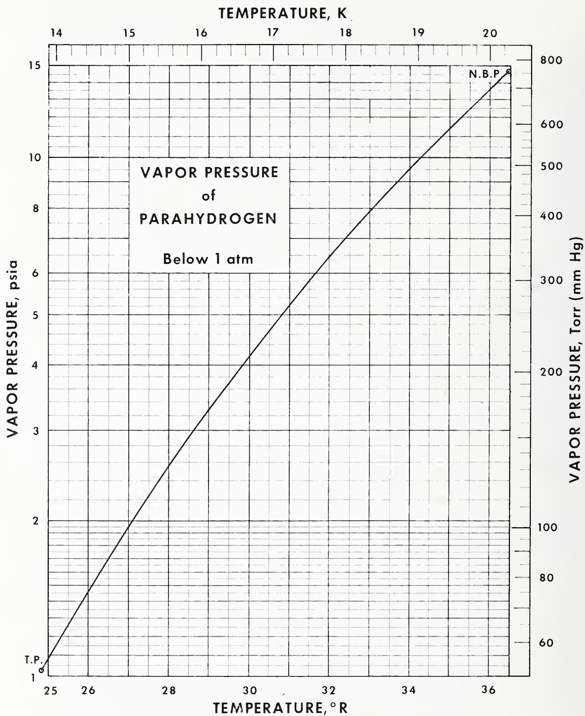
FIGURE 29. Vapor pressure of parahydrogen below 0.101325 MPa (1 atm).
