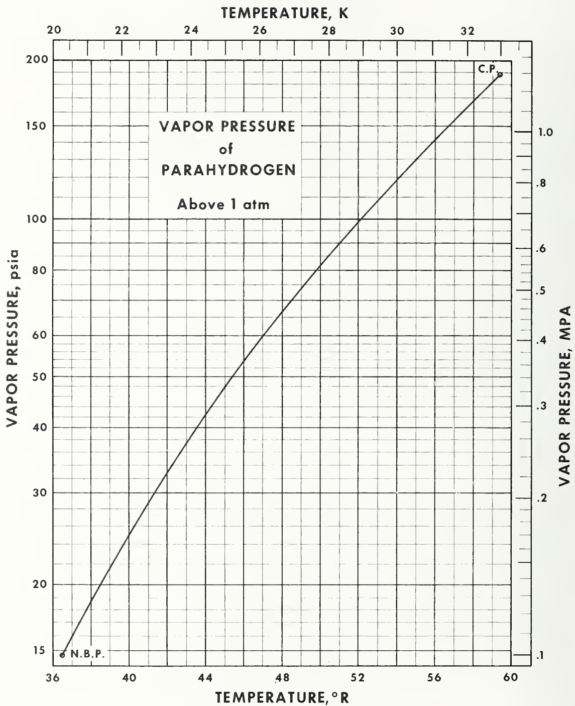
FIGURE 31. Vapor pressure of parahydrogen above 0.101325 MPa (1 atm).
