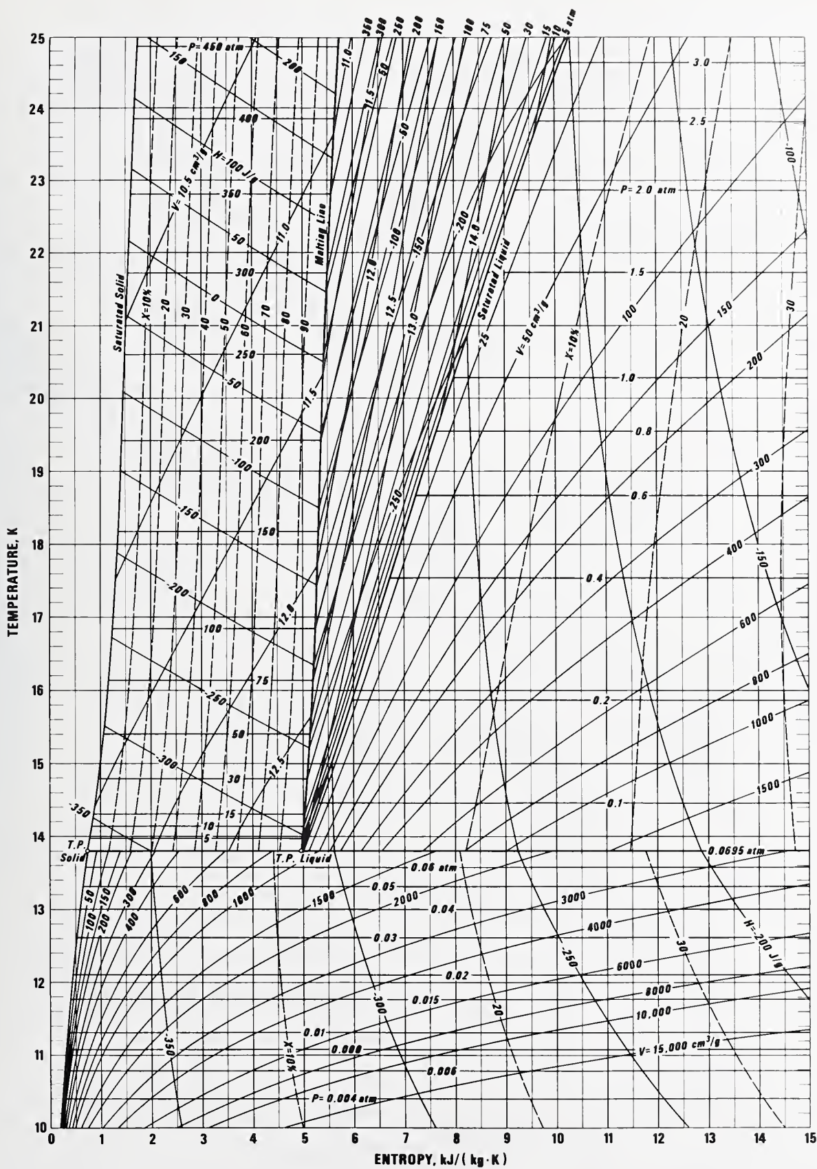
FIGURE 43. Parahydrogen, temperature-entropy diagram (10 to 25 K).
