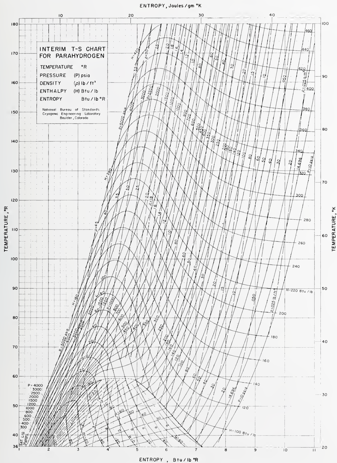
FIGURE 4. Parahydrogen temperature-entropy chart (20 to 100 K).
