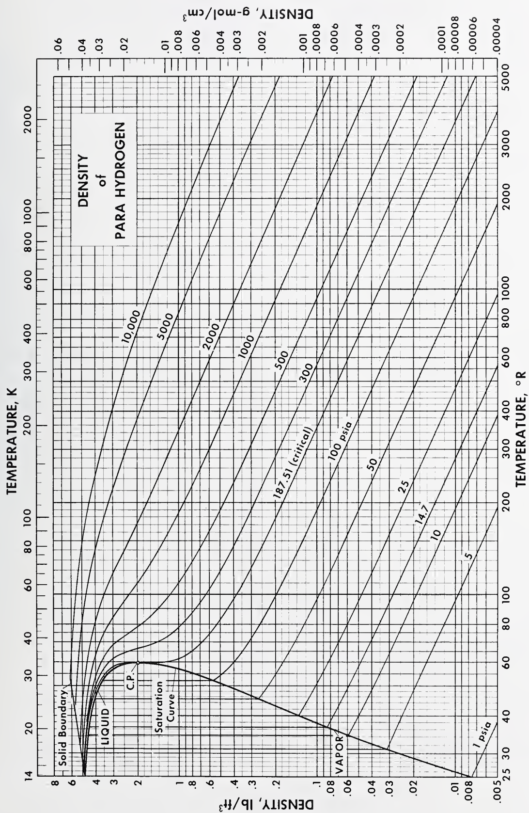
FIGURE 20. Density (P-ρ-T) of parahydrogen.
