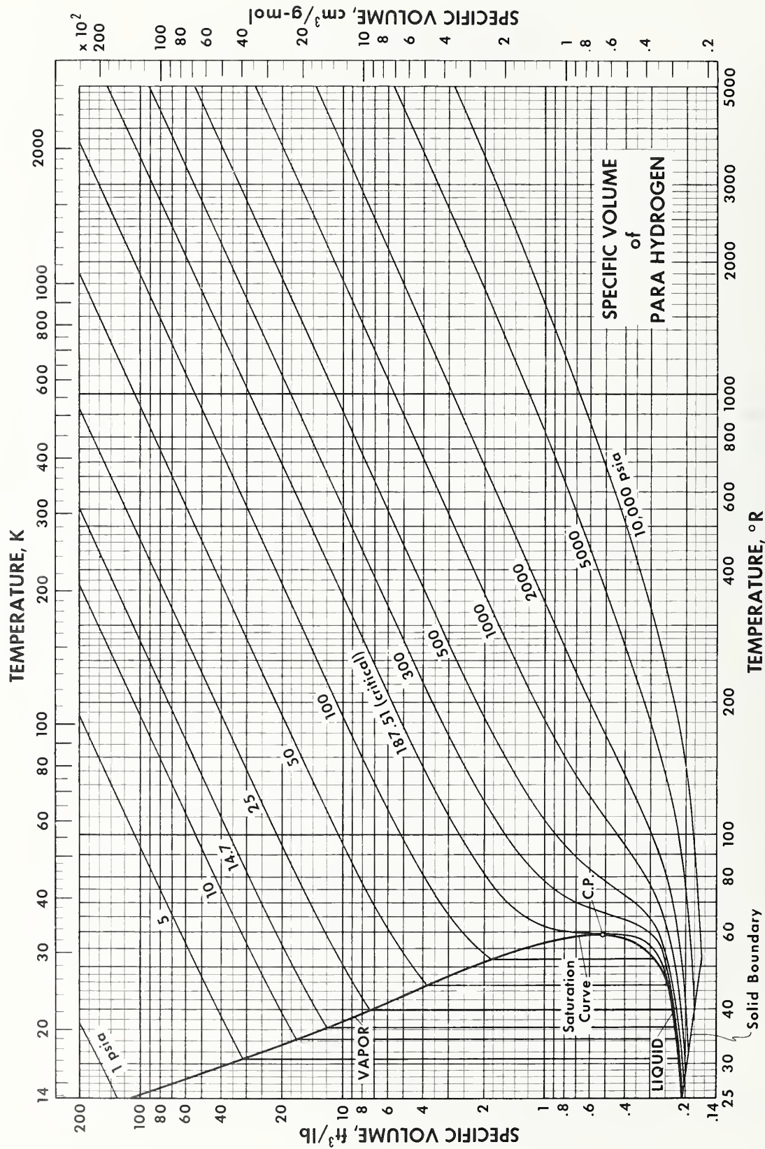
FIGURE 19. Specific volume (PVT) of parahydrogen.
