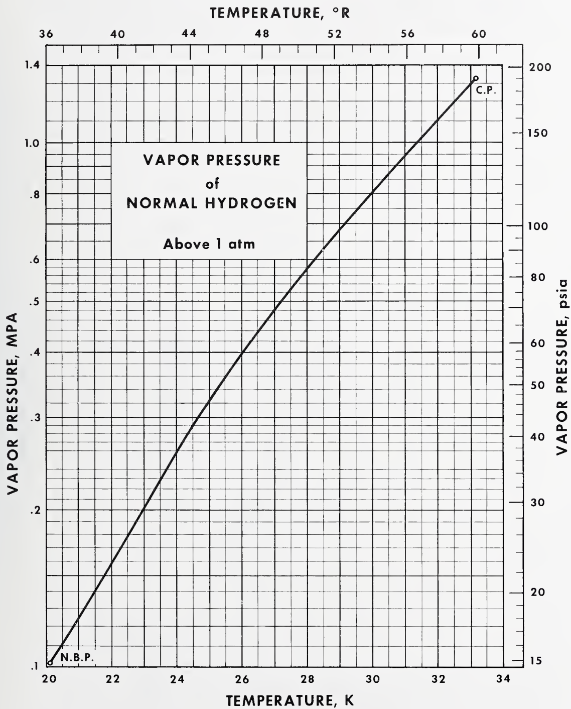
FIGURE 32. Vapor pressure of normal hydrogen above 0.101325 MPa (1 atm).
