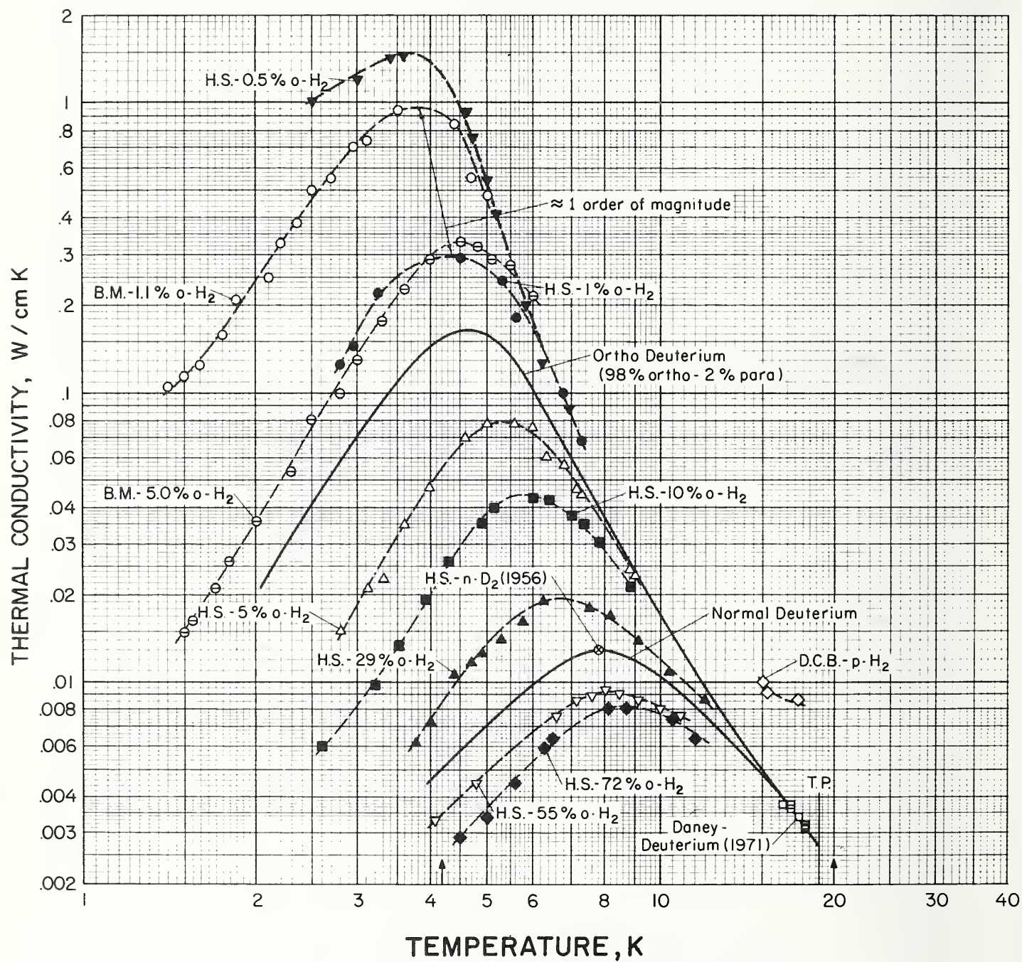
FIGURE 42. Thermal conductivity of solid hydrogen.
