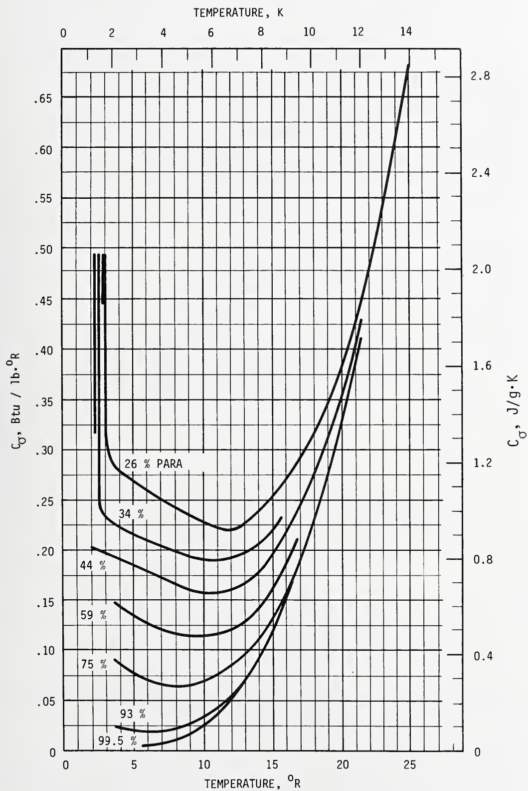
FIGURE 38. Specific heat (heat capacity) of saturated solid hydrogen.
