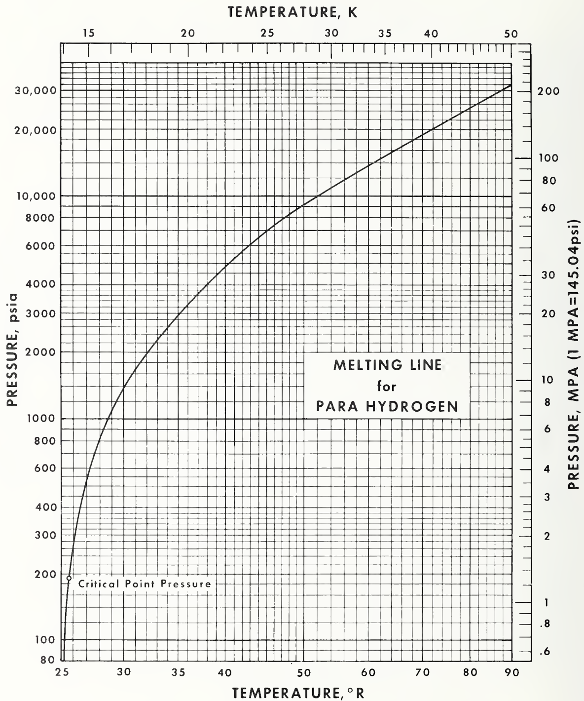
FIGURE 17. Melting line for parahydrogen (0.6 to 200 MPa).
