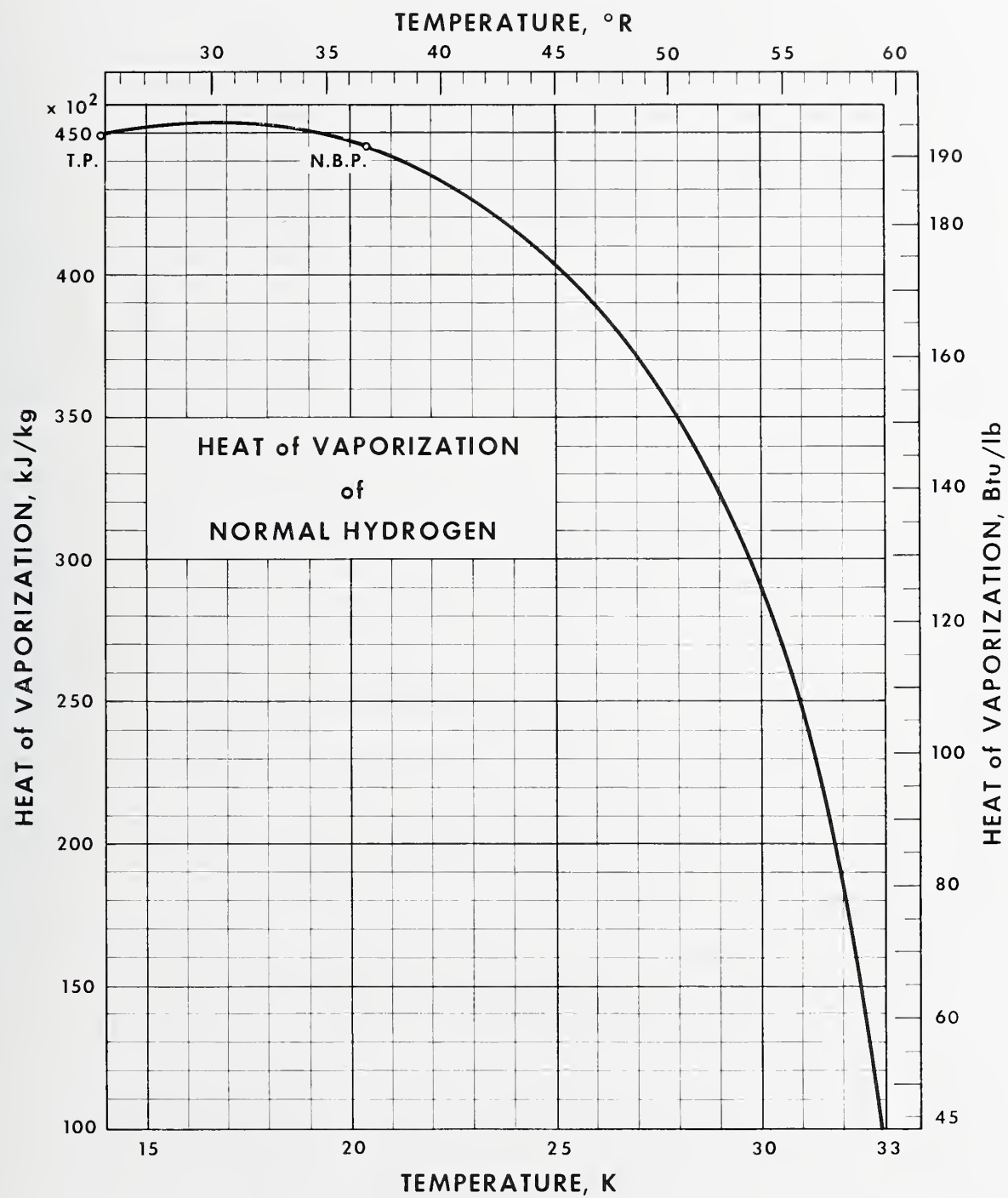
FIGURE 16. Latent heat of vaporization of normal hydrogen.
