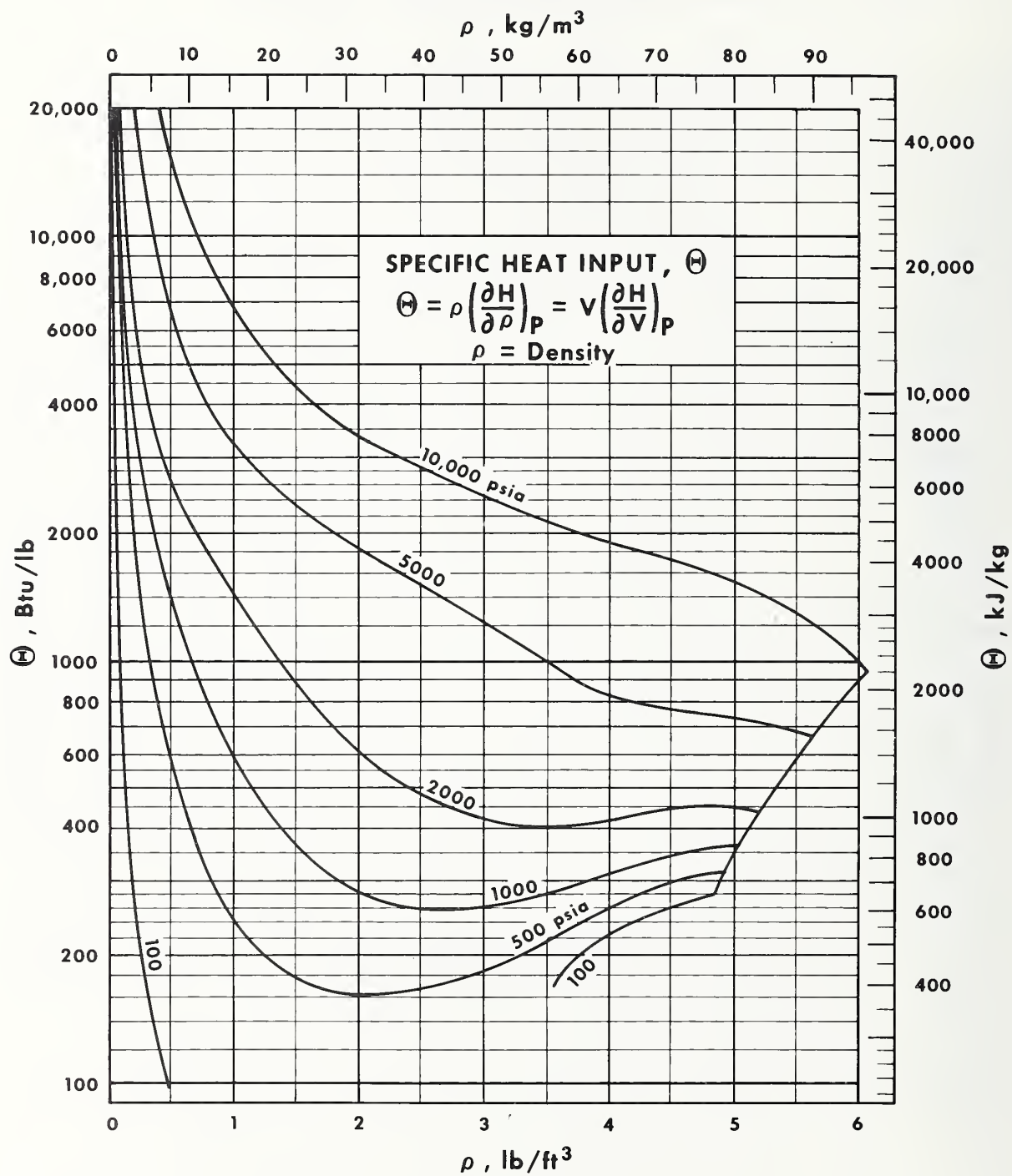
FIGURE 60. Specific heat input function for hydrogen.
