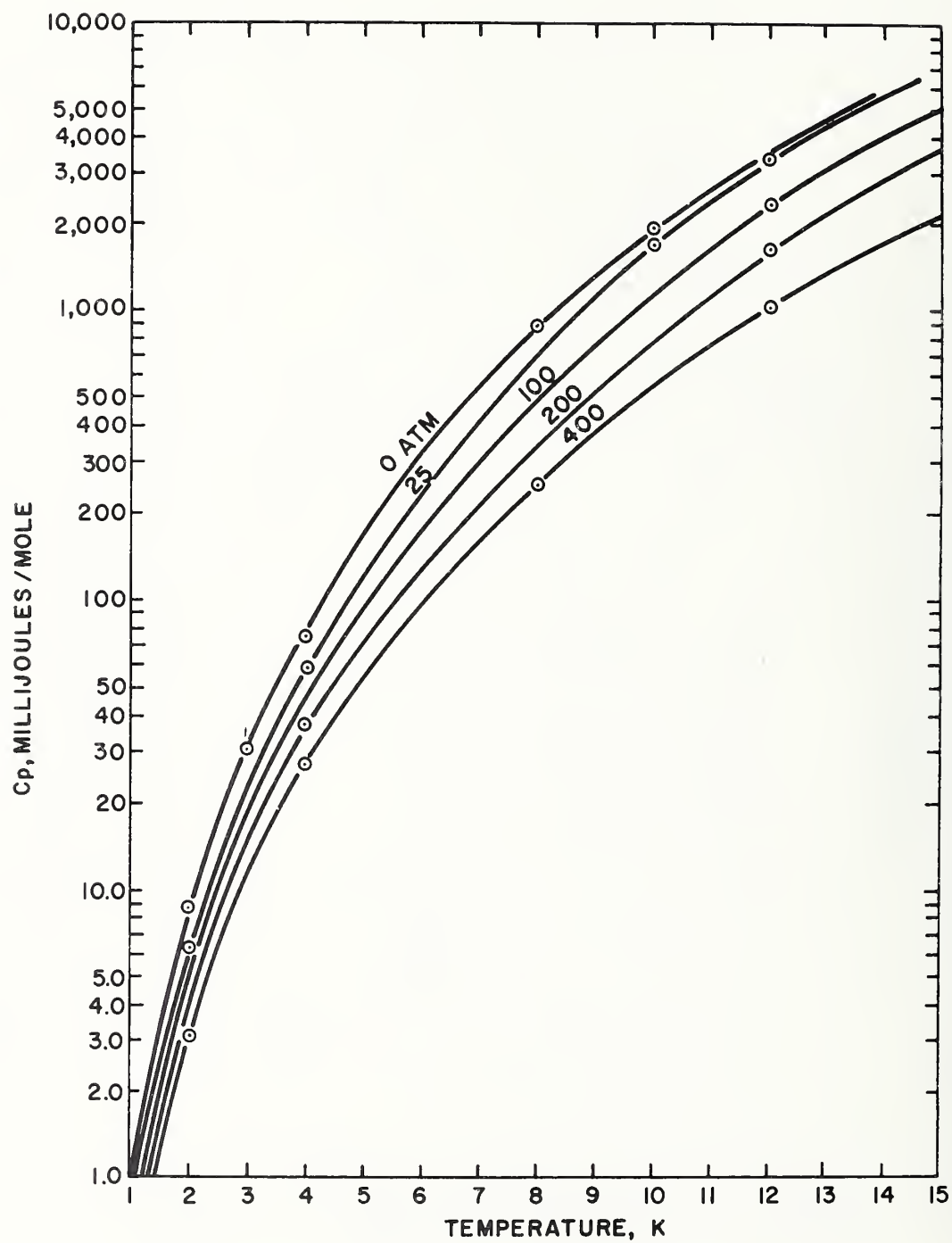
FIGURE 37. Isobars of C_p for compressed solid parahydrogen.
