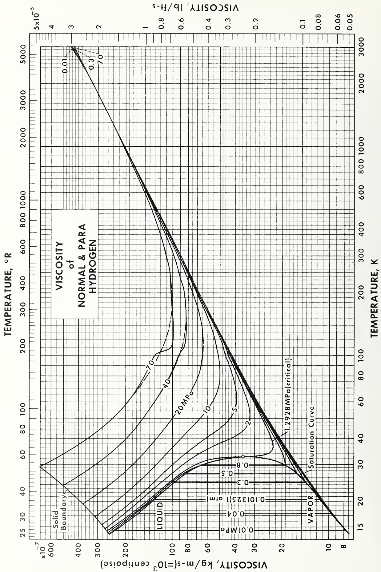
FIGURE 33. Viscosity of normal and parahydrogen.
