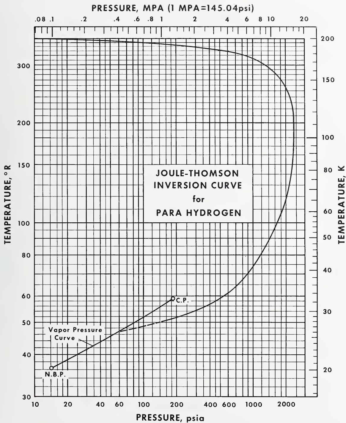
Figure 14. Joule-Thomson inversion curve for parahydrogen.
