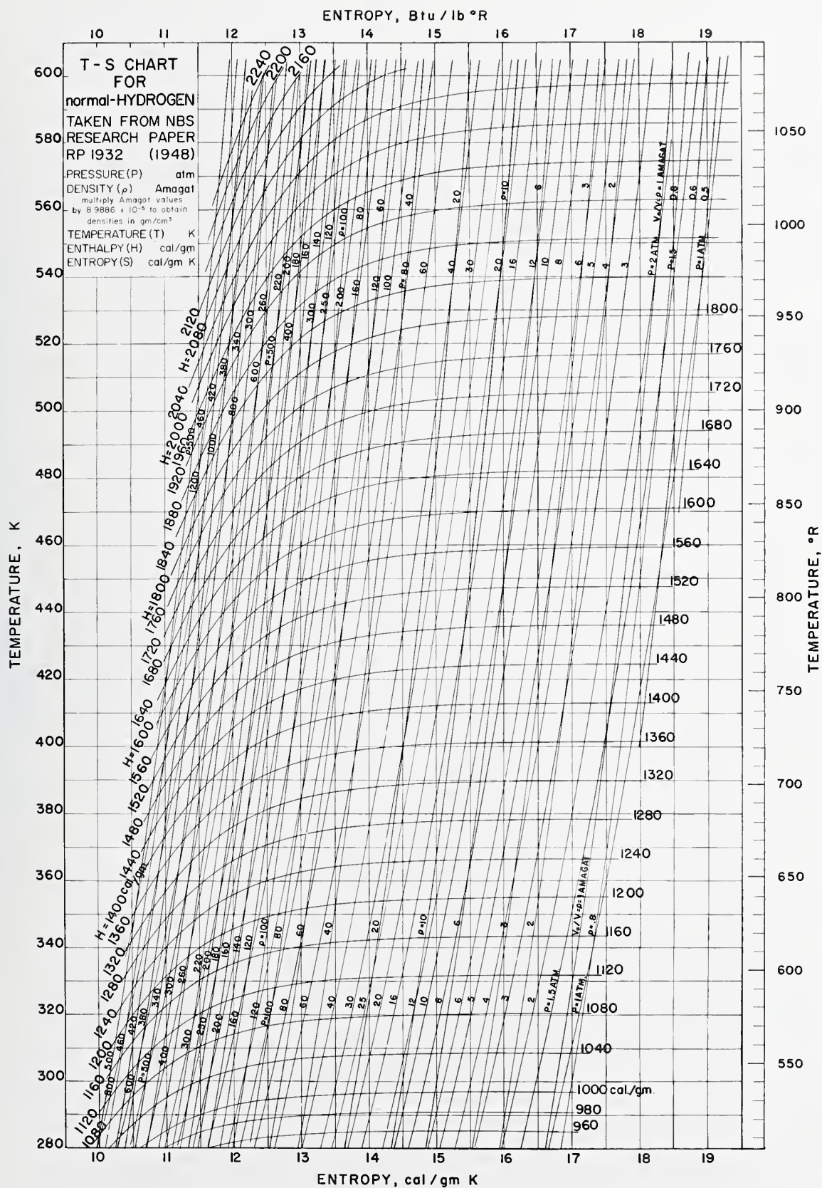
FIGURE 8. Normal hydrogen temperature-entropy chart (280 to 600 K).
