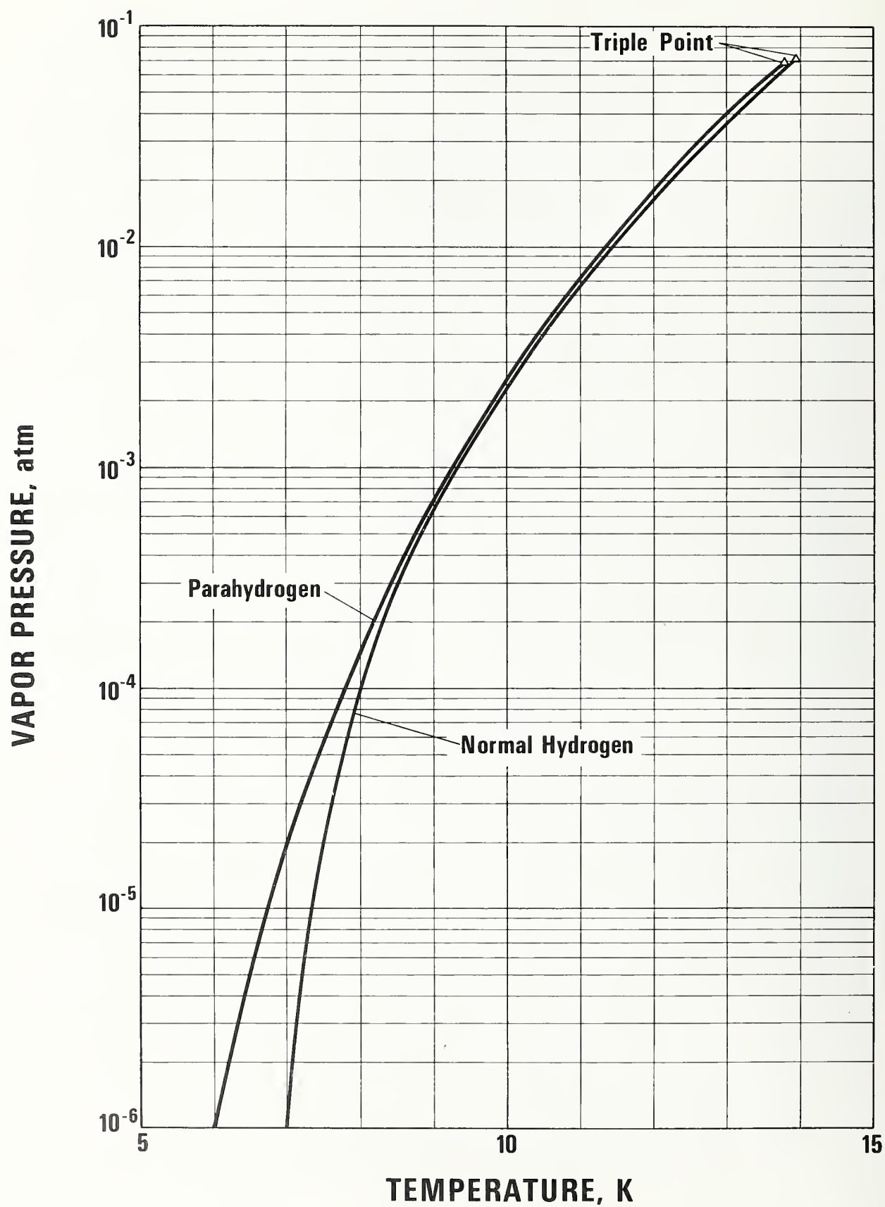
FIGURE 44. Vapor pressures of hydrogen below the triple point.
