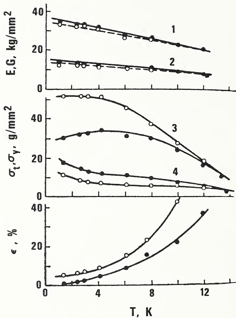
FIGURE 39. Temperature dependencies of the mechanical properties of normal and parahydrogen.
