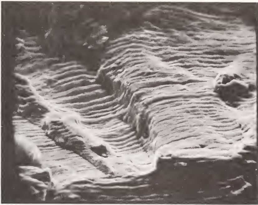
Figure 2. Scanning electron microscope photomicrograph (2100X) illustrating mechanical fatigue failure of a stainless steel (ASTM F-55) bone plate.
