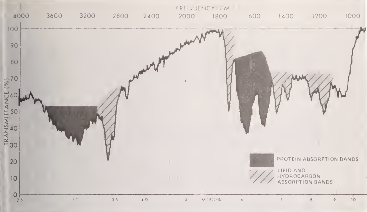
Figure 7A. Internal reflection infrared spectrum of the blood flow surface of a stabilized human umbilical cord vein harvested patent after 8-months implantation as a human arterial prosthesis.
