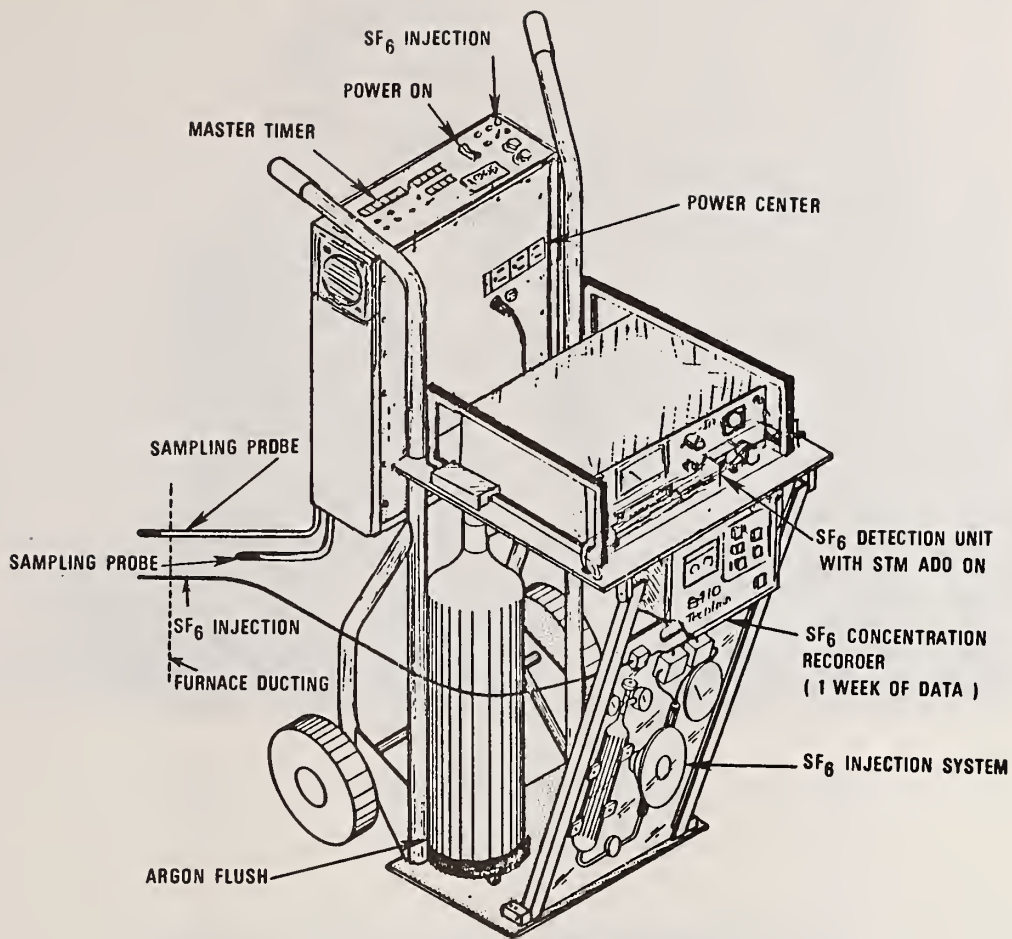
FIGURE 20 - EQUIPMENT FOR \text{SF}_6 TRACER GAS AIR EXCHANGE MEASUREMENT.
