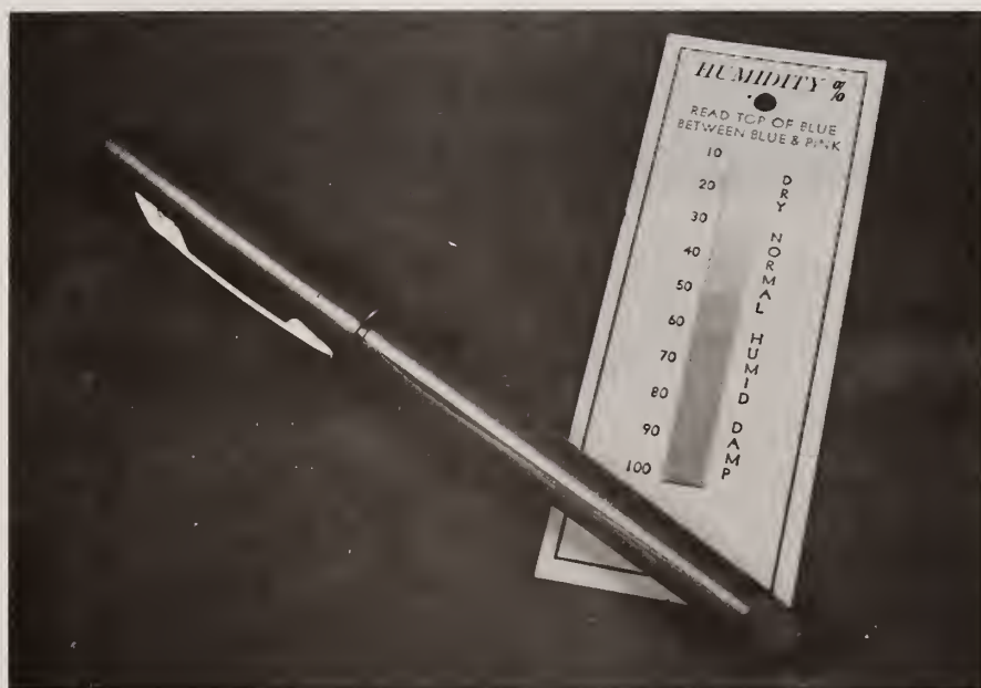
FIGURE 2 - PHOTOGRAPH OF COLOR CHANGE RELATIVE HUMIDITY INDICATOR.
