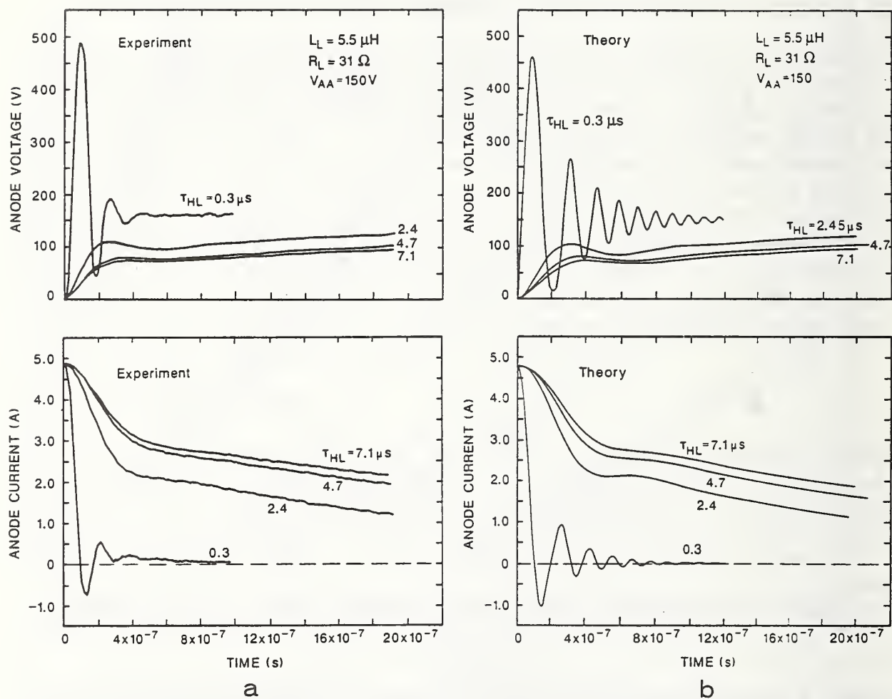
Figure 39. The measured (a) and simulated (b) series 31\text{-}\Omega resistor, 5.5\text{-}\mu\text{H} inductor load current and voltage waveforms for devices with different lifetimes.
