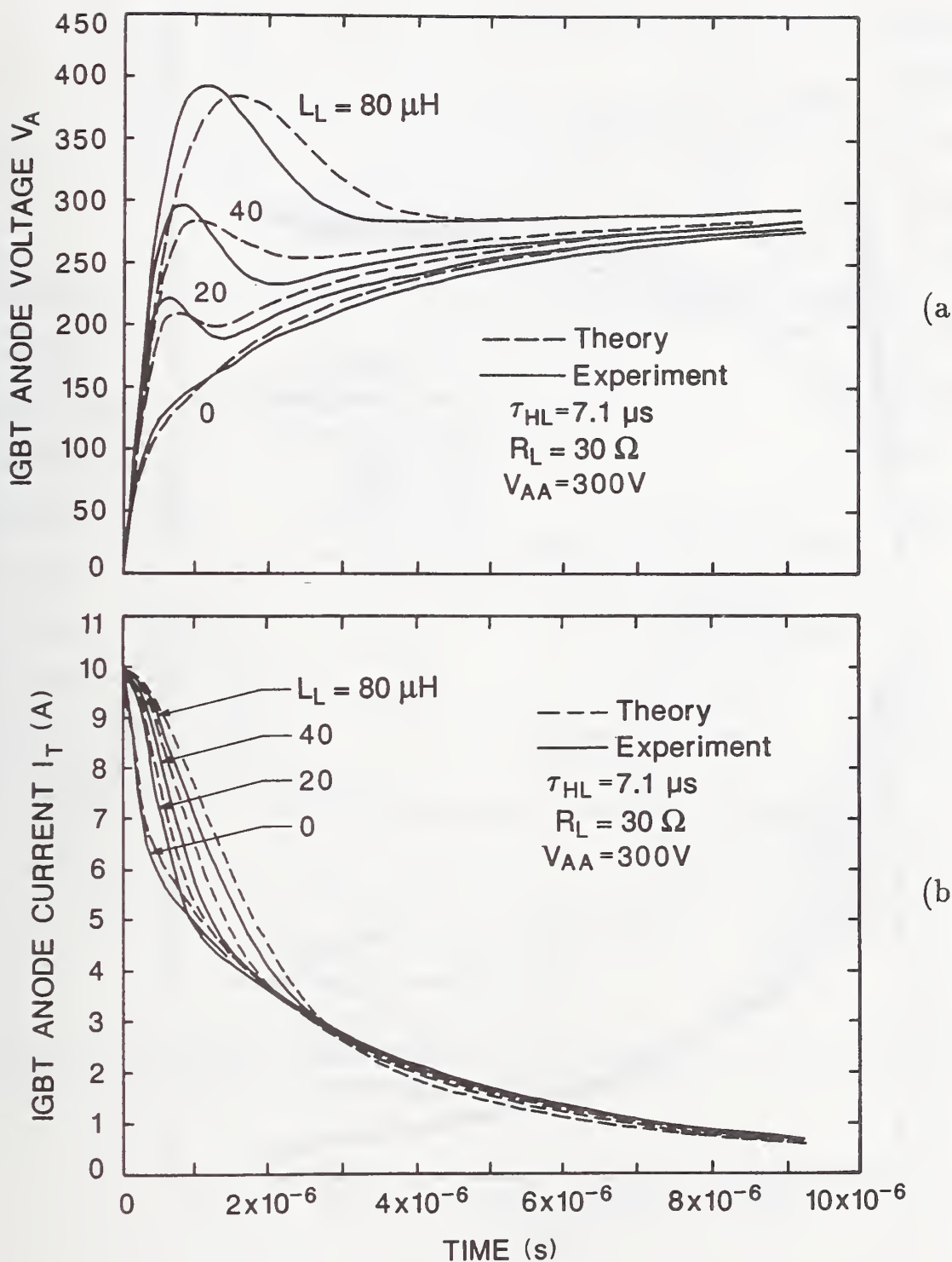
Figure 40. The measured and simulated series resistor-inductor load voltage (a) and current (b) waveforms for a 7.1- \mu\text{s} device and inductances from 0 to 80 \mu\text{H} .
