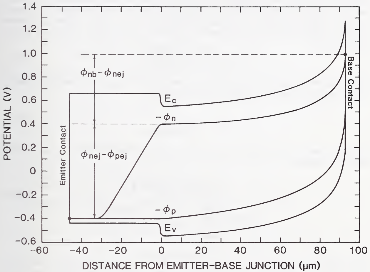
Figure A3.1. The band diagram from the emitter to base contacts for an IGBT with the physical parameters listed in tables 4 and 5, and a base lifetime of \tau_B = 1 \mu\text{s} , indicating the electron quasi-fermi potential drops in the emitter ( \phi_{nej} - \phi_{pej} ) and across the base ( \phi_{nb} - \phi_{nej} ).
