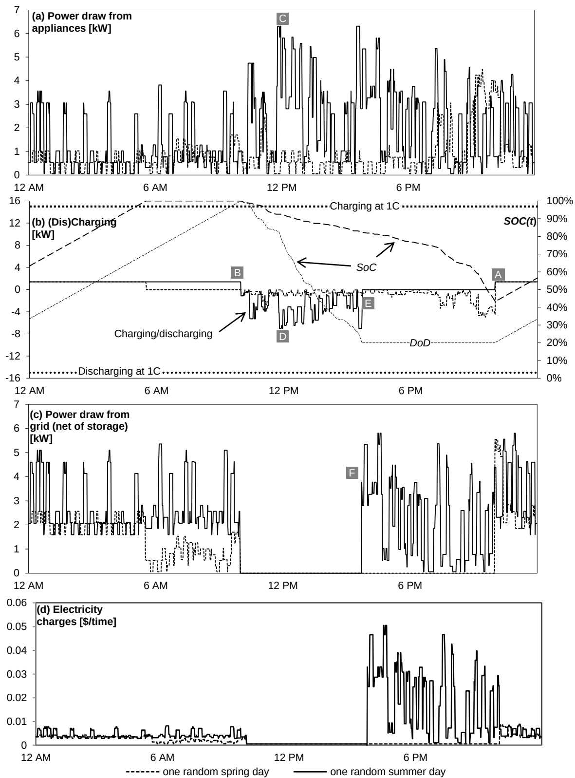
Figure 14. Data traces generated by the loadshifting strategy
