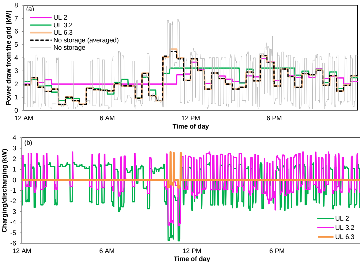
Figure 21. Demand profile simulations and storage (dis) charging patterns by implementing different operating ULs ( EC = 4.6 kWh).
