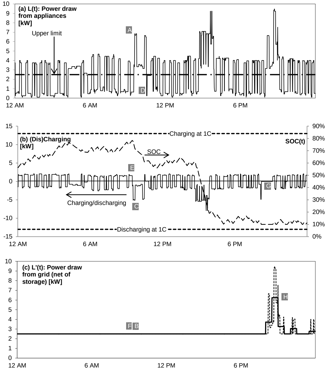
Figure 17. Data traces generated by the peak reduction strategy.
