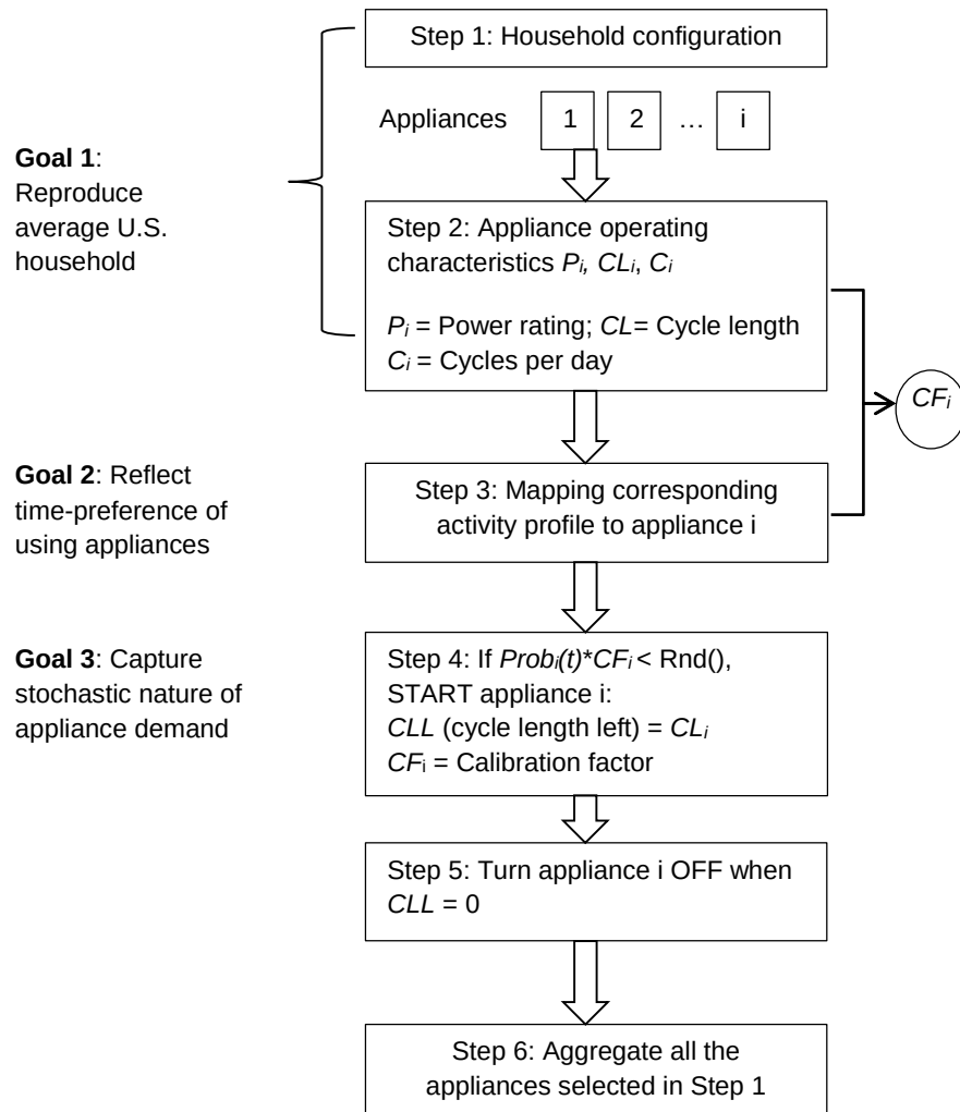
Figure 5. Illustration of the stochastic demand profile model.
