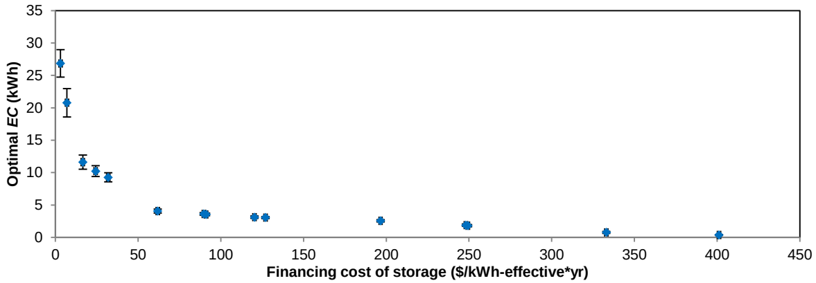
Figure 23. Optimal ECs for a variety of storage costs in the average-case scenario (peak reduction). Error bars represent one standard deviation above and below the mean.
