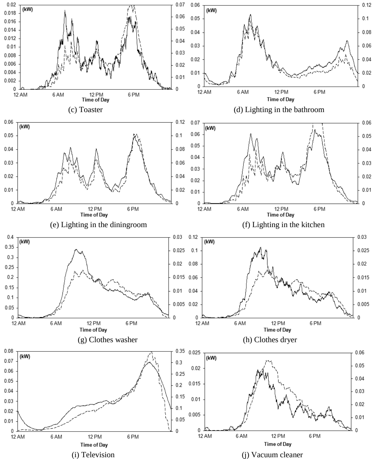
Figure 8 4 . Mean load curve from simulations and in-use probability profile from ATUS [57].
