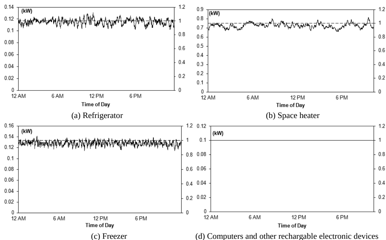
Figure 10 6 . Mean load curve from simulations and flat in-use probability profile
