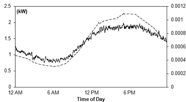
Figure 9 5 . Mean load curve from simulations and in-use probability profile for air-conditioning.
