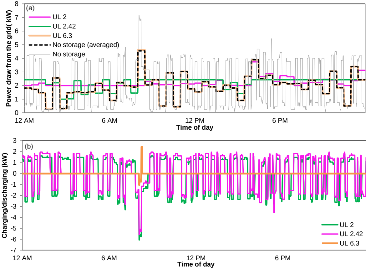
Figure 22. Demand profile simulations and storage (dis)charging patterns by implementing different operating UL s ( EC = 23.7 kWh)
