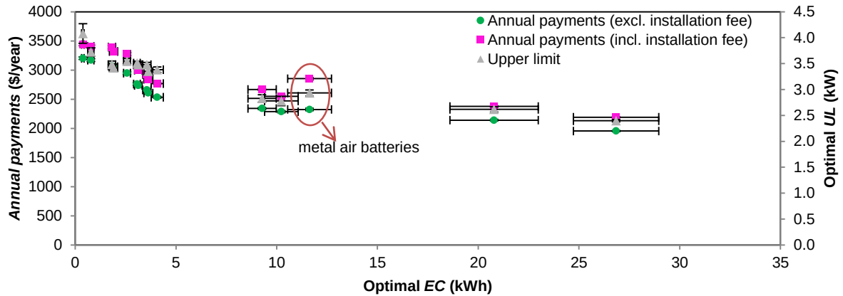
Figure 24. Annual payments and optimal ULs for a variety of storage options in the average case scenario (peak reduction). Error bars represent one standard deviation above and below the mean.
