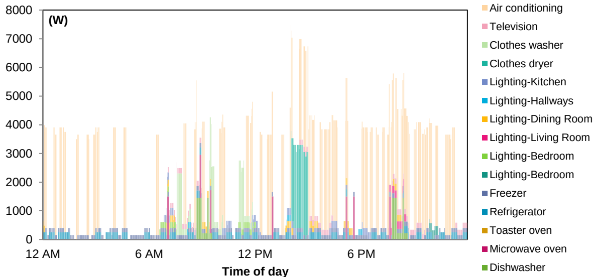
Figure 7. An example of one household demand profile generated by aggregating appliances demand profiles
