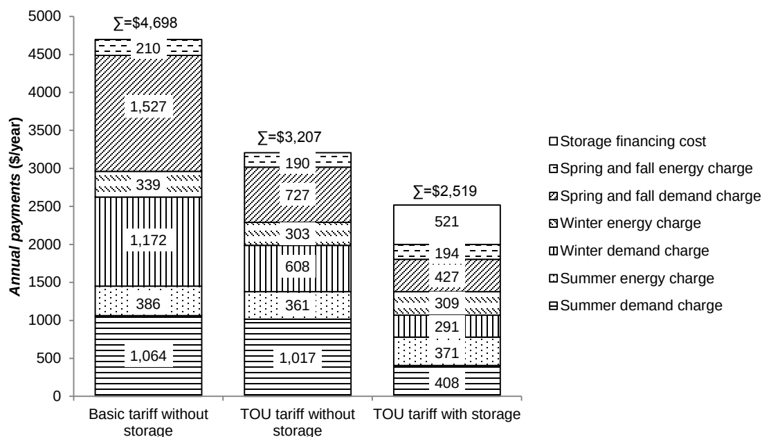
Figure 18. Annual payments breakdowns (under the kW tariff).
