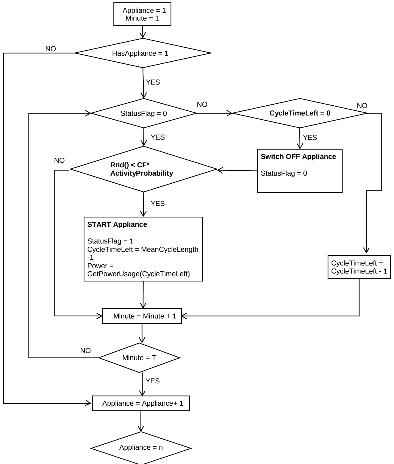
Figure 6 3 . Flow chart of agent-based logic in the appliance demand profile model.
