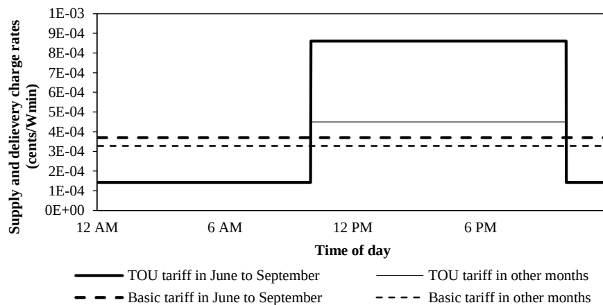
Figure 3. Daily electricity charge rates (supply and delivery, excluding monthly service fees).
