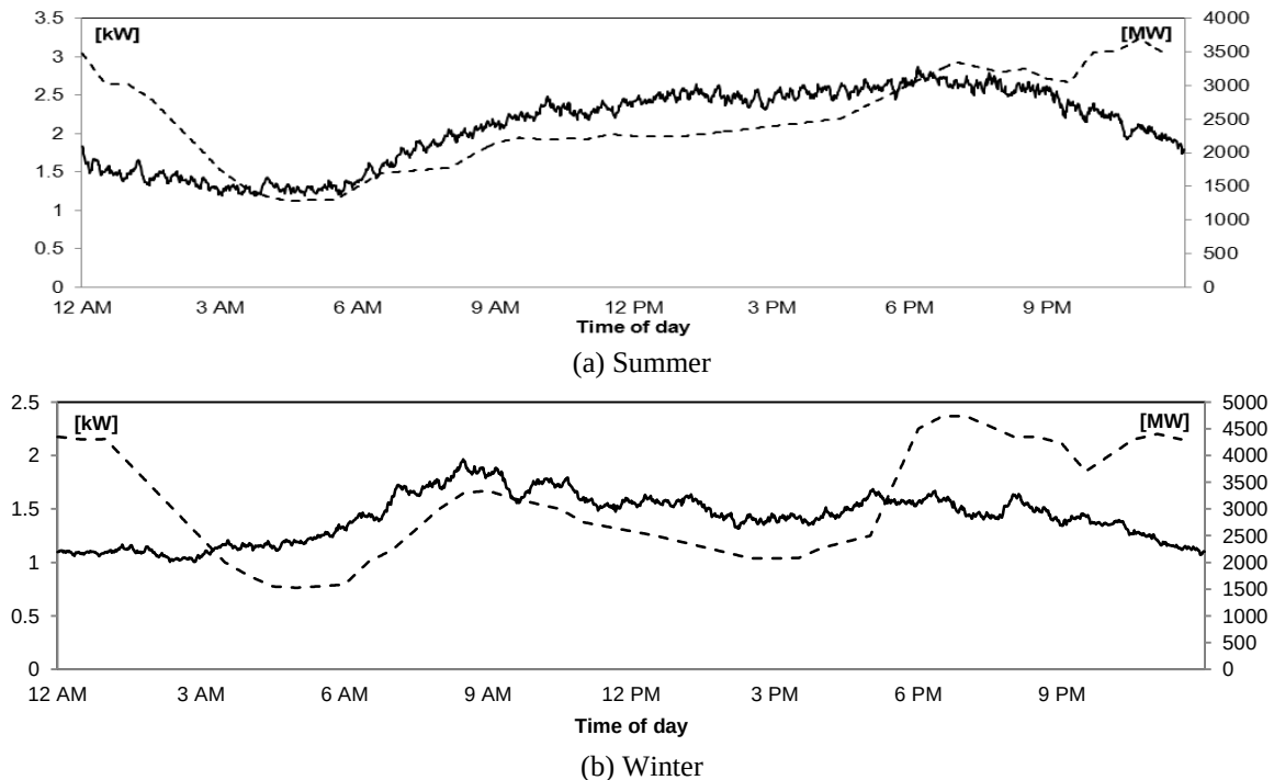
Figure 13. 8 Mean load curve from simulations versus aggregated demand curves reproduced from EMET[60].
