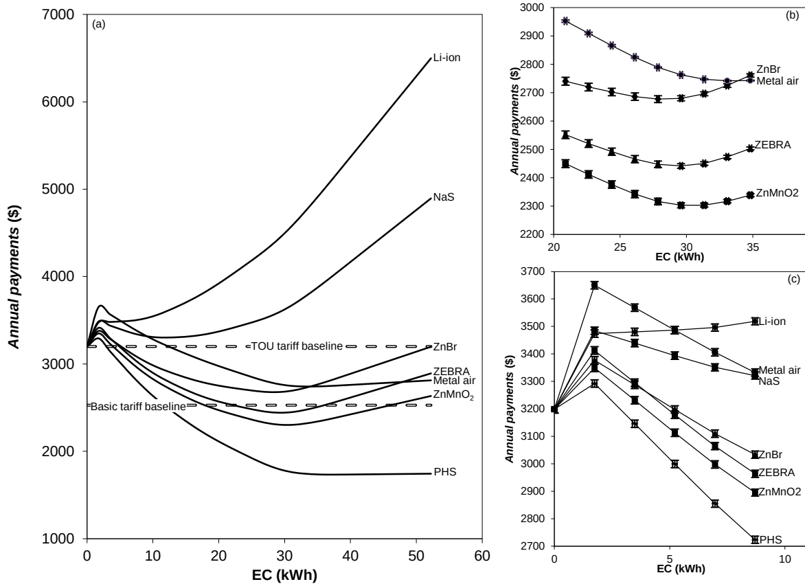
Figure 16. Annual payments for various storage technologies and capacities (loadshifting). Error bars represent one standard deviation above and below the mean.
