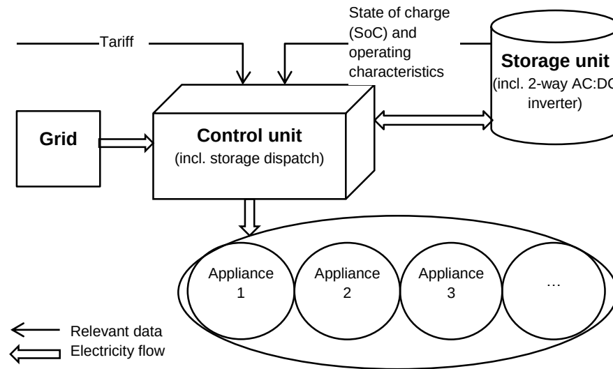
Figure 1. DR scheme and flows of relevant data and electricity.
