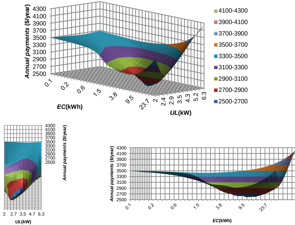
Figure 19. Surface plot of annual payments with varying EC s and varying UL s (peak reduction).
