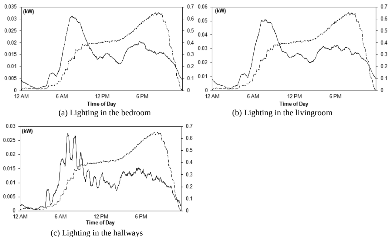
Figure 11 7 . Mean load curve from simulations and respondents being at home and awake probability profile.
