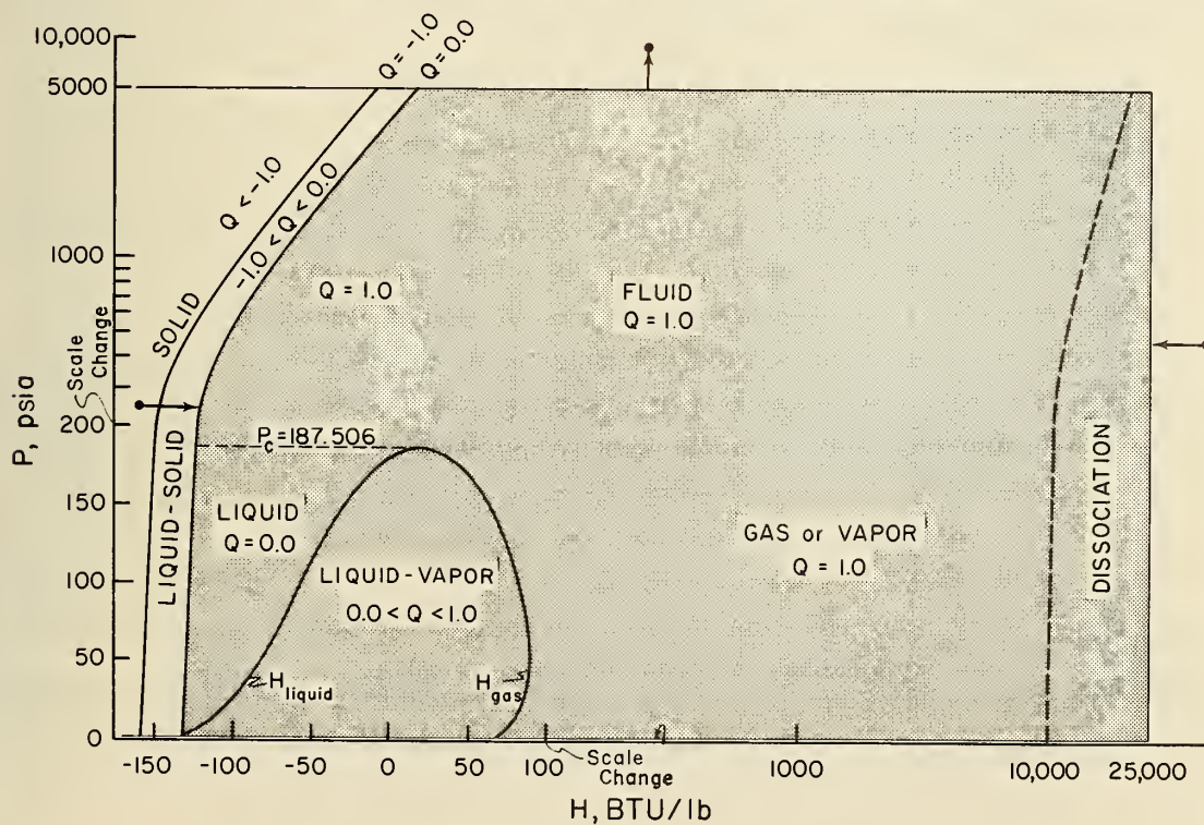
Figure 4. The P-H Phase Diagram for Parahydrogen
