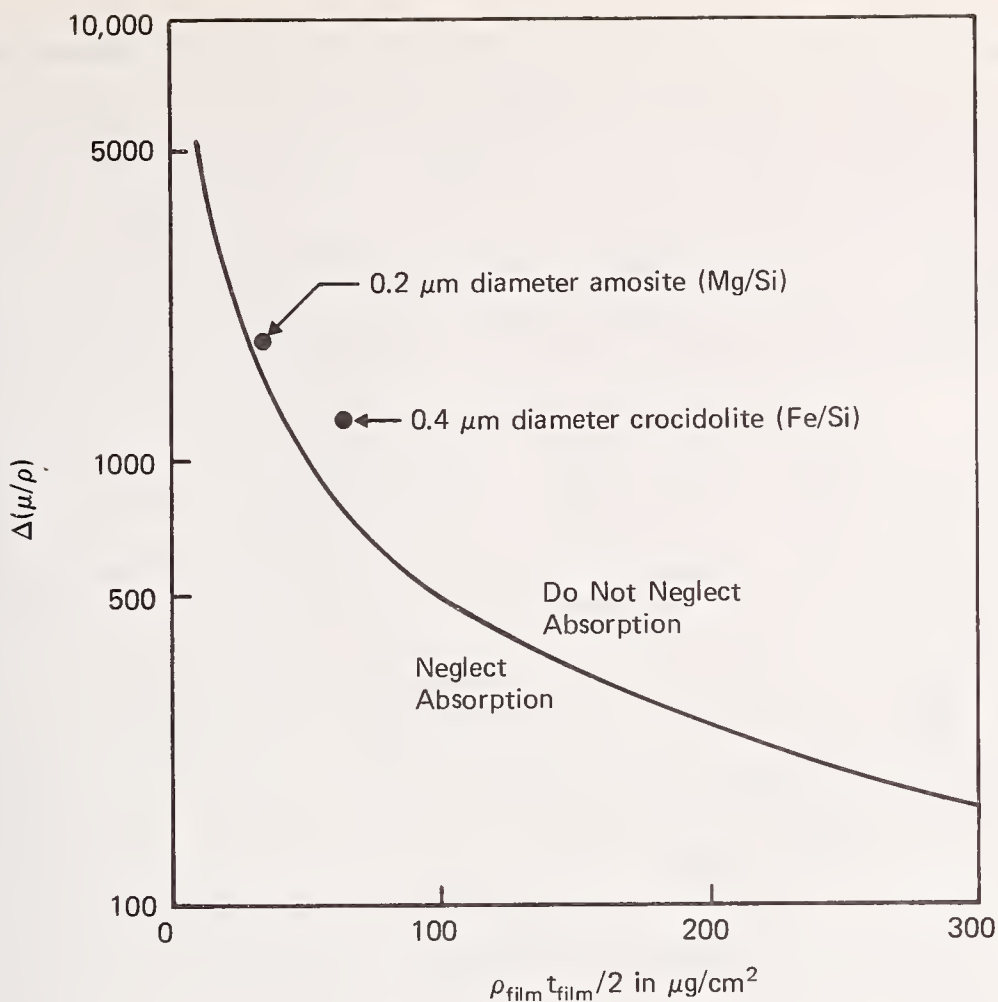
Figure 4. \Delta(\mu/\rho) = \mu/\rho \left|_{\text{film}}^{\text{B line}} - \mu/\rho \left|_{\text{film}}^{\text{A line}}\right.\right. (\rho t)_{\text{film}} = film mass thickness.
