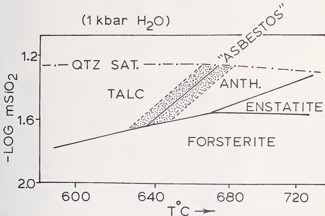
Figure 4. Adaptation of the enstatite-anthophyllite-talc-forsterite stability relationships at 1 kbar H 2 O to show a possible stability or metastability field of "talcbolcs asbestos" (stippled). Figure modified from Hemley et al. [13]. anth. = anthophyllite.
