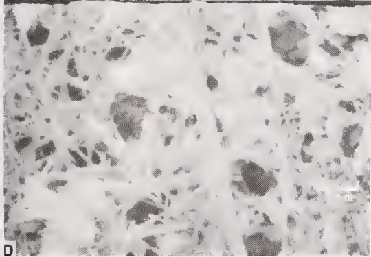
Figure 11. Mixture of nonasbestiform serpentine and chrysotile at five magnifications: A , X 450; B , X 2,250; C , X 1,800; D , X 9,000; and E , X 18,000. Rectangles indicate the area shown in the next panel.
