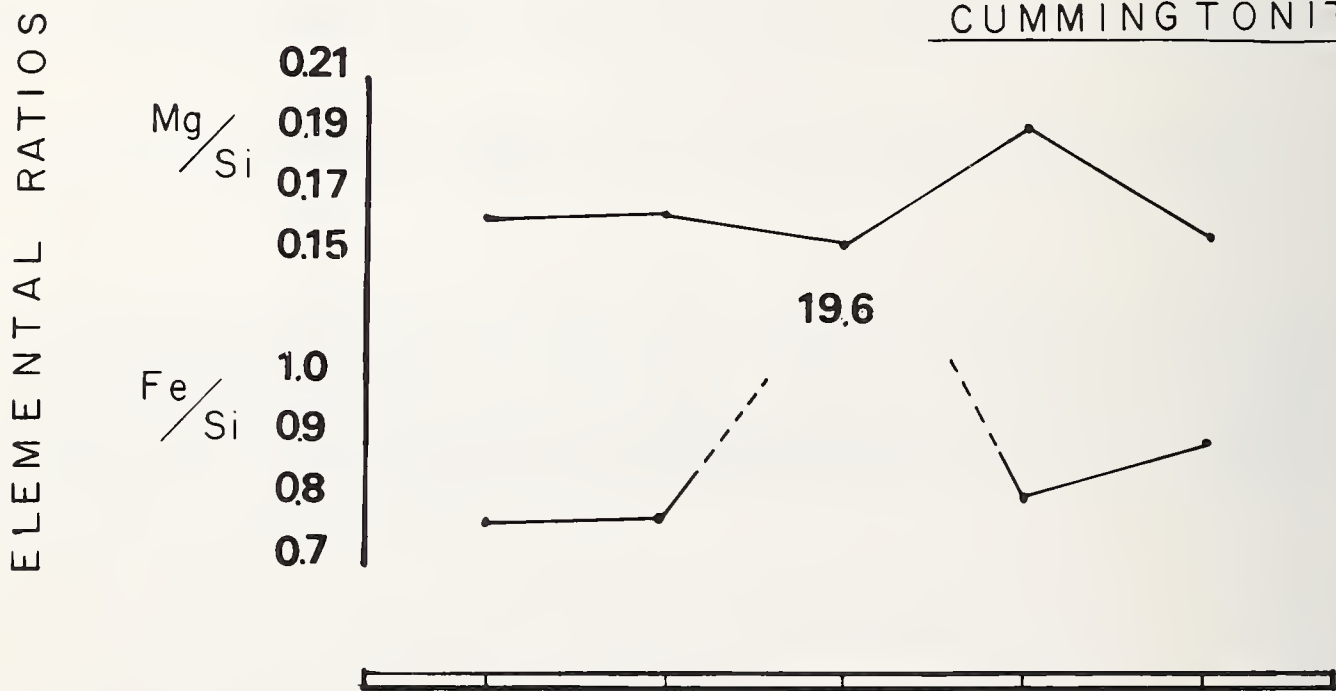
ANALYZED SPOTS (CUMMINGTONITE FIBERS 16 μm. dia. 0.2 μm.)
