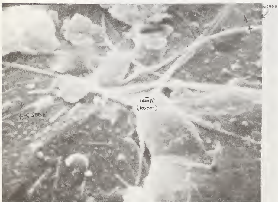
Figure 6. Spiked talc by SEM. 1.5% chrysotile x 13,500 at 35°.
