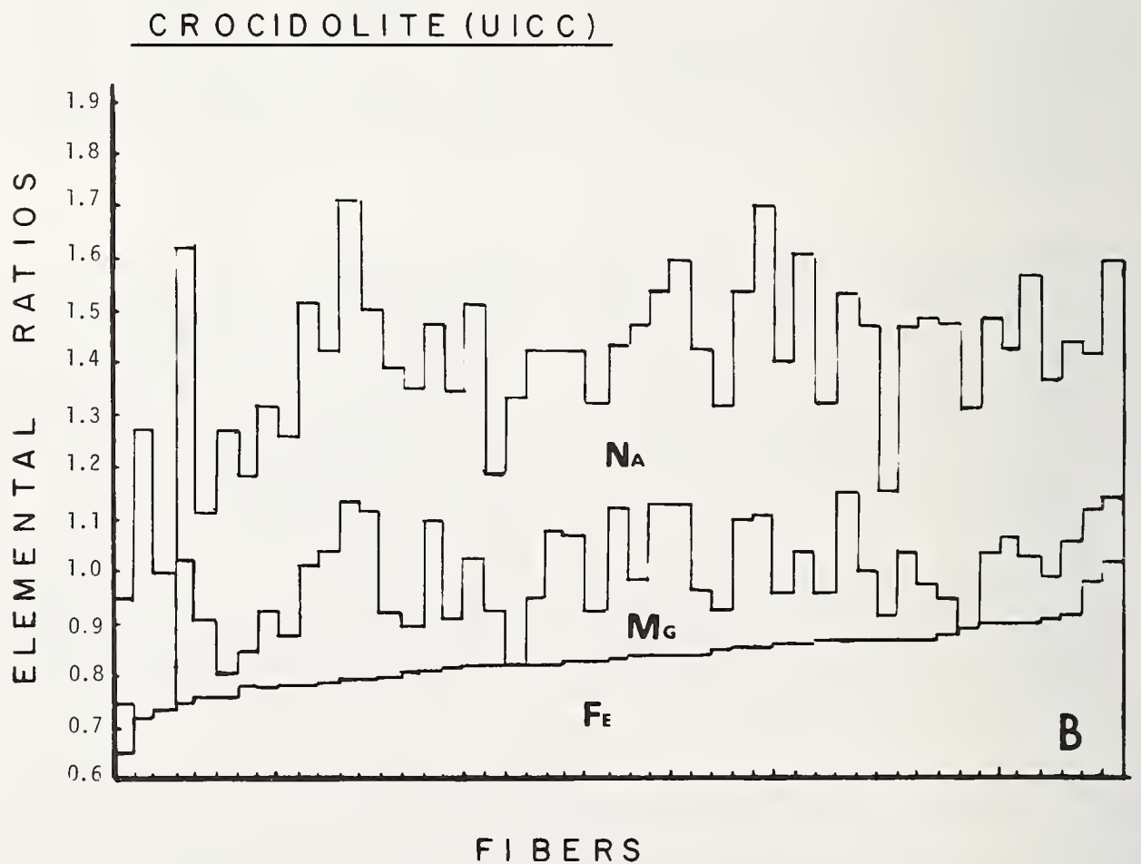
Figure 3. Corrected intensity ratios for UICC amosite (a) and UICC crocidolite (b). Intensity ratios are cumulative with the value for each element depicted as the difference between adjacent horizontal bars.
