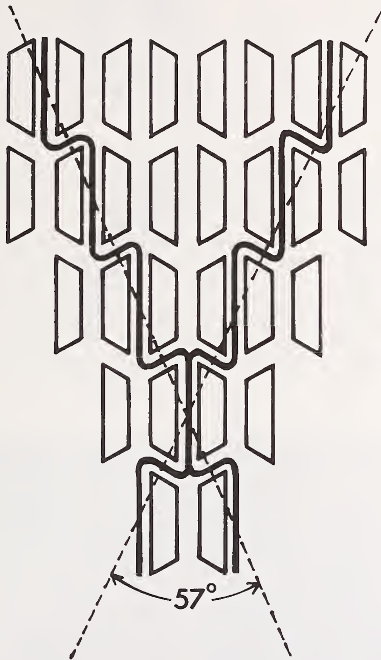
Figure 3. Schematic view of amphibole structure as seen down z axis, showing likely paths of weakness leading to cleavages intersecting at 57°.
