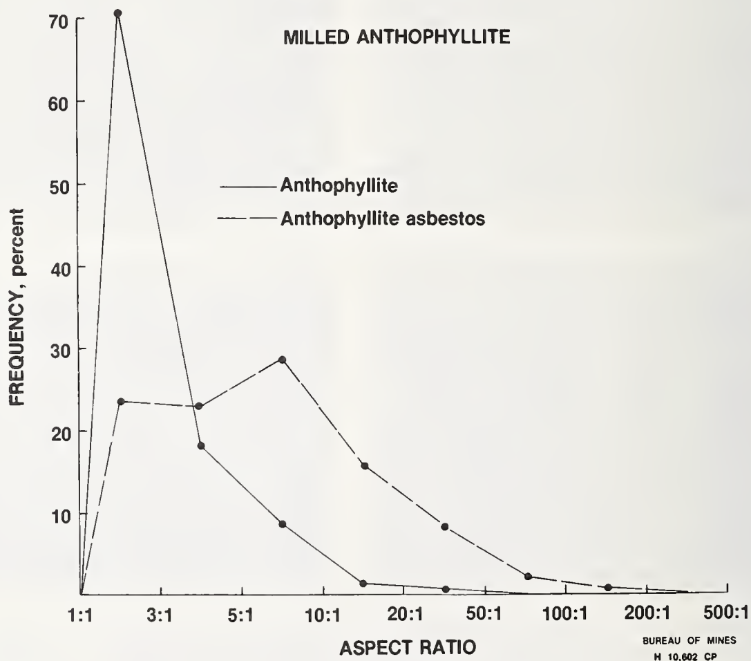
Figure 6. Frequency polygons for the aspect ratios of anthophyllite and anthophyllite asbestos.
