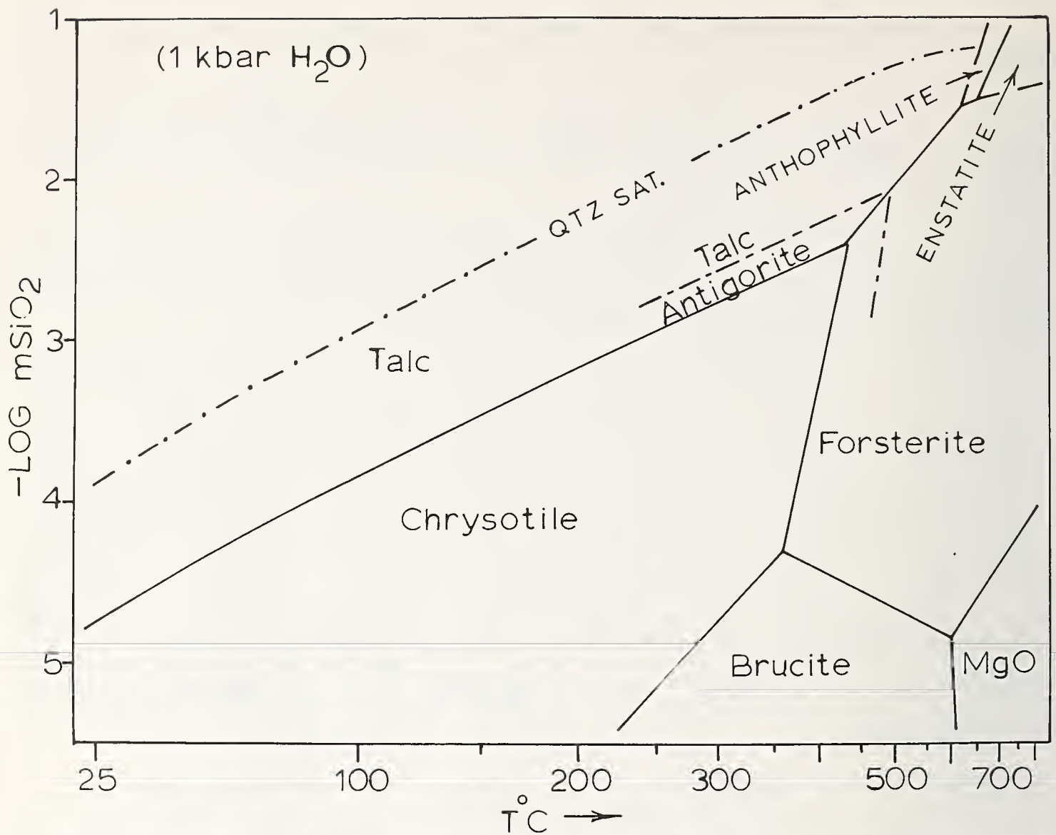
Figure 3. Mineral stability relations in the system MgO-SiO_2-H_2O as a function of log of molality of aqueous silica and temperature, at 1 kilobar H_2O pressure. Figure modified from Hemley et al. [13].
